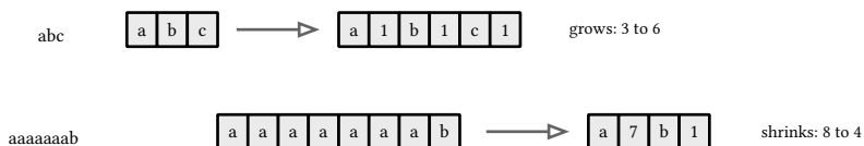
figure 27: counts always emitted: singles grow, runs shrink
