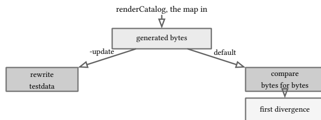
figure 72: two branches: compare by default, rewrite through the flag
