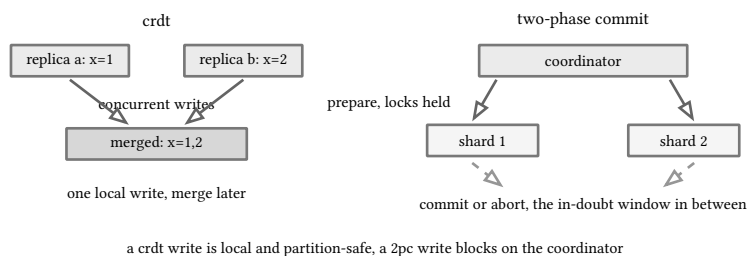
figure 116: merge converges with no coordinator, prepare and commit hold locks across round trips
