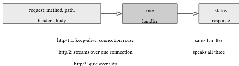
figure 82: request in, status out, one handler across versions
