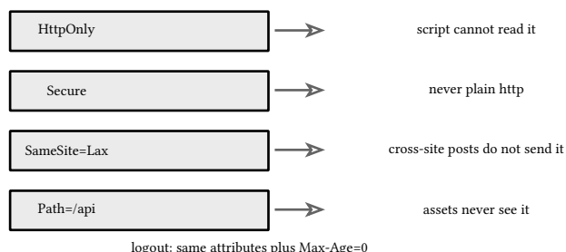
figure 150: the cookie's attributes, each one closing a named hole
