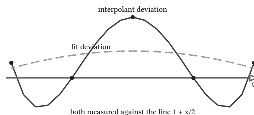
figure 130: deviation from the generating line: the interpolant swings, the fit stays flat
