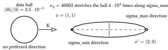
figure 141: the input ball mapped through the matrix to a kappa-stretched ellipse, the flip as one endpoint
