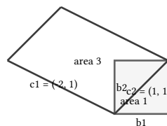
figure 58: the basis change matrix sends the unit square, area 1, to the column parallelogram, area 3 = |\det J|
