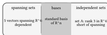
figure 29: spanning sets against independent sets, bases in the overlap
