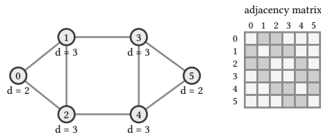
figure 87: G1 with its degrees and adjacency matrix, 36 cells holding 8 edges
