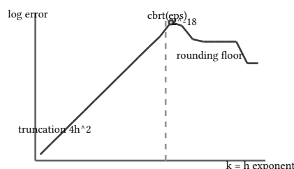
figure 55: central difference error against h , the U with its floor
