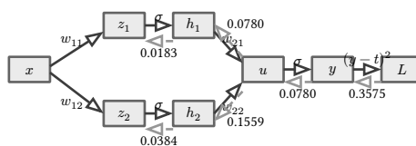
figure 71: forward pass solid, adjoint sweep dashed, every number measured in backprop.c at the pinned weights
