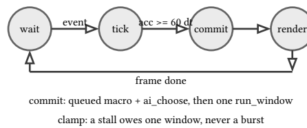
figure 190: the windowed loop as a state machine: timer ticks feed the accumulator, whole windows commit, every frame renders
