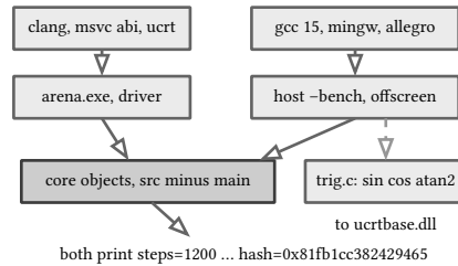
figure 184: two build lanes over one core: the clang-built driver and the gcc-built host, their bench hashes meeting at the pinned value through the ucrt routing
