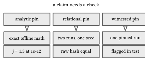
figure 182: the three pin tiers: analytic constants inside a stated epsilon, relational bit equality across runs, witnessed numbers pinned from the deterministic binary
