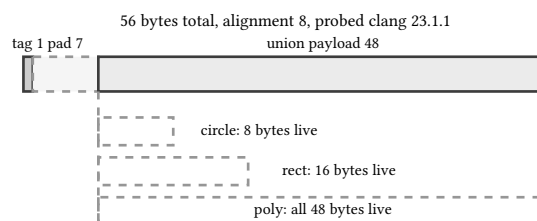
figure 156: struct shape, 56 bytes: one tag byte, 7 of padding, then the 48 byte union with the three payload footprints
