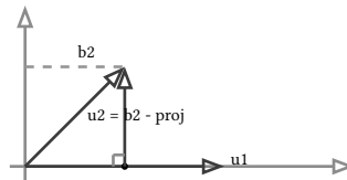
figure 47: gram-schmidt subtracts the projection, mml example 3.12 in two dimensions
