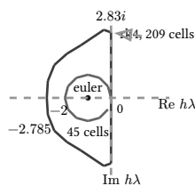
figure 135: the absolute stability regions on the h\lambda plane at equal scale, euler a disk of radius 1 inside the rk4 region reaching past minus 2.78
