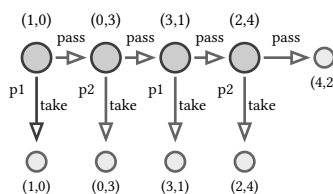
figure 150: the centipede, take drops out and pass chains right, rollback value above each node
