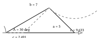
figure 18: the ambiguous case: a = 5 swings an arc through the base ray at two points, two triangles share A = 30 degrees and b = 7
