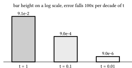
figure 60: linearization error at t = 1, 0.1, 0.01 on a log height scale, each decade of t cutting the error by 100
