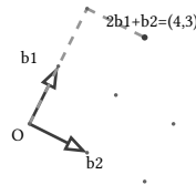
figure 26: linear combinations of b_1=(1,2) and b_2=(2,-1) as a lattice through the origin, 2b_1+b_2 marked
