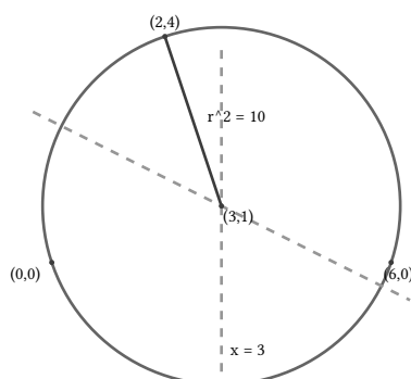
figure 23: circumcircle of (0,0), (6,0), (2,4): bisectors meet at (3,1), r^2 = 10
