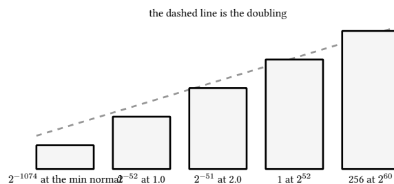
figure 2: one ulp doubles at every exponent step
