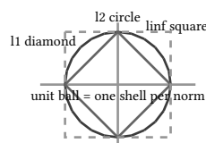
figure 30: unit balls of the three norms, diamond, circle, square
