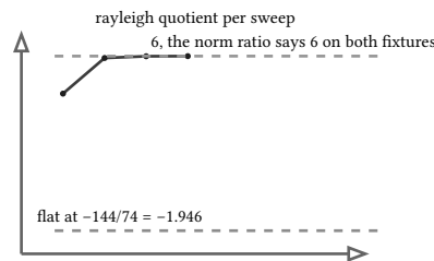
figure 140: the rayleigh quotient per sweep, one ladder climbing to 6, the equal-magnitude fixture flat at -1.946
