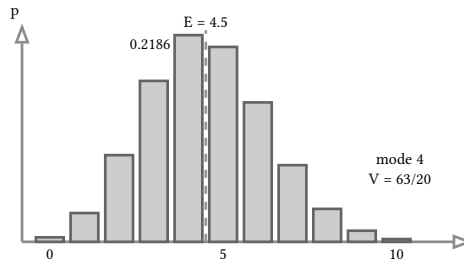
figure 110: binomial pmf bars for N = 15, mu = 0.3, mean line at 4.5
