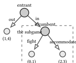
figure 151: entry deterrence, the dashed box is the incumbent subgame where the threat fails
