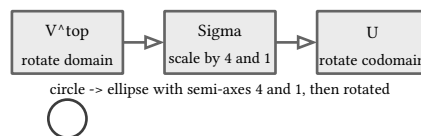
figure 48: svd as rotate, scale, rotate
