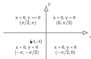
figure 15: the \text{atan2} return map: four quadrants, four ranges, both coordinates kept
