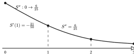
figure 129: the 4-knot fixture, one smooth curve from three cubics, second derivative continuous across the interior knots
