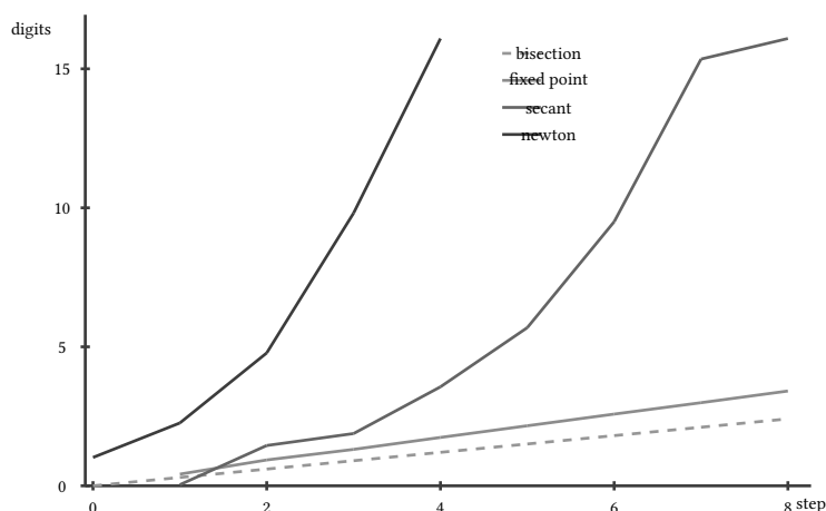
figure 123: digits of accuracy per iteration: bisection and fixed point crawl at fixed slopes, secant accelerates, newton doubles
