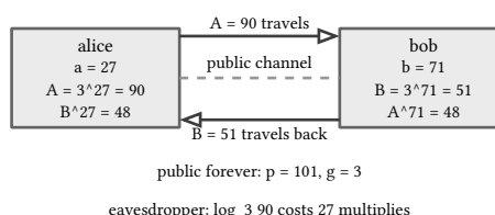
figure 106: the exchange: secrets 27 and 71 never cross the public line, the powers 90 and 51 do, and 48 emerges on both sides
