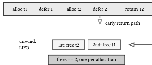
figure 159: scope timeline: defers register left to right and fire last first, on the early path too
