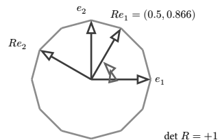
figure 43: rotation by \pi/3 , the basis stays orthonormal
