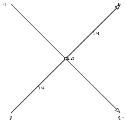
figure 22: the x crossing: two parametric segments meeting at t = u = 1/2
