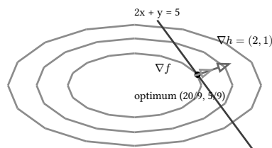
figure 65: the tangency: level ellipses of the objective against the constraint line, gradients aligned at the optimum
