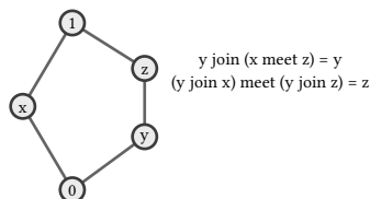
figure 91: the pentagon N5: every pair joins and meets, distributivity fails on the witness triple
