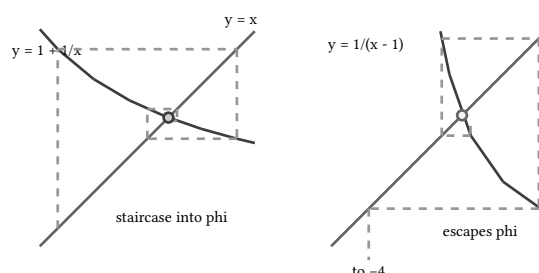
figure 120: two cobwebs for one equation: the convergent staircase into phi on the left, the repelling orbit that escapes on the right
