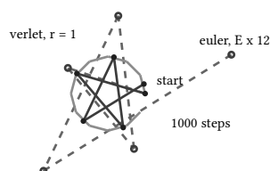
figure 136: the harmonic oscillator in phase space, euler spiraling out while verlet rides the circle
