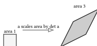
figure 44: unit square and its image, area scales by \det a = 3
