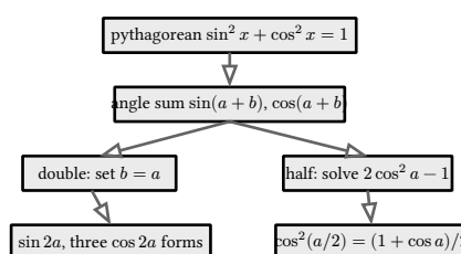
figure 14: the identity kit as one derivation: pythagorean at the base, angle sum above, double and half by substitution and solving
