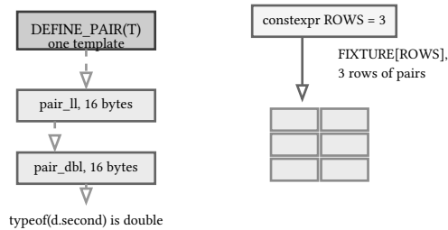
figure 158: one macro stamps every pair type, constexpr sizes the fixture, typeof picks the field type
