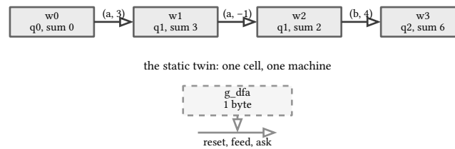
figure 175: the world threading above, the one byte static twin below
