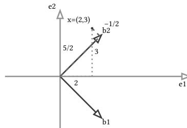
figure 31: the same vector read in two bases, standard coefficients 2 and 3, tilted coefficients -\frac{1}{2} and \frac{5}{2}
