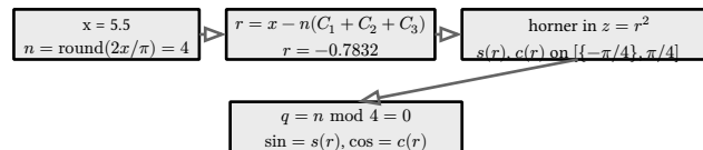
figure 16: the reduction pipeline for x = 5.5 : nearest multiple, three-piece subtraction, polynomial, quadrant dispatch
