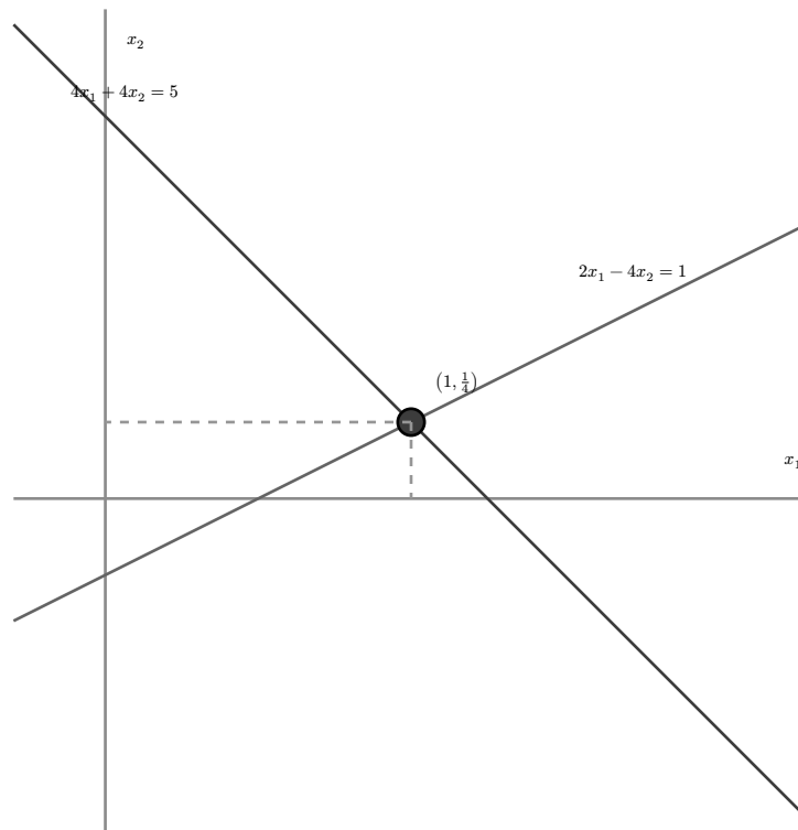
figure 32: two lines, one crossing point at (1, 1/4) , the row picture of the fixed system
