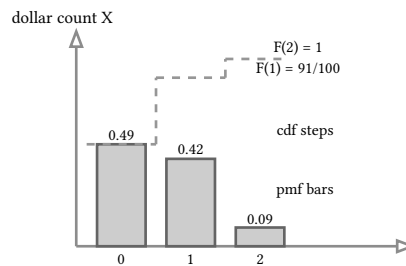
figure 109: two-coin pmf bars with cdf steps, heights exact
