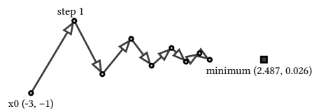
figure 63: the 0.085 zigzag across the valley toward (2.487, 0.026)
