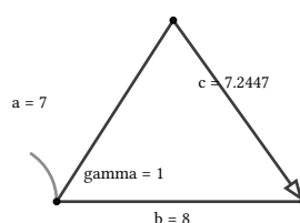
figure 17: the 7-8-1 triangle to scale: \gamma = 1 rad between a = 7 and b = 8 , c = 7.2447 opposite
