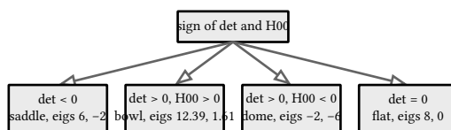
figure 59: definiteness of a 2x2 hessian read off det and the diagonal, each verdict confirmed by eigenvalues
