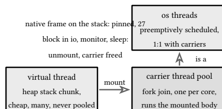
figure 16: a virtual thread mounts on a carrier, blocks, unmounts, remounts
