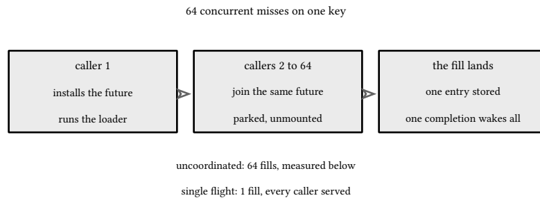
figure 51: the stampede collapsed: one fill, everyone else parked on its future
