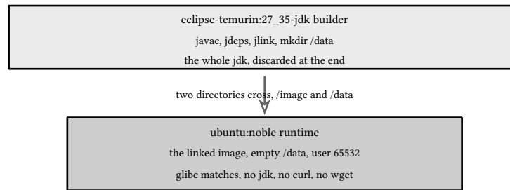
figure 57: two stages, two directories cross: the builder dies with the build, noble runs them
