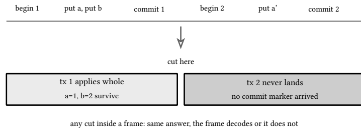
figure 47: a log recovers to the last committed group, whatever the cut
