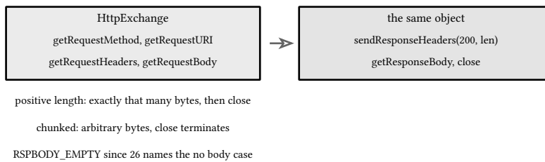
figure 23: one object is the whole transaction: request in, response out, close at the end
