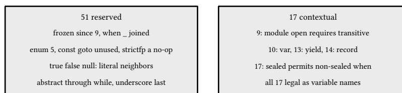
figure 5: the keyword taxonomy: 51 reserved and frozen, 17 contextual and dated
