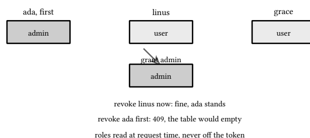
figure 43: the grant table: one column per user, the admin row must never empty
