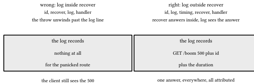
figure 32: wrong order versus right: where the log sits decides what it sees
