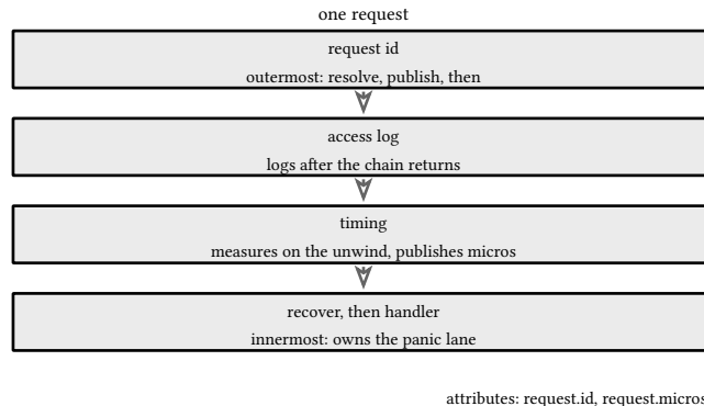
figure 29: the chain is a list iterator: list order is runtime order, code after the call runs on the unwind
