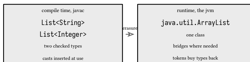
figure 10: what javac sees, what the jvm sees
