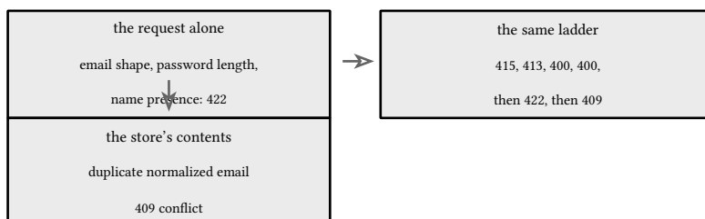
figure 34: same request shape, two truths: rules about the request, conflict about the store
