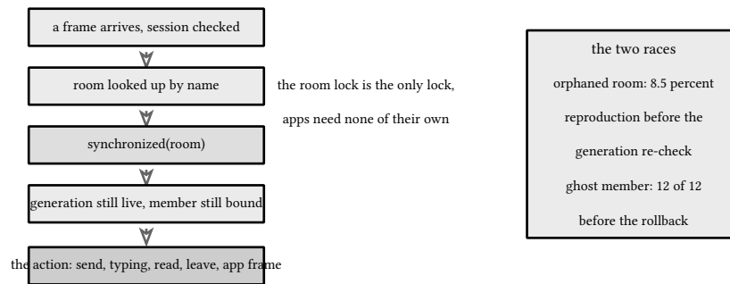
figure 63: the hub's one guarded path, everything re-checked under the room lock
