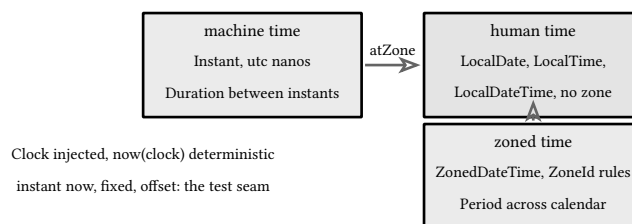
figure 19: the type lattice: machine time left, calendar right, zones bridged
