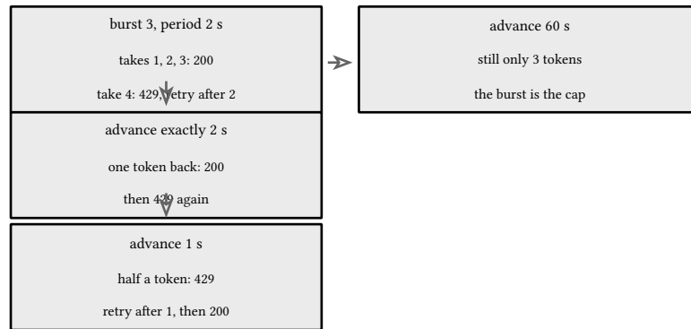
figure 52: the bucket's answers, every boundary exact under a frozen clock
