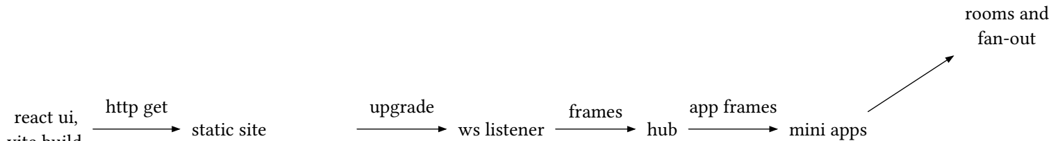
figure 61: the capstone, one process, one port, two protocols
