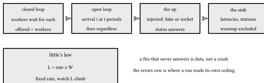
figure 55: workers, pacer, server, sink: one harness, two loops
