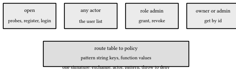
figure 41: four policies, one signature, the table maps routes onto them
