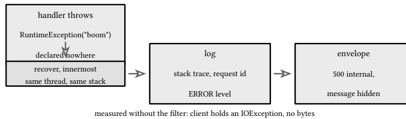
figure 30: panic unwind: one path to the log, one to the envelope
