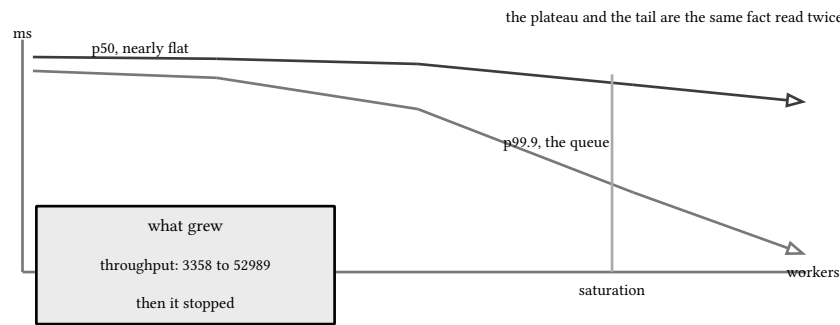
figure 56: the ladder's p50 and p99.9 against offered load, the tail is the story
