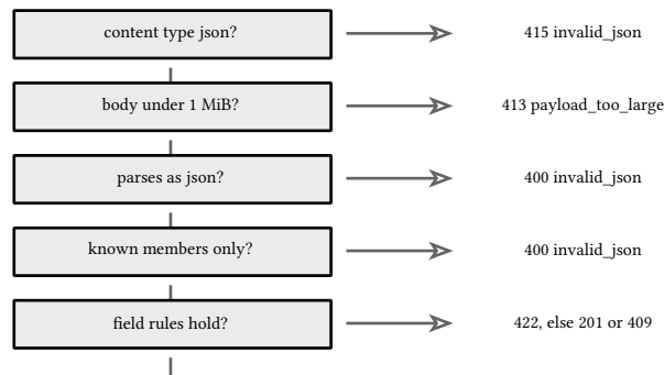
figure 26: the decode ladder: each rung rejects a class of bad input before the next runs
