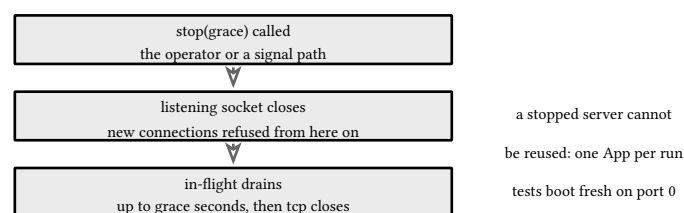
figure 27: the stop order: listener first, drain second, connections last
