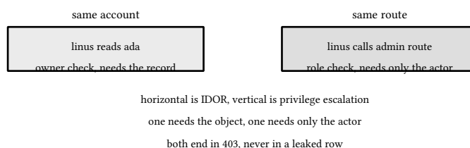
figure 42: horizontal versus vertical: two axes of privilege, two different checks
