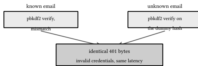
figure 38: the timing-equalized login: unknown email pays what a wrong password pays
