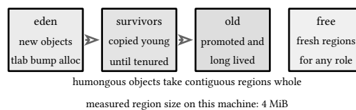
figure 17: the G1 heap: regions classified by role, evacuation moves survivors between them
