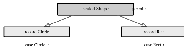
figure 15: the tree the switch is checked against
