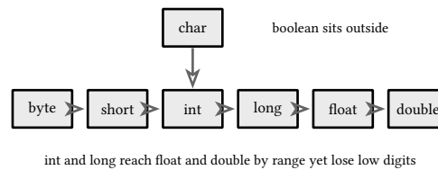
figure 6: the conversion lattice: arrows widen implicitly, everything else casts
