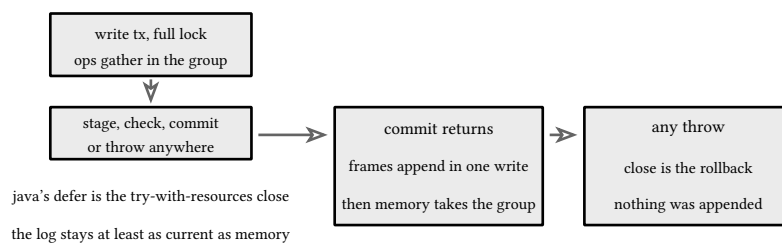
figure 48: a transaction's exits, every one of them clean
