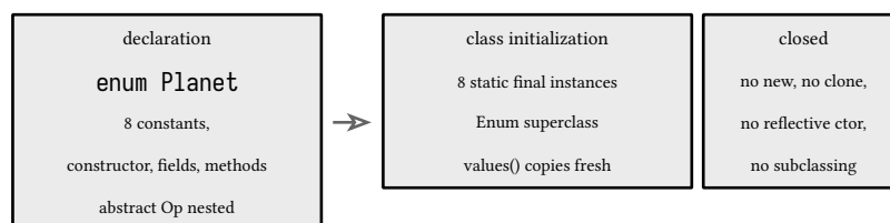
figure 12: one enum declaration, what the runtime holds
