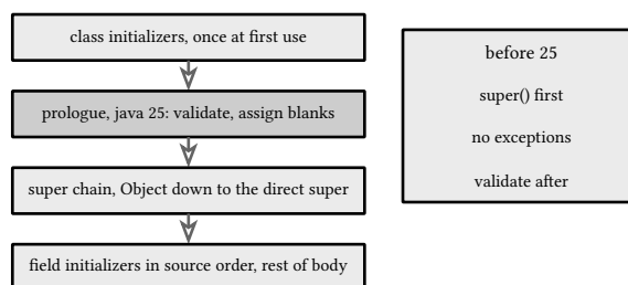
figure 8: one construction, top to bottom
