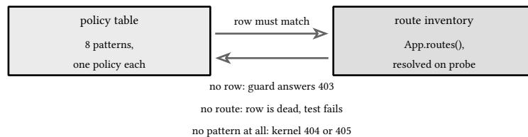
figure 44: the audit: table and route inventory face each other, both directions checked
