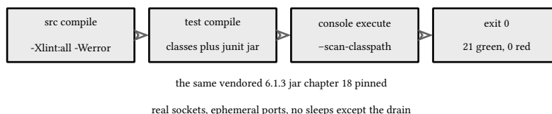
figure 28: the test lane: two compiles, one console run, exit 0 green
