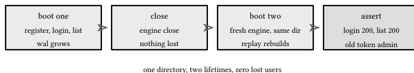
figure 49: the reboot proof: two processes, one directory, everything comes back
