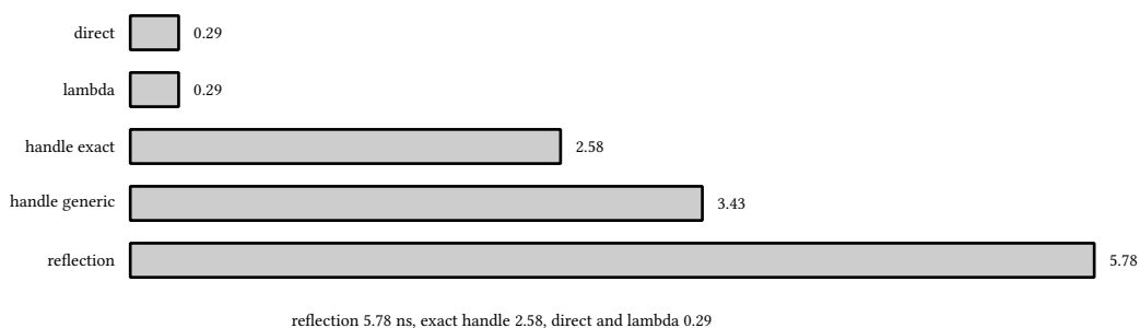
figure 21: call mechanisms by measured cost, nanoseconds per call, lower is better
