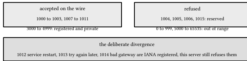
figure 62: the close code table this server enforces
