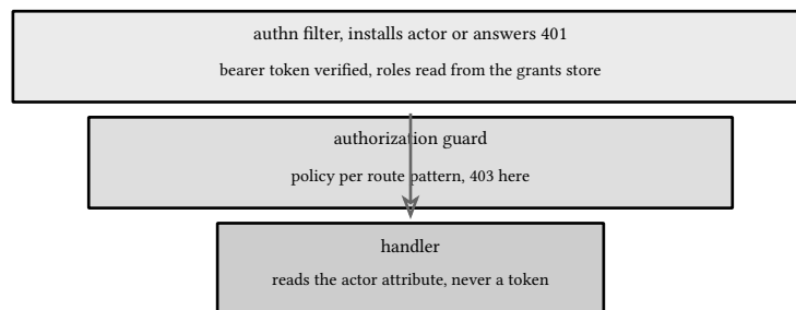
figure 40: two layers in wiring order: authn outside, guard inside, handler last
