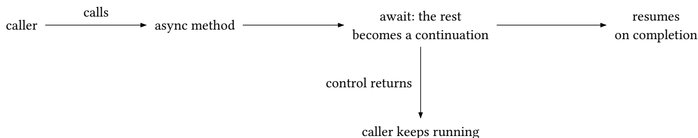
figure 57: await as suspension, one method lowered to a state machine
