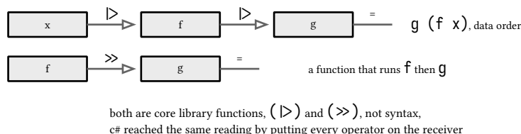
figure 124: pipe and compose, library functions that read in data order
