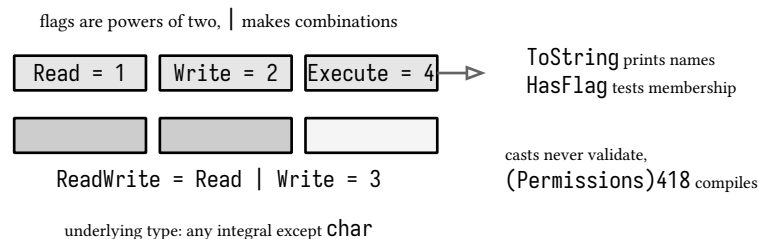
figure 21: enum bits, powers of two combine, names print, casts unchecked
