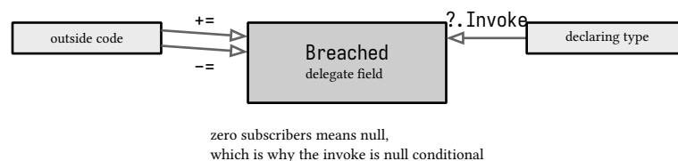
figure 28: an event, one delegate field behind permission walls
