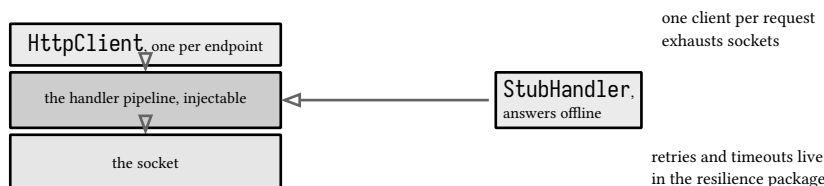
figure 104: the handler chain is the http test seam
