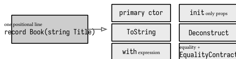
figure 18: one record declaration, the six members the compiler synthesizes
