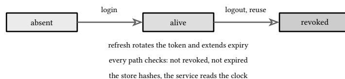
figure 159: the session lifecycle: login creates, refresh extends, logout or reuse revokes
