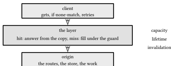
figure 186: the layer sits between client and origin, answering what it can
