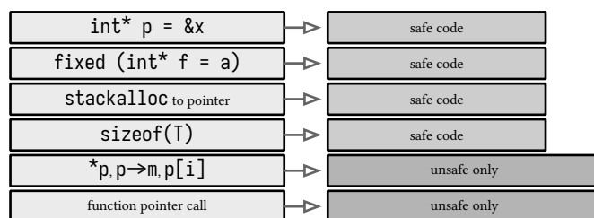
figure 69: the boundary moved, pointer existence is safe, access is not
