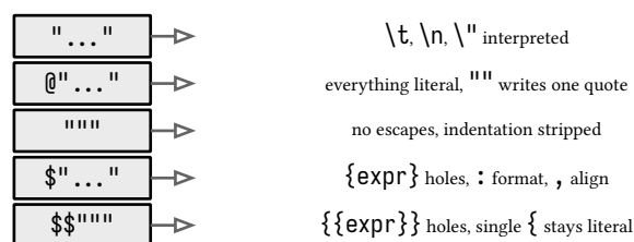
figure 11: the five string forms and their escape policies
