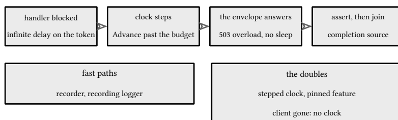
figure 149: the harness: gates hold handlers, clocks step, channels join
