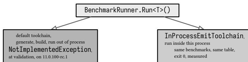
figure 80: two toolchains, one dead on the rc sdk, one working
