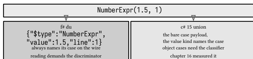
figure 132: one case, two wires, the envelope is the difference
