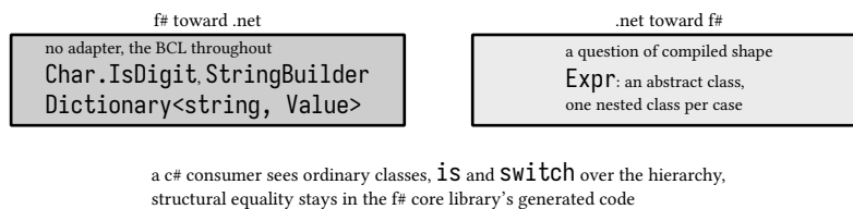
figure 131: interop both directions, plain bcl calls out, ordinary classes in
