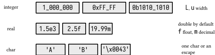
figure 10: literal inventory, bases, separators, suffixes, escapes
