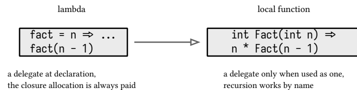
figure 51: lambda vs local function, when the delegate is created
