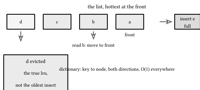
figure 188: a read moves its node to the front, an insert evicts the back
