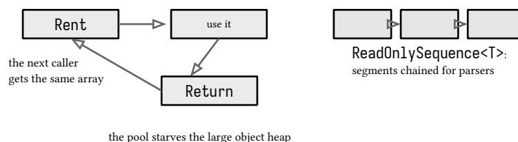
figure 97: arraypool cycles arrays, the sequence chains segments
