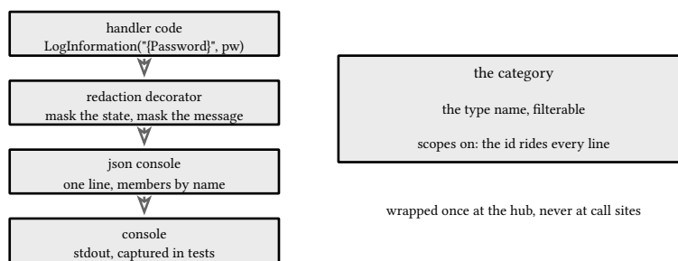
figure 200: the logger's own stack: call site through provider to console
