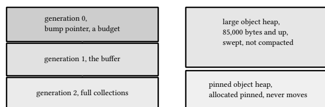
figure 71: the managed heap: three generations with budgets, two special heaps beside them
