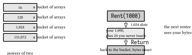
figure 75: the bucket ladder: rent rounds up, return is voluntary, nothing clears
