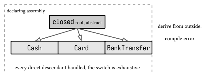
figure 20: closed, the descendant set is fixed inside the assembly
