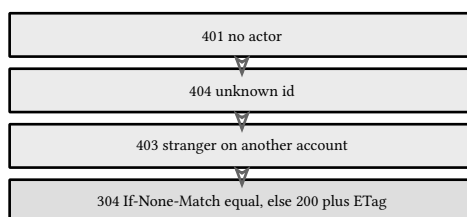
figure 155: one request climbs the ladder, each rung one contract code
