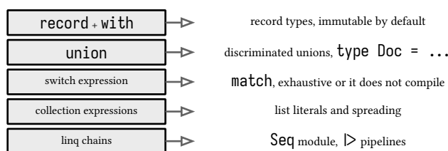
figure 116: each c# piece, its f# ancestry
