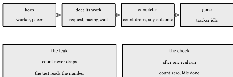
figure 213: a task lifecycle: born, joined, or leaked
