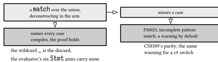
figure 122: match deconstructing as it branches, the incomplete case warned
