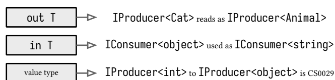
figure 32: variance legality, out and in convert, value types freeze
