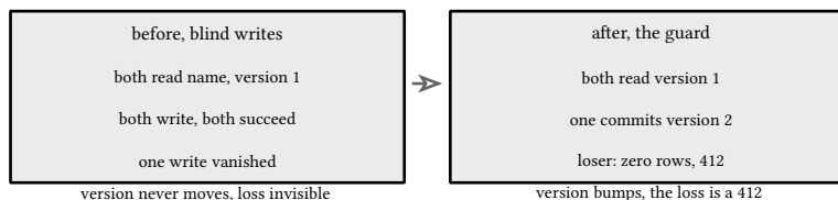
listing 240: the guarded update: check, bump, and write in one statement, zero rows is the refusal (source: csharp-net/api/src/CsharpBook.Api/Store/SqliteUserStore.cs , lines 83-100)
