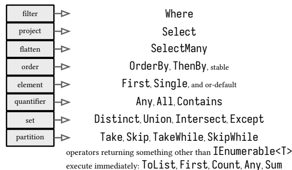
figure 90: the operator families, one job each
