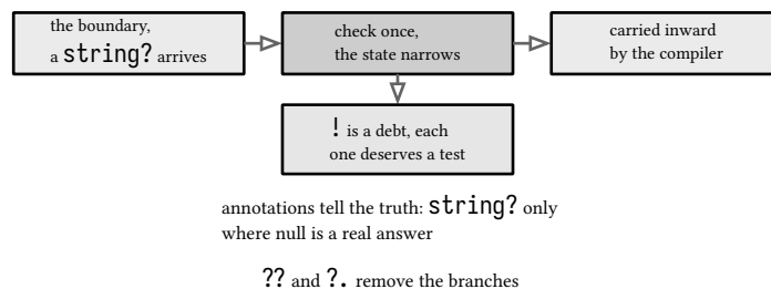
figure 110: nullable discipline, check once at the boundary
