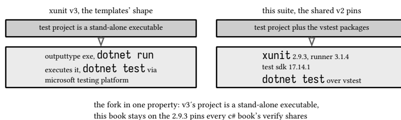
figure 4: the v2/v3 fork in one property, a v3 suite executes itself while this book stays on the shared v2 pins
