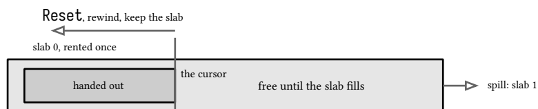
listing 107: bump allocation with a rewind: rent, exhaust, reset (source: csharp-net/samples/src/Ch11/Arena.cs, lines 33-73)
