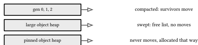
figure 73: three heaps, three movement policies
