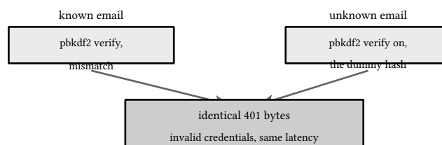
figure 158: the timing-equalized login: unknown email pays what a wrong password pays
