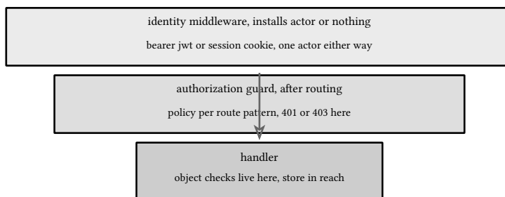
figure 165: two layers in wiring order: identity outside, guard inside, handler last
