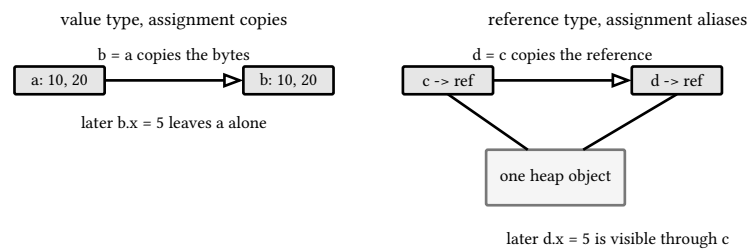
figure 15: what assignment does in each category
