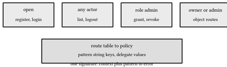
figure 167: four policies, one signature, the table maps routes onto them
