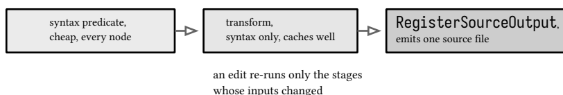
listing 124: the initialize pipeline: filter syntax, emit source (source: csharp-net/samples/src/CsharpBook.Generators/SummaryGenerator.cs, lines 9-40)
