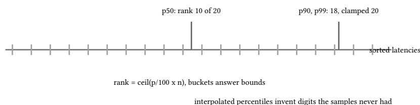
figure 204: the tail ladder: where p50, p90, p99 sit in one sorted sample
