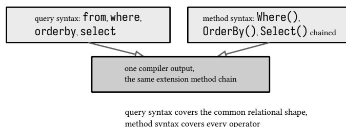
figure 88: two spellings, one compiler output
