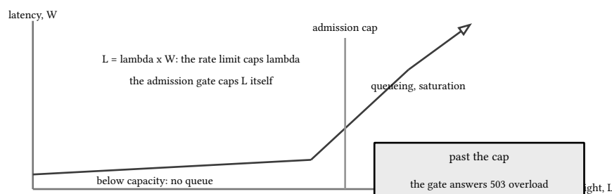
figure 199: latency versus concurrency: the hockey stick the admission cap cuts off
