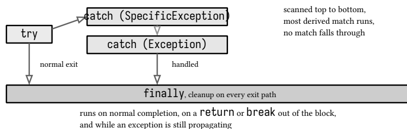
figure 53: try catch finally, the scan and the guaranteed bar
