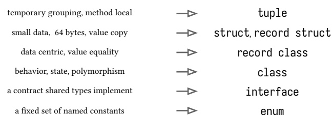
figure 16: the kind of type ladder, lightest to heaviest
