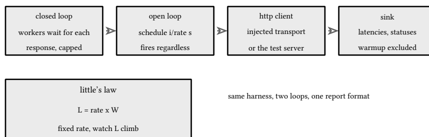
figure 207: workers, host, latency sink: one harness, two loops
