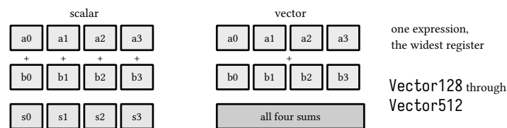
figure 98: simd lanes, one wide add against four narrow ones
