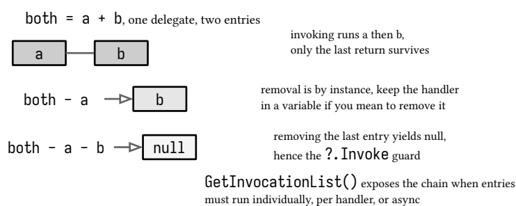
figure 48: the multicast chain, combine, invoke in order, remove by instance
