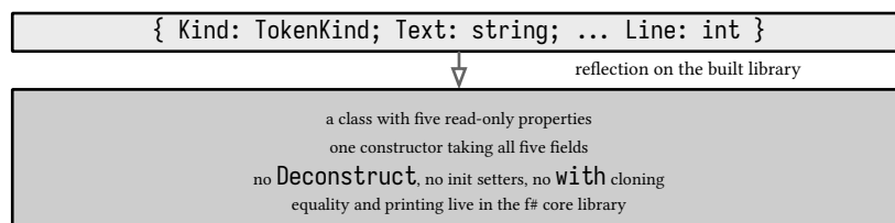
figure 120: one brace declaration, the compiled shape reflection measures
