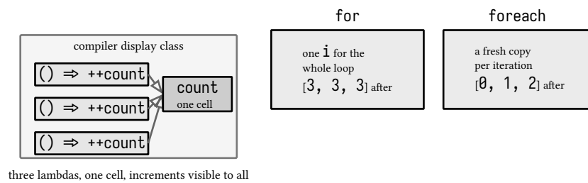
figure 47: closures, one hoisted cell shared, the loop capture trap
