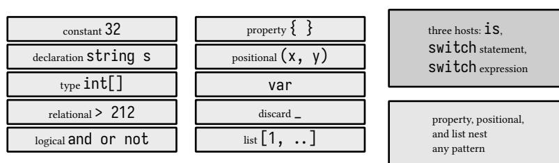
figure 34: the pattern inventory, ten kinds, three hosts, the recursive three
