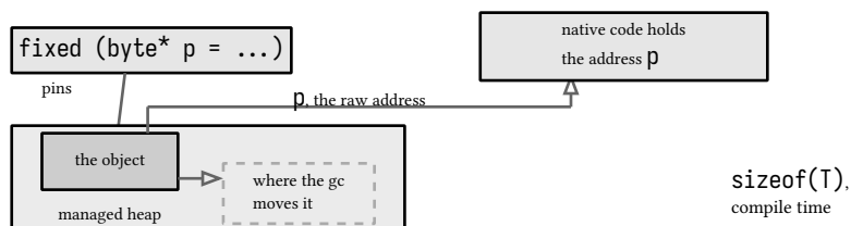
figure 68: fixed pins the object while native code holds its address
