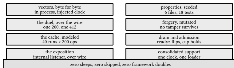
figure 228: the suite as one ledger: every row a test file family observes
