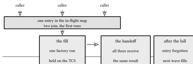
figure 183: three requests arrive together, one origin read happens
