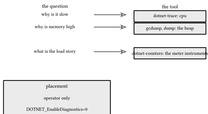
figure 205: which tool answers which question, all over one ipc channel
