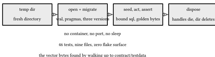
figure 179: a store test's lifecycle, nothing shared between runs
