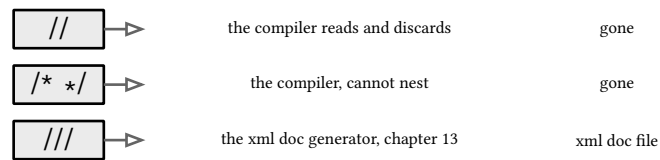
figure 14: three comment forms, their consumers, and what survives
