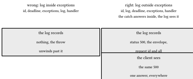
figure 148: wrong order versus right: where the log sits decides what it sees
