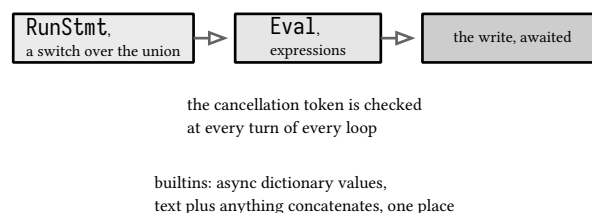
figure 235: the evaluator, a statement walk with awaits inside
