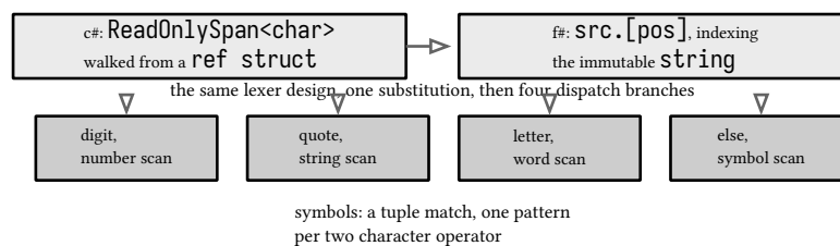
figure 126: the lexer, index arithmetic over the immutable string
