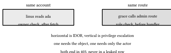
figure 169: horizontal versus vertical: two axes of privilege, two different checks
