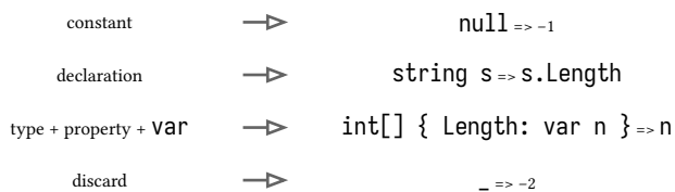
figure 40: one switch expression, four pattern kinds composed
