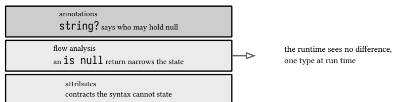
figure 23: nullable reference types, three compile time layers over one runtime type
