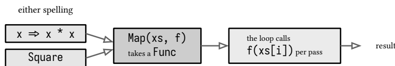
figure 49: behavior as data, one map over any transformation
