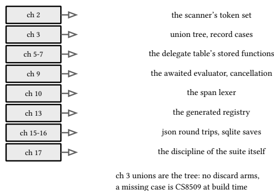
figure 238: every chapter cashed in one interpreter
