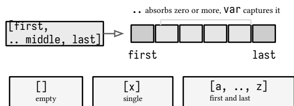
figure 39: list patterns, element wise with a slice in the middle
