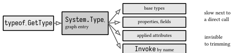
figure 85: system.type, the entry point to the metadata graph
