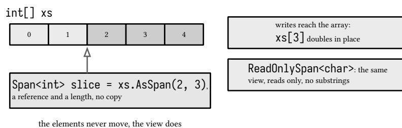
figure 64: a span is a reference and a length into storage, no copy
