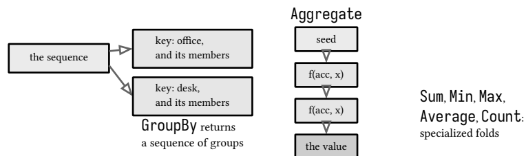
figure 91: groupby clusters by key, aggregate folds to a value
