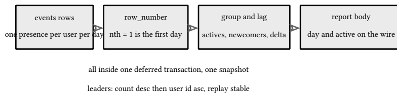
figure 178: events rows to windows to the report body
