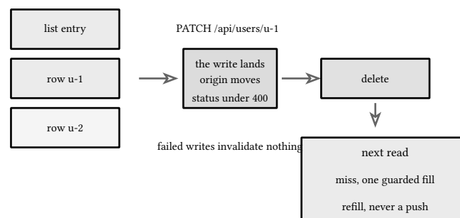
figure 191: write to a row: the row and the list go, the refill is the only writer
