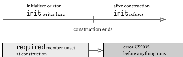
figure 26: the construction timeline, init's window and required's gate
