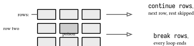
figure 43: labeled exits, break rows leaves, continue rows advances
