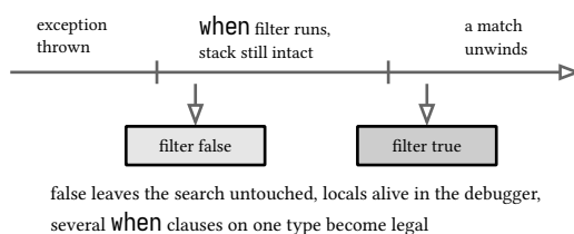
figure 54: the when filter, evaluated before the stack unwinds
