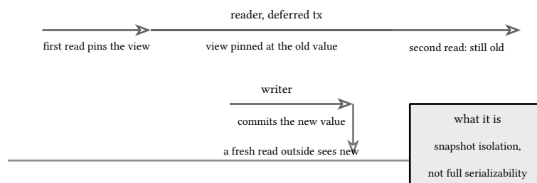
figure 176: one timeline: the reader's view holds
