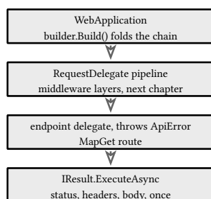
figure 136: the request climbs the pipeline, the result executes into the response
