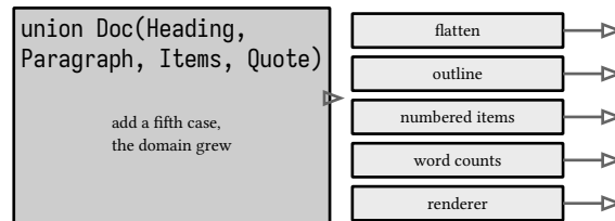
figure 114: a new case turns every transform red until handled
