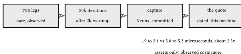
figure 209: the bench flow: leg, capture, quote
