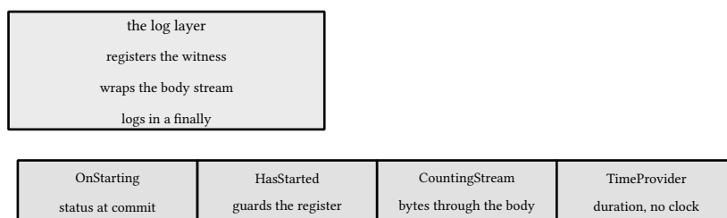
figure 146: status read at commit through OnStarting, bytes counted at the body
