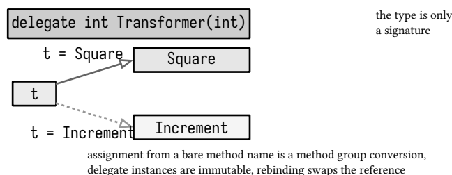
figure 45: a delegate type, a bound method group, and a rebinding
