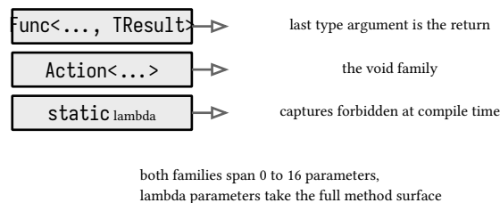
figure 46: the two delegate families and the lambda surface
