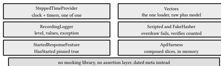
figure 225: the double set: one of each kind, strict by construction
