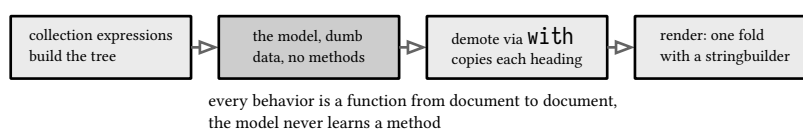
figure 113: data over behavior, transforms walk a model that stays dumb
