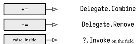
figure 50: event operations, the two outside verbs and the guarded raise
