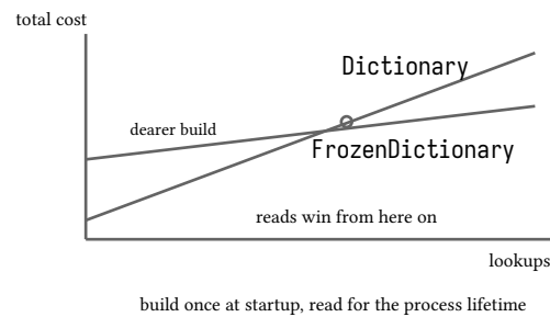
figure 96: frozen collections, pay at freeze, read cheaper forever
