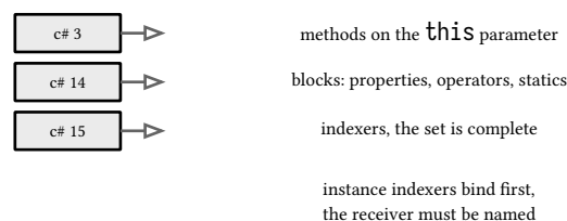
figure 30: extension indexers, the last member kind joins the block
