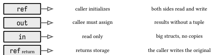
listing 94: in takes the big struct without copying it (source: csharp-net/samples/src/Ch10/Memory.cs, lines 48-49)
