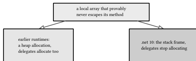
figure 70: escape analysis, provably local allocations move to the frame
