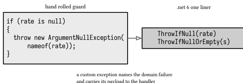
figure 52: the guard clause, four lines to one
