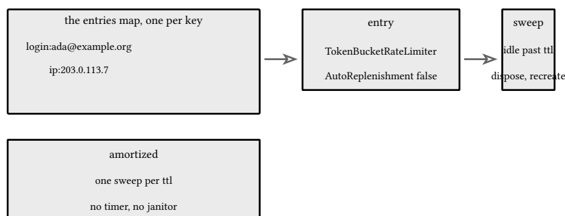
figure 195: key to bucket map, first use creates, idle age retires
