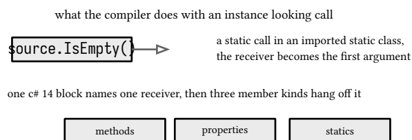
figure 29: extension members, an instance call rewritten to a static one
