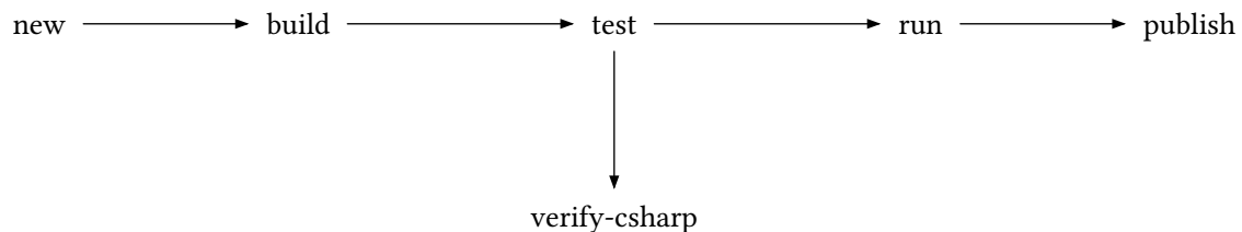
figure 3: the dev loop as a pipeline, test the gate every listing depends on
