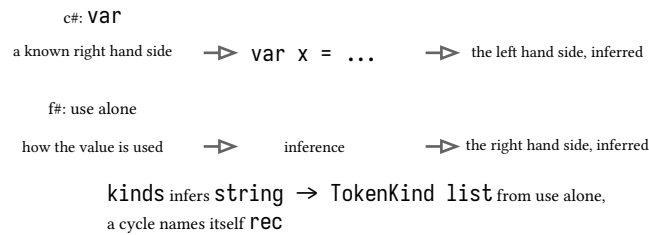
figure 119: the two inference directions, var from a known right, f# from use
