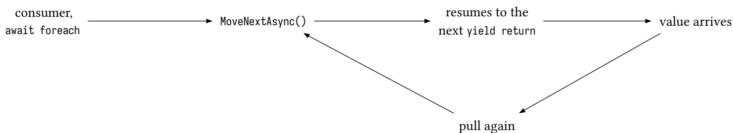
figure 61: async streams, one value per movenextasync, pulled by the consumer
