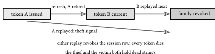
figure 163: the refresh family: rotation forks, reuse revokes everything
