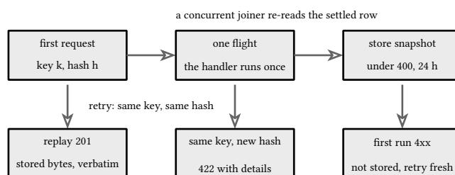
figure 182: one key's life: first run, snapshot, replay
