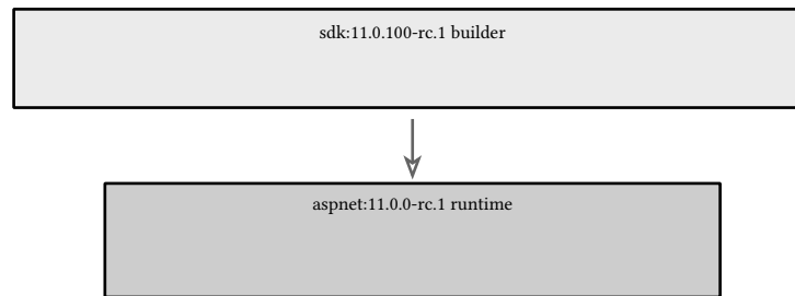
figure 214: two stages, one boundary: the builder dies with the build, aspnet runs the app
