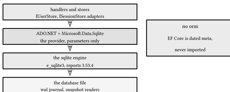
figure 172: the stack the store sits on
