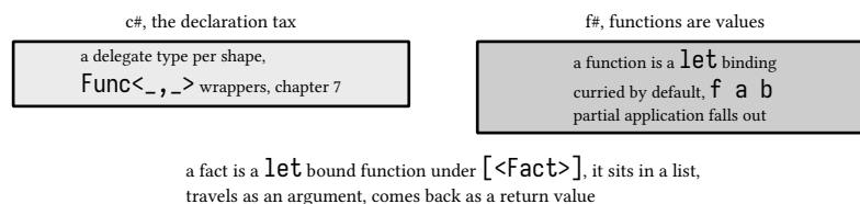
figure 118: functions as values, the delegate tax c# pays against the f# default
