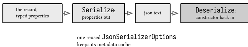
figure 100: the json round trip, properties out, constructor back in
