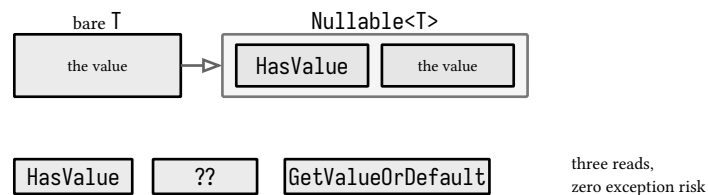
figure 22: nullable value types, a wrapper with a has flag beside the value
