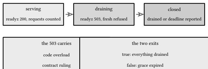
figure 211: the drain lifecycle: serving, draining, closed
