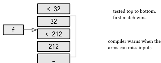
figure 35: switch expression arms, top to bottom, first match wins
