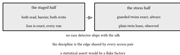
figure 185: the canary's two halves, one bug class
