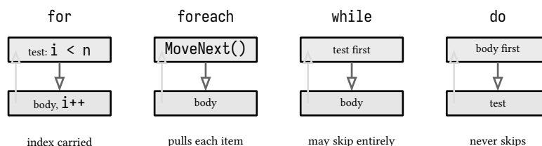
figure 42: four loop shapes, where the test sits in each
