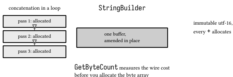
figure 103: string churn against one builder buffer
