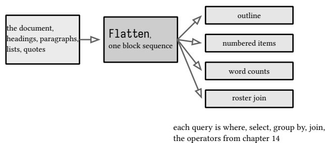
figure 115: the sample as pipelines, flatten once then query
