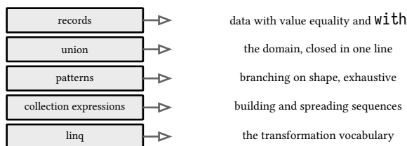
figure 112: five pieces, one job each, composed into one style
