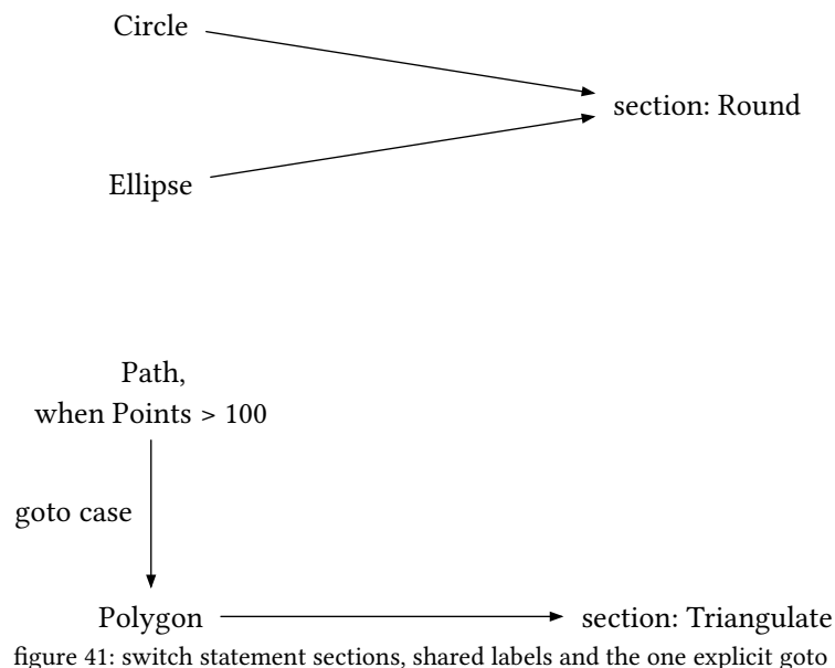
figure 41: switch statement sections, shared labels and the one explicit goto
