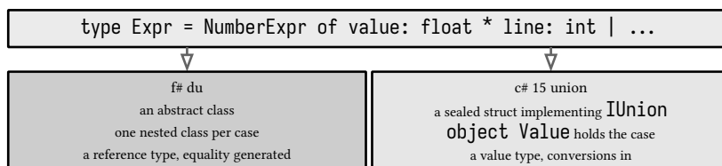
figure 121: same idea, two runtimes, the union in c# and the du in f#
