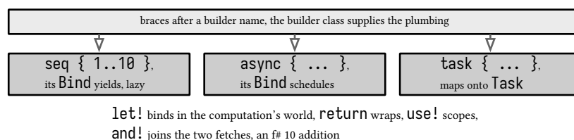
figure 128: computation expressions, one pattern behind seq , async , and task
