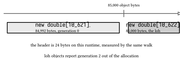
figure 72: the threshold, measured: 24 header bytes plus 8 per element crosses at 10,622
