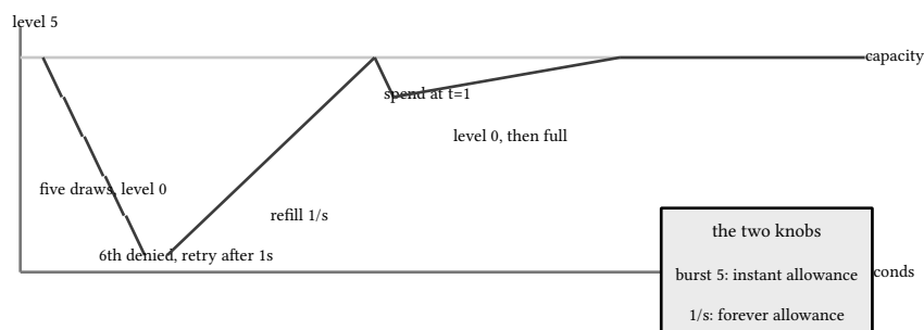
figure 194: bucket level over one draw timeline, the refill climbing between bursts
