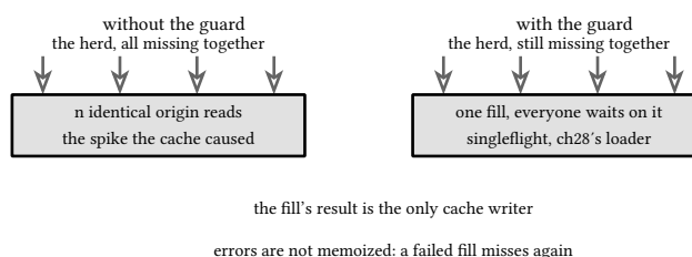
figure 190: the same expiry, with and without the guard
