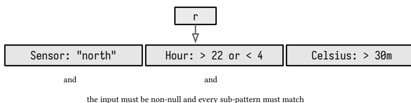
listing 54: an extended property pattern with a logical or inside (source: csharp-net/samples/src/Ch06/Flow.cs, lines 26-28)
