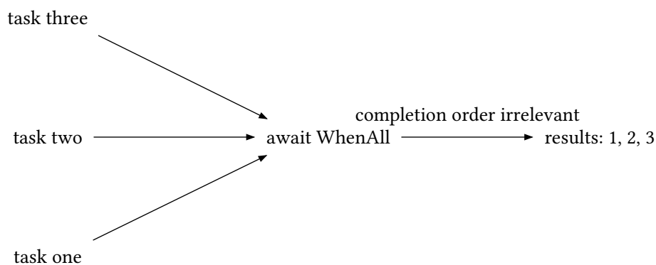
figure 58: WhenAll fans in, one await point, results in input order
