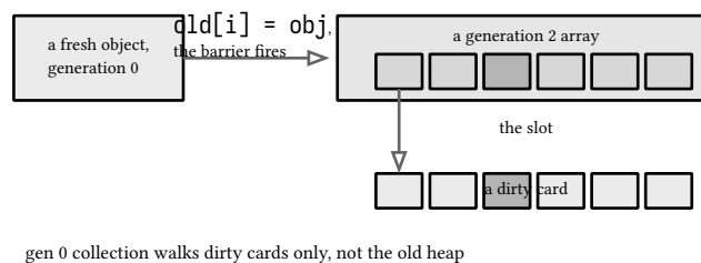
figure 74: the card table: a store into an old object dirties the card that names it
