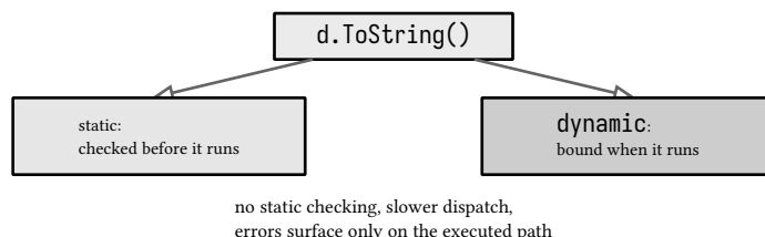
figure 86: dynamic defers binding from compile time to run time
