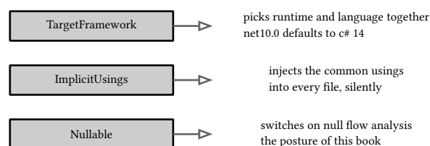
figure 2: three csproj properties, what each one controls
