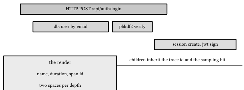
figure 202: one login request's spans over time, the tree the collector prints
