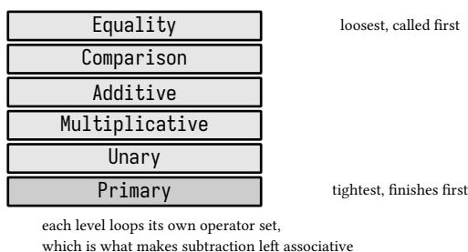
figure 233: precedence as call depth, tighter operators deeper
