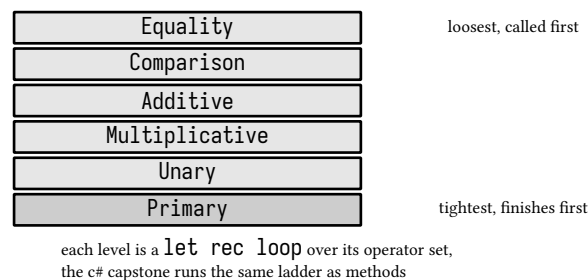
figure 127: precedence as call depth, one recursive loop per level
