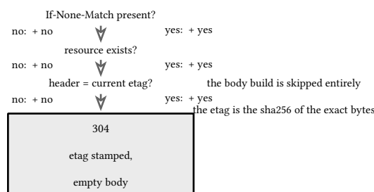
figure 181: the conditional GET decision
