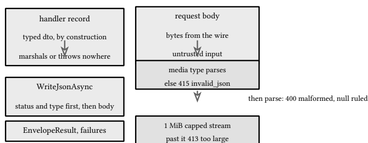
figure 139: two write sites, one decode ladder, four contract statuses
