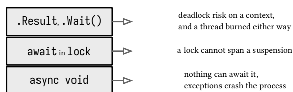
figure 62: the banned list, each rule with its cause
