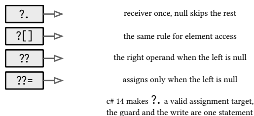
figure 44: the null operators, what each short circuits
