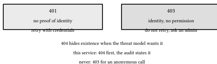
figure 168: the two failure codes, and the one deliberate blur
