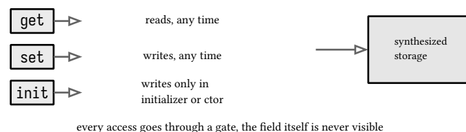
figure 24: a property, one storage behind three accessor gates
