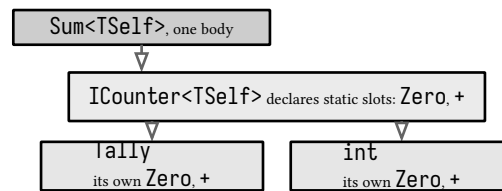
figure 33: generic math, one sum resolved through per-type static slots
