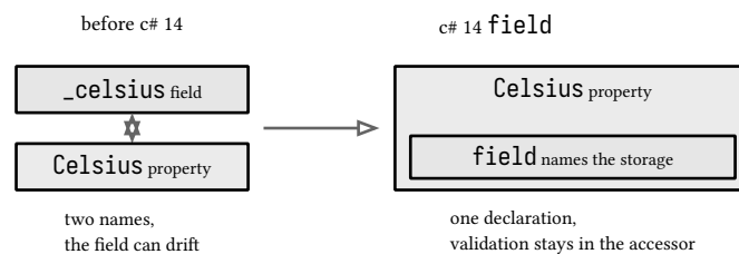
figure 25: backing fields before and after the c# 14 field keyword
