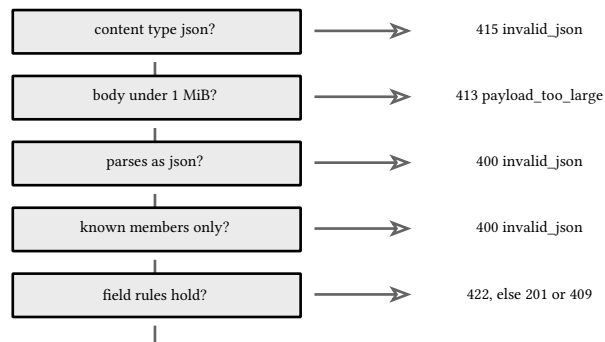
figure 151: the decode ladder: each rung rejects a class of bad input
