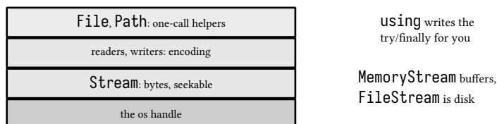
figure 102: the io stack, one call helpers over streams over handles
