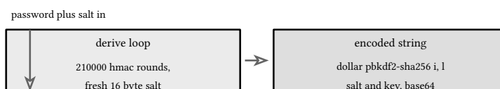
figure 157: pbkdf2: one hmac chain, parameters riding in the string
