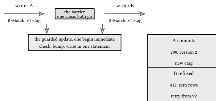
figure 180: two patchers, one barrier, one winner
