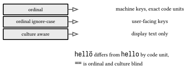
figure 109: the comparer grid, which rule for which job
