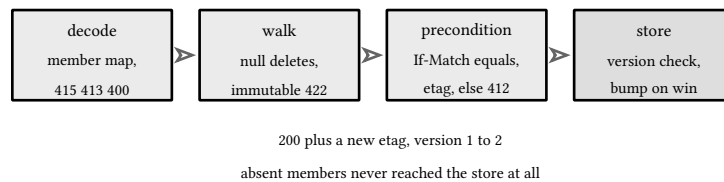
figure 153: a patch request walks the members, then the precondition, then the store
