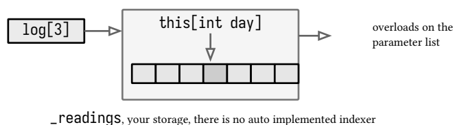
figure 27: an indexer, bracket syntax delegated to private storage
