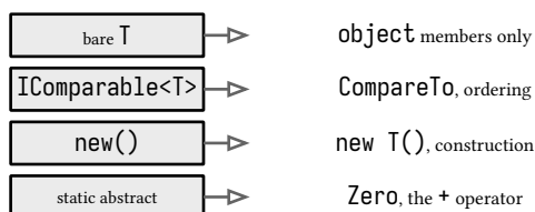
figure 31: each constraint purchases the operations it unlocks
