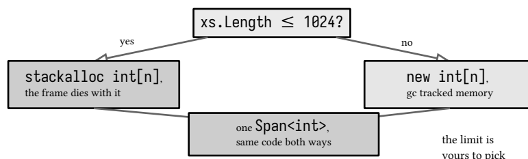
figure 65: stackalloc, stack under the limit, heap above, one span either way
