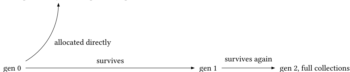
figure 63: the generational heap, survivors climb, big objects stay put
