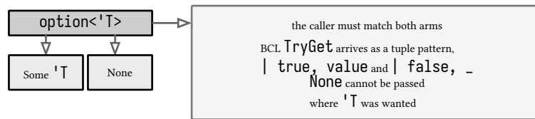
figure 123: option, absence as a value the type system counts
