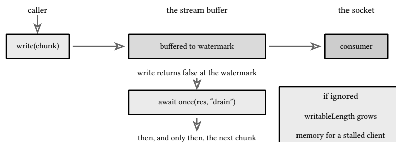
figure 201: the write path: offer, buffer, drain, offer again
