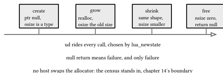
figure 42: one block's life through the hook
