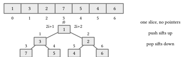
figure 13: one slice as a tree: children of i at 2i+1 and 2i+2
