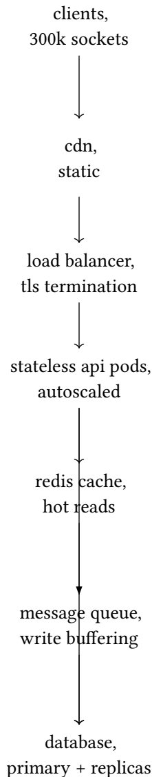
figure 90: 300k concurrent users, the shape that holds: stateless edges, shared cache, queue-absorbed writes, one replicated database
