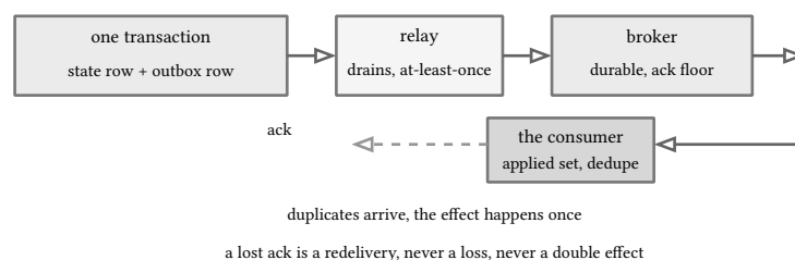
figure 117: at-least-once into an idempotent consumer, the outbox closing the dual write
