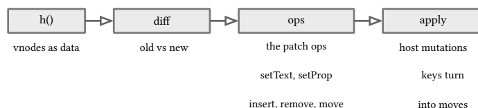
figure 60: h builds vnodes, diff emits ops, the host applies the change
