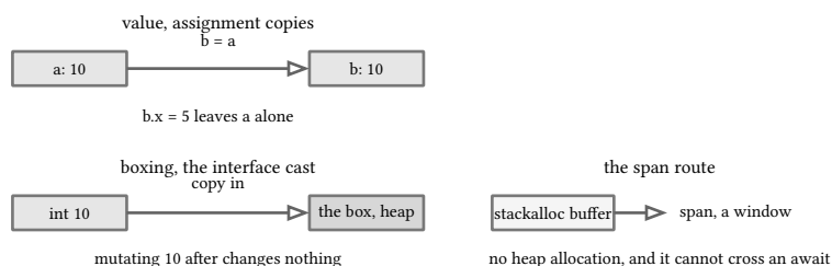
figure 145: assignment copies the value, an interface cast copies it into a heap box, spans stay off the heap
