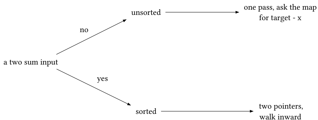
figure 23: sorted input walks two pointers inward, otherwise the complement map in one pass
