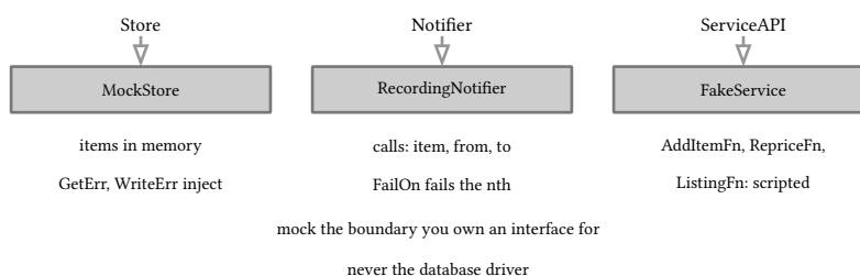
figure 70: three fakes behind the three interfaces the code already owns
