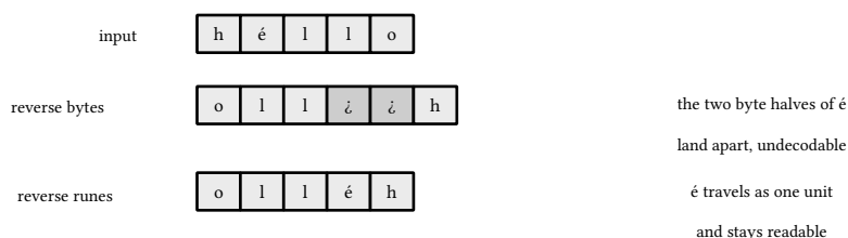
figure 19: runes are code points: the pair stays whole, the bytes do not
