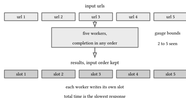
figure 93: indexed slots keep input order across any completion order
