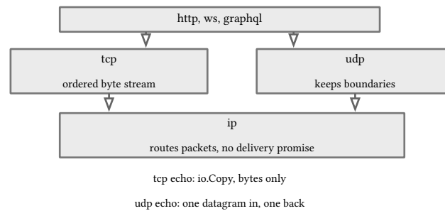
figure 81: ip routes, tcp streams, udp keeps boundaries
