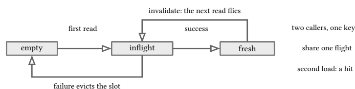
figure 56: the request cache state machine rtk query automates
