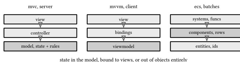
figure 8: one question at three altitudes: where state lives
