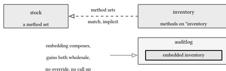
figure 5: structural satisfaction: the method sets match, the type never says so
