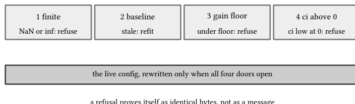
figure 129: four doors, every check before the write, any refusal leaves the bytes identical
