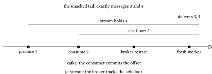
figure 102: kill the broker, restart: the floor survives, the tail is redelivered
