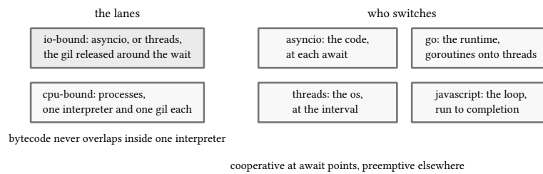
figure 139: io waits in either lane, cpu leaves the interpreter, and the models differ in who switches
