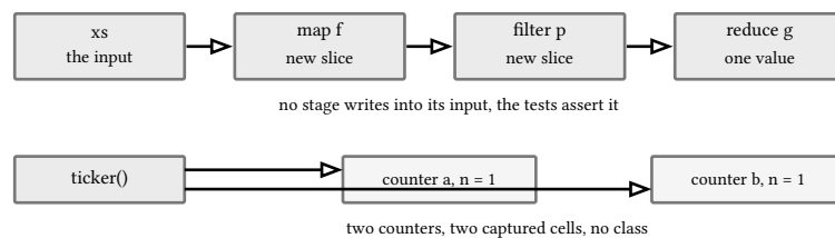
figure 7: pure stages never mutate, a closure is a function plus its own cell
