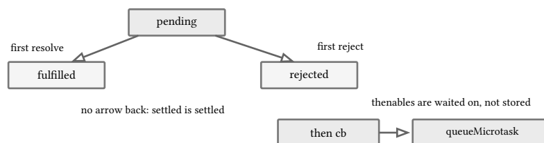
figure 41: settle once, callbacks always microtasked, thenables assimilated
