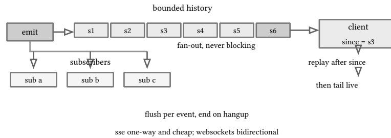
figure 98: bounded history plus subscribers: replay after since, then tail
