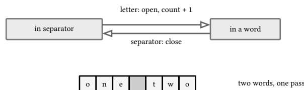
figure 38: a state machine over characters, no split and no regex
