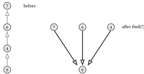
figure 110: find(7) walks three hops, then re-parents the whole path onto the root
