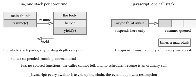
figure 141: lua parks whole stacks and owns no scheduler, javascript parks one frame and pays the queue
