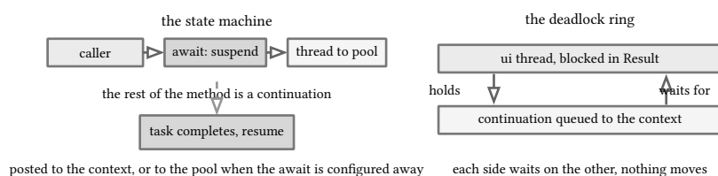
figure 143: suspension frees the thread, a blocked context waits on itself
