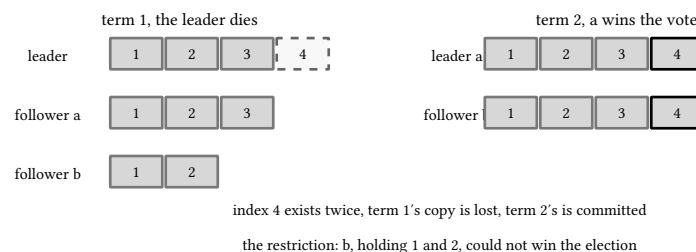
figure 115: one leader per term, the committed prefix survives the change, the tail does not
