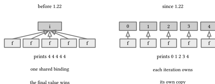
figure 65: one shared binding against per-iteration copies, the 1.22 fix
