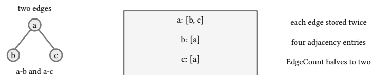
figure 15: undirected edges live in both adjacency lists
