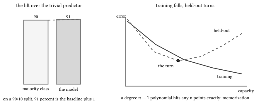
figure 126: the baseline owns the number, the gap opens where the fit memorizes
