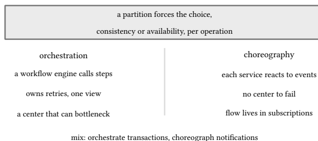
figure 89: cap picks per operation; center versus no center
