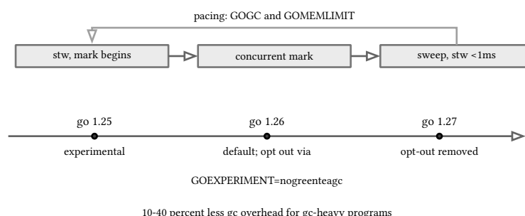
figure 63: tri-color mark and sweep, the green tea default timeline
