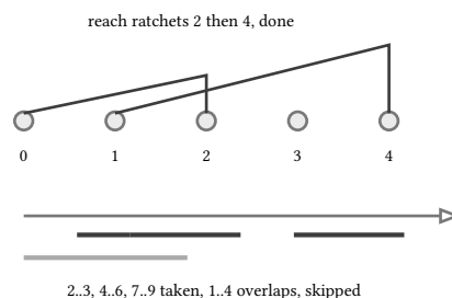
figure 105: reach ratchets up and never revisits, finish first takes three and skips one
