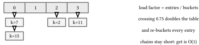
figure 11: chained buckets, doubling at load factor 0.75
