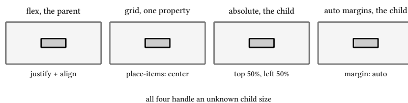
figure 35: four models: the parent flexes, the grid places, the child translates, the child absorbs
