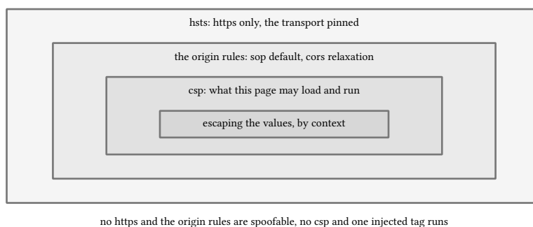
figure 157: the layers are concentric: each one assumes the layer outside it held
