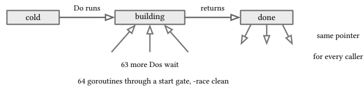
figure 68: once.Do: one build, every caller shares the result
