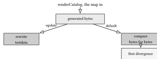
figure 72: two branches: compare by default, rewrite through the flag
