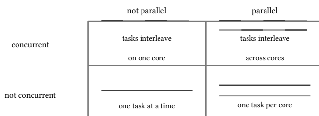
figure 61: parallelism is cores, concurrency is structure
