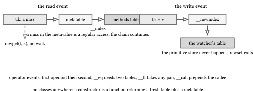
figure 140: the read miss walks the index chain, the write detours, the raw pair exits both
