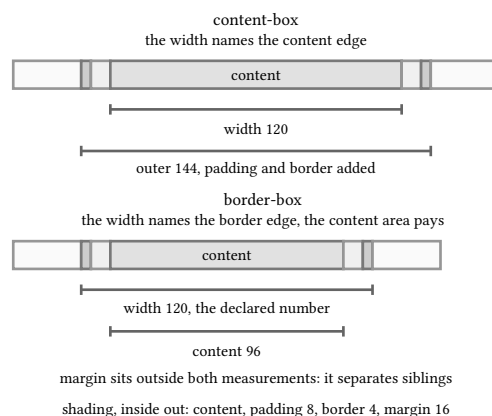
figure 147: one element measured both ways, the width property names a different edge
