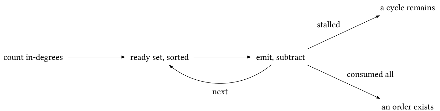
figure 18: in-degrees drain through the sorted ready set, a stall is the cycle
