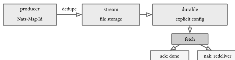
figure 101: stamp for dedupe, bind the durable, ack or nak
