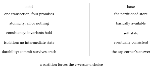
figure 74: acid's four promises against base's partition trade
