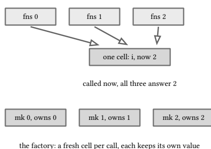
figure 138: three lambdas share the loop's one cell and all answer 2, the factory mints a cell per call
