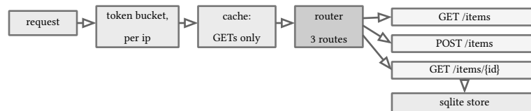
figure 94: limiter and cache in front, GETs only cached
