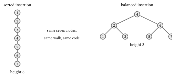
figure 12: same algorithm, two shapes: height 6 against height 2
