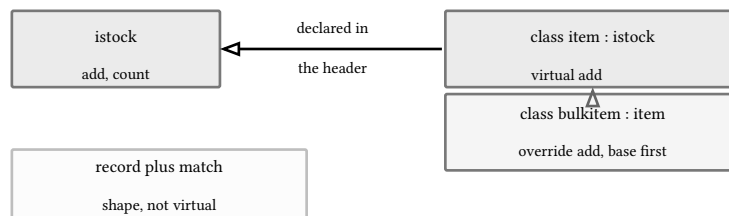
figure 6: nominal satisfaction: the header says it, the override calls base
