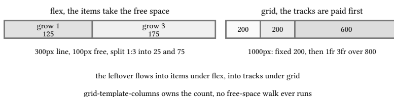
figure 149: flex distributes leftover space into items, grid distributes it into tracks first
