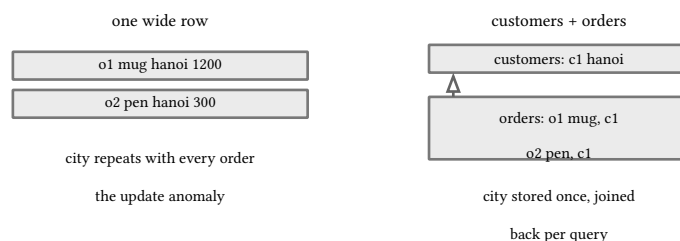
figure 76: the same facts as one wide row against customers plus orders
