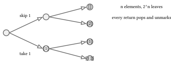
figure 106: two branches per element, the undo runs after each return
