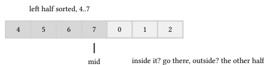
figure 104: mid splits the rotation, the sorted half answers, the other half inherits
