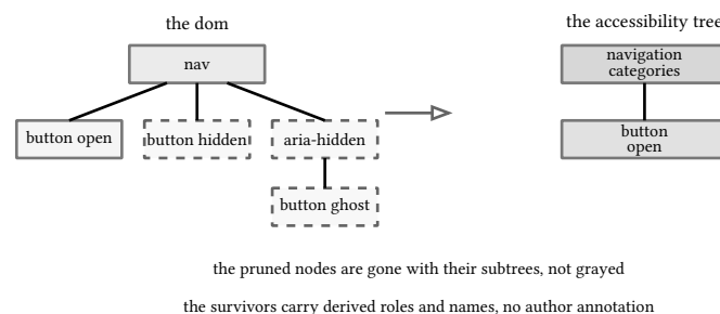
figure 153: the nav subtree before and after the reduction: hidden prunes, roles and names survive
