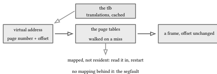
figure 119: a page number through the tables to a frame, the tlb skipping the walk
