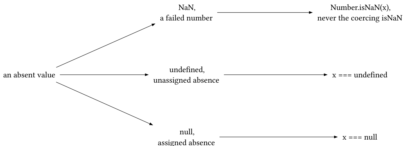
figure 31: three absences, three distinct tests, ?? touches only two of them
