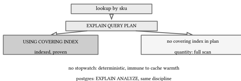
figure 77: the plan text is the proof, not the timing
