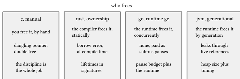
figure 185: four ways to answer who frees this memory
