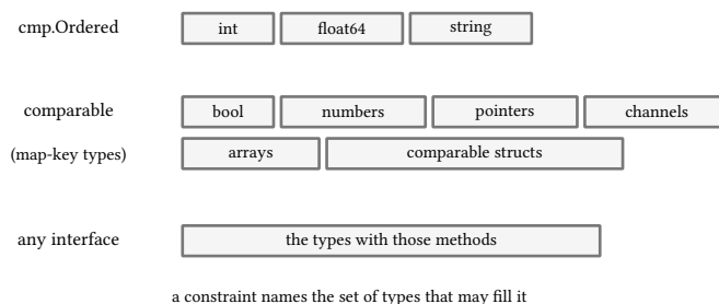
figure 66: constraints are type sets: ordered, comparable, methods
