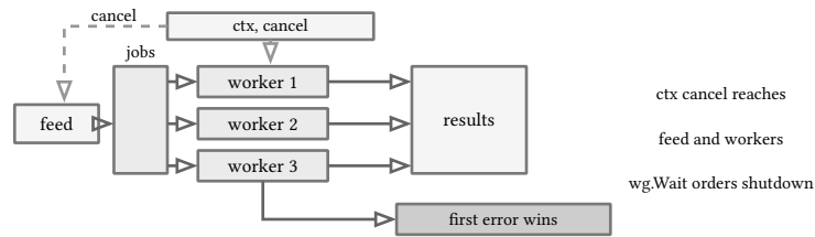
figure 64: the pool: fixed workers, first error cancels, wait orders shutdown
