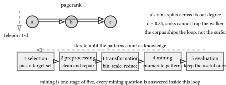
figure 135: the surfer with damping on top, the five-stage loop underneath, mining is stage 4
