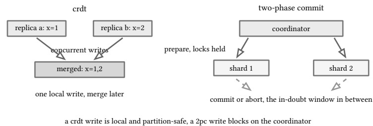
figure 116: merge converges with no coordinator, prepare and commit hold locks across round trips
