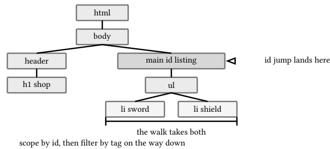
figure 34: the id jump scopes the search, then every li below it is a descendant hit
