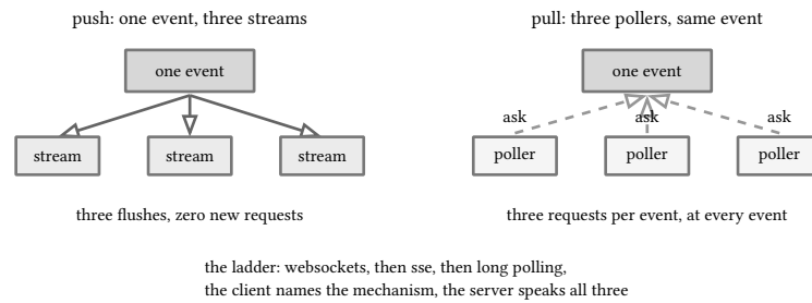
figure 167: push against pull: the same fanout through both delivery shapes
