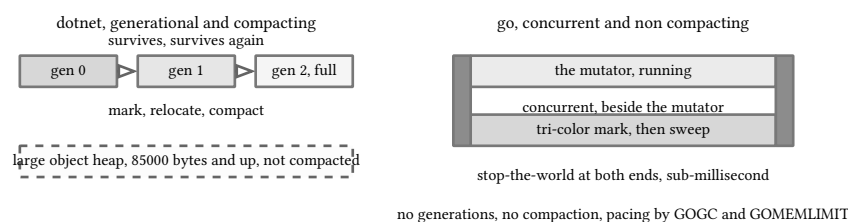
figure 146: dotnet compacts survivors up the generations, go sweeps concurrently and moves nothing
