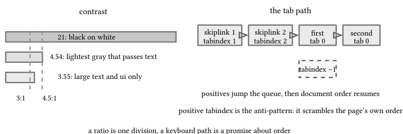
figure 154: the contrast ladder against its two thresholds, and the keyboard path the tab walk takes
