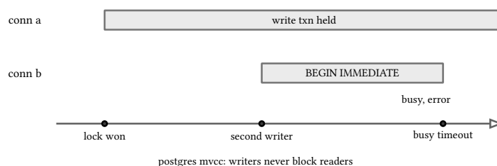
figure 78: the second writer waits out the timeout, then fails busy
