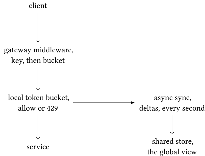
figure 164: local buckets on the hot path, the shared store off it, sync in between
