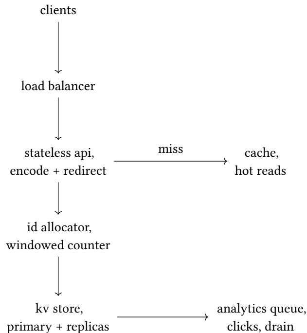
figure 163: the shortener: stateless edges, an allocator per pod, one store, cache beside
