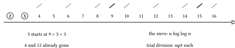
figure 20: each prime starts crossing at p times p , the smaller multiples are gone
