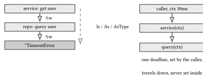
figure 67: errors chain through %w, timeouts travel down the context
