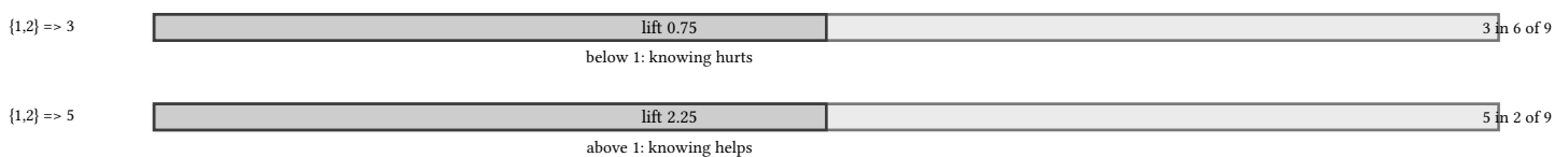
figure 134: same confidence 0.5, opposite lift: the consequent's own support decides
