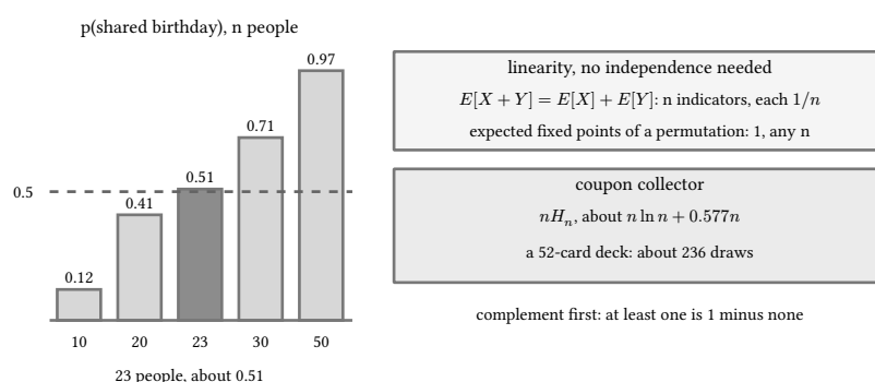
figure 124: the birthday ladder crosses one half at 23 people, linearity turns sums into additions
