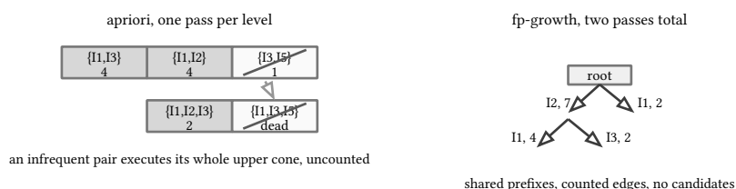
figure 132: one dead pair kills its whole upper cone, the tree shares prefixes and counts edges
