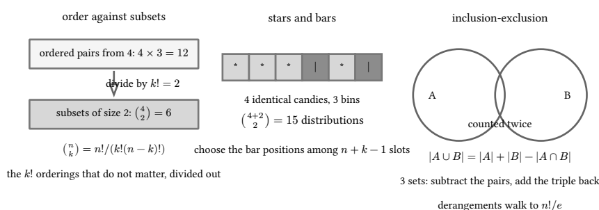
figure 125: order divides out, bars make bins identical, the overlap is added back once
