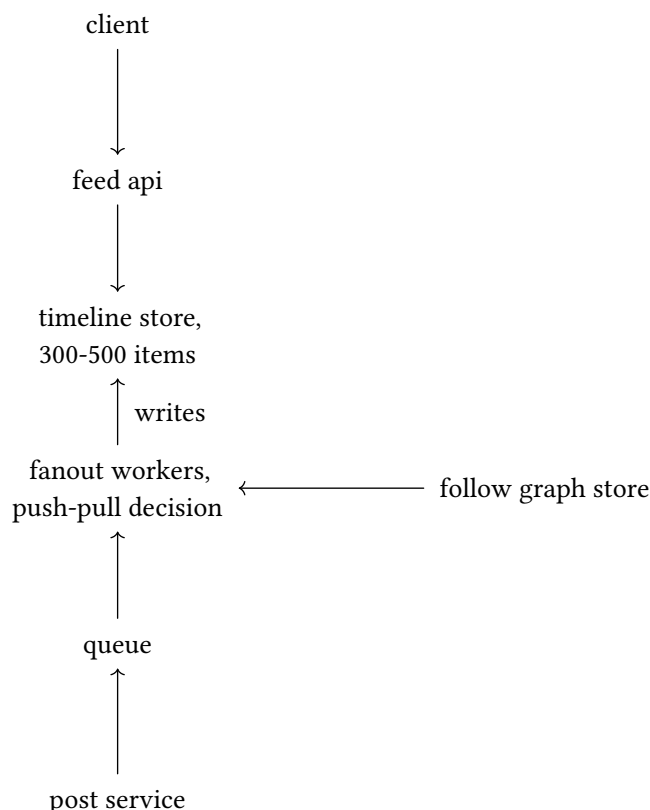
figure 165: posts through a queue to fanout workers, readers hit the timeline
