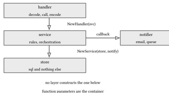
figure 69: four layers wired by constructor injection, no layer builds another
