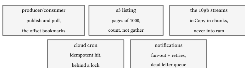
figure 92: the remaining inventory in one composite: queue, page, stream, lock, fan-out
