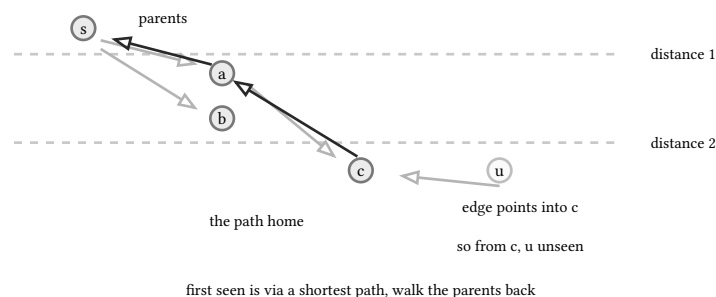
figure 17: first seen is via a shortest path, the parents walk it home
