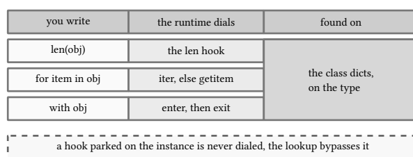
figure 137: implicit calls dial hooks on the type, the instance's namespace is bypassed
