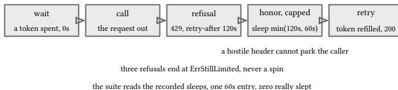
figure 95: the capped retry: one 429, one minute, the retry lands
