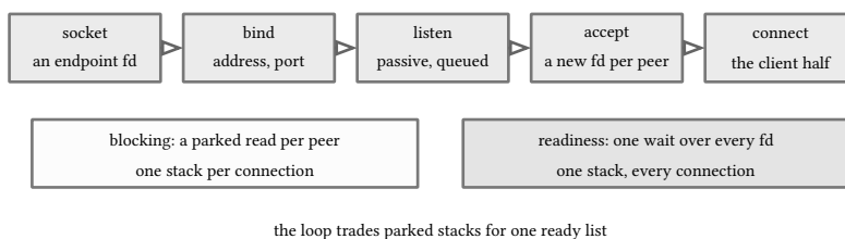
figure 122: socket, bind, listen, accept, connect, then the two shapes over the connections
