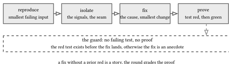
figure 180: reproduce, isolate, fix, prove, the failing test arrives before the fix
