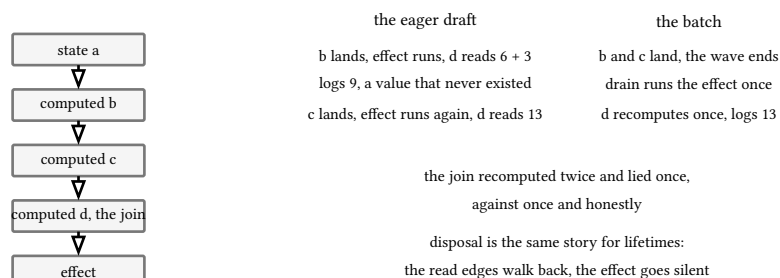
figure 44: one set, one join recompute: the eager draft logged a value that never existed
