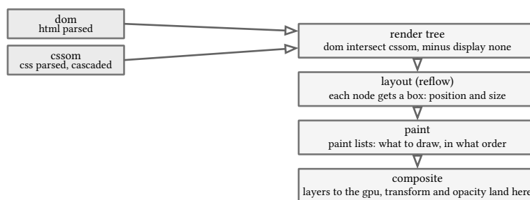
figure 151: two trees in, a render tree out, then the three stages, each producing its own artifact
