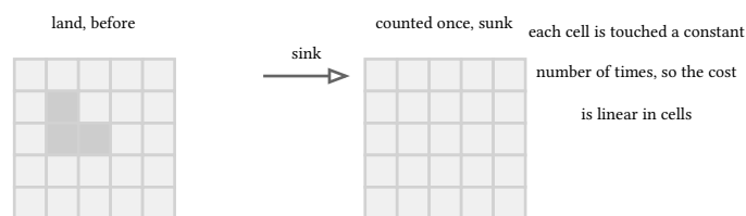
figure 24: the scan counts once per island, the sink claims the whole thing
