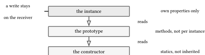
figure 32: reads walk the chain, writes stay on the receiver
