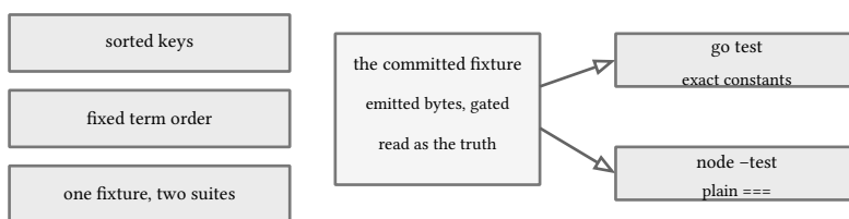
figure 73: the three rules, one fixture, two suites, plain equality on both sides
