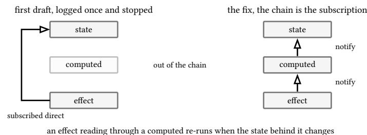
figure 43: the subscription edge, through the computed, never around it
