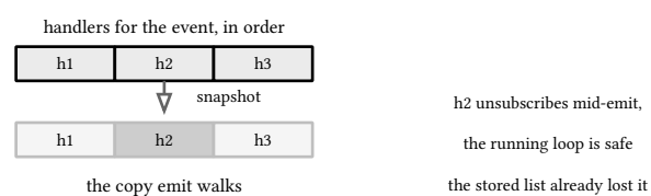
figure 39: registration-ordered list, emit iterates a copy
