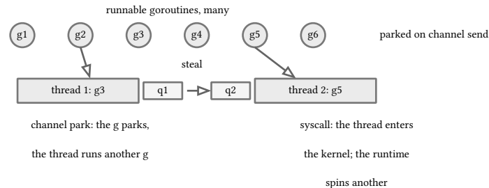
figure 62: M goroutines multiplexed onto N threads: park versus syscall
