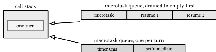
figure 33: one call stack, the microtask queue drained to empty between macrotask turns
