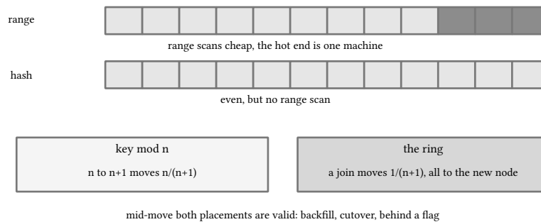
figure 114: range concentrates the hot end, hash spreads evenly, the join sets the blast radius
