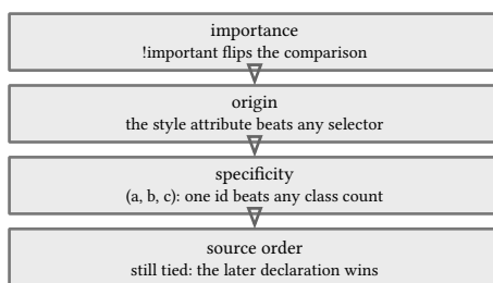
figure 148: the cascade ladder, one rung per tiebreaker, the first difference decides
