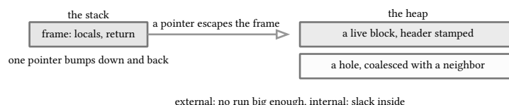
figure 118: the stack bumps and dies with the return, the heap waits for the free
