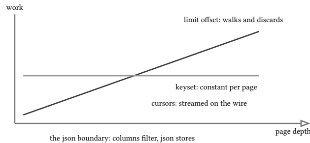
figure 79: offset cost grows with depth; keyset stays constant
