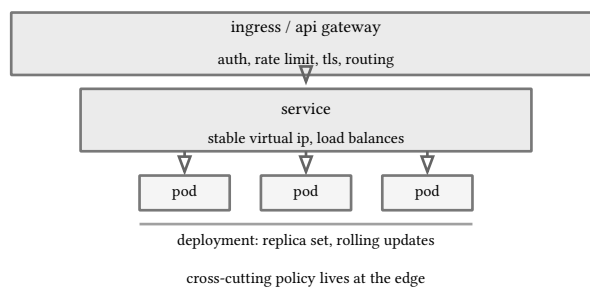
figure 87: ingress fronts services, services balance across pods
