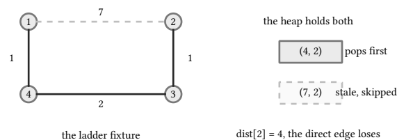
figure 109: one node, two entries: the shorter candidate wins the pop, the longer surfaces later and is skipped
