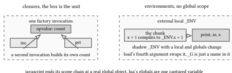
figure 142: one upvalue box per executed declaration, the chunk's globals one captured _ENV
