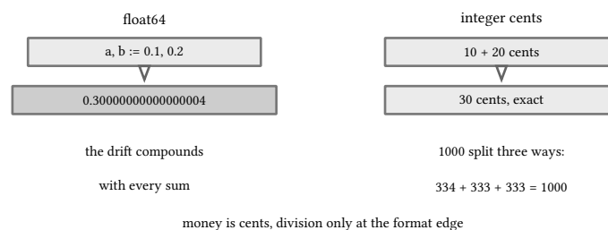
figure 75: float drifts, cents stay exact, splits sum back
