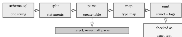
figure 96: split, parse, map, emit, with loud rejection
