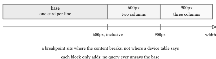
figure 150: the breakpoint ladder: the base is always on, each block adds from its threshold rightward
