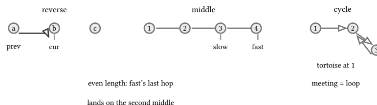
figure 22: three two-pointer dances over one node type
