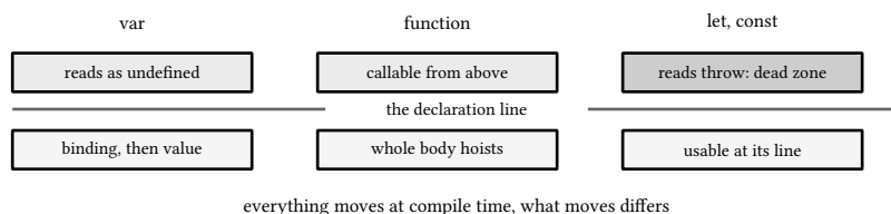
figure 28: what moves at compile time, per keyword
