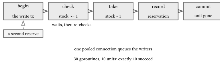
figure 97: check, take, record in one transaction: no double sell
