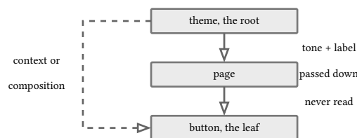
figure 49: drilling repeats the downward flow until a leaf uses what the root had
