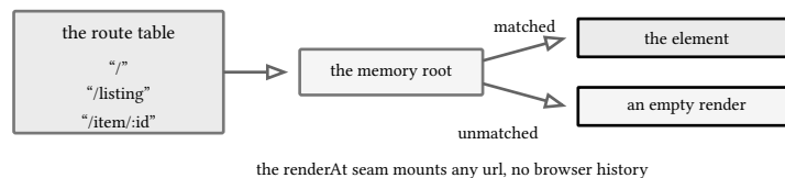
figure 53: routes as data under one in-memory root, any url mounted
