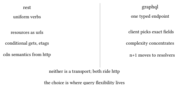
figure 85: rest against graphql: where the flexibility lives
