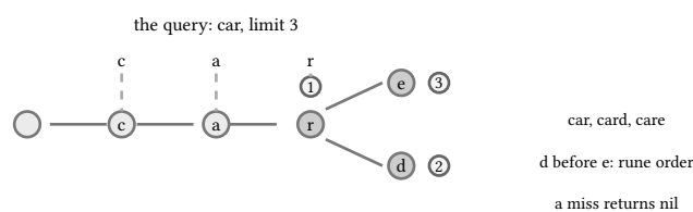
figure 26: walk to the prefix node, enumerate in rune order, cap at the limit
