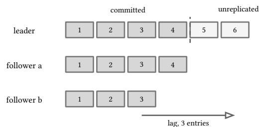
figure 113: the leader's log, two followers behind it, the gap is the lag
