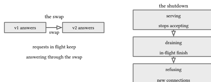
listing 107: the deployable front swaps handlers; GracefulShutdown drains with a timeout (source: interview-repertoire/samples/ch21-go/storefront.go, lines 254-288)
