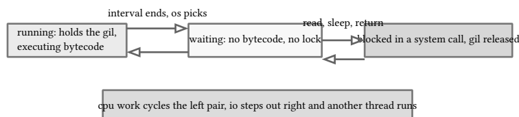
figure 136: one thread through the gil: the two ways out of running, only one of them overlaps
