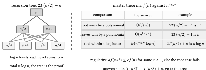
figure 123: the recursion tree sums level by level, the theorem only compares the root against the leaves
