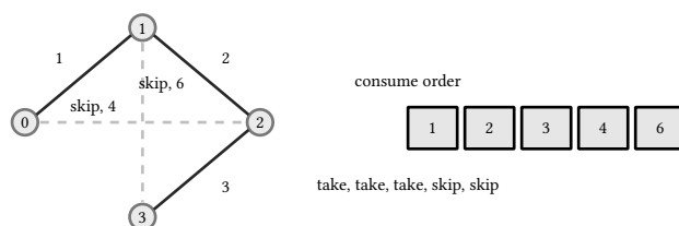
figure 111: the box fixture: the 1, 2, and 3 edges span, the 4 and the 6 would close cycles
