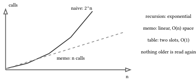
figure 25: one recurrence, three costs: exponential, cached, two rolling slots
