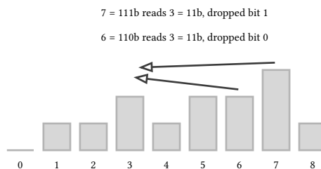
figure 107: the ladder's row is its parent plus the bit it dropped
