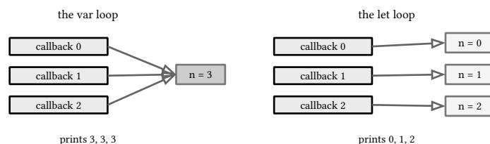
figure 29: one shared cell prints 3, per-iteration cells print 0 1 2
