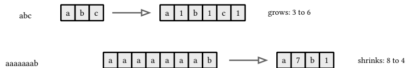
figure 27: counts always emitted: singles grow, runs shrink
