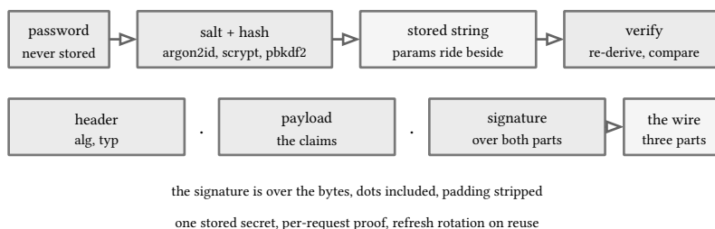
figure 158: the hash lane proves who you are once, the token lane carries the proof per request
