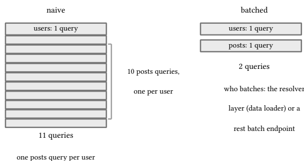
figure 57: ten users naive is 11 queries, batched is 2
