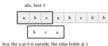
figure 103: the edge only ever moves right, a repeat outside the window cannot shrink it
