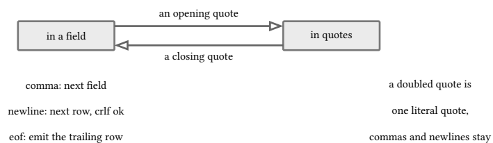
figure 45: the quote state machine: doubles escape, the trailing row still emits
