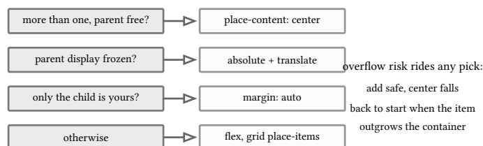
figure 36: which centering tool when: the ladder the model walks
