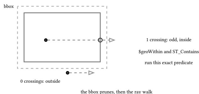
figure 80: ray casting east: odd crossings inside; the bbox prunes first
