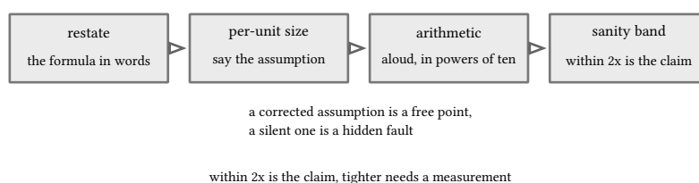
figure 159: the four moves, in order, every estimate
