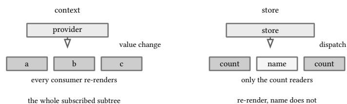
figure 55: context versus a store: who re-renders on a change
