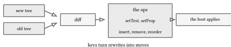
figure 50: elements are data, the diff emits ops, the host applies them
