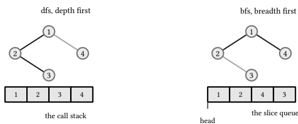
figure 16: two frontiers, one visited set: the call stack against the head-indexed queue
