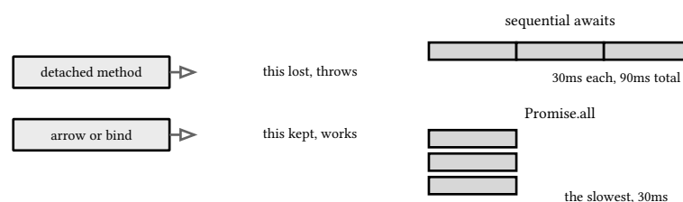
figure 37: this binds at the call site or lexically, awaits sum or take the slowest
