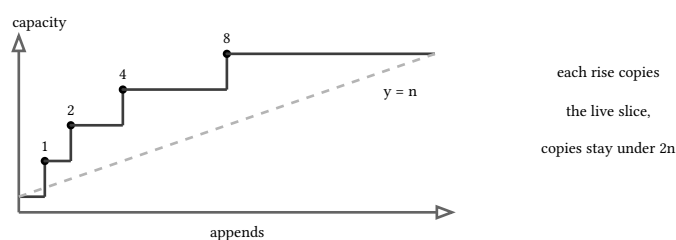
figure 9: the capacity stair-step against n , why append is constant on average
