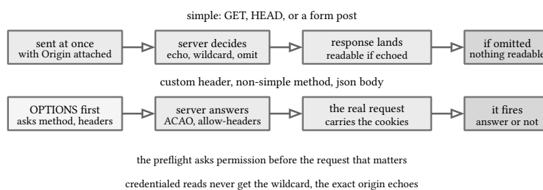
figure 156: the two lanes: simple requests fly, everything else asks first
