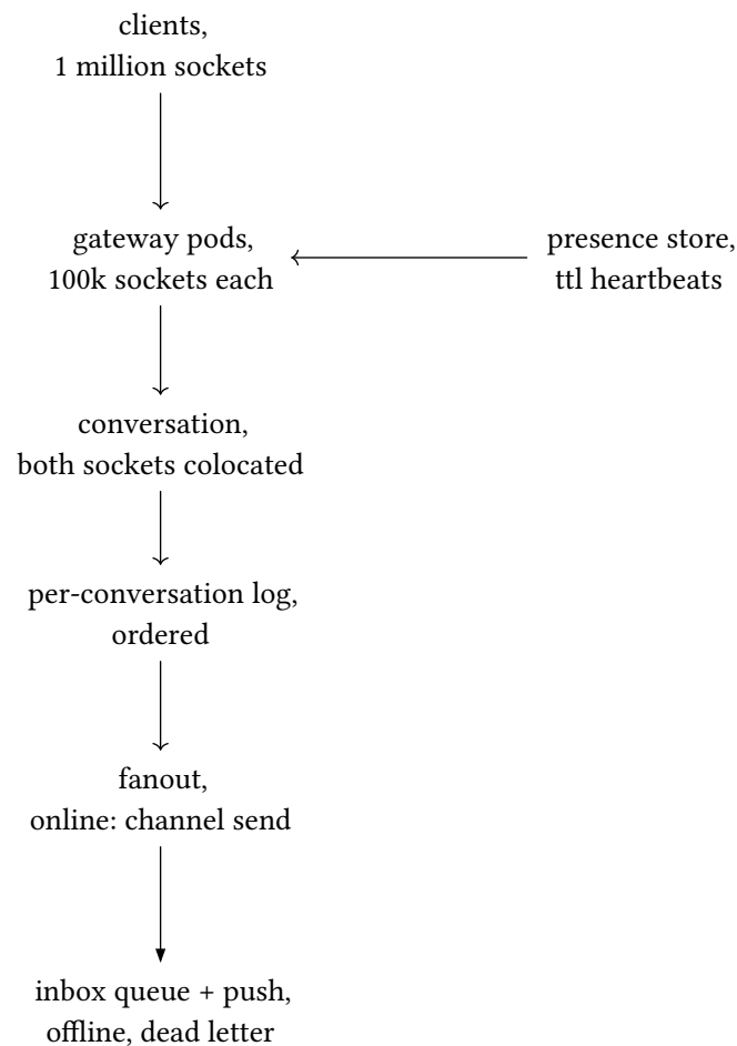
figure 166: hash by conversation, both sockets on one pod, inbox for the offline
