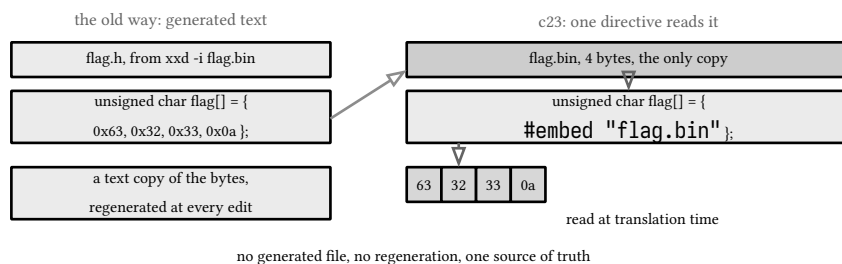
figure 7: generated header versus embed, same four bytes through the old path and the c23 path
