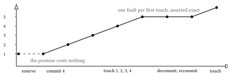
figure 48: cumulative faults across the sample’s lifetime: flat through reserve and commit, one step per first touch
