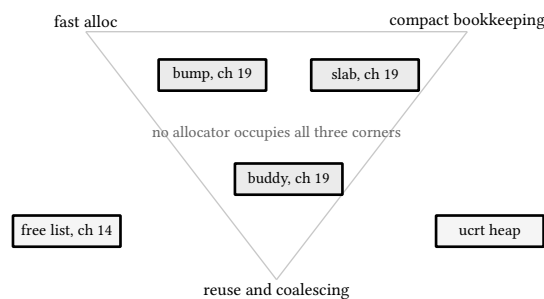
figure 74: the contract triangle and where each allocator in this chapter sits
