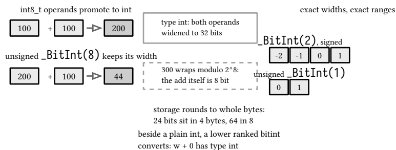
figure 10: the promotion lanes, int8_t widens to int , unsigned _BitInt(8) wraps in place
