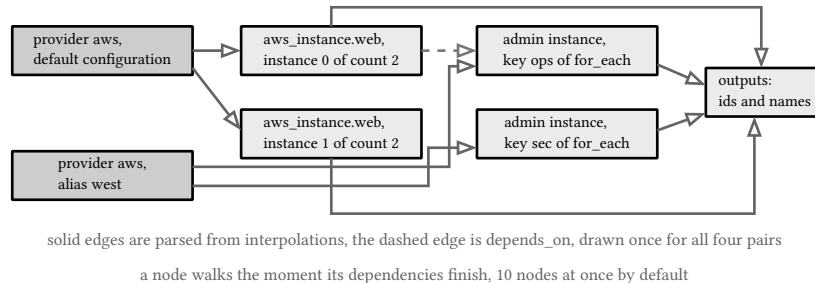
figure 101: the graph implied by the sample: two provider configurations feed four resource instances, outputs read them all
