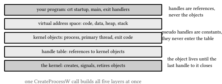
figure 41: one process as five layers, what each layer holds, and who owns it
