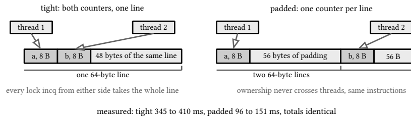
figure 51: one line, two owners, and the coherence traffic that follows
