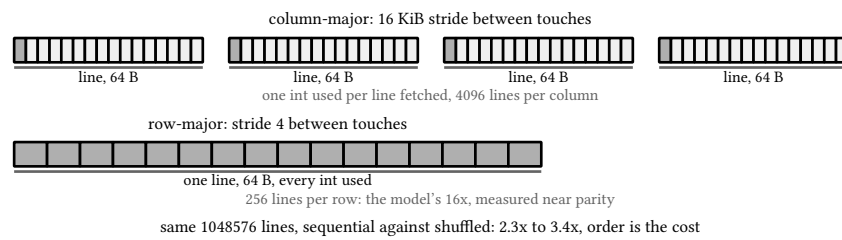
figure 50: before and after: the same matrix column by column and row by row
