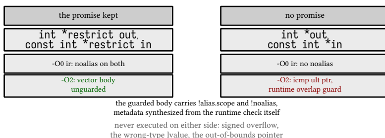
figure 18: one word of promise, two machines: what the -O2 ir shows for each twin
