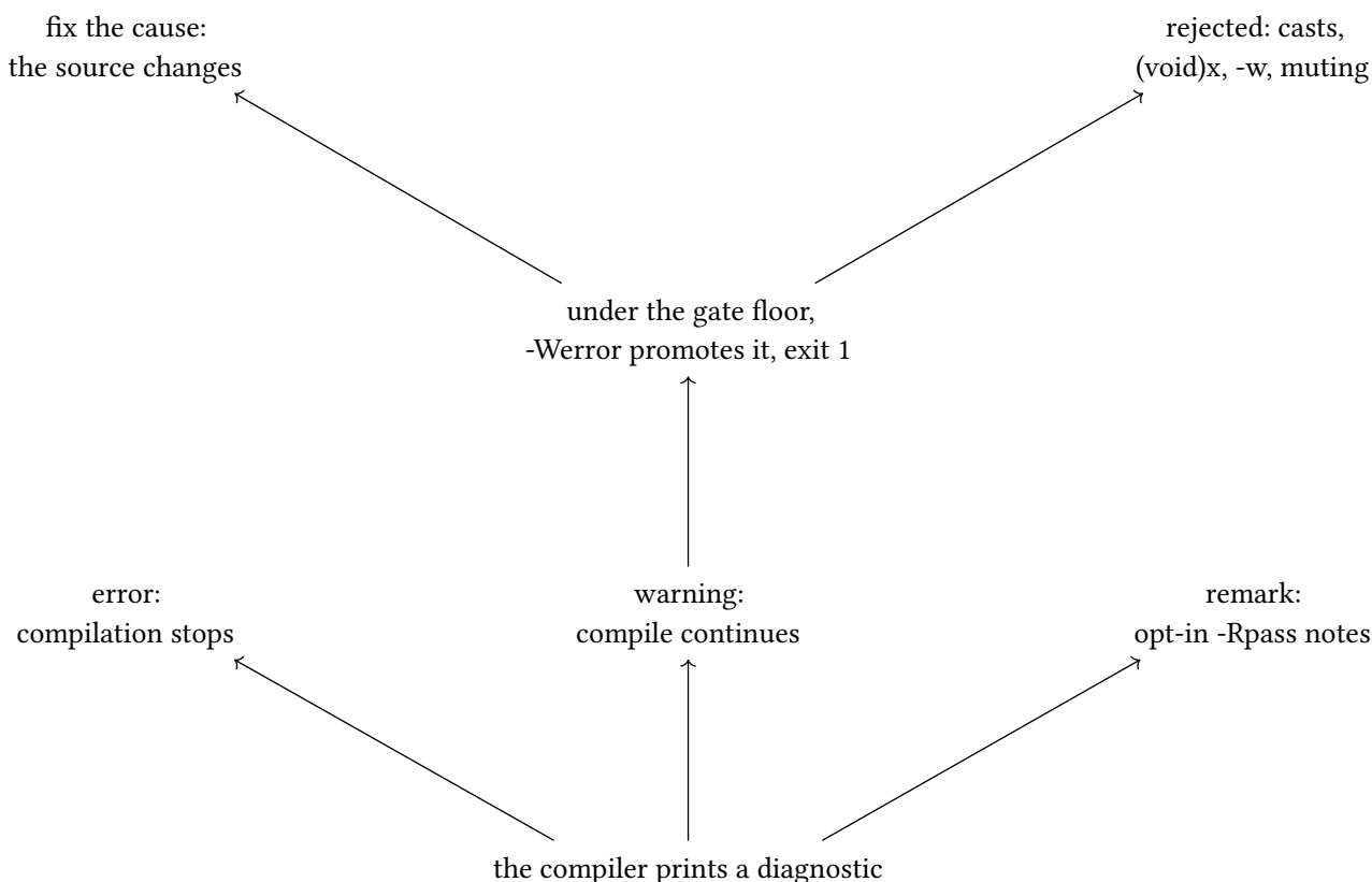
figure 37: the diagnostic taxonomy and the fix discipline under the gate
