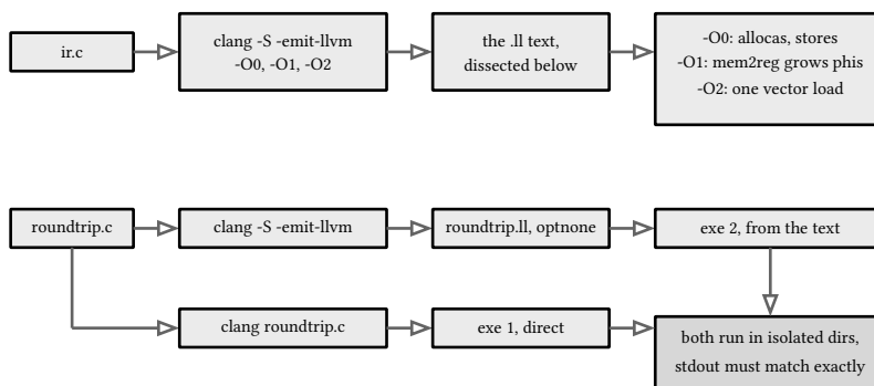
figure 29: one source, two routes through the driver: one stops at the text for reading, one compiles the text back and demands the same output
