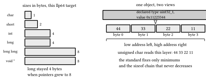
figure 9: sizes this target chose, and the two views of one uint32_t object
