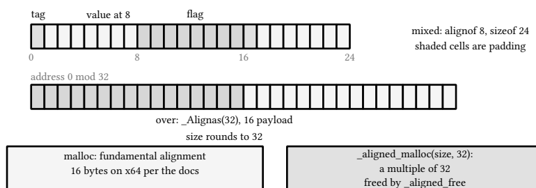
figure 15: padding inside struct mixed, the 32 byte lift, and the two allocators' promises
