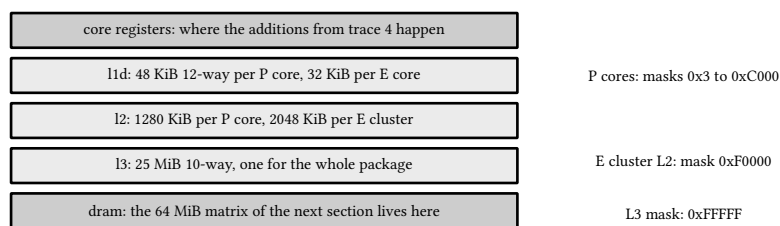
figure 49: the hierarchy the probe reported, one layer per level, the 64-byte line riding every boundary
