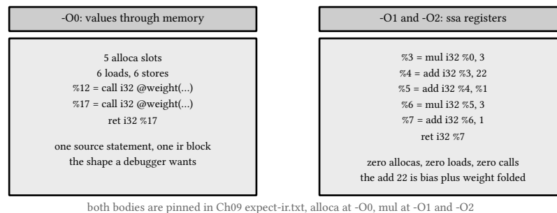
figure 33: the same mix at -O0 and at -O1, -O2, mem2reg deleted every alloca the frontend needed
