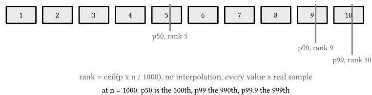
figure 84: a sorted sample of ten with the rank marks p50, p90, p99 sit on
