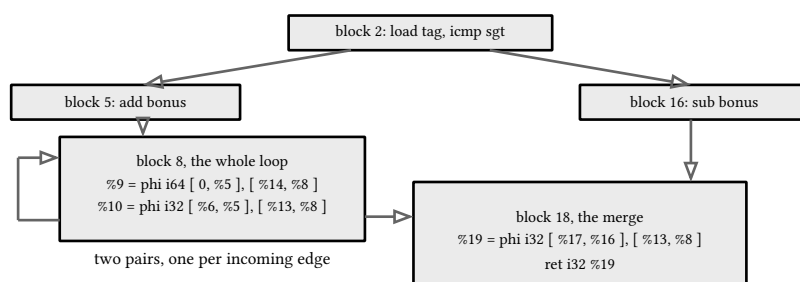
figure 30: tally at -O1 : blocks, the back edge, and the three phis with the pairs they merge
