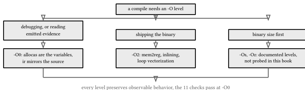
figure 36: choosing a level, and what each answer buys
