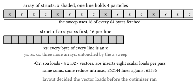
figure 52: the same particles two ways, and what each -O2 kernel loads
