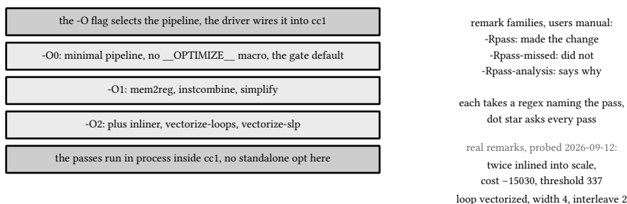
figure 27: the pass pipelines the -O flags select, and the remark families that report them
