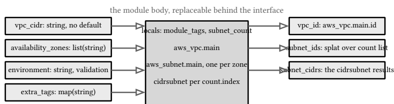
figure 105: the module as a data structure: variables enter left, outputs leave right, locals never leave
