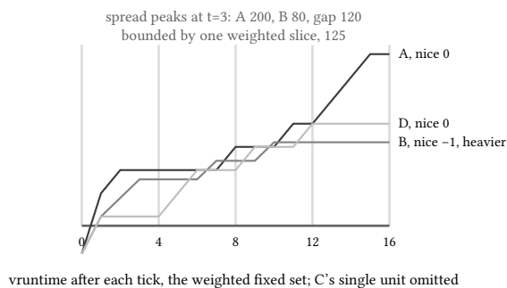
figure 69: vruntime trajectories of the weighted run: three lines converging inside one weighted slice
