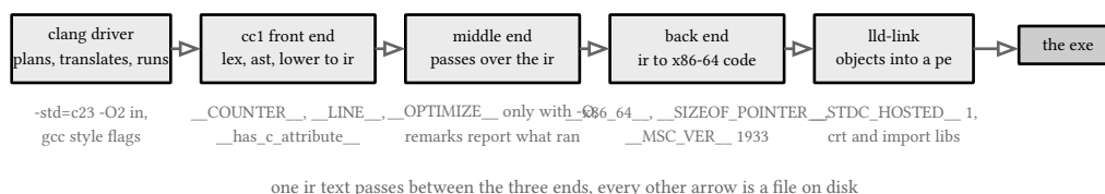
figure 25: the pipeline the driver runs, one box per stage, and the fingerprints each stage leaves
