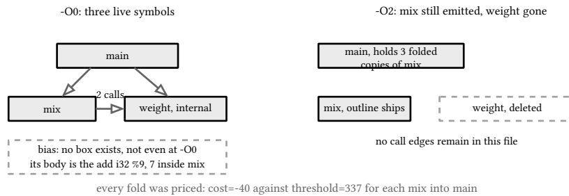
figure 34: the call graph of mem2reg.c at -O0 and at -O2, weight vanishes, mix survives standalone
