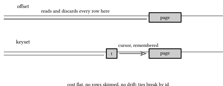
figure 154: offset walks the whole prefix, keyset jumps to the remembered position
