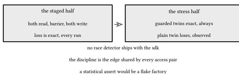
figure 185: the canary's two halves, one bug class
