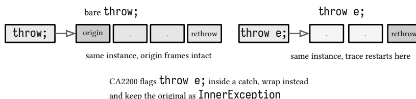
figure 55: rethrowing, one word decides whether the origin survives
