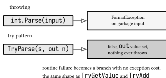
figure 56: two error models, throwing parse vs try pattern
