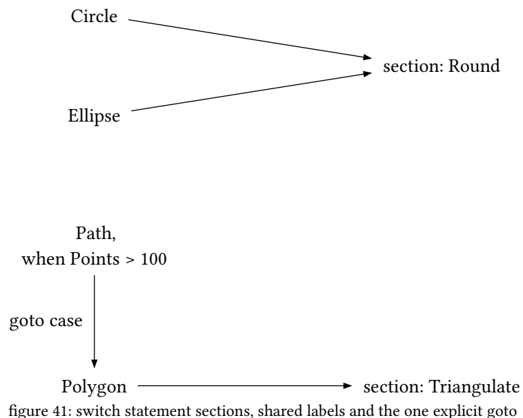
figure 41: switch statement sections, shared labels and the one explicit goto
