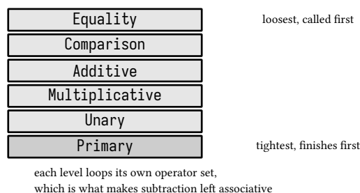
figure 233: precedence as call depth, tighter operators deeper
