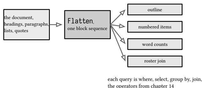
figure 115: the sample as pipelines, flatten once then query
