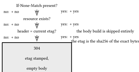
figure 181: the conditional GET decision
