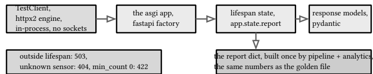
figure 213: the served report's layer stack, and the status codes at the edges
