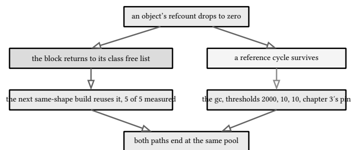
listing 160: the recap checks: thresholds unchanged from chapter 3, the churn absorbed, gen0 counted (source: python/samples/src/Ch13/freelists.py , lines 50-71)
