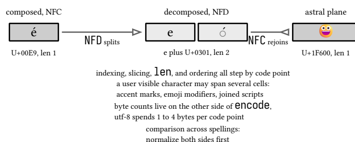
figure 17: the same character, three spellings, and what indexing sees
