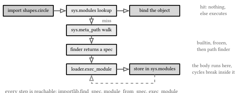
figure 42: one import statement as a state walk: cache probe, meta path, spec, execution, binding
