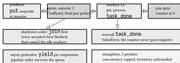
figure 90: the queue as a data structure: bounded inventory between producer and workers, the unfinished counter gating join, the semaphore gating concurrency
