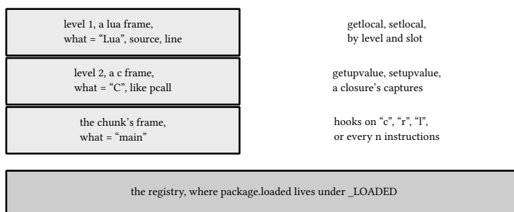
listing 106: classification by what field, traceback through xpcall (source: lua/samples/ch13_stdlib3.lua, lines 5-23)
