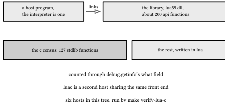
figure 63: the seam from both sides, a host linking the library
