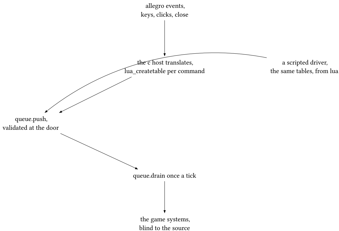
figure 92: two producers, one queue, one consumer
