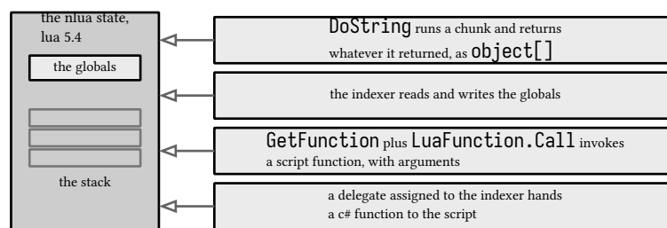
figure 52: the host's four moves over one nlua state, the stack shape the lua book teaches in c
