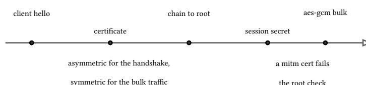
figure 84: handshake with asymmetric, bulk with symmetric
