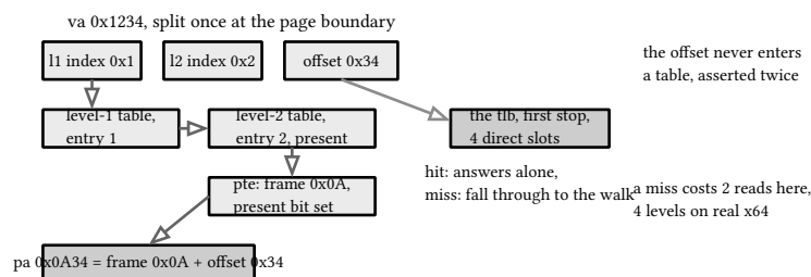
figure 46: va 0x1234 through the machine: the split, the tlb, both levels, the frame
