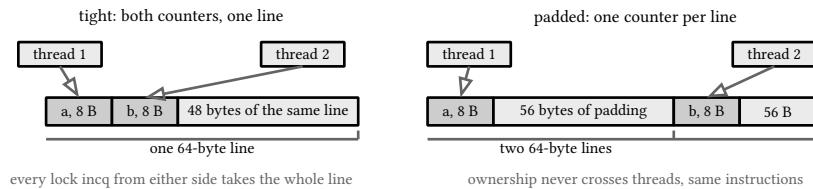
figure 51: one line, two owners, and the coherence traffic that follows
