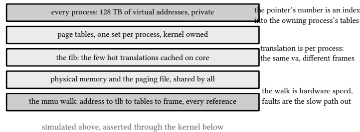
figure 45: from pointer to dram: what each layer owns and who sees it
