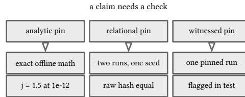
figure 182: the three pin tiers: analytic constants inside a stated epsilon, relational bit equality across runs, witnessed numbers pinned from the deterministic binary
