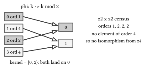
figure 99: the parity map collapses z_4 onto z_2 with kernel \{0,2\} , while the order census separates z_4 from z_2 \times z_2 with no map at all
