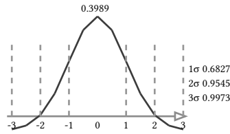
figure 111: standard gaussian with the 1, 2, and 3 sigma bands
