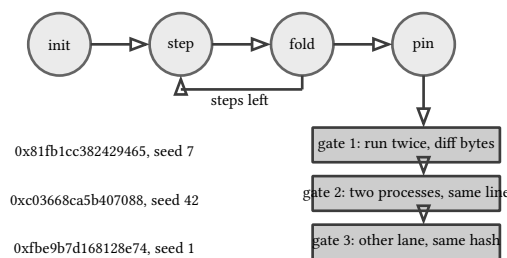
figure 192: the driver's hash discipline as a state machine: seed to init, the step and fold loop, then three comparison gates closing on the pins
