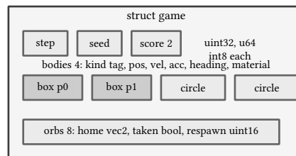
figure 181: the game state as one value: scalar bookkeeping, a tagged body array, and an orb array, everything fixed capacity
