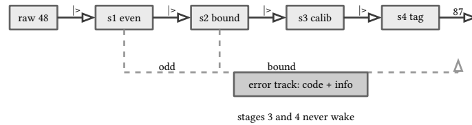
figure 174: the happy track with the macro sugar, the dashed error track bypassing the later stages
