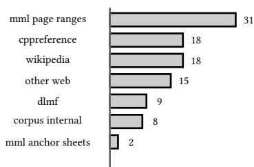
figure 198: the source base by class, the url prefix decides the class, bar length is row count
