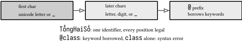
figure 7: identifier grammar, position one, later positions, and the @ escape
