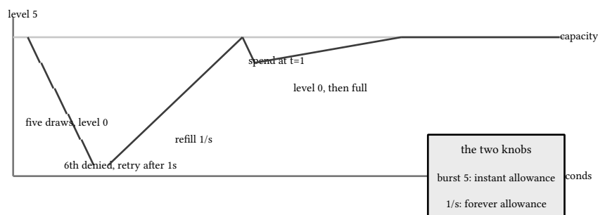
figure 194: bucket level over one draw timeline, the refill climbing between bursts
