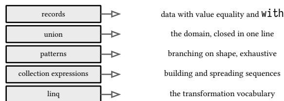
figure 112: five pieces, one job each, composed into one style
