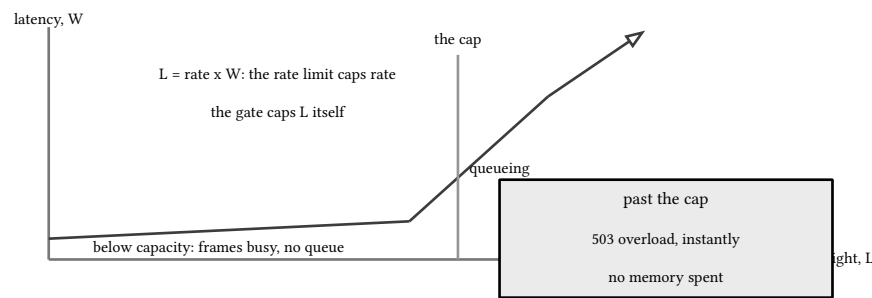
figure 198: latency versus in-flight: the hockey stick the gate cuts
