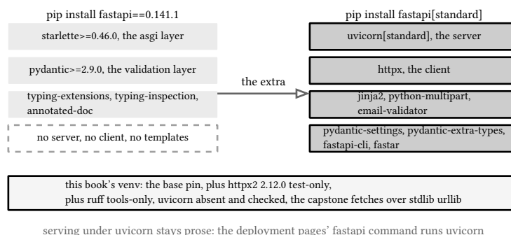
figure 95: the two installs, before and after the extra
