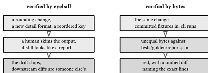
figure 212: the same behavior change, verified by eyeball and verified by bytes
