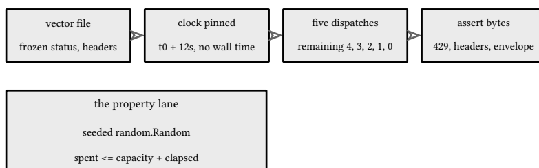
figure 176: the fixed-vector pipeline: file in, draws through the layer, bytes out
