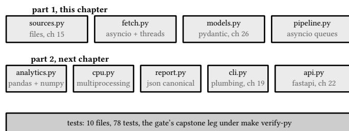
figure 204: the nine modules and the pillar chapter each one assembles
