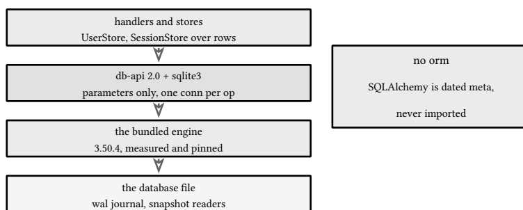
figure 149: the stack the store sits on, one borrowed connection at a time
