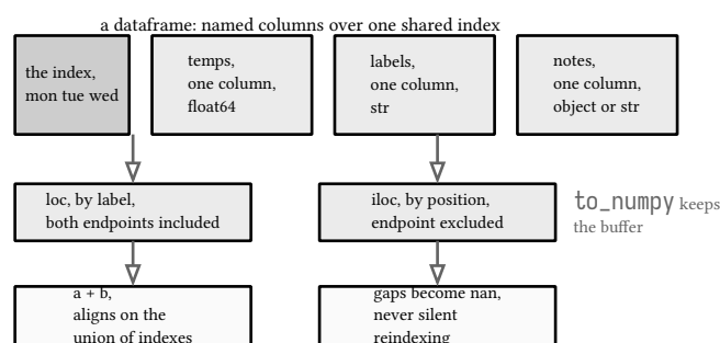
figure 104: a frame as columns over one shared index, the two addressing doors, and the union rule
