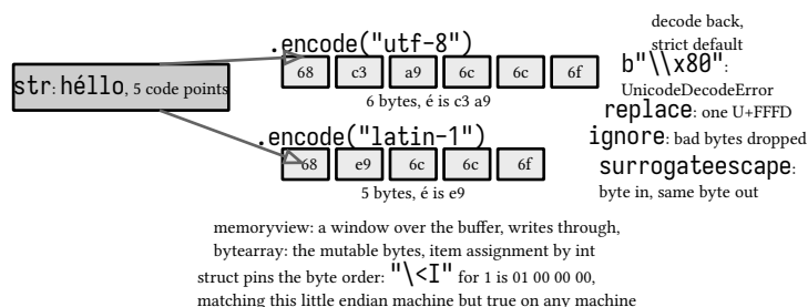
figure 18: one word through encode and decode, and where each error policy lands
