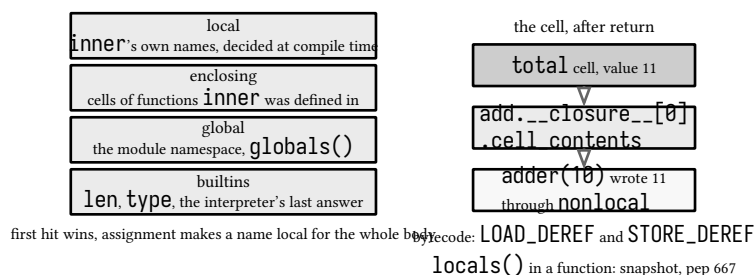
figure 21: the legb stack, and the cell a closure carries
