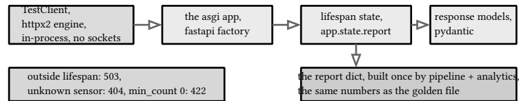
figure 213: the served report's layer stack, and the status codes at the edges
