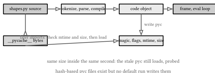
figure 45: source to running code: the two trips, first import and every later one
