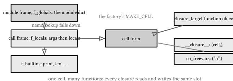
figure 46: a frame and its chain, with a cell bridging two frames
