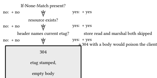
figure 158: the conditional GET decision
