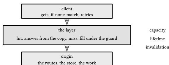
figure 164: the layer sits between client and origin, answering what it can
