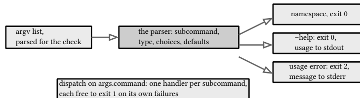
figure 80: where one argv list goes: dispatch and the three exits
