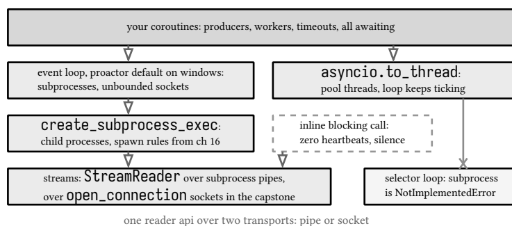
figure 91: the three ways off the loop as a layer stack: pool threads for blocking calls, child processes for real work, streams as the shared io surface, the selector alternative gated
