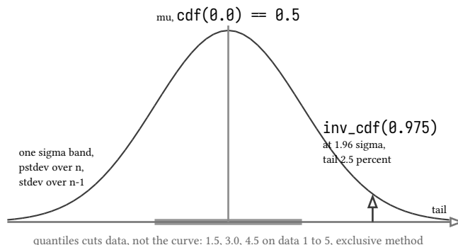
figure 97: the standard normal as a curve: cdf at zero, the 2.5 percent tail beyond 1.96 sigma, the one sigma band the two stdevs measure
