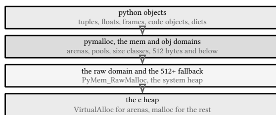
figure 49: the allocator stack: objects ride the mem and obj domains into pymalloc, raw memory and everything above 512 bytes ride the c heap
