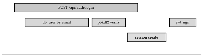
figure 181: one login request's spans over time, the tree the recorder prints
