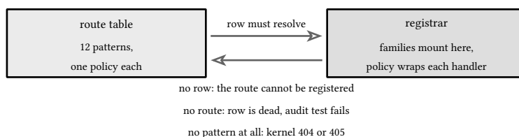
figure 147: the audit: table and registrar face each other, both directions checked
