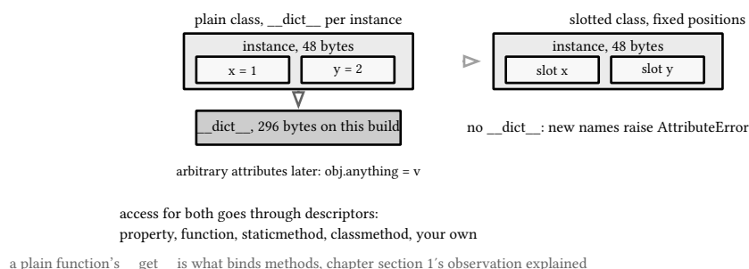
figure 28: where attributes live, with and without slots
