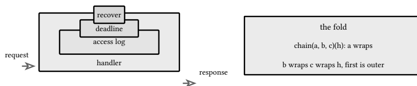
figure 119: the onion: first argument outermost, request in, response out
