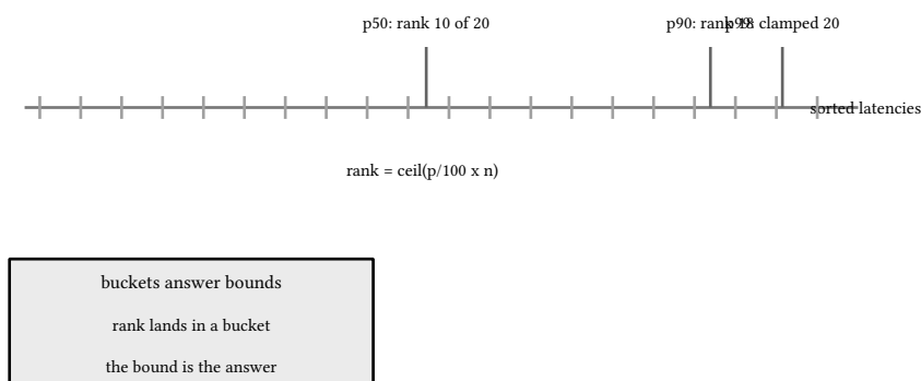
figure 183: the tail ladder: where p50, p90, p99 sit in one sorted sample
