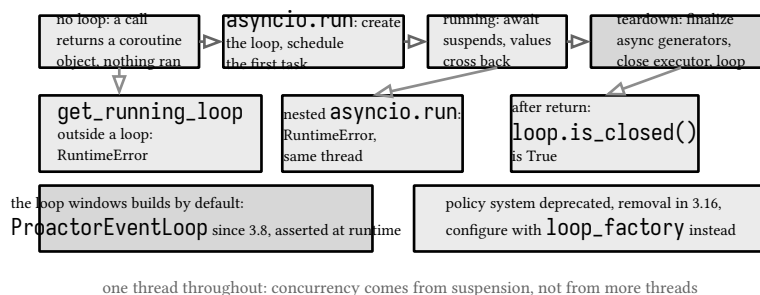
figure 88: the lifecycle of one asyncio.run as a state machine: no loop, loop created and driven, closed on return, the proactor default on windows
