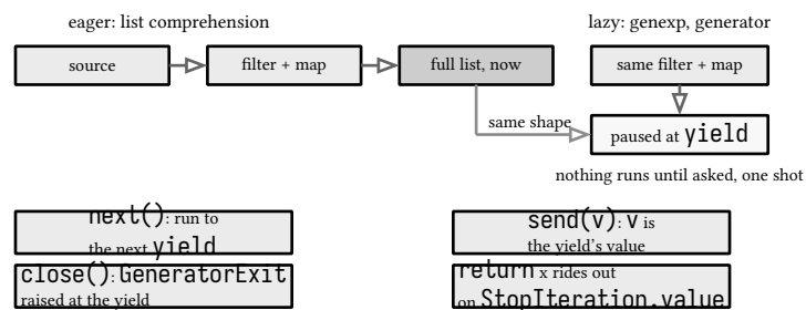
figure 15: one pipeline, two evaluations, and the two way generator channel
