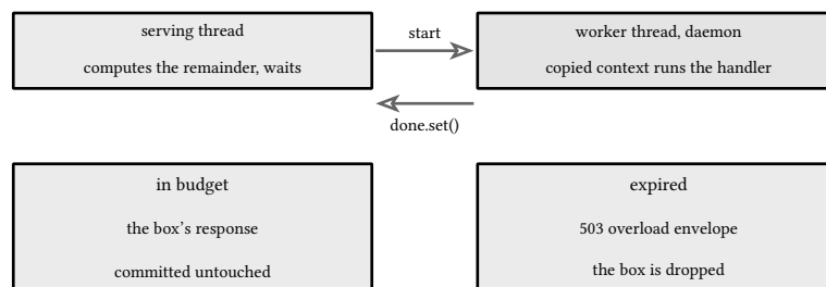
figure 123: two threads, one box: the wait decides who answers
