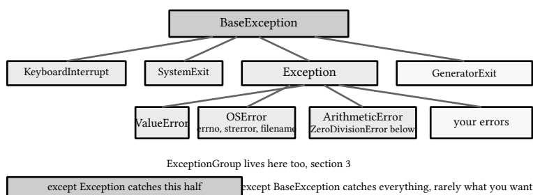
figure 37: the tree, and what a handler can see
