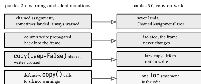
figure 105: before and after: the same four edits in the 2.x world and the 3.0 copy-on-write world
