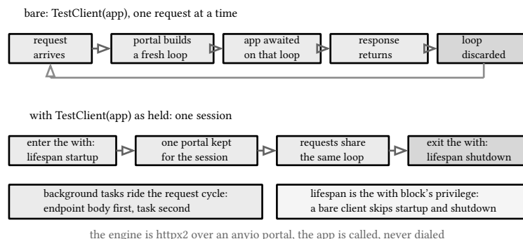
figure 94: the client's two modes as state machines: a fresh loop per request, or one held session with lifespan brackets
