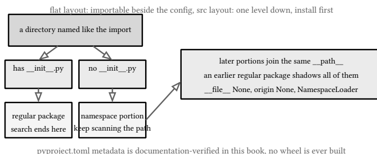
figure 43: layout as a decision: what the path finder does with a directory it is handed
