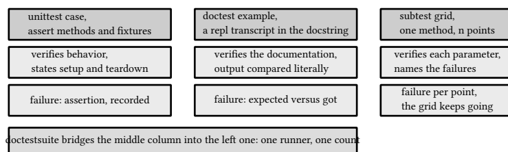
figure 86: three ways to state an expectation, and what each one verifies
