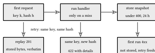
figure 159: one key's life: first run, snapshot, replay
