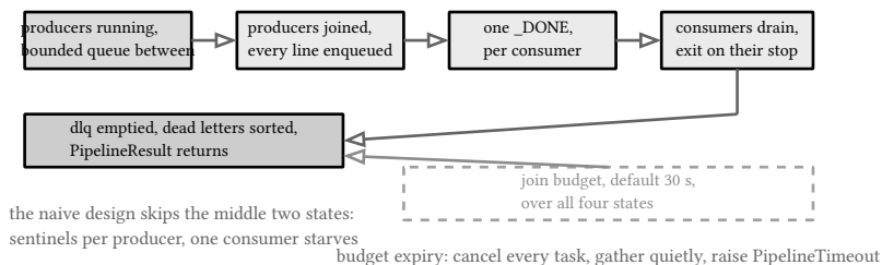
figure 207: the drain as a state machine: join, sentinel per consumer, exit, and the budget over all of it
