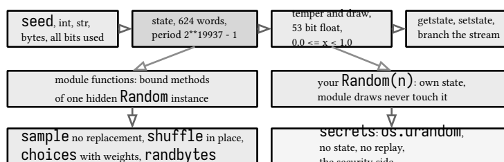
figure 99: random as a state machine: seed into 624 words of state, next per draw, module functions bound to the hidden instance, secrets on a different road entirely
