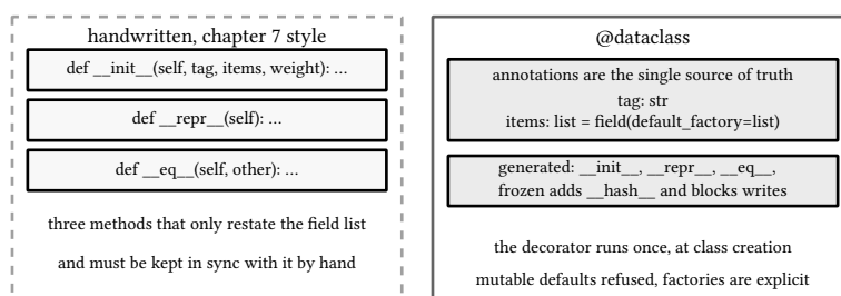
figure 33: the same record, handwritten and decorated
