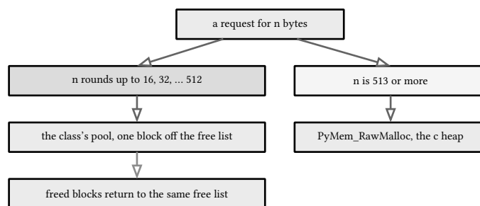
figure 51: the dispatch: a request rounds up to its class through 512, above it the raw heap takes the request unsized
