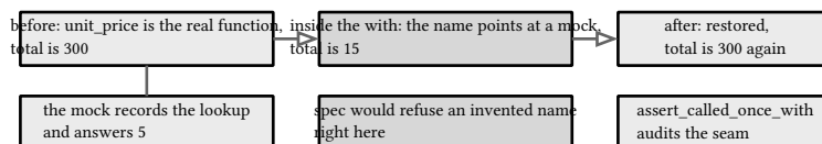
figure 85: one namespace before, during, and after a patch
