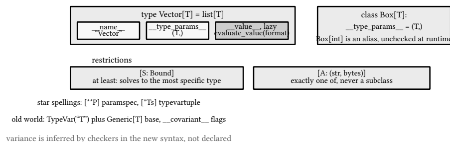
figure 30: what pep 695 builds, and where laziness sits
