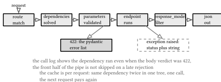
figure 93: the typed request pipeline with its two early exits
