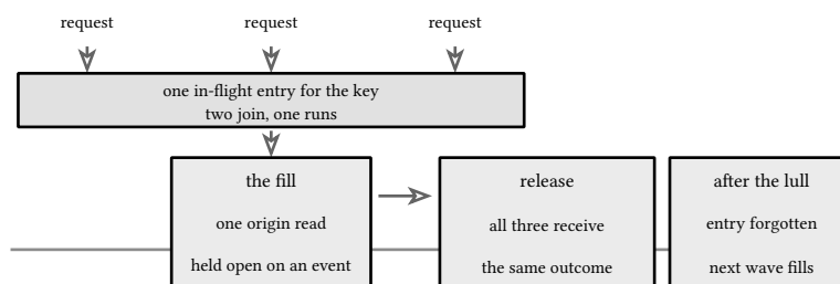
figure 160: three requests arrive together, one origin read happens
