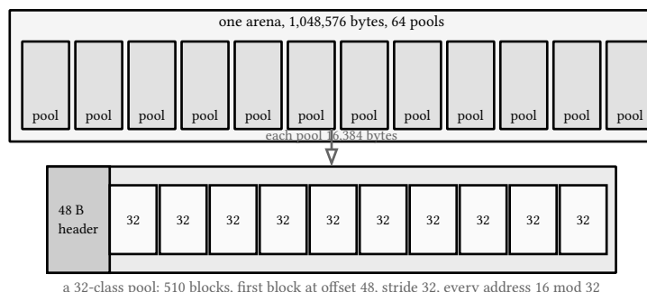
figure 50: one arena of 64 pools: each pool owns one class, the header costs 48 bytes, and blocks of the 32 class fill the rest at a fixed stride
