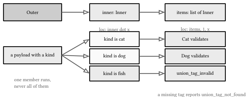
figure 110: the composed tree with its error paths, and the discriminator routing one payload to exactly one member
