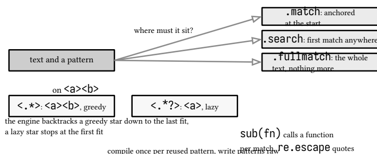
figure 19: choosing the matcher, and the two quantifier temperaments
