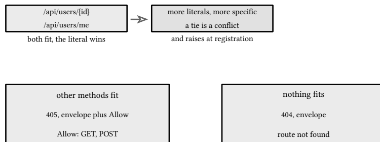
figure 113: literals beat parameters, ties raise at registration, leftovers split into 405 and 404
