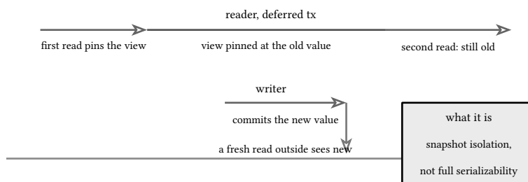
figure 153: one timeline: the reader's view holds
