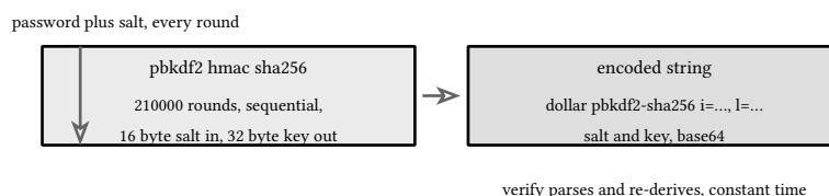
figure 133: pbkdf2: the salt and iteration count ride beside the derived key
