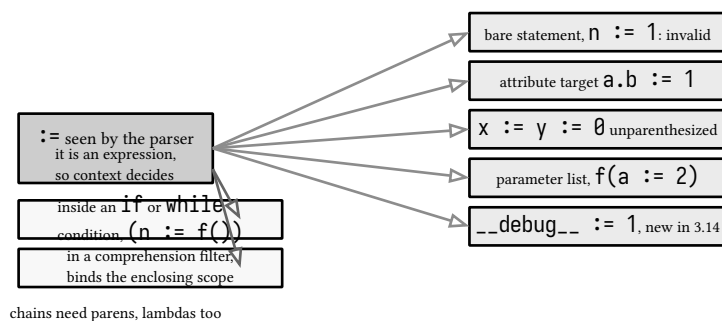
figure 8: where a walrus parses and where it is refused
