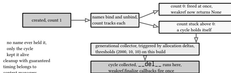
figure 12: the life of an object, refcounting first, the collector only for cycles
