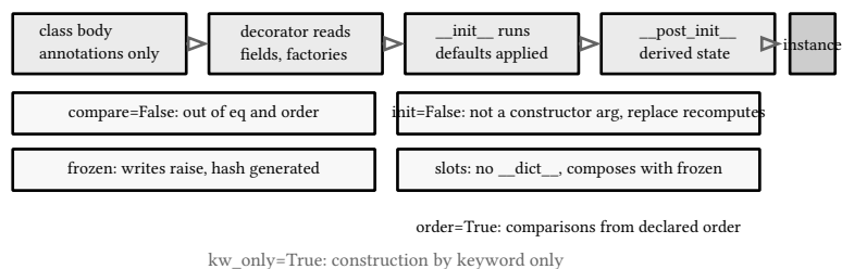
figure 34: the pipeline from decorator to instance, where each knob bites
