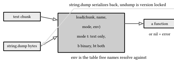
figure 4: load as the text to function boundary, the mode gate and the dump round trip
