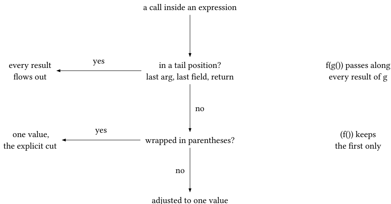
figure 25: when a call's results expand, and when they are cut
