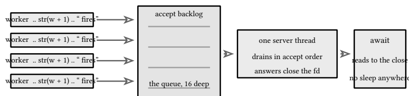
figure 162: one round of the driver: four connects, the backlog, answers in order
