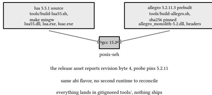
figure 89: the vendored toolchain, two libraries one compiler
