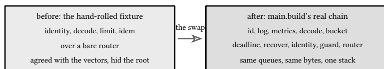
listing 244: the swap: the queues and seams feed main.build, the stack is the root's own (source: lua/service/tests/harness.lua, lines 29-51)
