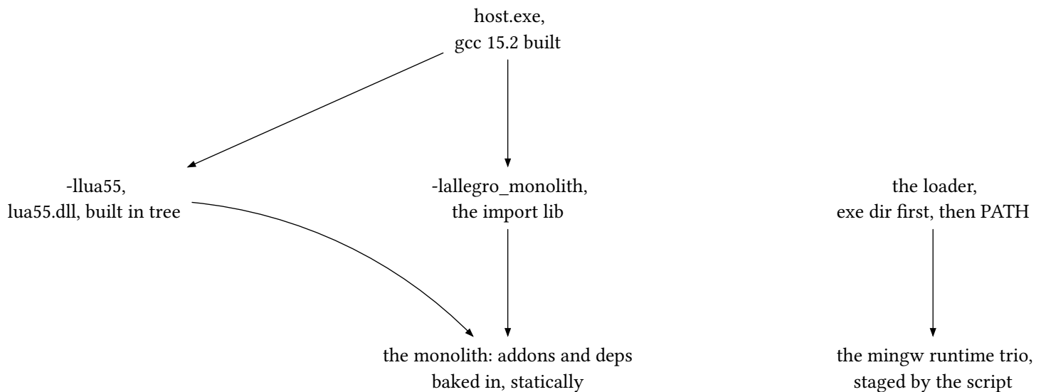
figure 90: one host binary, two libraries, the dlls it loads
