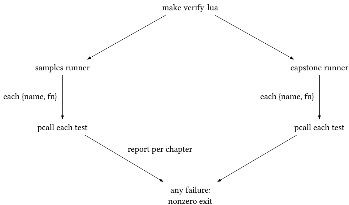
figure 2: the runner pipeline, chapter modules through pcall to the exit code
