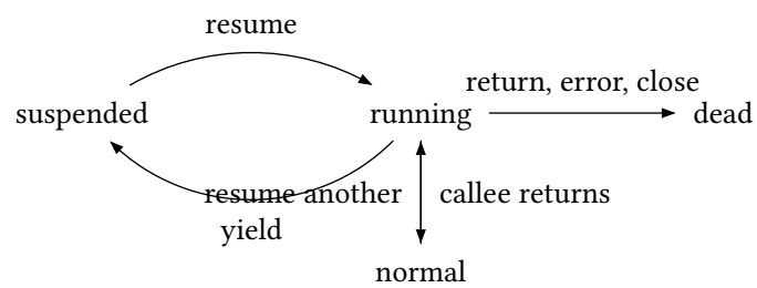
figure 33: coroutine states
