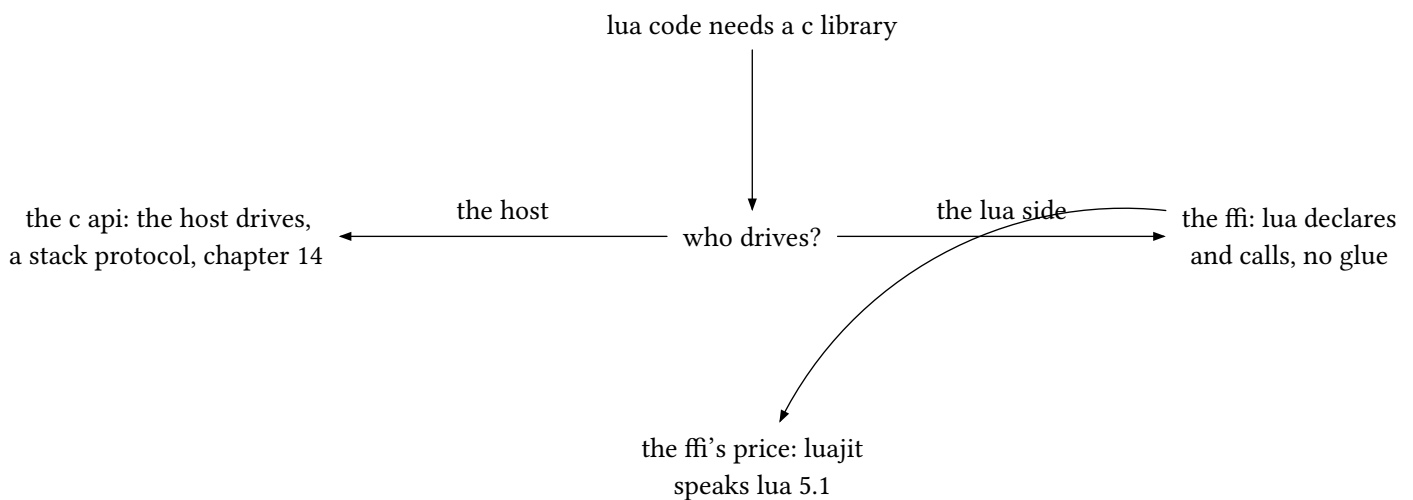
figure 82: the two roads to c, who drives the calls
