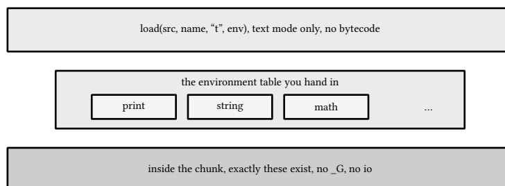
listing 139: a three function environment (source: lua/samples/ch16_idioms.lua, lines 160-165)
