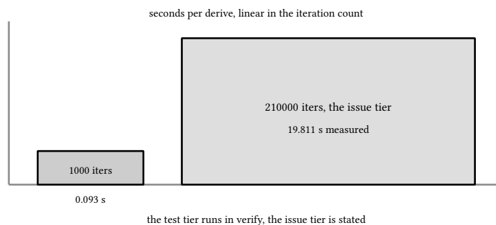
figure 117: the measured ladder: cost against iteration count, 2026-09-27 pin
