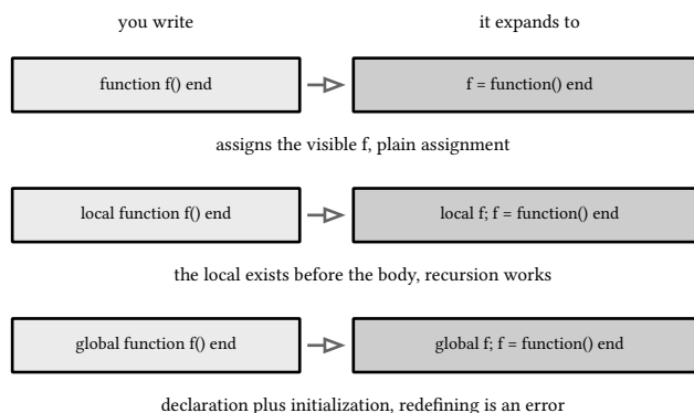
figure 24: the three definition sugars and what each expands to
