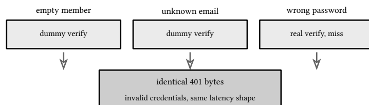
figure 118: three misses, one lane: the stopwatch learns nothing
