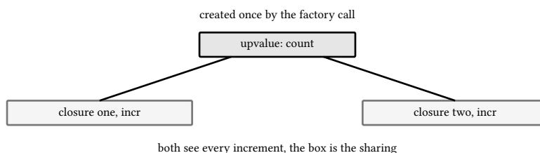
figure 27: two closures from one factory, one upvalue box between them
