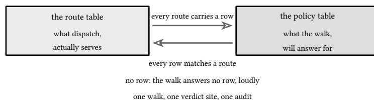
figure 128: the audit faces the tables: both directions, both named
