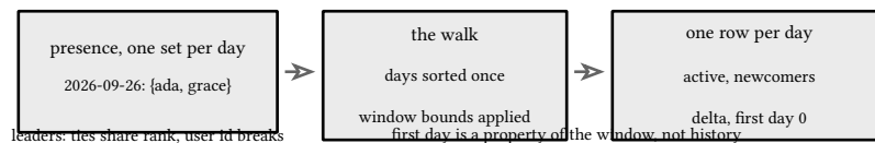
figure 167: events to series, the window bounds every step
