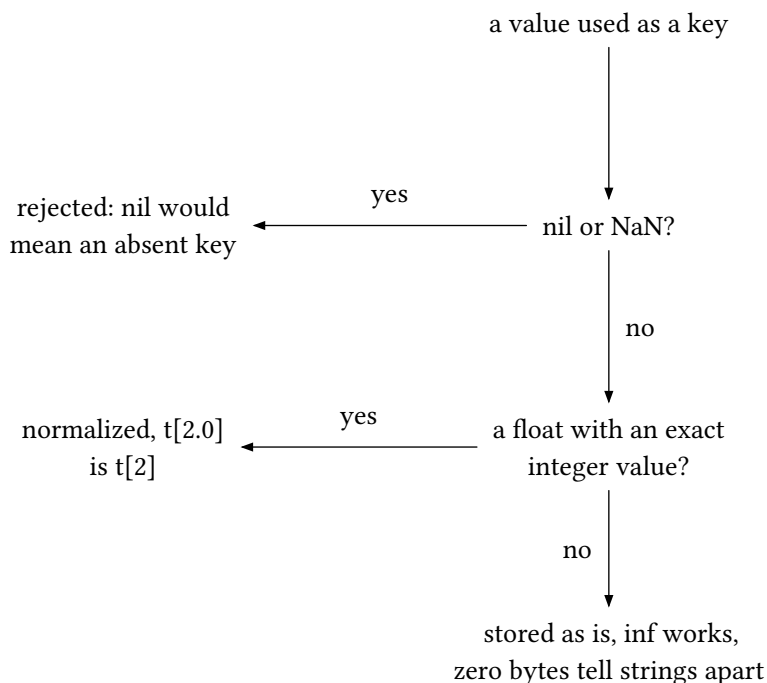
figure 11: what a table accepts as a key, the two rejections and the float normalization
