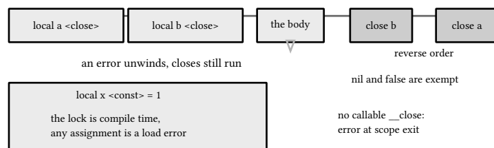
figure 21: the life of a block, const at compile time, closes at exit in reverse
