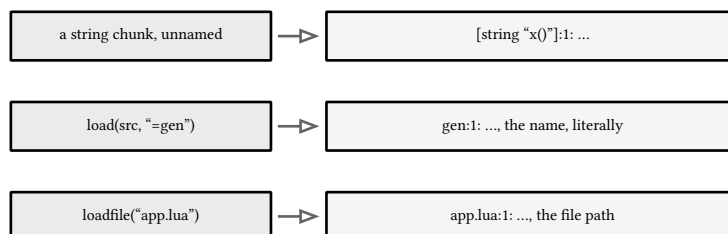
listing 128: the three prefix forms (source: lua/samples/ch14_capi.lua, lines 56-68)
