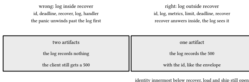
figure 107: wrong order versus right: where the log sits decides what it sees
