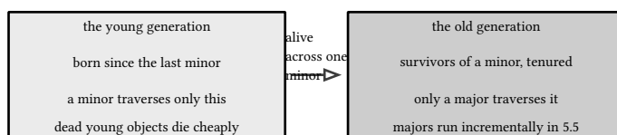
listing 65: tenured garbage is minor-proof, the major frees it (source: lua/samples/ch09_collector.lua, lines 120-139)
