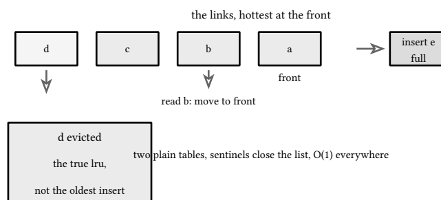
figure 141: a read moves its node to the front, an insert evicts the back
