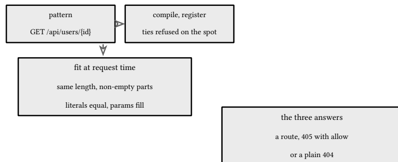
figure 96: compile once at registration, fit every request, refuse the ties
