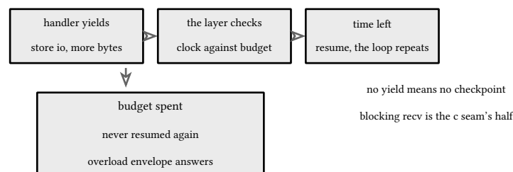
figure 105: each yield is a checkpoint, expiry is a refusal to resume
