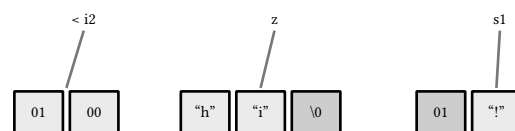
listing 95: round trip, byte order, sized strings (source: lua/samples/ch11_stdlib1.lua, lines 103-112)
