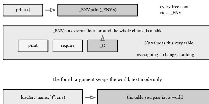
figure 34: how free names really resolve, and what load 's fourth argument swaps
