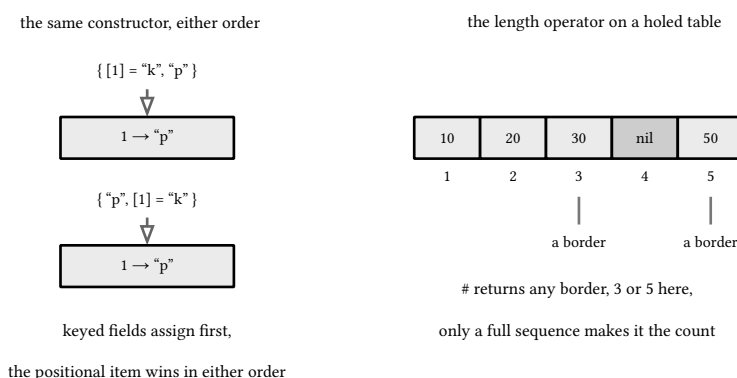
figure 19: constructor collisions and the length border
