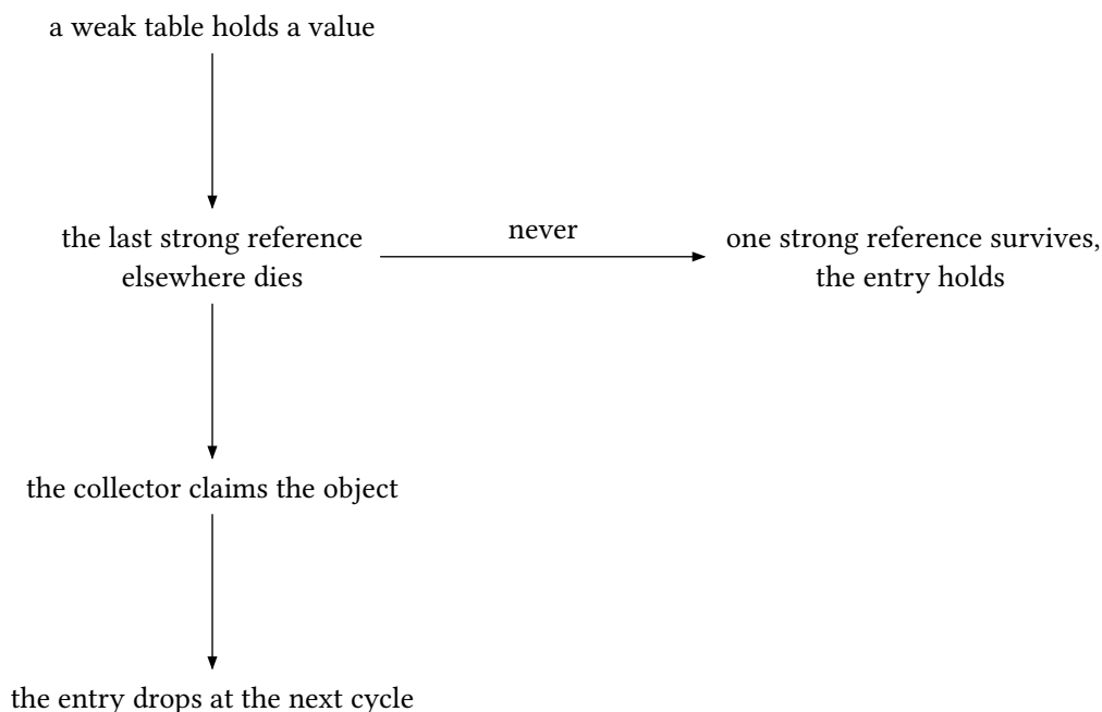
figure 43: a weak entry's life
