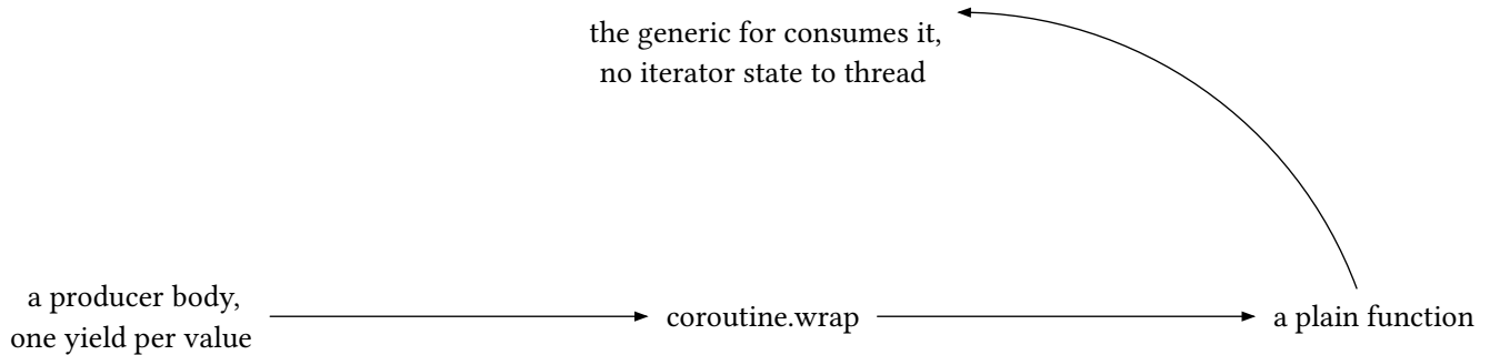
figure 31: wrap turns a producer into the function the generic for wants
