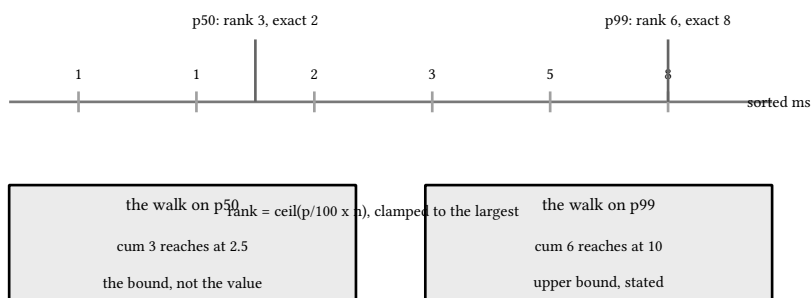
figure 161: the sorted ladder, the exact answer and the bucket's bound beside it
