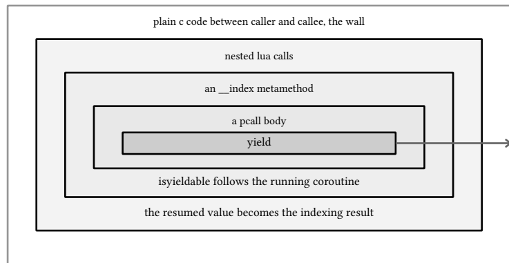
figure 32: the boundaries a yield crosses, and the one it cannot
