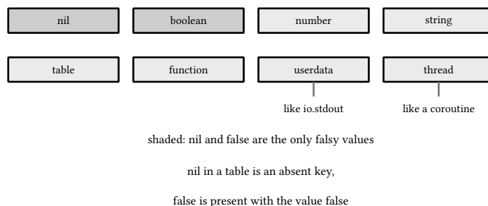
figure 9: the eight types, each reachable from plain lua, and the two falsy ones
