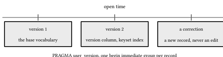
figure 131: the version ladder only grows right
