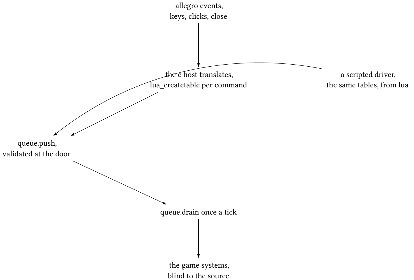
figure 92: two producers, one queue, one consumer
