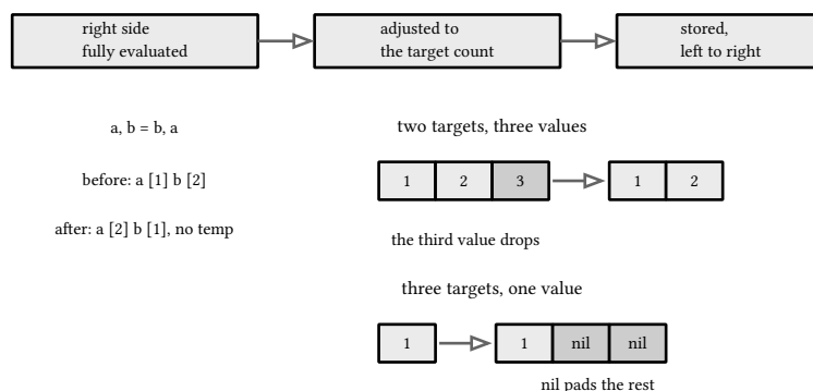
figure 20: assignment as a list operation, evaluate, adjust, then store
