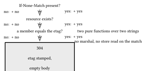
figure 137: the conditional GET decision
