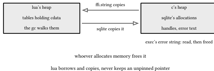
figure 85: who owns what, two heaps and the arrows between them
