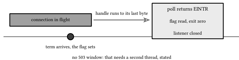
figure 170: the drain a single thread can honestly give
