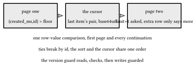
figure 134: pages chained by the same pair the sort uses
