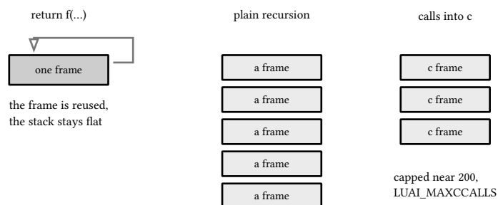
figure 28: tail calls reuse the frame, plain recursion pays a frame per level
