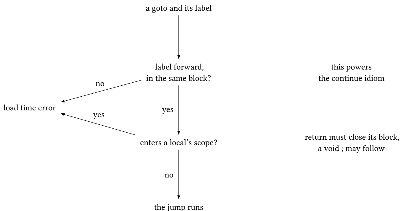
figure 23: goto validity, and return closing its block
