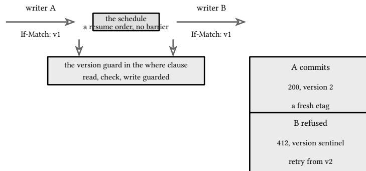
figure 136: two etags read at v1, the guard crowns one
