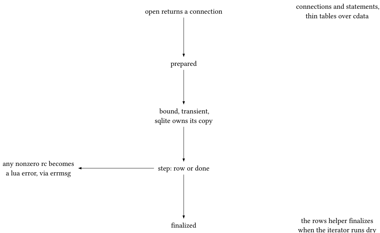
figure 84: a statement's life, prepare to finalize
