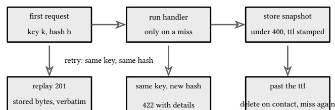
figure 138: one key's life: first run, snapshot, replay
