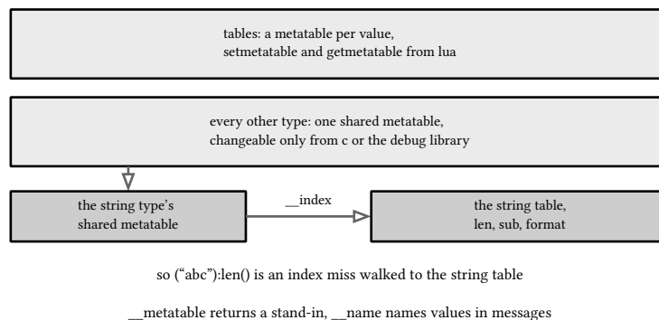
figure 12: where metatables live, per value for tables, one shared per type for the rest
