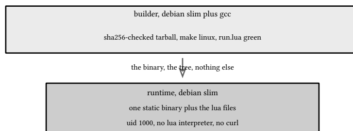
figure 171: two stages, one binary and one tree cross
