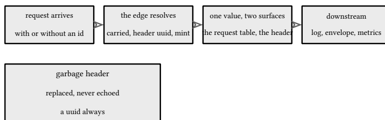
figure 103: one id, born at the edge, quoted by everything downstream
