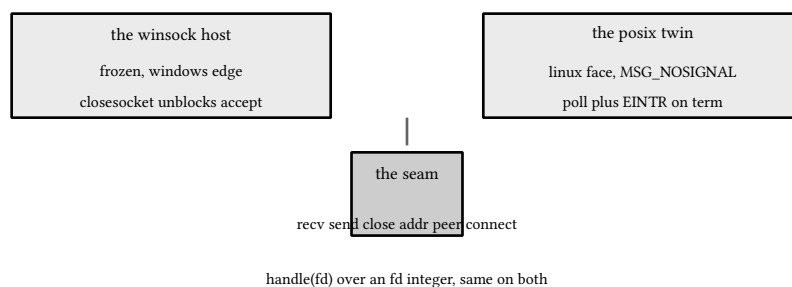
figure 166: two hosts around one seam, the service module never learns which answered
