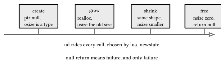
figure 42: one block's life through the hook
