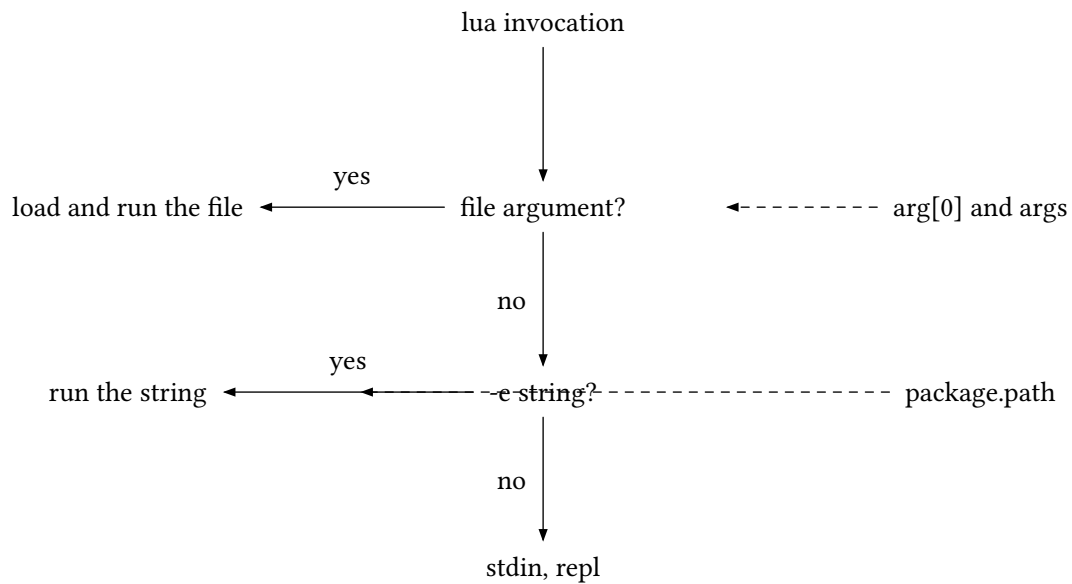
figure 3: how the standalone interpreter picks its chunk, with arg and package.path around it
