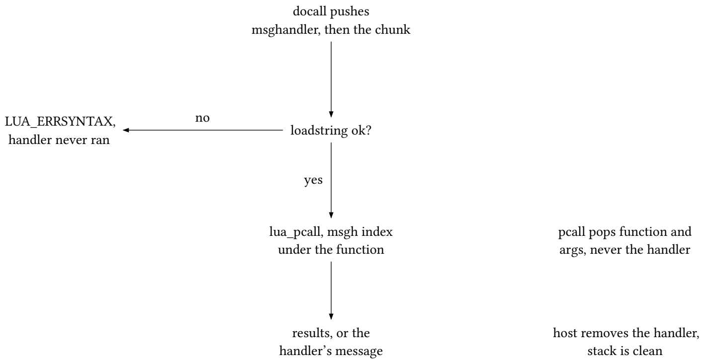
figure 67: one protected call, handler under function, results or one error
