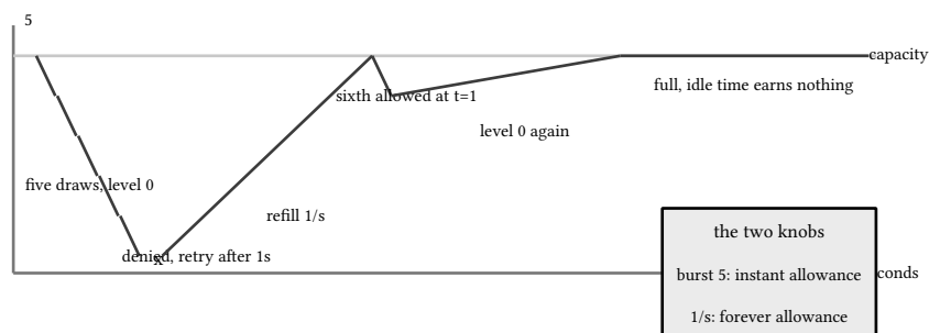
figure 148: bucket level over one draw timeline, the refill climbing between bursts
