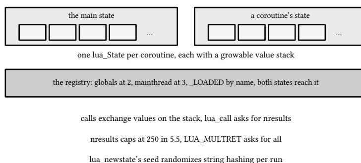
figure 71: what a host drives, states, their stacks, and the registry
