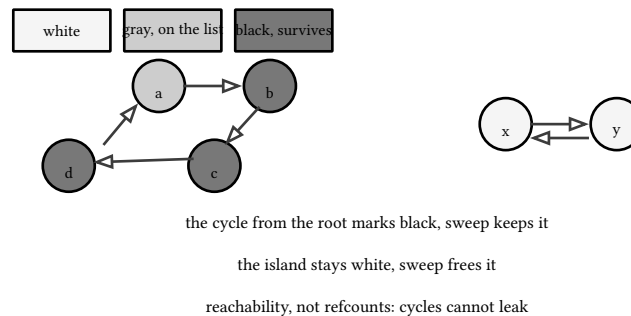
figure 39: three colors over the toy graph, one walk
