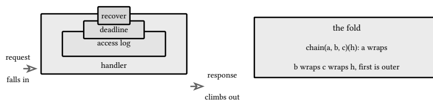
figure 102: the onion: first argument outside, request falls in, response climbs out
