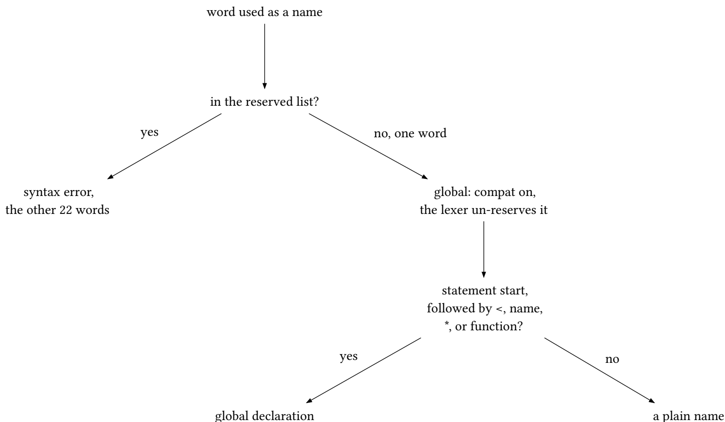
figure 5: why exactly one reserved word parses as a name, the compat un-reserving and the declaration lookahead
