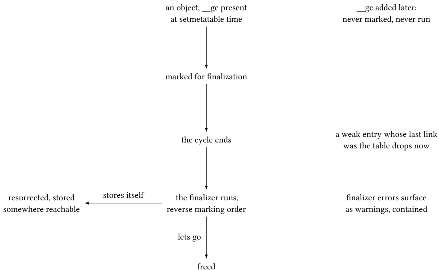
figure 36: an object with a finalizer, from marking to resurrection
