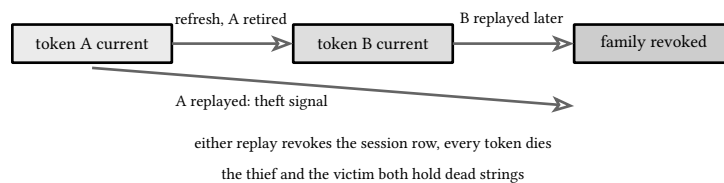
figure 122: the family: rotation forks, either replay revokes everything
