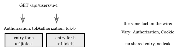
listing 210: the vary pair and the key, fixed order, values not identities (source: lua/service/cache.lua, lines 11-21)
