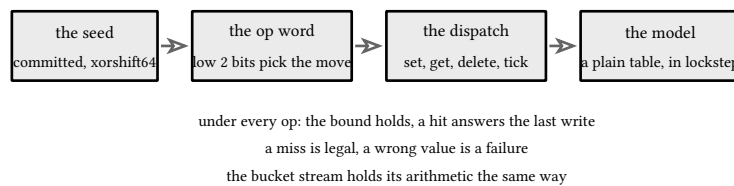
figure 180: seed to stream to model, the invariant under every step
