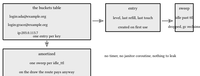
figure 149: key to bucket table, first use creates, idle age retires
