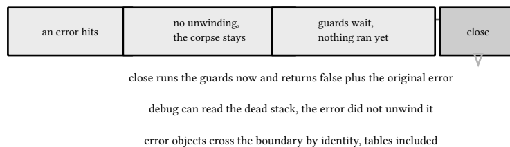
figure 29: an error kills the coroutine without unwinding, close settles it later
