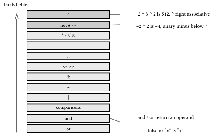
figure 15: the precedence ladder from loosest to tightest, with the two traps
