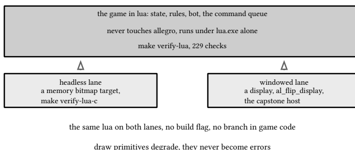
figure 93: headless by design, what a window adds and what it does not
