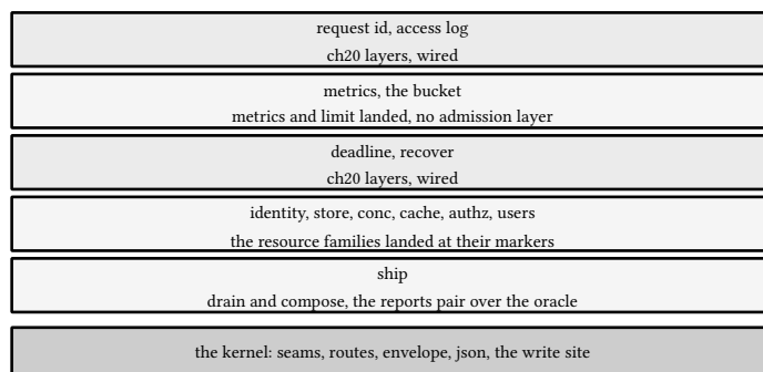
figure 100: the root as a wiring rail: the families land at their markers in request order
