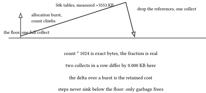
figure 37: count as an oscilloscope, the floor, the ramp, the drop
