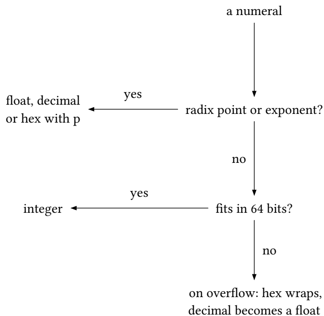
figure 8: numeral classification, what forces a float and the two overflow rules
