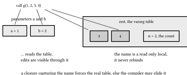
figure 26: where the extra arguments land in the 5.5 vararg model
