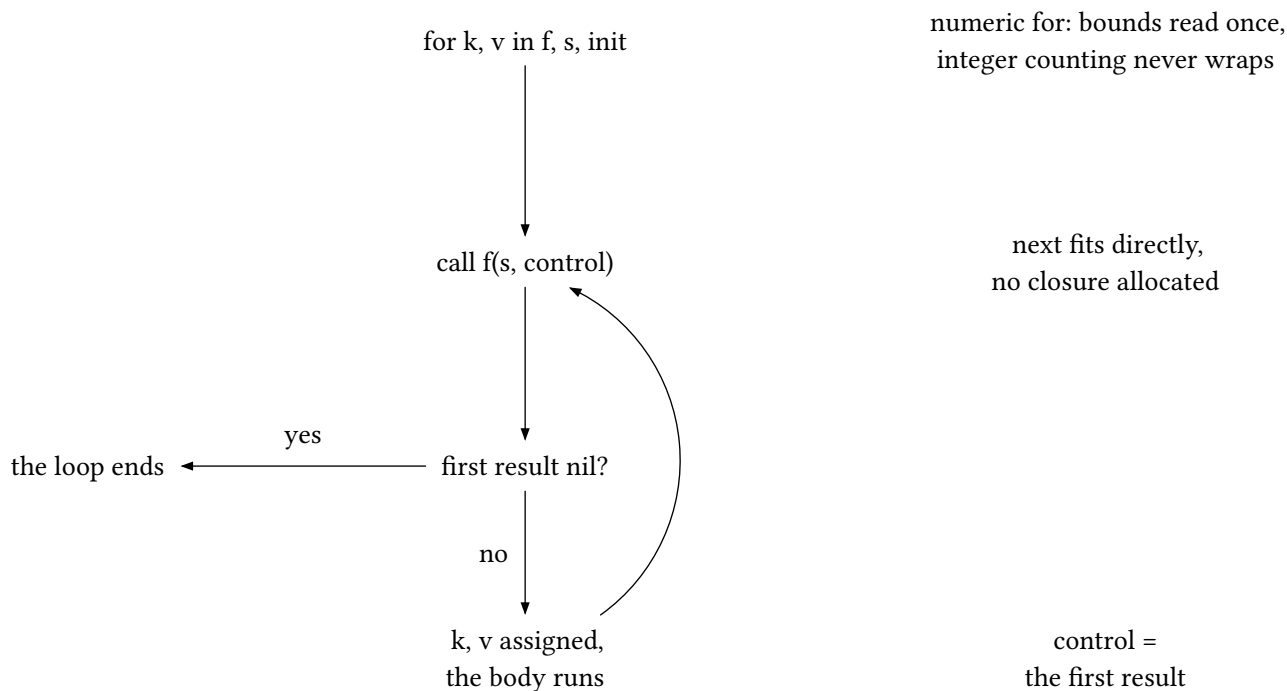
figure 22: the generic for as a call loop, the first nil terminates it
