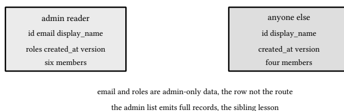
figure 114: two orders out of one record, the reader decides nothing
