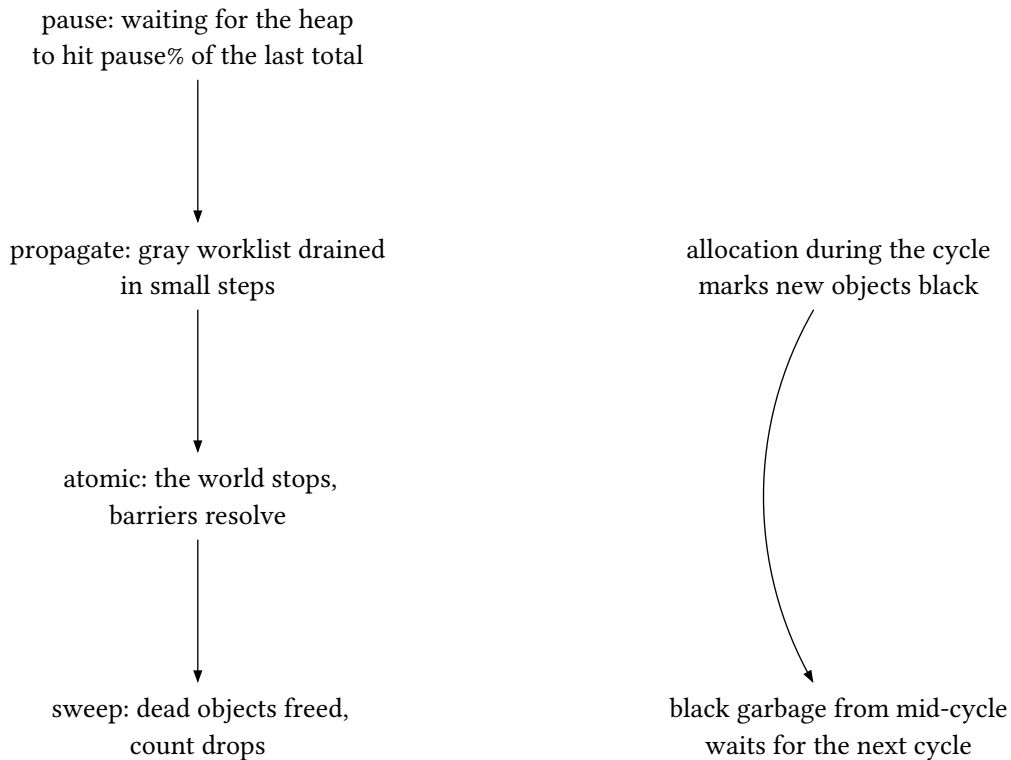
figure 38: one incremental cycle, sliced
