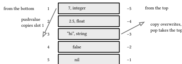
listing 118: pop, settop, pushvalue, copy (source: lua/samples-c/src/Ch14/stack.c, lines 50-64)
