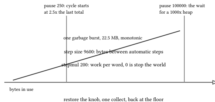
figure 40: the pause threshold against the heap
