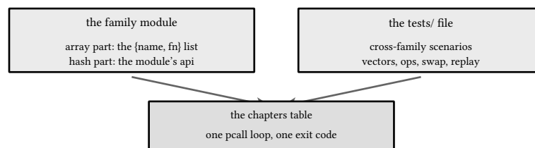
figure 177: the two shapes, one runner
