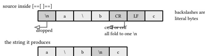
figure 7: long bracket scanning, the dropped first newline and the folded line ends
