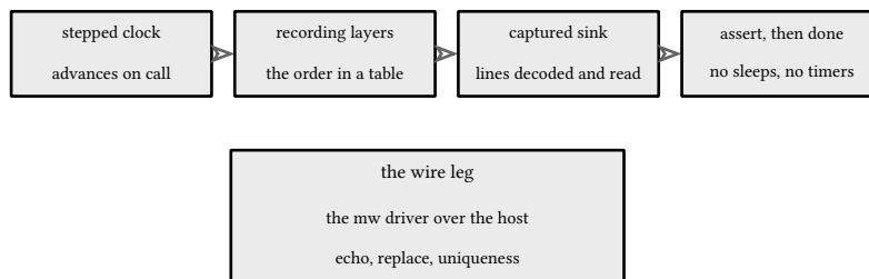
figure 108: stepped clocks, recording layers, captured sinks: the harness has no timers
