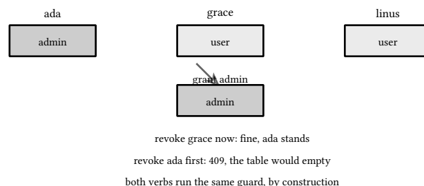
figure 127: the grant table: the admin row must never empty, both verbs checked
