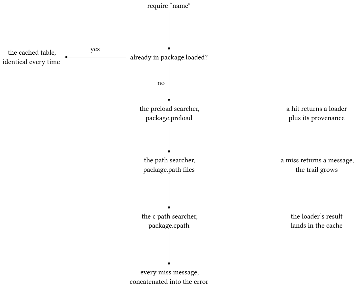
figure 62: the require pipeline, searchers in order, the cache in front
