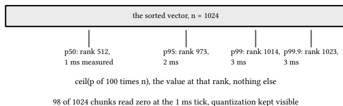
figure 49: the nearest-rank ladder over the sorted vector
