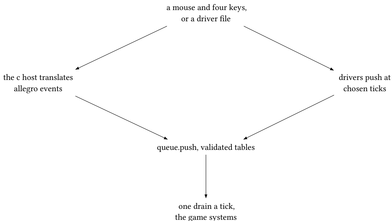
figure 183: two hands, one queue, one game
