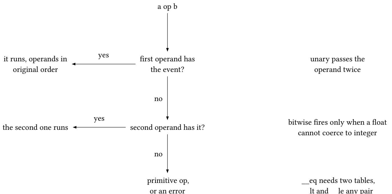
figure 13: metamethod lookup for a binary operation, the first operand's event first
