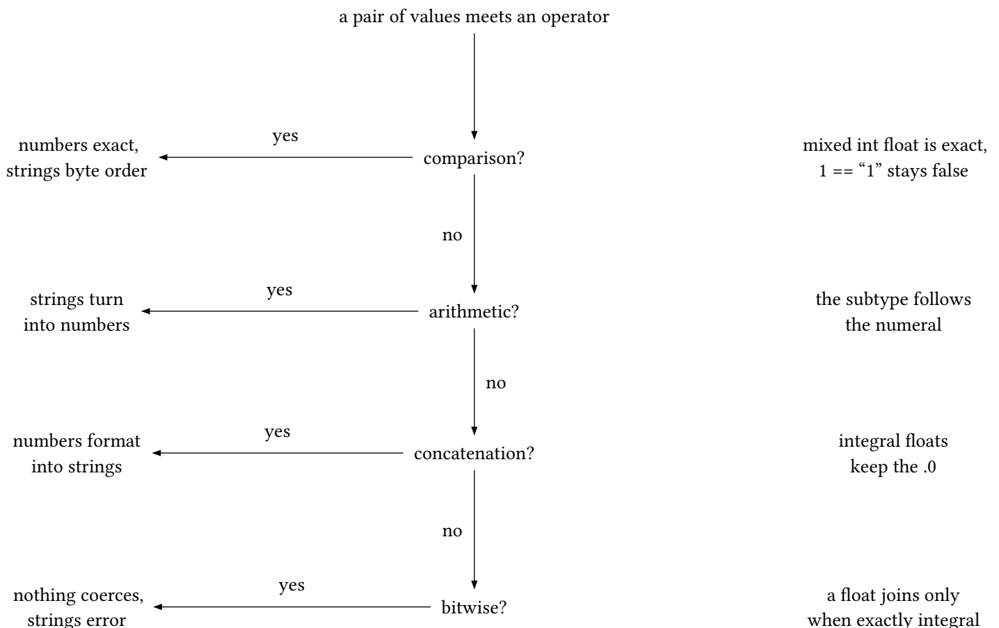
figure 18: which operators coerce which operand types, and where the boundary is
