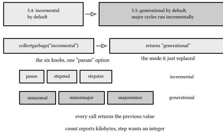
figure 35: the 5.5 collector, the default flip and where the knobs went
