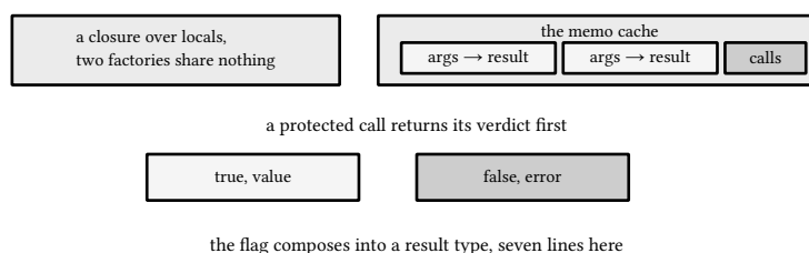
figure 80: closure state, the memo cache, and pcall as a result type
