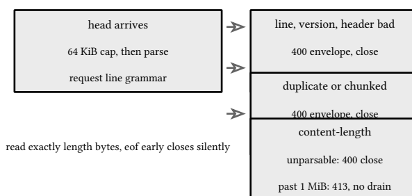
figure 95: the framing decision tree, every leaf an envelope or a closed connection
