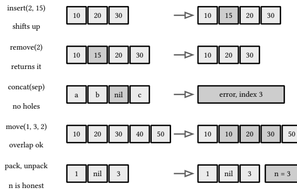
figure 57: the five table operations over the array part
