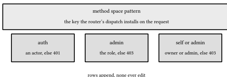
figure 125: rows as data: one key, three flags, the walk reads them in order
