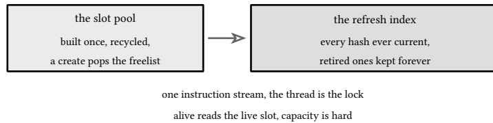
figure 119: the session pool: slots from a freelist, one refresh index, no lock
