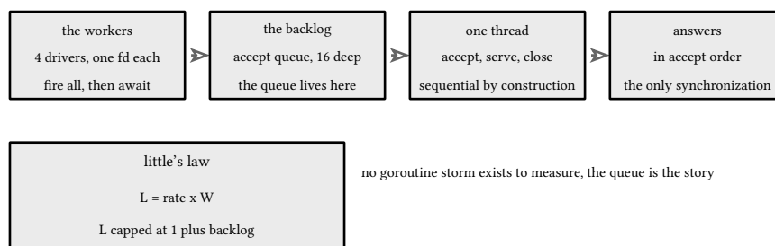
figure 160: the wire under load: workers, backlog, one server thread
