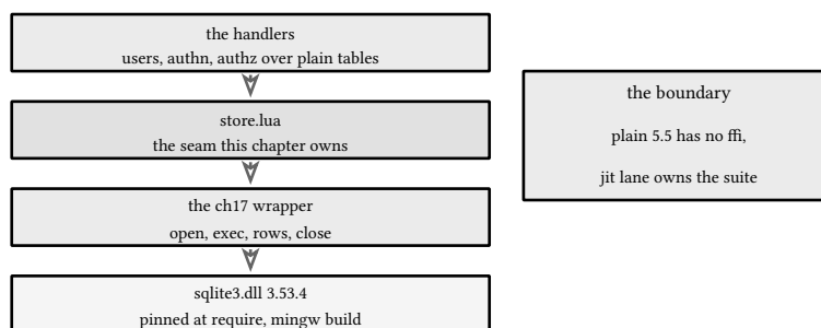
figure 130: the lane the store rides, and the one it never crosses
