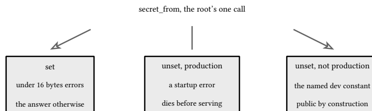
figure 169: one reader of the environment, three answers, one of them fatal
