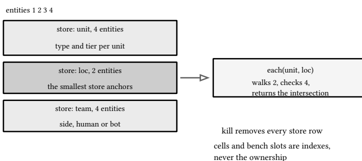
figure 184: entities, per-component stores, the anchor law
