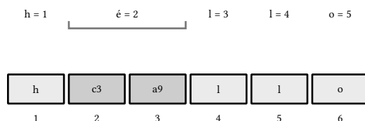
listing 96: code points, offsets, codes, invalid encoding (source: lua/samples/ch11_stdlib1.lua, lines 114-128)
