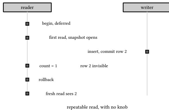
figure 17: the snapshot interleaving, two connections on one timeline
