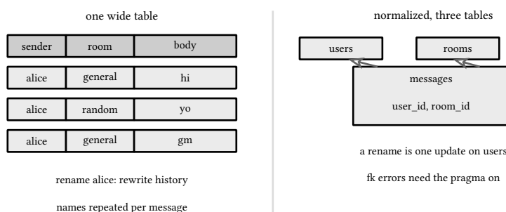
figure 15: the wide row against the normalized shape, and what a rename costs
