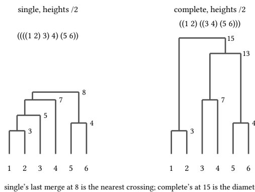
figure 130: two trees from one prefix: min chains into a caterpillar, max balances
