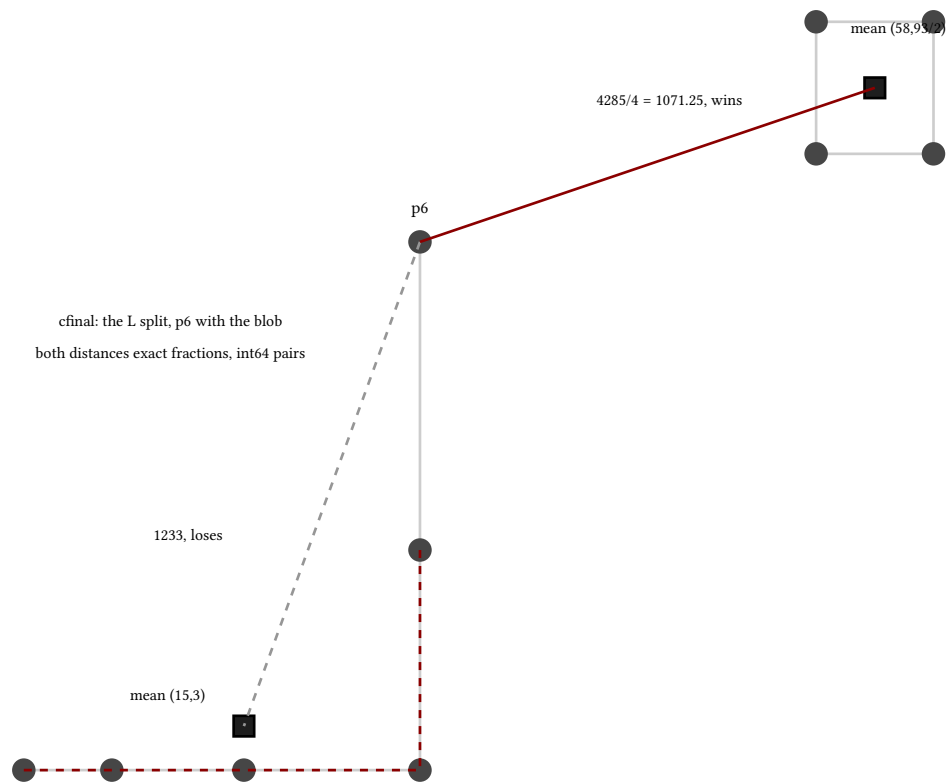
figure 141: means against an L: the blob mean stands 1071.25 from p6, the arm mean 1233
