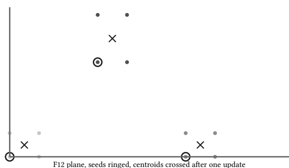
figure 193: fixture F12: three 4-point rectangles, the three seeds ringed, final centroids crossed, sse 144
