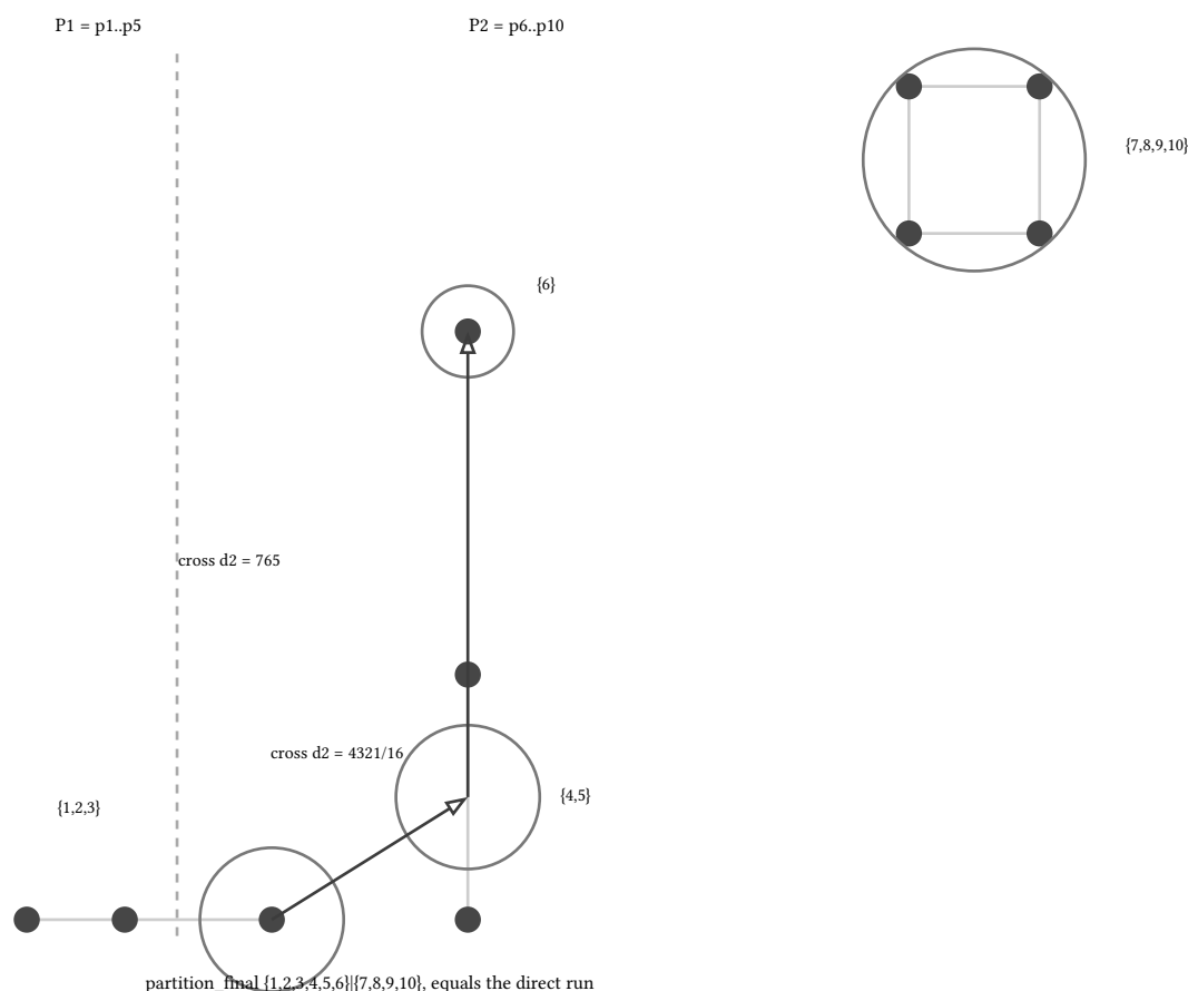
figure 143: partition, cluster each side, label across: the same final partition
