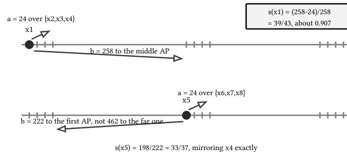
figure 138: one width, two arrows: a stays home, b visits the nearest stranger
