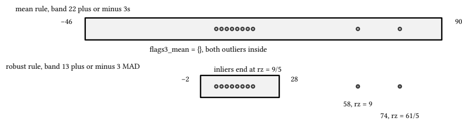
figure 152: the same ten values under the mean band and the robust band
