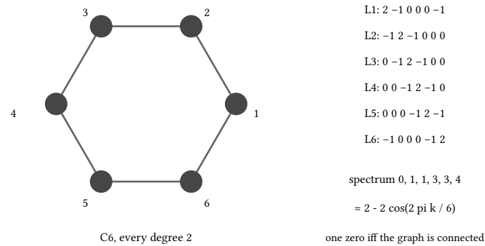
figure 145: one graph, one matrix, one spectrum: the cycle is closed form all the way down
