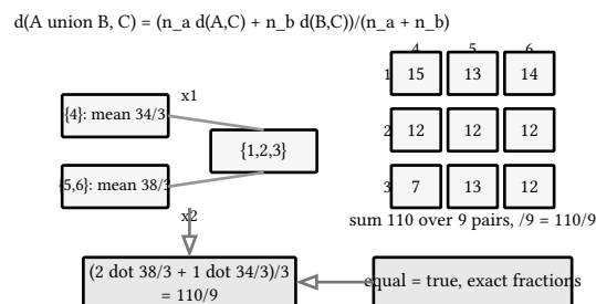
figure 132: the same fraction from two old distances or nine cross pairs
