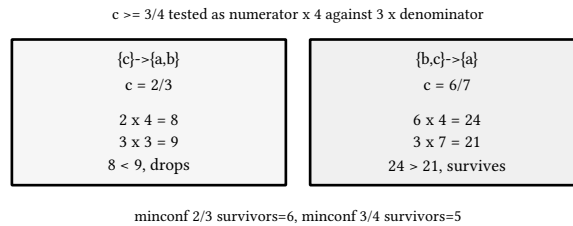
figure 112: two boundary fractions, one drops at 3/4 , one survives
