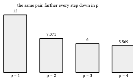
figure 18: four distances from one difference vector, shrinking in p
