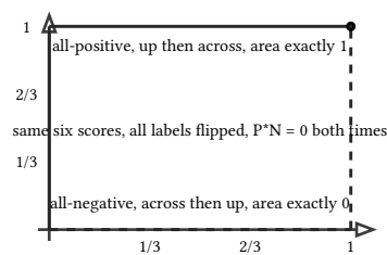
figure 74: both degenerate curves on one unit square, hugging different edges
