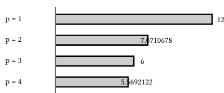
figure 191: the lp ladder on the diff triple (3,4,5), bar length is the distance, all strictly decreasing
