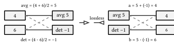
figure 39: one butterfly forward and back on the pair (4, 6)
