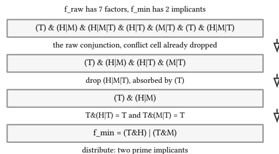
figure 174: absorption in three moves, from seven factors to two prime implicants
