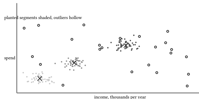
figure 197: the seed-42 corpus in the income-spend plane, every eighth inlier and all 24 outliers, crosses mark the planted centroids
