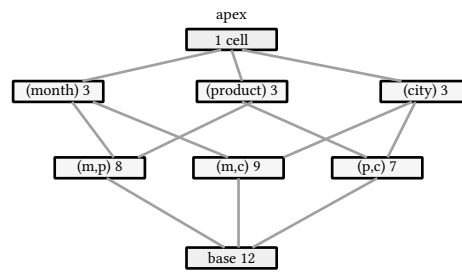
figure 43: the cube lattice, nonempty cells per cuboid, 46 of 64
