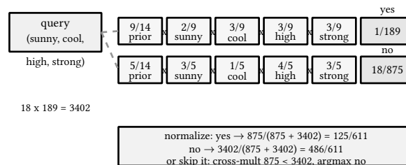
figure 75: two factor chains from one query, normalize last or not at all
