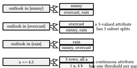
figure 58: binary encodings: three subset splits for outlook, one threshold for x
