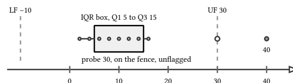
figure 151: the box and the fences, 40 outside, a probe sitting exactly on the upper fence
