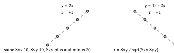
figure 25: two perfect lines, one rising, one falling, r at both endpoints
