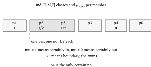
figure 167: the five classes of the full partition, each member carrying its membership grade
