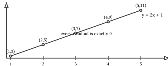
figure 46: fixture A, five points on the line y = 2x + 1 , residuals zero
