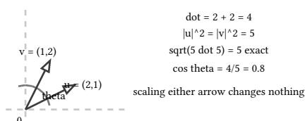
figure 23: pair 2 in the plane, equal lengths, cos of the angle 0.8
