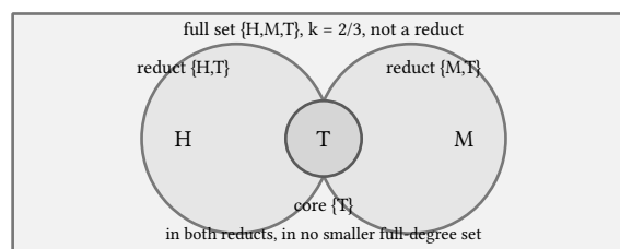
figure 171: the core is what both reducts share, the full set contains both and is too big
