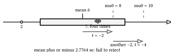
figure 159: the t fixture on the value line: one claimed mean inside the critical band, one outside
