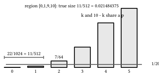
figure 158: two-sided p per k against the 1/20 budget; the region stops after k = 1
