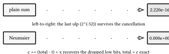
figure 146: two lanes summing the same six products: only the compensated lane hits the pinned zero
