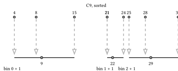
figure 12: each value pulled to its bin mean, 9, 22, 29
