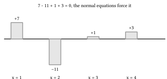
figure 48: the four fixture B residuals in tenths, positive and negative, sum zero
