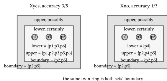
figure 166: the bracket around each decision: shaded boundary ring between lower and upper
