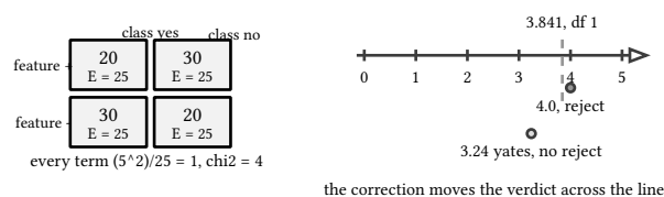
figure 32: the 2x2 table and the two verdicts against the df 1 threshold
