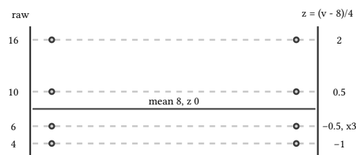
figure 15: the same six values on the raw ruler and the z ruler
