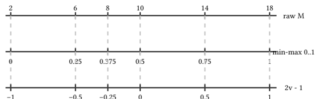
figure 14: three rulers, same spacing, the affine map at work
