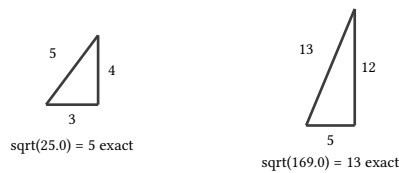
figure 19: two pythagorean pairs, both roots exact
