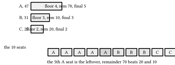
figure 28: the 10 seats: floors first, the leftover seat lands on A
