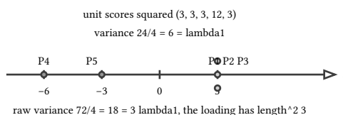
figure 37: five scores on the first component, variance 6 is the eigenvalue
