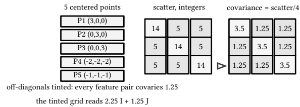
figure 34: the 5 points, their scatter, and their covariance over n minus 1
