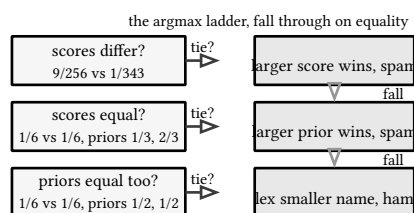
listing 146: two planted ties, one resolved at each rung (source: kdd/samples/src/Ch19/text.c, lines 112-120)
