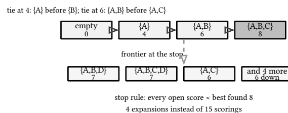
figure 31: four expansions down the spine, the frontier never tops 8
