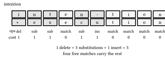
figure 24: the intention to execution alignment, five paid cells
