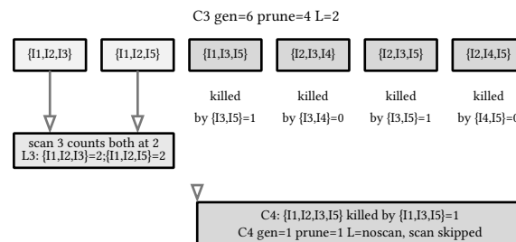
figure 102: six joins, four killed by their pairs, two counted at exactly the bar
