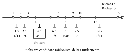
figure 57: the 8-row axis, 7 midpoint candidates, 4.5 wins with 3/10
