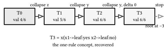
figure 64: the pruning rounds, validation climbing 4, 5, 6, 6 of 6, then stop
