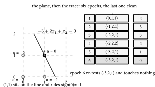
figure 84: AND in the plane, the boundary through (1,1), the epoch trace at right
