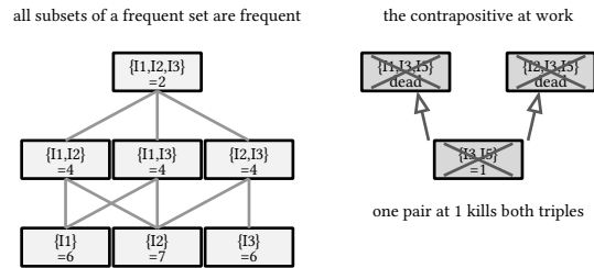
figure 101: support falls or holds moving up, one infrequent pair executes its whole upper cone
