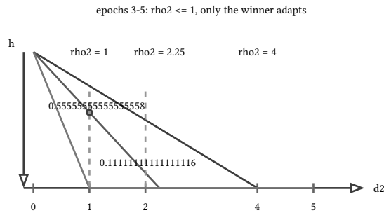
figure 178: the kernel over grid distance, five shrinking epochs, bubble by epoch 3
