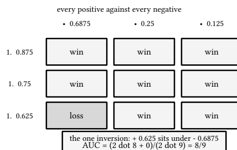
figure 72: the 3x3 pair grid, eight wins and the one inversion
