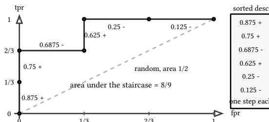
figure 71: the seven-point staircase on the unit square, each step named by the score that caused it
