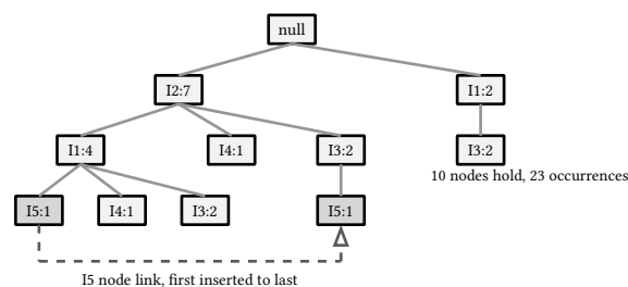
figure 114: the fp-tree, solid edges share prefixes, the dashed chain is the I5 node link
