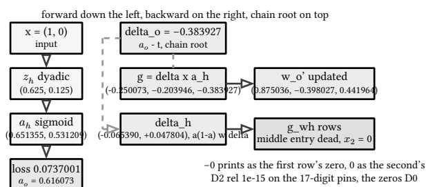
figure 88: one example down the net, backward chain root on top, dead column boxed
