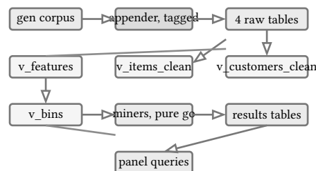
figure 198: the data path, wide boxes are tables and views, the appender is the only writer
