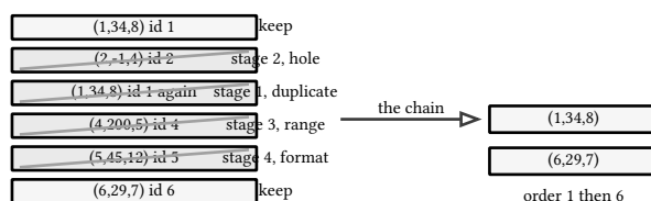
figure 3: the six input rows, four struck out, two survivors
