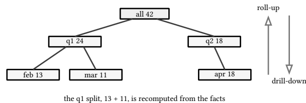
figure 44: the time hierarchy, roll-up aggregates up, drill-down refines down
