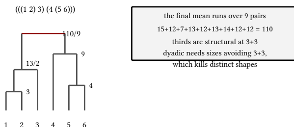
figure 131: average keeps every distance in play and pays in thirds
