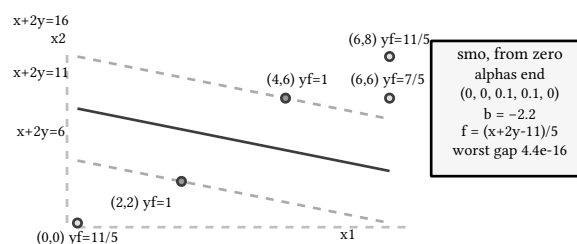
figure 92: the 5-point fixture and the plane SMO finds, supports at (4,6) and (2,2)
