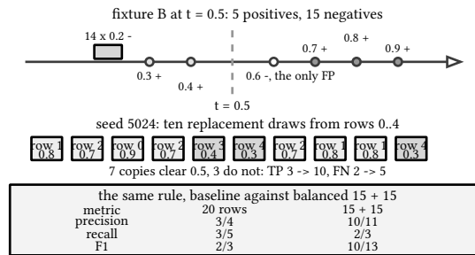
figure 99: fixture B on the score line, then ten drawn copies of the minority
