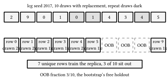
figure 70: ten draws over ten row slots, 7 unique, rows 6, 7, 8 never drawn
