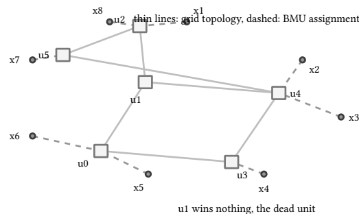
figure 181: the final map in data space, dashed lines tie each input to its winner
