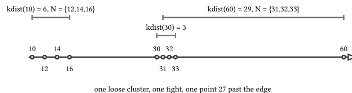
figure 153: nine points, three neighborhoods: loose, tight, and stranded
