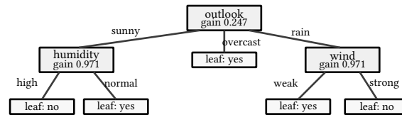
figure 53: the learned tree, five leaves, depth 2, gains at each split
