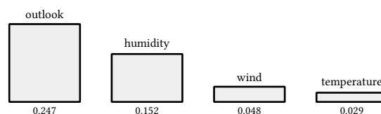
figure 52: the four root gains, outlook wins, temperature never helped
