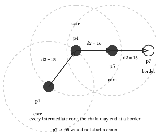
figure 135: three hops, every intermediate core, ending at a border
