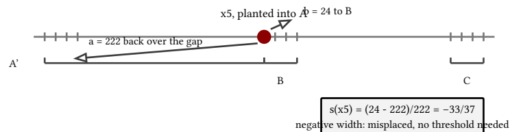
figure 140: one point dragged across the 204 gap: a explodes, b collapses, s goes negative
