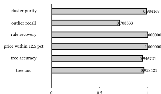
figure 199: the six recovery numbers of the canonical run, bar length is the value, one is perfect
