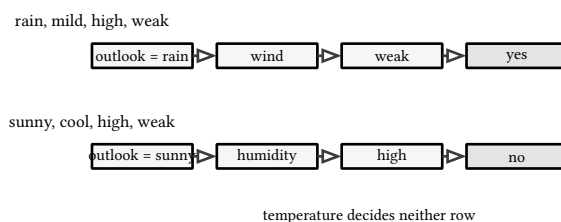
figure 54: two held-out rows walked through the tree, two different paths
