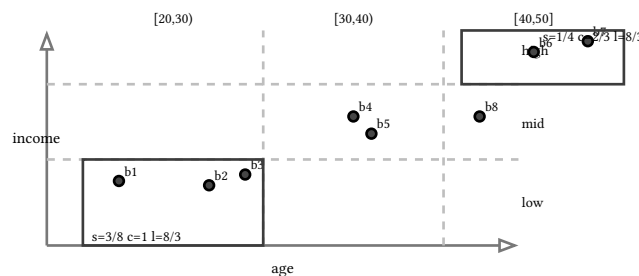
figure 120: age against income, the bin grid, and where the two rules live
