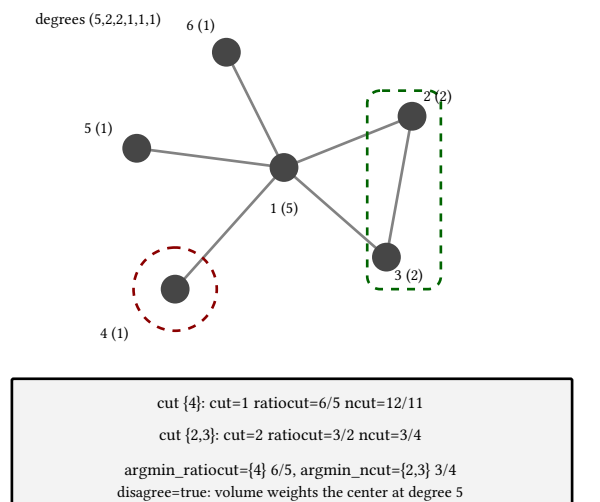
figure 148: on the star, ratiocut isolates a pendant, ncut cuts the light rim pair
