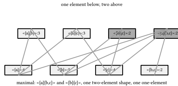
figure 123: the eight frequent sequences, containment edges up, maximal dark
