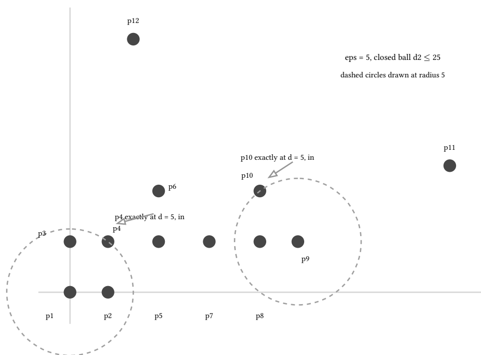
figure 133: the fixture: two boundary pairs sit exactly on the closed eps ball
