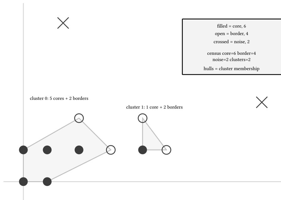
figure 134: the census on the plane: 6 cores, 4 borders, 2 noise, 2 clusters
