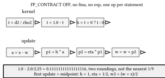
figure 180: two statement chains, each box one correctly-rounded operation
