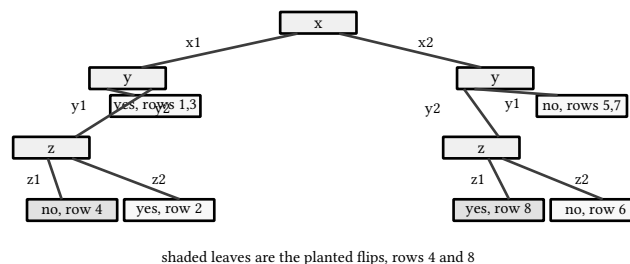
figure 63: T0, six leaves, the two z levels exist only to fit the flips
