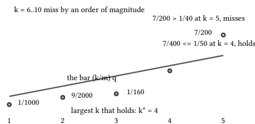
figure 163: sorted p against the rising (k/m) q bar: the pace holds through k = 4 , breaks at k = 5
