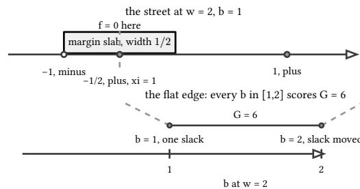
figure 90: the soft-margin fixture on a line, and the flat edge of its optimum
