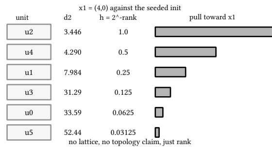
figure 187: x1's six units on the distance ladder, strength halving with rank
