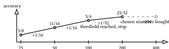
figure 29: the accuracy staircase, the third gain hits the threshold and 400 is never bought
