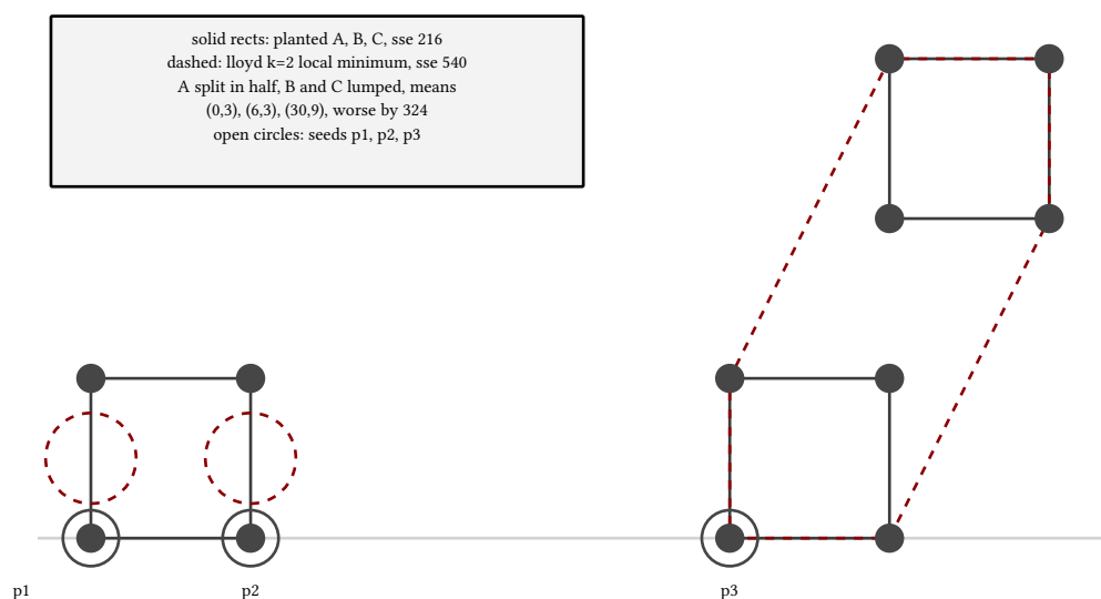
figure 127: the same 12 shapes, two answers: planted rectangles against lloyd's hulls
