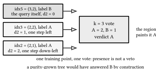
figure 83: the self at d_2 = 0 contributes one vote and loses
