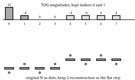
figure 40: the noisy magnitudes, two kept, and the flat step that comes back
