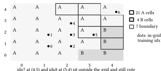
figure 82: the decision region at k = 3, training points marked, boundary cells outlined
