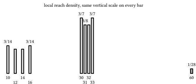
figure 154: the density landscape: lrd per point, tight cluster high, straggler near zero
