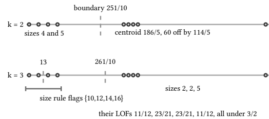
figure 156: two fixed-point partitions; the size rule flags what LOF forgives
