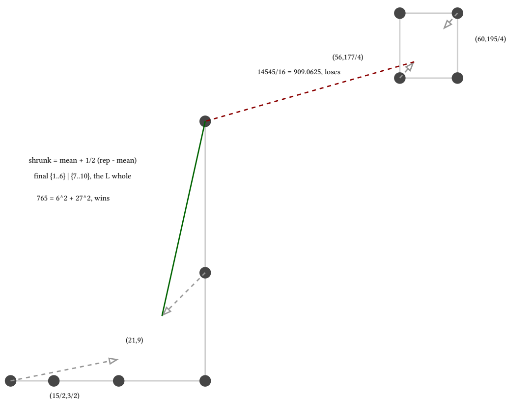
figure 142: shrunk reps: the arm keeps an extreme near p6, the blob pulls its corners in
