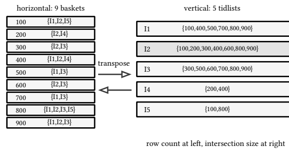
figure 105: the same nine baskets read row-wise and column-wise
