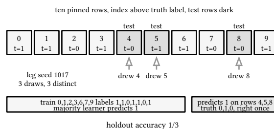
figure 68: ten rows split by three pinned draws, the majority learner scores 1 of 3
