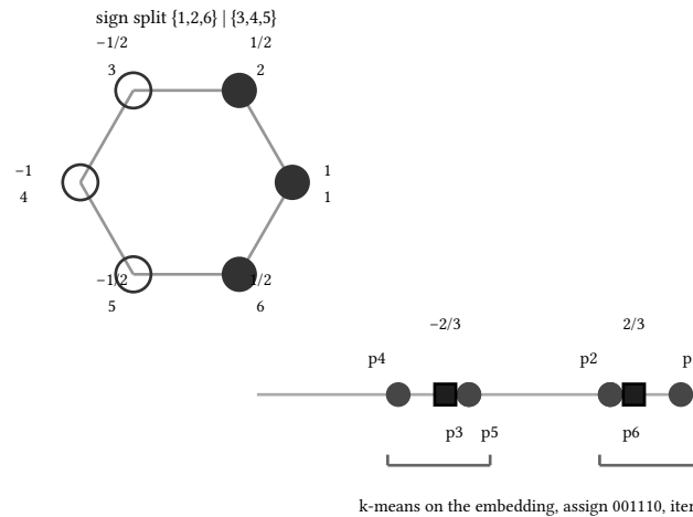
figure 147: signs on the ring, values on the line, k-means reproducing the split
