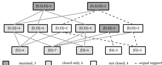
figure 109: the 13-itemset lattice, dashed edges where support holds instead of falling
