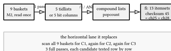
figure 108: one pass builds the columns, every later count is pure set work
