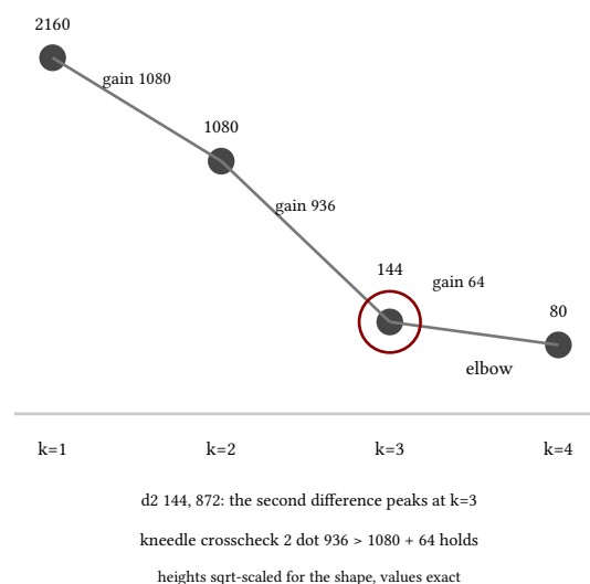
figure 126: the optimal sse curve and the elbow at the largest second difference
