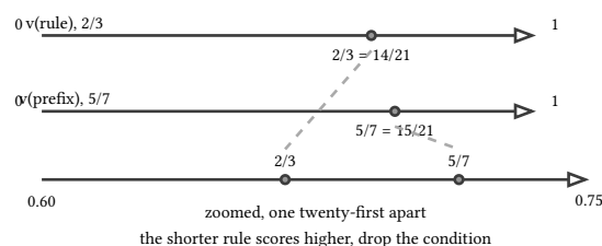
figure 61: two estimates of correctness, 2/3 against 5/7, zoomed at the bottom
