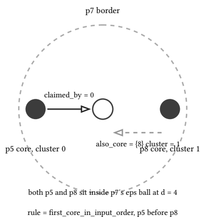
figure 136: one border, two legal claims, one pinned rule
