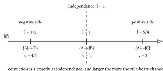
figure 117: lift against the independence line, conviction underneath
