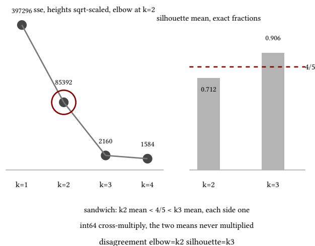
figure 139: the elbow stops at k=2, the silhouette mean climbs to k=3
