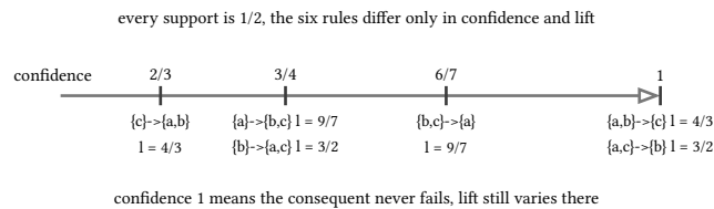
figure 111: the six confidences with their lifts, certainty at the right
