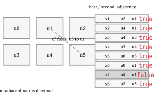
figure 182: the 2x3 lattice with each input's two best units, the diagonal pair highlighted
