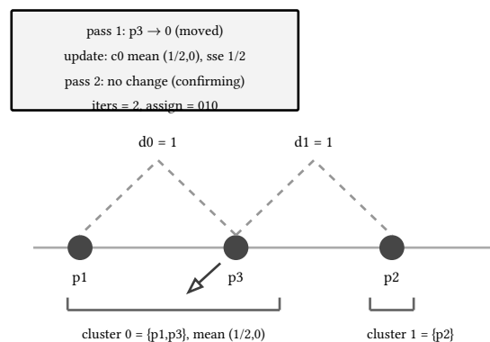
figure 128: one tie, one rule: the lowest cluster index wins
