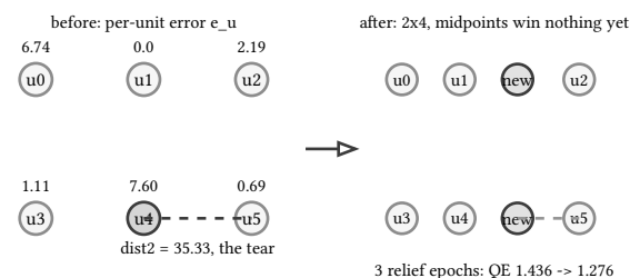
figure 186: 2x3 to 2x4: the new column between the worst unit and its farthest neighbor
