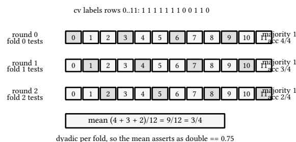
figure 69: three rounds, each fold tests once, mean 9/12 = 3/4
