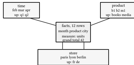
figure 42: the star: one fact table, three dimensions, three hierarchies
