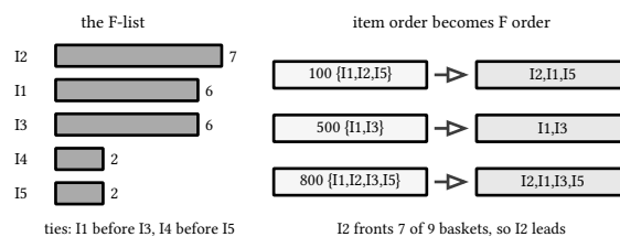
figure 113: rank by count, then write transactions so shared items come first
