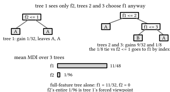
figure 96: three trees on drawn feature subsets, and what importance measures
