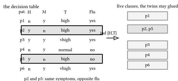
figure 165: the flu table and the partition its best pair of attributes induces
