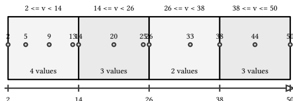
figure 10: S_{12} in four equal-width shelves, width 12 over 2 to 50
