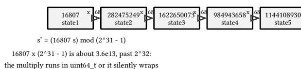
figure 26: the state chain from seed 1, one multiply and one mod per hop
