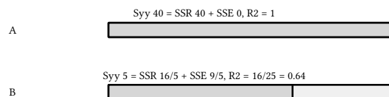
figure 49: variance explained, fixture A fills the bar, fixture B fills 16 of 25
