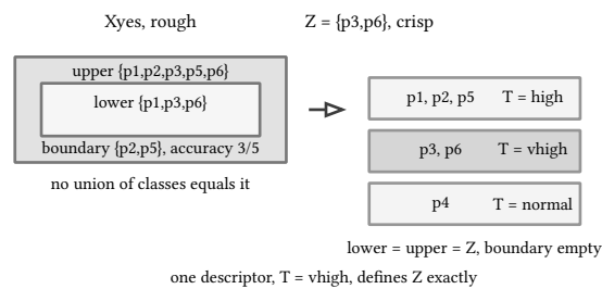
figure 168: Xyes needs a bracket, Z is exactly one class of \text{ind}\{T\}
