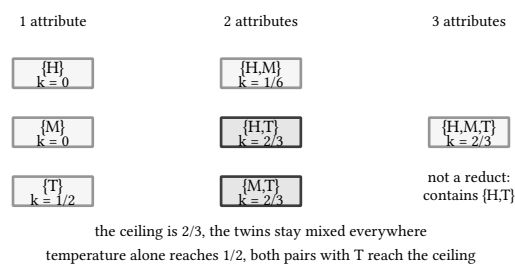
figure 169: all 7 nonempty subsets by size, degree k under each, reducts boxed
