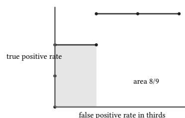
figure 192: the seven pinned corners in thirds, the staircase from (0,0) to (1,1), concordant area 8/9
