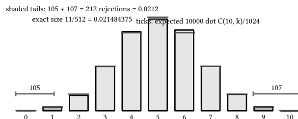
figure 160: 10000 simulated trials: counts against expected ticks, rejection tails shaded
