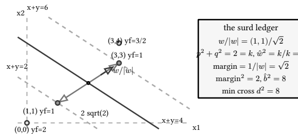
figure 89: the hard-margin street: supports at y_f = 1 , margin \sqrt{2} per side
