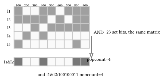
figure 107: the vertical matrix as bits, AND intersects, popcount supports
