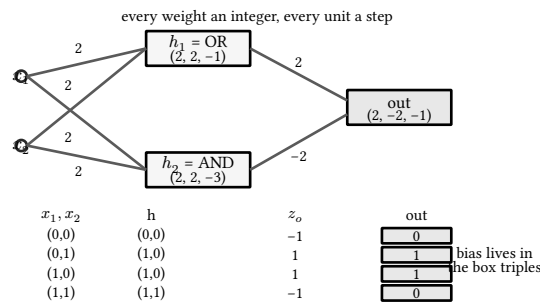
figure 86: the 2-2-1 wiring with weights on the edges, truth table beneath
