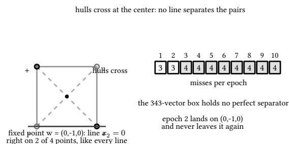
figure 85: the XOR square, crossing hulls, and the fixed-point line along the bottom
