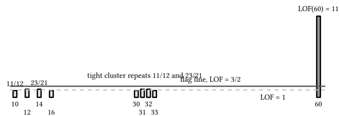
figure 155: nine LOF values against the 3/2 flag line, one bar above it
