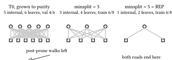
figure 66: three sizes of tree, pre-pruning and post-pruning meet in the middle
