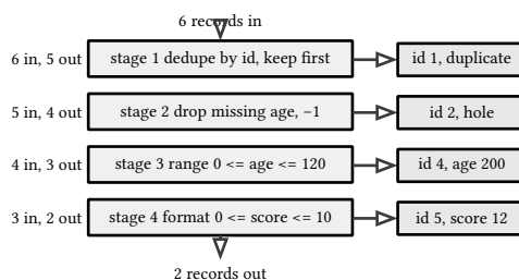
figure 2: six records through four filters, one drop per stage
