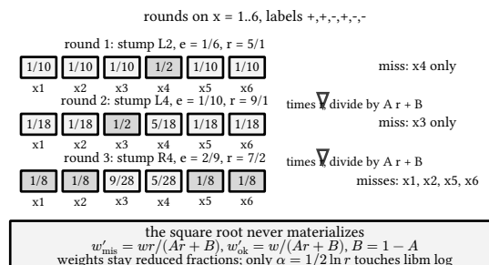
figure 94: weights after each round as exact fractions, misses shaded
