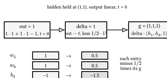
figure 87: the one step as a pipeline, the three weights before and after
