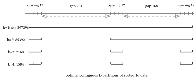
figure 137: the line, its gaps, and the optimal partitions the dp prices
