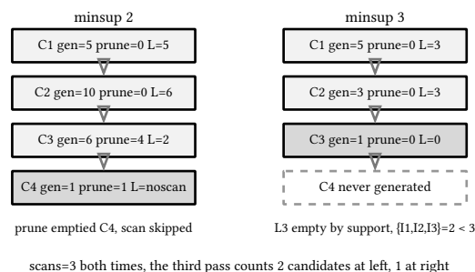
figure 103: both runs take three scans and stop for different reasons
