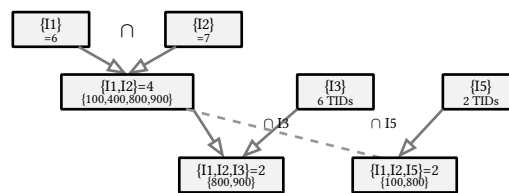
figure 106: compound supports by intersection alone, no basket read again
