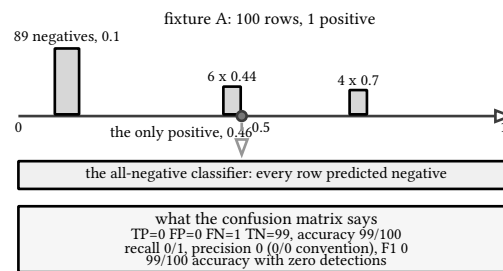
figure 97: fixture A's score landscape, and the classifier that ignores it
