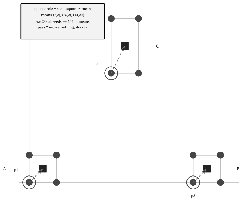
figure 125: assignment then means: three seeds, one update, integer centroids
