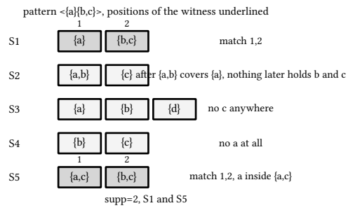
figure 124: five sequences, two witnesses, three different reasons to refuse
