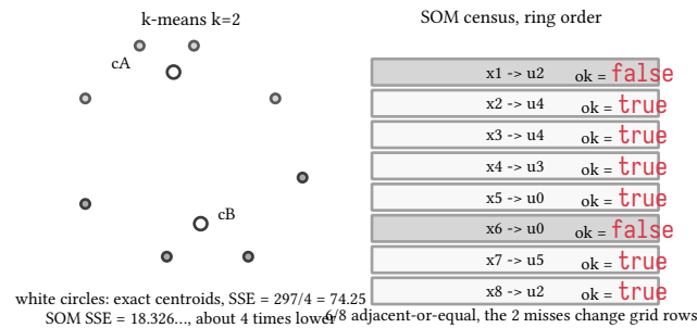
figure 184: k-means splits the ring in two, the SOM walks it around the lattice
