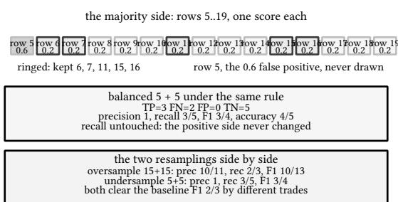
figure 100: the 15 majority rows, 5 kept by rejection, and the two resamplings compared
