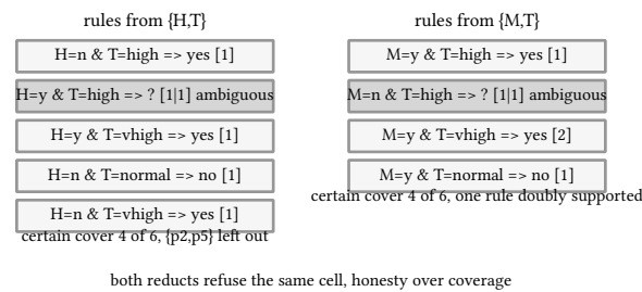
figure 176: two rule sets, one shared hole: the twins classify under neither
