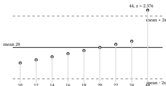
figure 8: the series against the mean and the 2-sigma band, only 44 escapes
