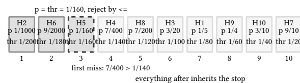
figure 162: holm's walk over sorted list P: three rejects, an exact boundary, one stop
