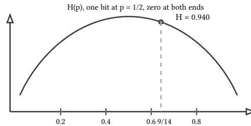
figure 50: the binary entropy curve, the root's 9 of 14 sits near the peak
