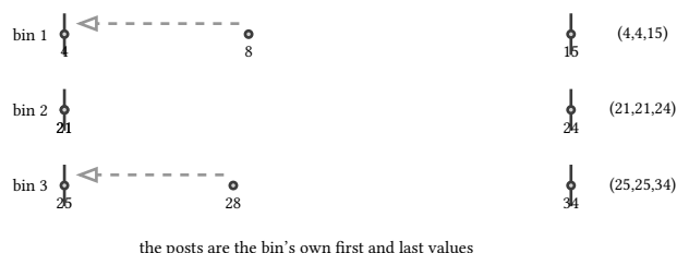
figure 13: each bin's values snap to the nearer of its two boundary posts
