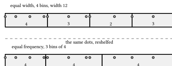
figure 11: the same 12 values cut by width into 4 and by depth into 3
