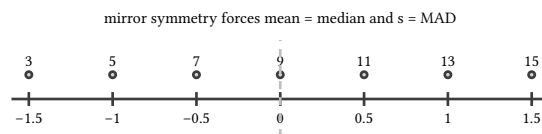
figure 17: the symmetric ladder, raw values above, z values below
