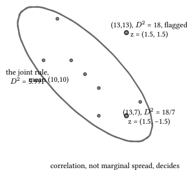
figure 150: the tilted joint rule: both probes are marginally quiet, only one is outside
