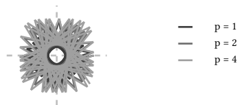
same center, same radius 1, three geometries
