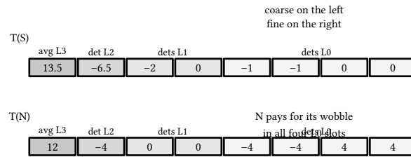
figure 38: the 8 coefficients of each signal shelved by scale
