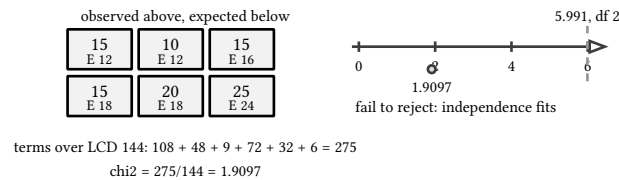
figure 33: observed against expected in six cells, the statistic far under the df 2 line
