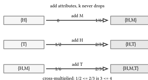
figure 172: k is nondecreasing up every edge, three witnessed climbs
