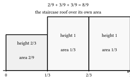
figure 73: the three nonzero trapezoids, 2/9 + 1/3 + 1/3 = 8/9
