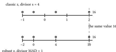
figure 16: value 16 measured on the classic ruler and the robust ruler
