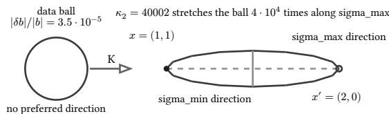
figure 141: the input ball mapped through the matrix to a kappa-stretched ellipse, the flip as one endpoint
