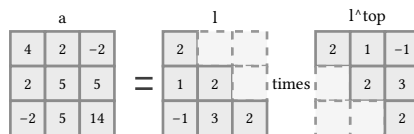
figure 46: cholesky splits a into two triangular shadows of itself
