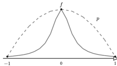
figure 125: the runge bump on three nodes and its exact parabola, agreeing at the nodes and nowhere else
