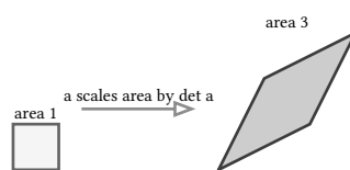
figure 44: unit square and its image, area scales by \det a = 3
