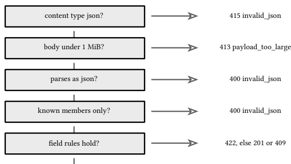
figure 116: the decode ladder: each rung rejects a class of bad input
