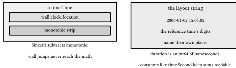
figure 66: two clocks in one value: wall for people, monotonic for math
