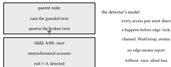
figure 151: the canary's two verdicts, one mechanism
