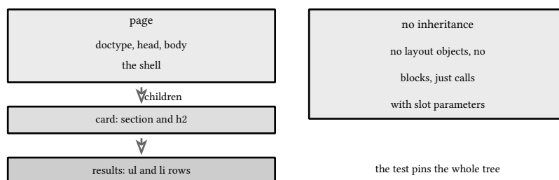
figure 96: composition is call structure: page around card around results
