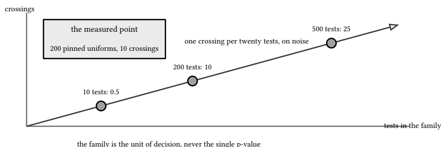
figure 195: expected false positives against family size at the 0.05 bar, with the measured null family
