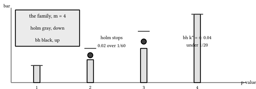
figure 202: the contrast family under both bar ladders: step-down stops early, step-up clears all four
