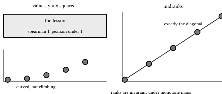
figure 200: values versus ranks: a nonlinear monotone pair flattens to the diagonal
