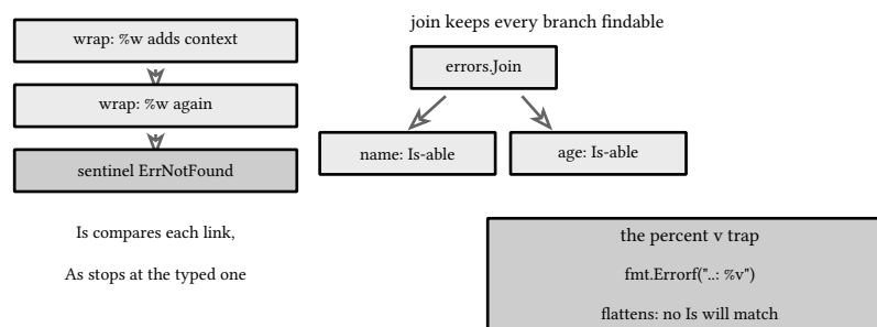
figure 34: the wrap chain and the join tree, walked by Is and As
