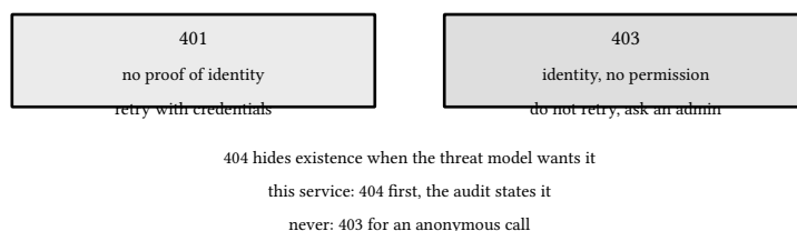
figure 133: the two failure codes, and the one deliberate blur
