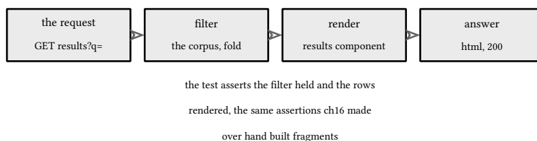
figure 98: the swap consumes a component render, same bytes as ch16
