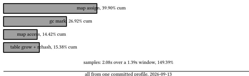
figure 229: where build's cpu goes, one profile, four buckets
