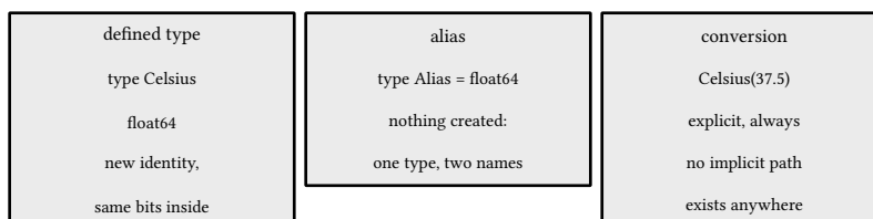
figure 15: three relations: defined type, alias, explicit conversion
