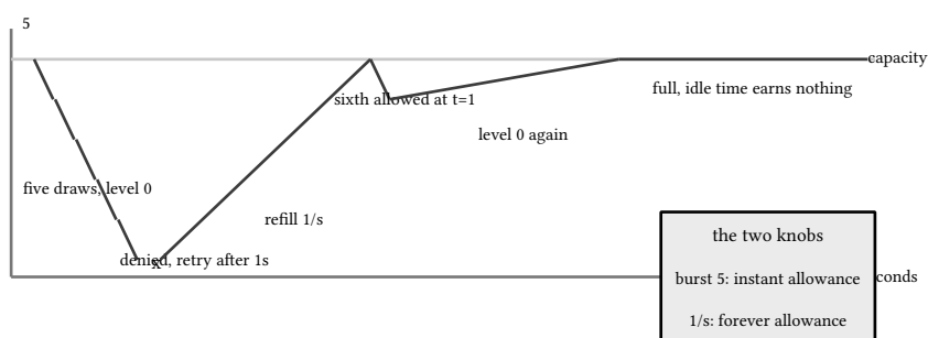
figure 160: bucket level over one draw timeline, the refill climbing between bursts
