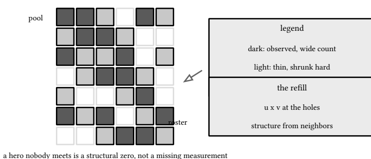
figure 206: the pool-by-roster grid: observed cells, thin cells, and holes refilled by low-rank structure
