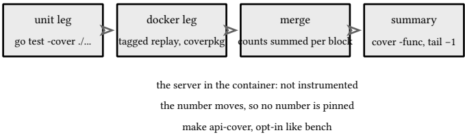
figure 193: two legs, two profiles, one merged summary
