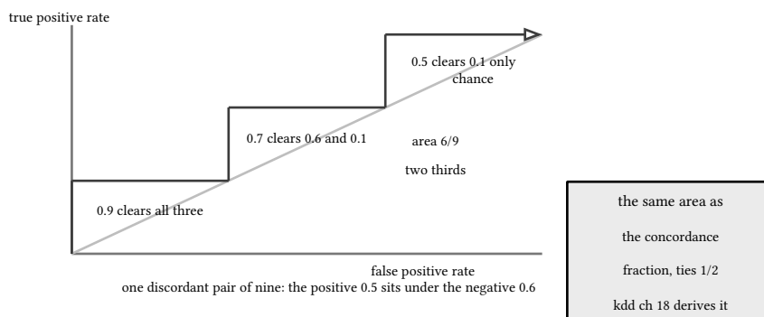
figure 199: the fixture's roc curve: a step per threshold, area 2/3 over the chance diagonal
