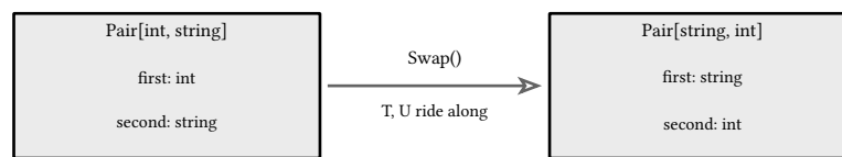
figure 18: the receiver's parameters ride along: swap with no explicit instantiation
