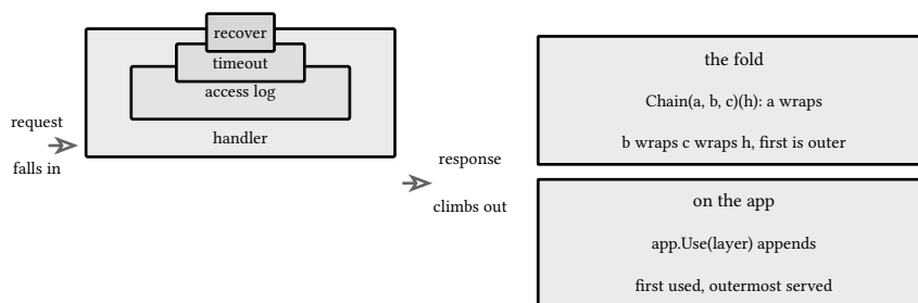
figure 108: the onion: first argument outermost, request in, response out
