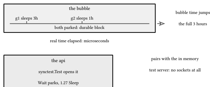
figure 78: the synctest bubble: fake time advances only when everyone is parked
