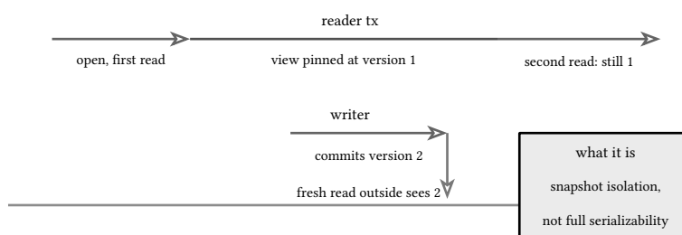
figure 141: one timeline: the reader's view holds
