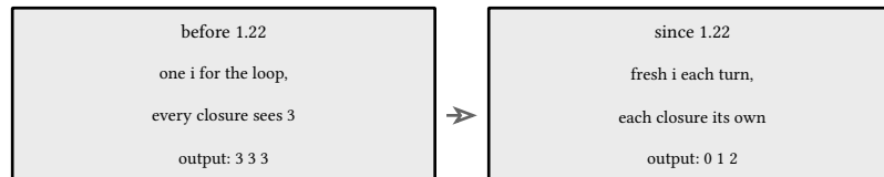
listing 27: per iteration capture, 0 1 2 since go 1.22 (source: go/samples/ch05/functions.go, lines 54-60)
