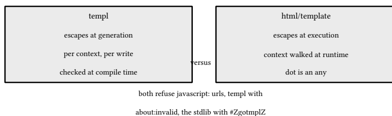
figure 97: same contract, different sentinels, different checking time
