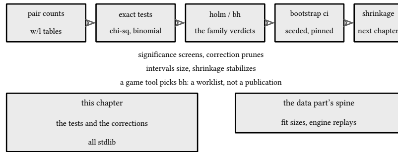
figure 203: the screening chain: each stage's output is the next stage's contract
