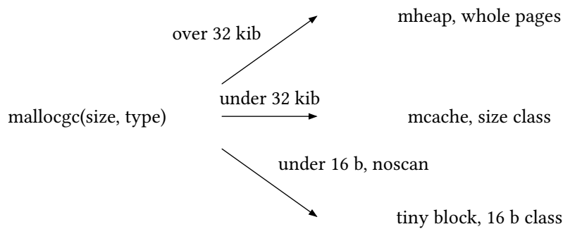
figure 47: every request sorted at the door, three doors out
