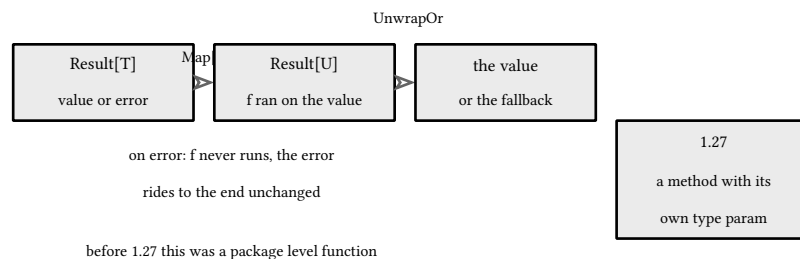
figure 224: result chains with the error riding along, map short circuits
