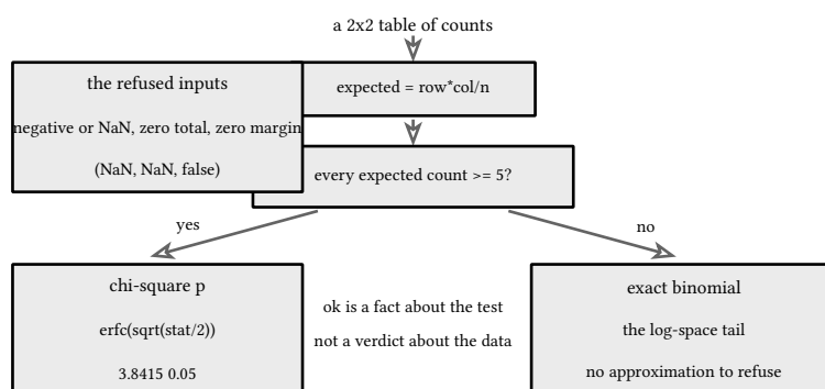
figure 197: the fallback decision: the gate on expected counts routes the table to the approximation or the exact tail
