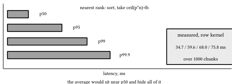
figure 61: the tail ladder over 1000 chunks
