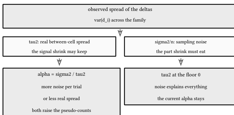
figure 205: the variance decomposition: observed spread splits into real signal and sampling noise
