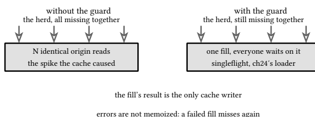
figure 156: the same expiry, with and without the guard
