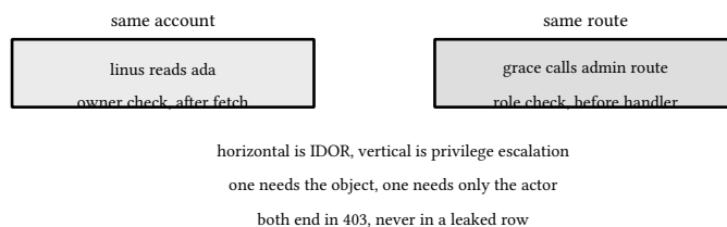
figure 134: horizontal versus vertical: two axes of privilege, two different checks
