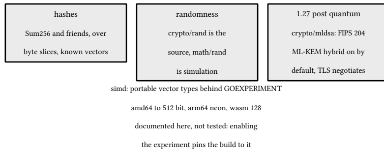
figure 72: the crypto and simd corner of the tour
