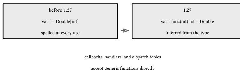
figure 20: function type inference, generalized in 1.27
