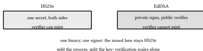
figure 127: shared secret versus split key: who can mint, who can check
