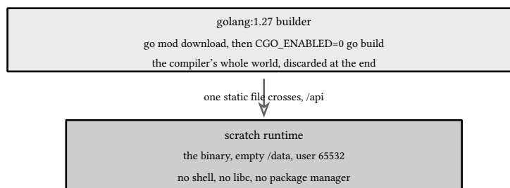
figure 180: two stages, one file crosses: the builder dies with the build, scratch runs the binary
