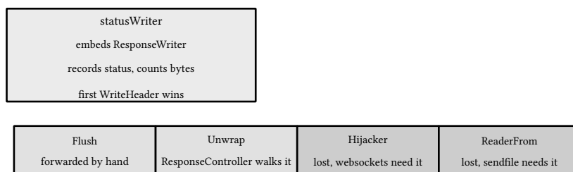
listing 133: the status-capturing writer: first status wins, bytes counted (source: go/api/internal/middleware/accesslog.go , lines 38-58)
