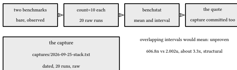
figure 175: the bench flow: code, capture, statistics, quote
