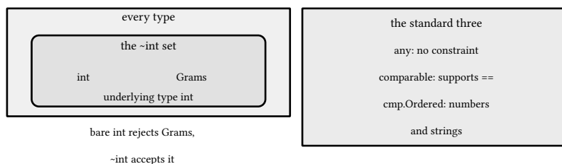
figure 17: constraints are interfaces: type sets, with the tilde opening the door
