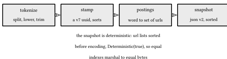
figure 226: body to doc to postings to snapshot, one fold each way
