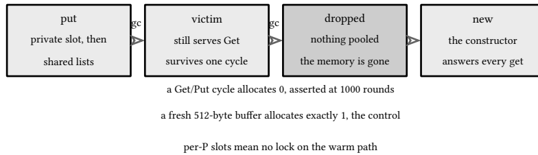
figure 53: the pool across two collections
