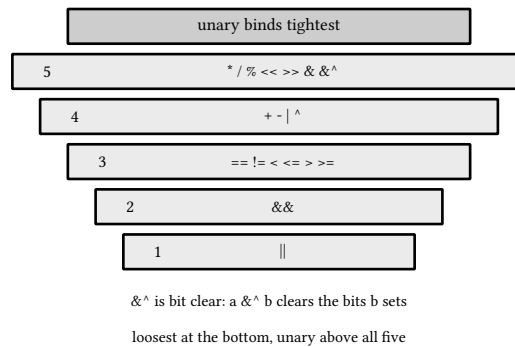
figure 9: five binary levels with unary above them all, comparisons yield untyped bool
