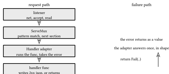
figure 101: the request climbs down the stack, the failure climbs back up as a value
