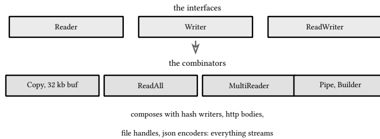
figure 73: three interfaces, combinators over them, everything composes
