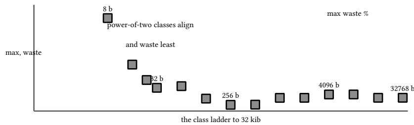
figure 50: class size against max waste, the spacing is the trade
