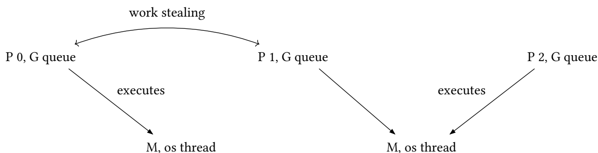
figure 43: G, M, P: goroutines wait in P run queues, M threads execute them, idle queues steal
