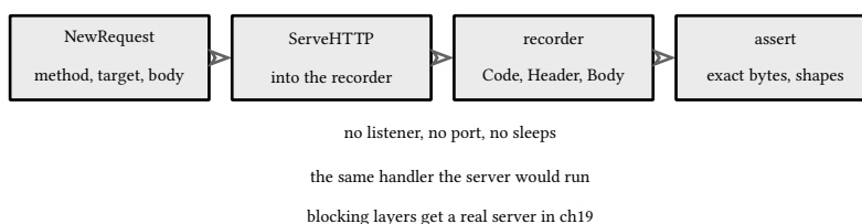
figure 105: request to handler to recorder to assertions, all one function call
