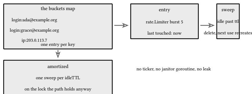
figure 161: key to limiter map, first use creates, idle age retires
