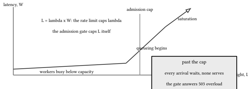
figure 165: latency versus concurrency: the hockey stick the admission cap cuts off
