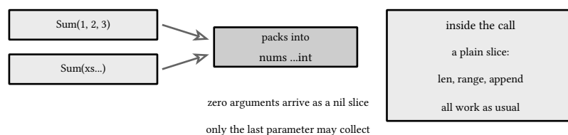
figure 24: variadics: two call shapes pack into one slice parameter
