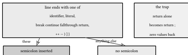
figure 8: semicolon insertion: the line-final token rule, and the return trap
