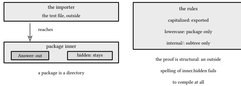
figure 42: the export boundary as a stack: capitalization crosses, lowercase stays
