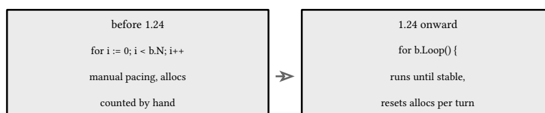
figure 77: b.Loop , the 1.24 harness that replaced the b.N loop
