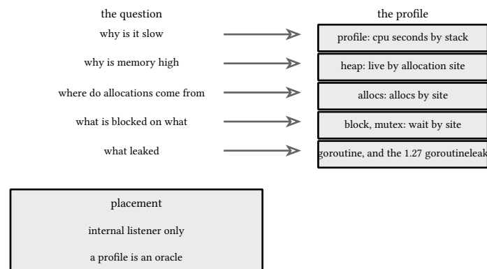
figure 171: which profile answers which question
