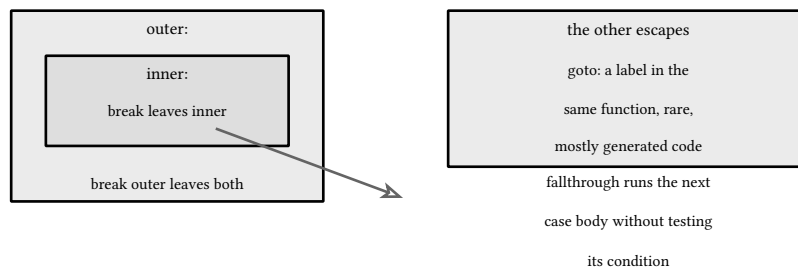
figure 40: the label names which loop the break leaves
