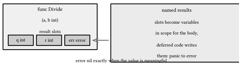
figure 21: results are slots the function owns, named ones stay in scope
