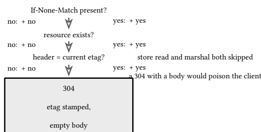
figure 146: the conditional GET decision
