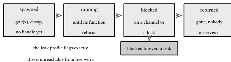
figure 46: spawned to returned with nobody watching, the leak is the blocked-forever case
