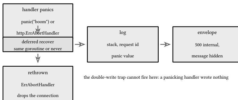
figure 109: panic unwind: one path to the log, one to the envelope, one rethrown
