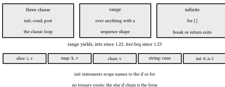
figure 38: one for keyword, three forms, and what range yields
