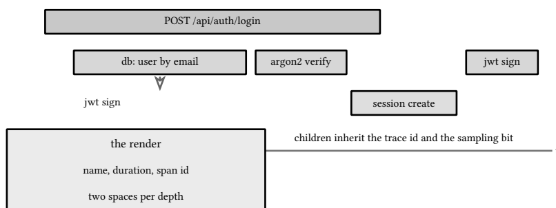
figure 168: one login request's spans over time, the tree the render prints
