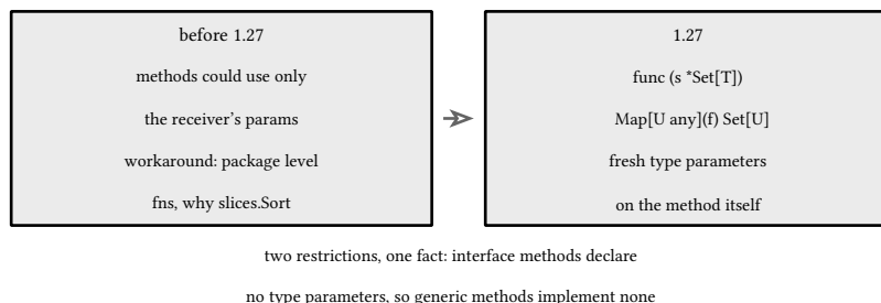
figure 19: generic methods, the 1.27 change: fresh parameters on the method
