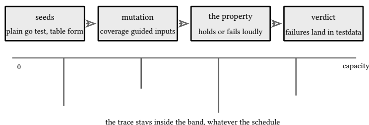
figure 188: seed to mutation to verdict, the bounds band drawn through a refill trace
