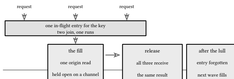
figure 148: three requests arrive together, one origin read happens
