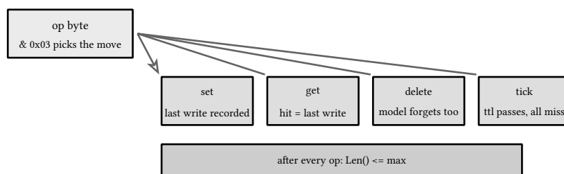
figure 189: ops and states with the bound guard under every step
