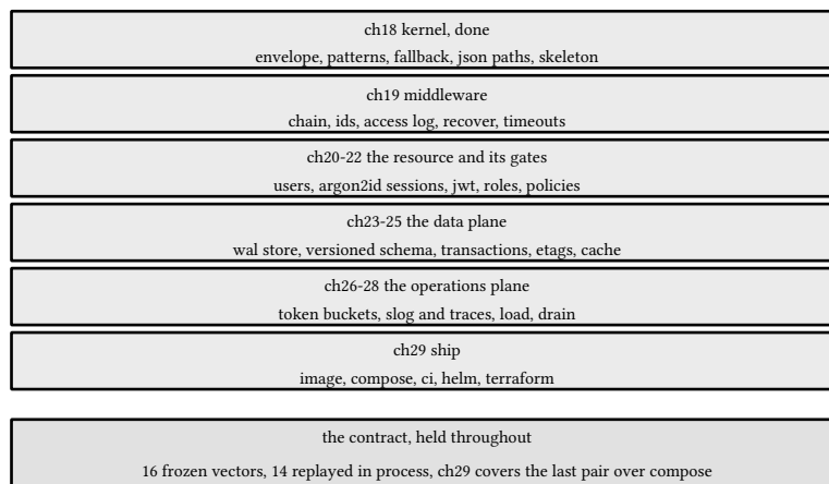
figure 107: the part as seven rows: every chapter adds routes or layers, none rewrites the kernel
