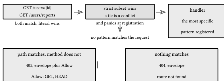
figure 102: pattern precedence: specific beats general, ties panic, leftovers split into 405 and 404
