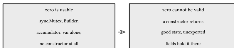
figure 81: aim at a usable zero, and when zero cannot work, construct
