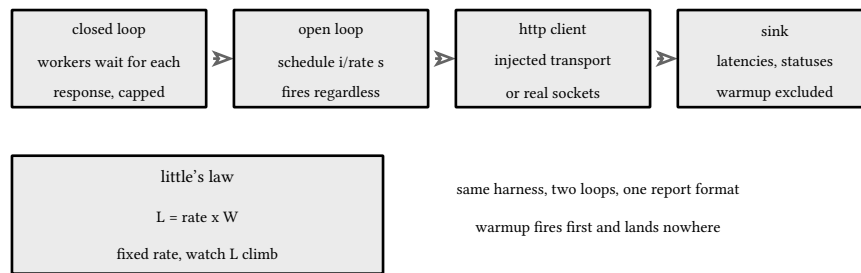
figure 173: workers, server, latency sink: one harness, two clocks
