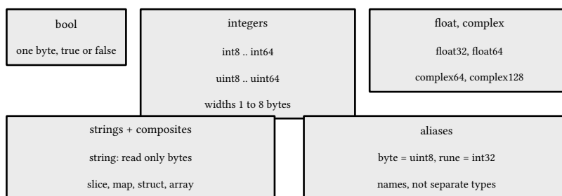
listing 9: sizes from unsafe.sizeof, rune is 4 bytes as int32 (source: go/samples/ch03/types.go, lines 32-50)
