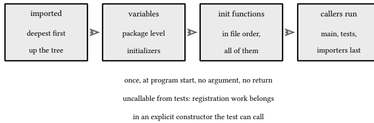
figure 26: package initialization runs once, in order, before any caller
