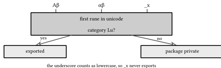
figure 6: export is one lexical test: the first rune decides
