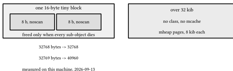
figure 51: tiny packing below, page rounding above
