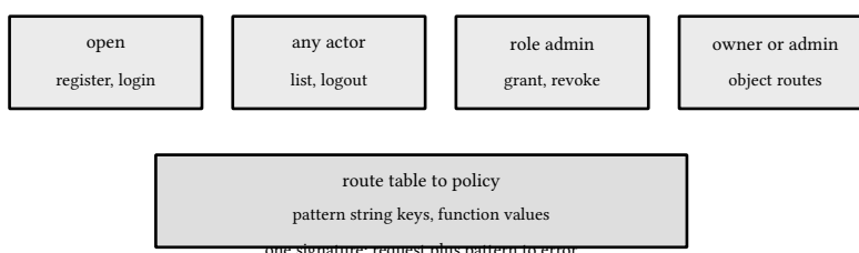
figure 132: four policies, one signature, the table maps routes onto them
