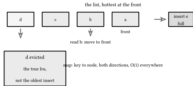
figure 154: a read moves its node to the front, an insert evicts the back
