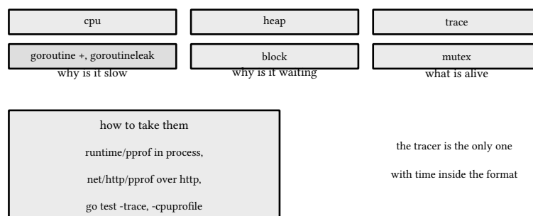
figure 55: six captures, three questions
