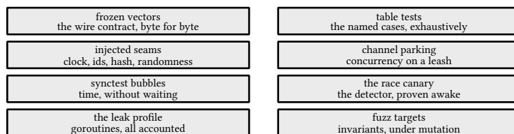
figure 187: the suite's layers, each against the one thing it proves
