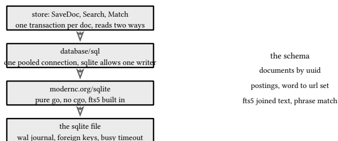
figure 227: the store stack: one interface, one pooled connection of one, one file
