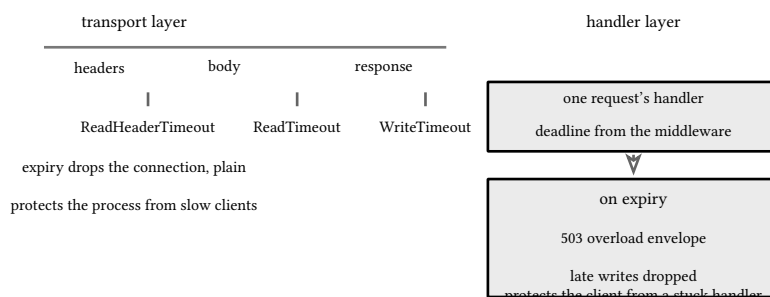
figure 112: two clocks: transport deadlines kill connections, the handler deadline answers
