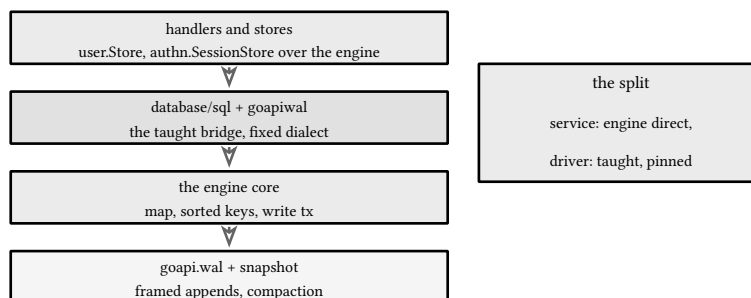
figure 137: the stack the store sits on: standard interface, owned engine, wal plus snapshot, no cgo
