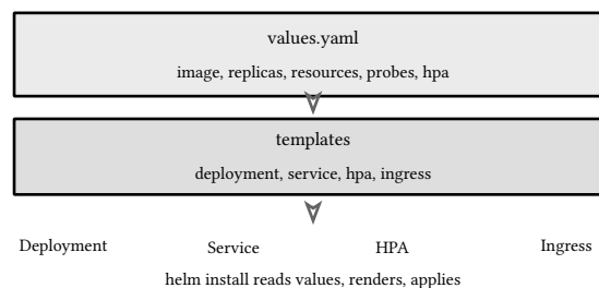
figure 184: the chart's layers: values flow down, objects render out
