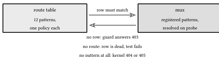
figure 135: the audit: table and mux face each other, both directions checked
