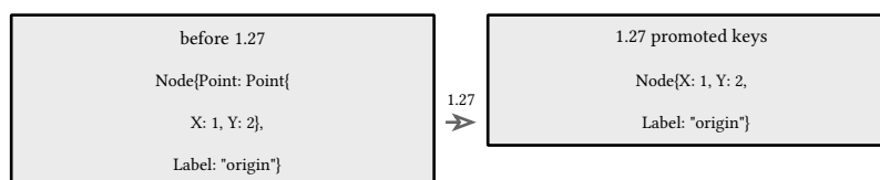
figure 14: composite literal keys before and after 1.27 promotion
