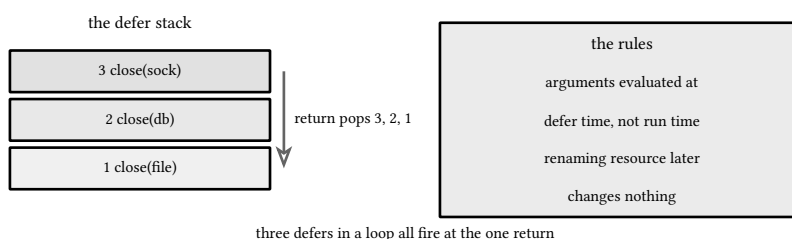
figure 22: defers stack up lifo, arguments already captured at registration
