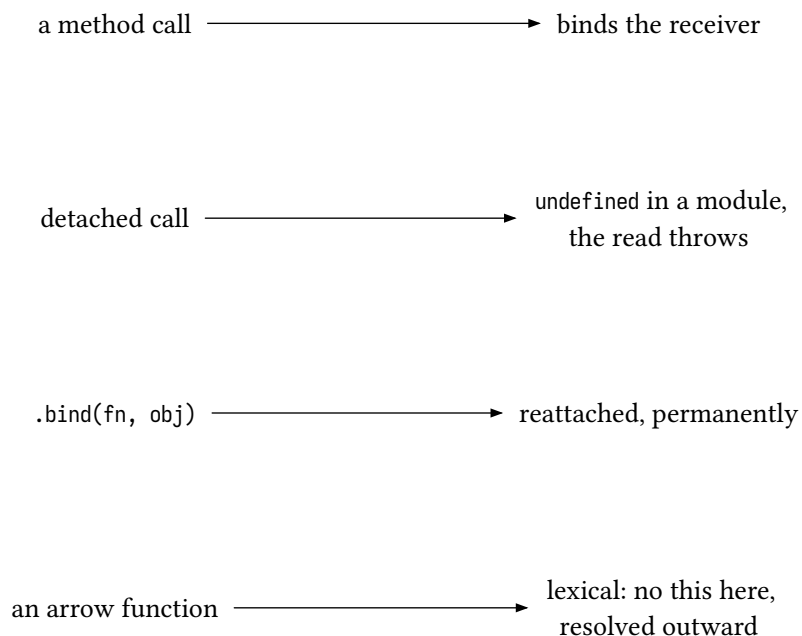
figure 10: receiver resolution, four ways a call finds its this
