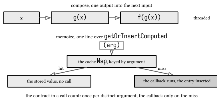
figure 14: compose threading one lane, memoize branching on the cache
