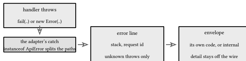
figure 139: one path to the log, one to the envelope, nothing rethrown
