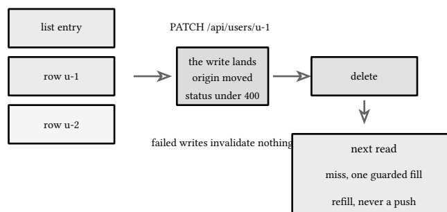
figure 182: write to a row: the row, the list, and children go, the refill is the only writer
