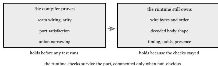
figure 219: two columns, both true
