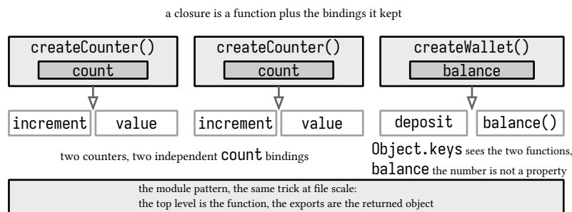
figure 12: the closure kept per call, and the module as the same trick at file scale
