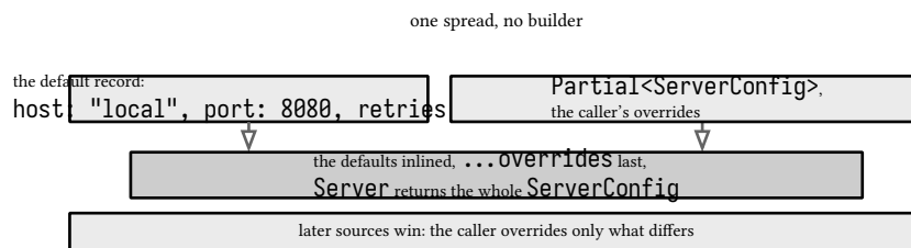
figure 112: defaults, Partial over one spread, no builder
