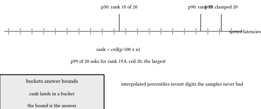
figure 200: the tail ladder: where p50, p90, p99 sit in one sorted sample
