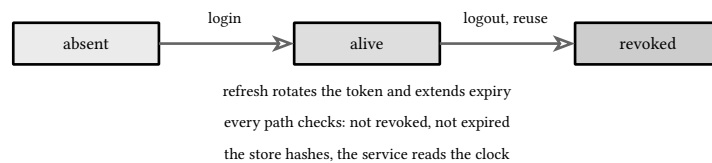
figure 151: the session lifecycle: login creates, refresh rotates, logout or reuse revokes
