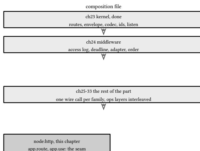
figure 134: every chapter lands as one import and one call, in chapter order
