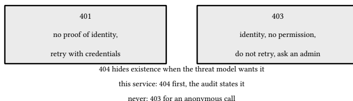
figure 160: the two failure codes, and the one deliberate blur
