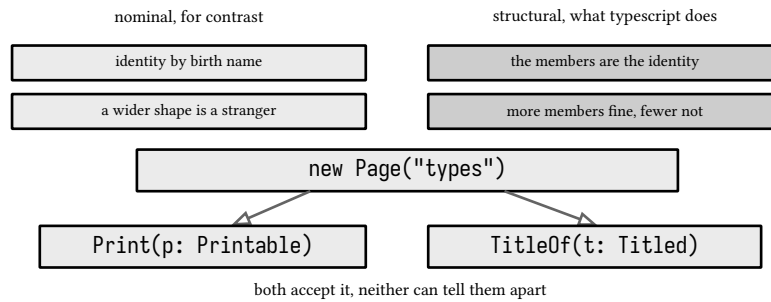
figure 71: nominal against structural, one value through both worlds
