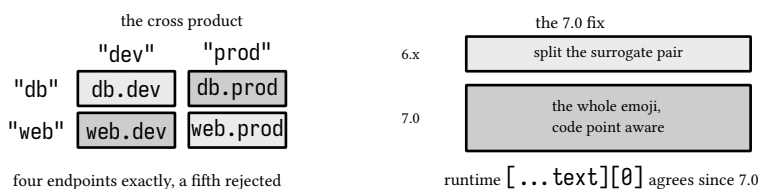
figure 92: a cross product of unions, and the 7.0 code point fix
