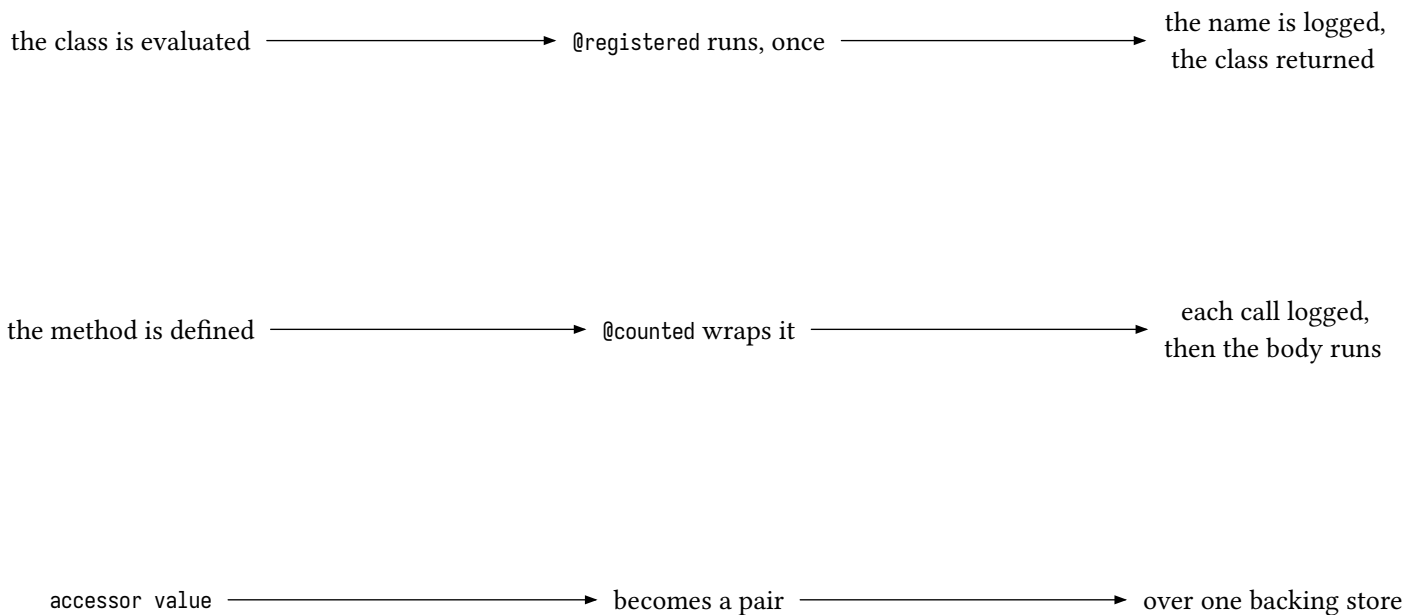
figure 98: decorators at definition time, wrappers at call time
