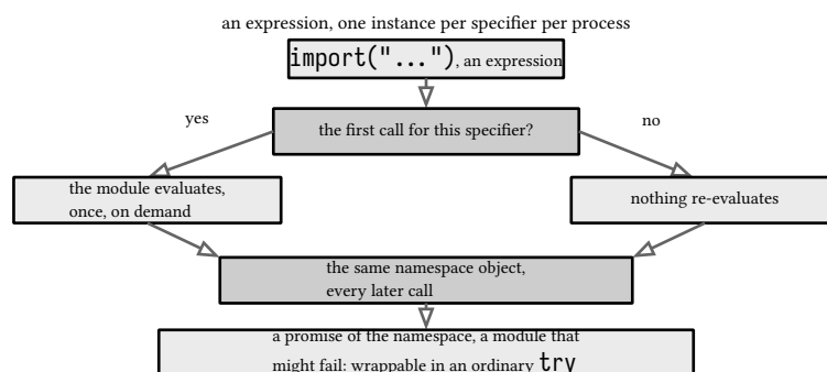
figure 36: the dynamic import, one namespace per specifier
