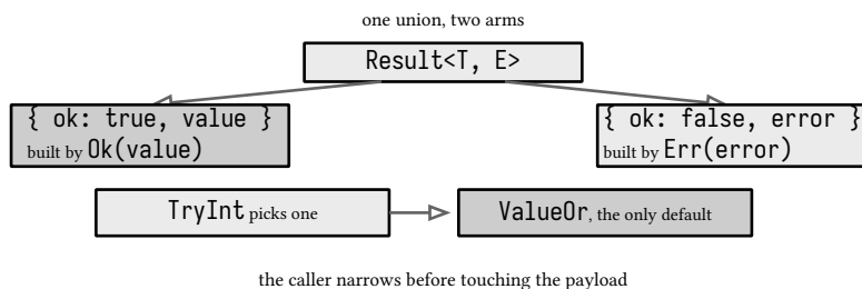
figure 108: the result union, two arms one contract
