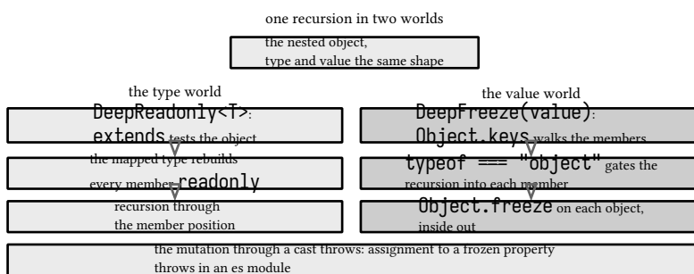
listing 149: DeepReadonly over DeepFreeze (source: javascript/tssamples/ch20/idioms.ts, lines 42-55)
