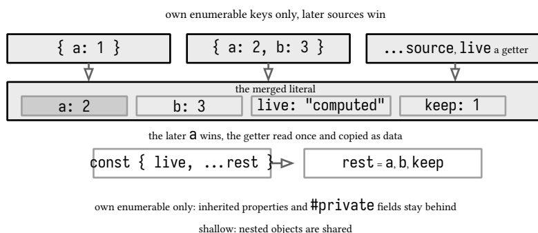
figure 21: spread merging three sources into one snapshot, rest collecting the unnamed
