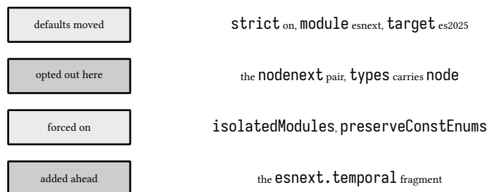
figure 63: tsconfig options by what 7.0 lets a project still turn
