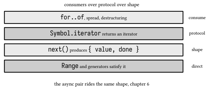
figure 22: the protocol, stacked
