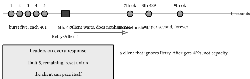
figure 187: a client that honors Retry-After: five through, one refused, the next at the reset instant
