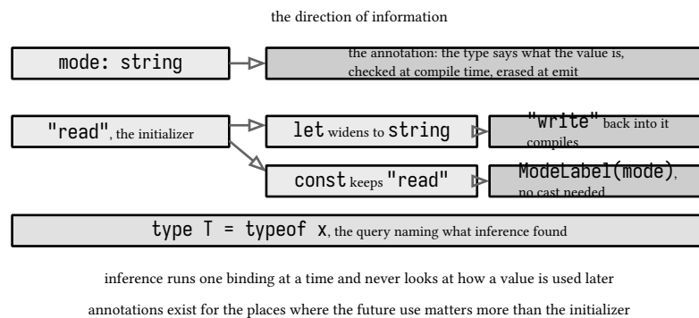
figure 65: annotation and inference, let widening against const keeping
