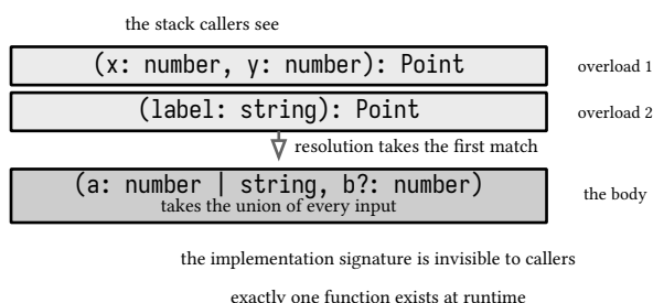
figure 74: the overload stack, two signatures callers see over one body
