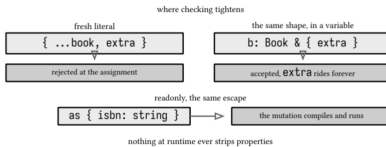
figure 81: excess property checks and readonly, where the tightening stops
