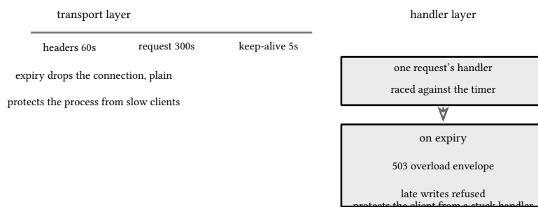
figure 138: two clocks: transport deadlines kill connections, the handler deadline answers
