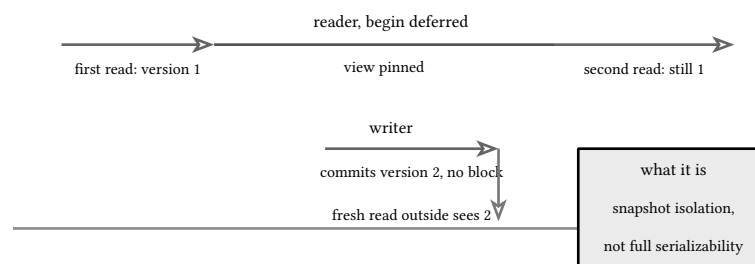
figure 168: one timeline: the reader's view holds
