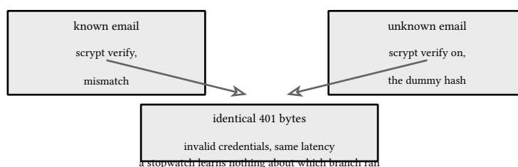
figure 150: the timing-equalized login: unknown email pays what a wrong password pays
