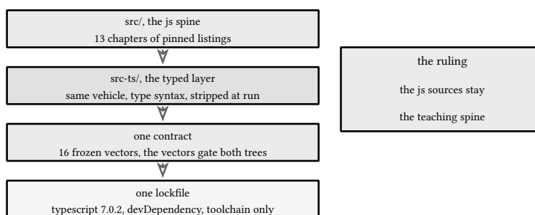
figure 215: two notations, one contract underneath
