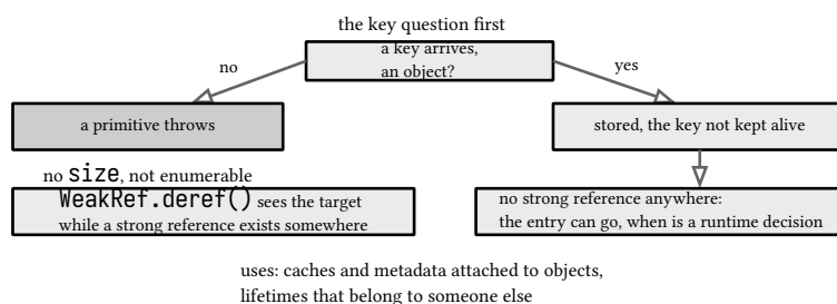
figure 27: the weak side, what is deterministic and what the runtime owns
