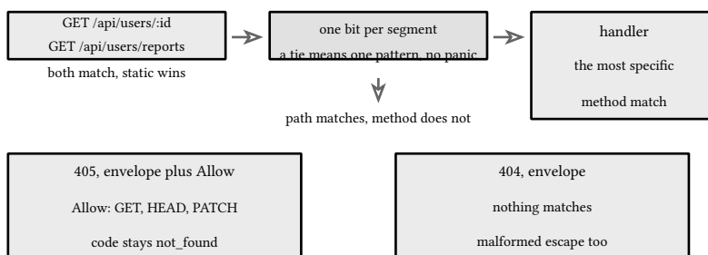
figure 130: static beats param, ties are unrepresentable, leftovers split into 405 and 404
