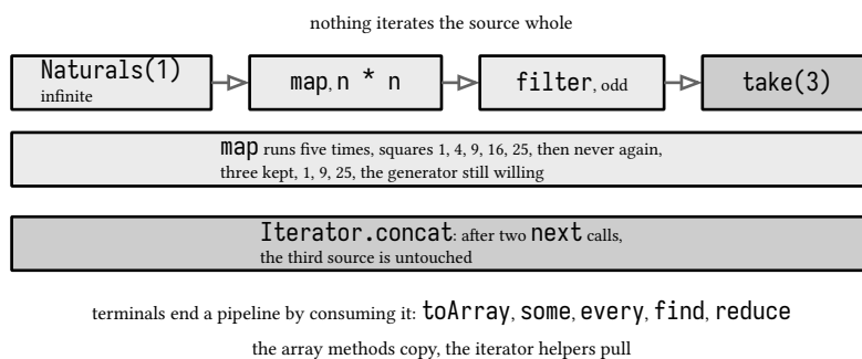
figure 24: the pull discipline, each helper an iterator wrapping the last
