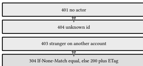
figure 147: one request climbs the ladder, each rung one contract code
