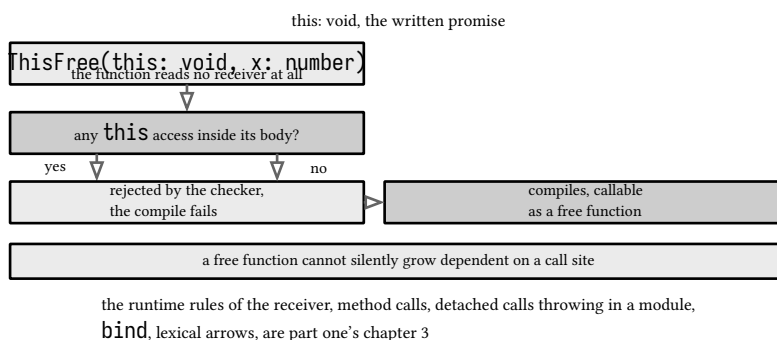
figure 78: the checked this , a written promise the checker enforces
