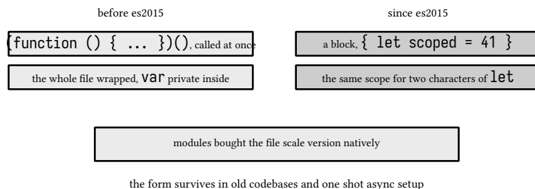
figure 13: the iife against the block that replaced it, the same scope re-priced
