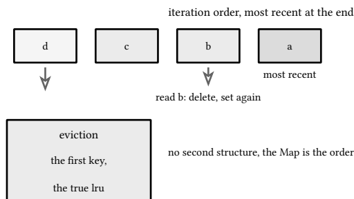
figure 179: one Map, oldest first, hottest last
