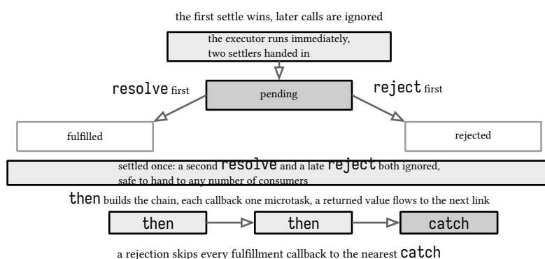
figure 30: the settle once machine, the chain riding beneath
