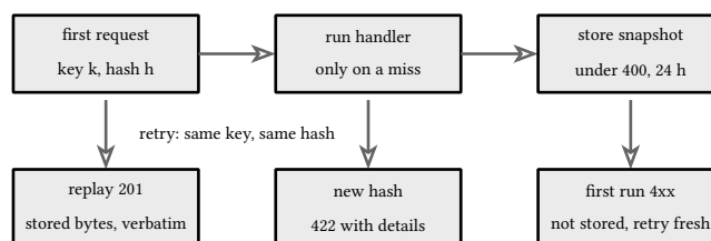
figure 175: one key's life: first run, snapshot, replay, refusal
