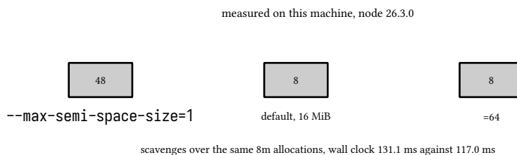
figure 52: scavenge count against semi space size, one churn workload
