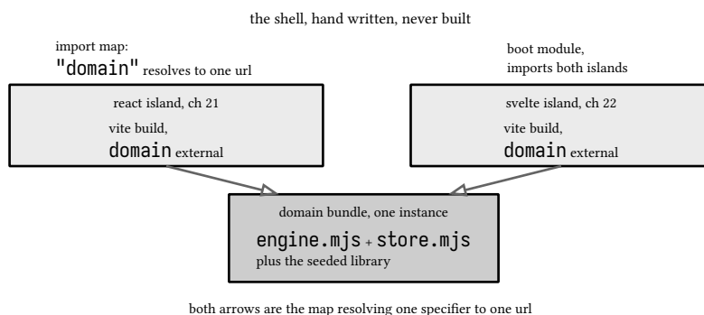
figure 228: one shell, one map, two islands, one engine
