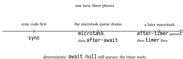
figure 29: one run through the queues, in order
