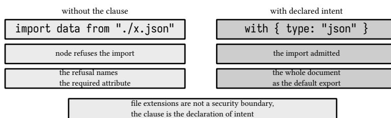
figure 37: the with clause, declared intent against the refusal
