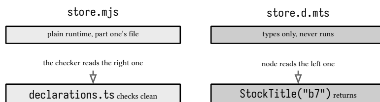
figure 102: the declaration boundary, who reads which file
