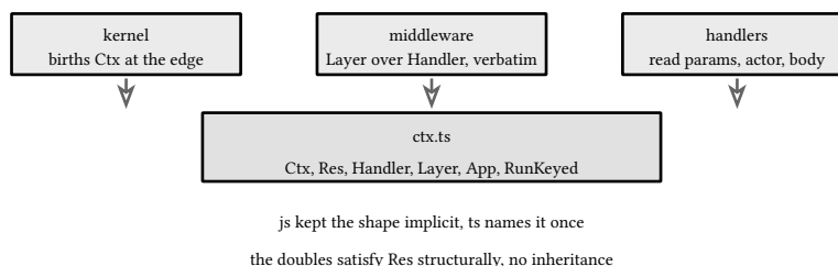
figure 217: one seam module, three consumers, no drift
