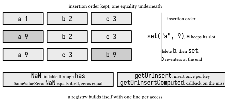
figure 25: the map slots through three operations, order as the visible fact
