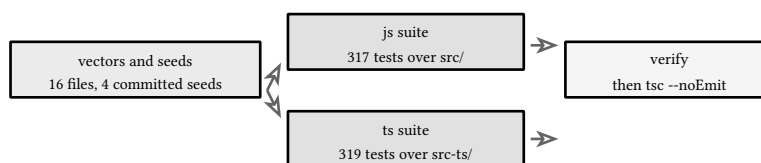
figure 220: one suite, two trees, one gate
