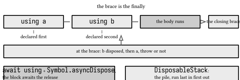
figure 39: the block scope as a resource scope
