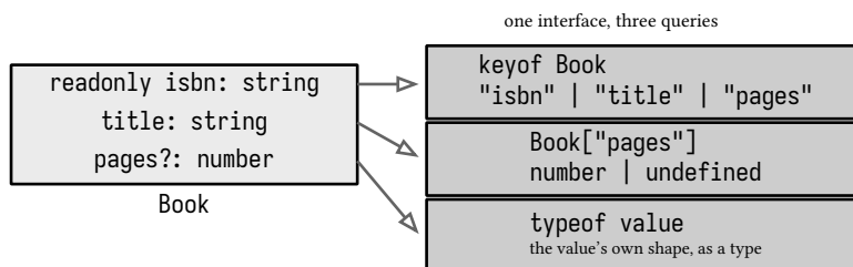
figure 89: keyof , indexed access, and typeof against one interface
