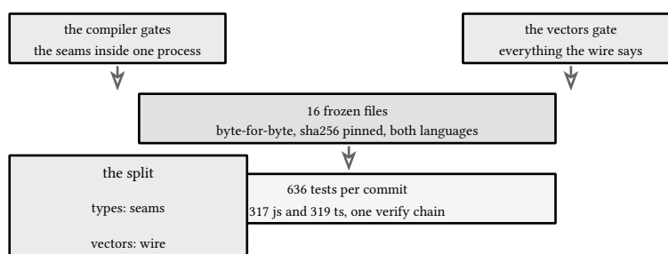
figure 222: what gates what
