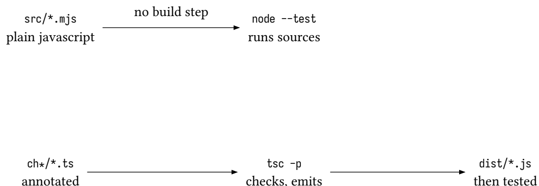
figure 3: the two verify chains, one stage for part i, two for part ii
