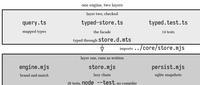
figure 223: the two layers, who runs and who checks
