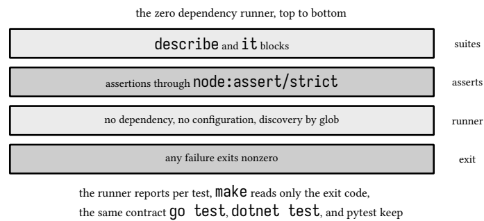
figure 2: the test framework stacked, blocks to assertions to the exit code
