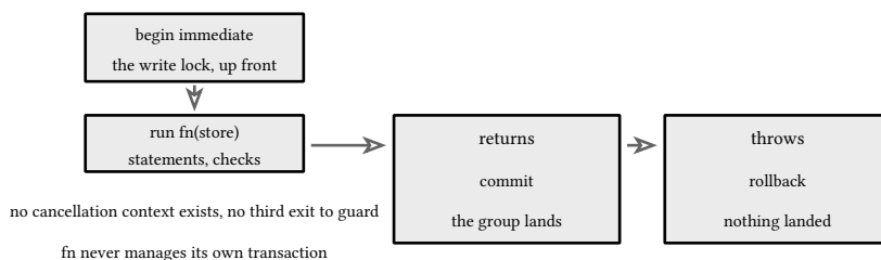
figure 167: a transaction has exactly two exits
