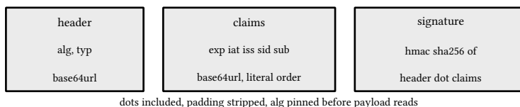
figure 153: three segments, the signature covers exactly the first two
