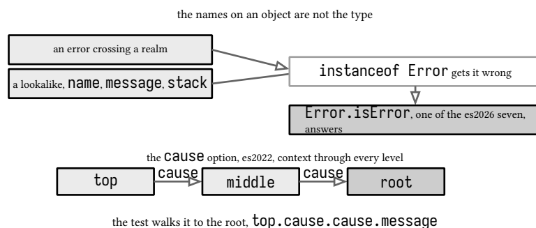
figure 43: the type question, and the chain that carries context
