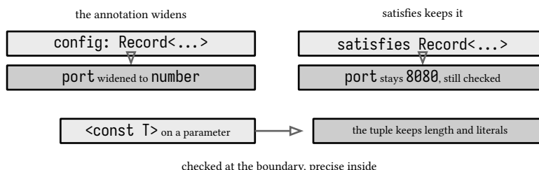
figure 113: widening against satisfies, literals kept while checked
