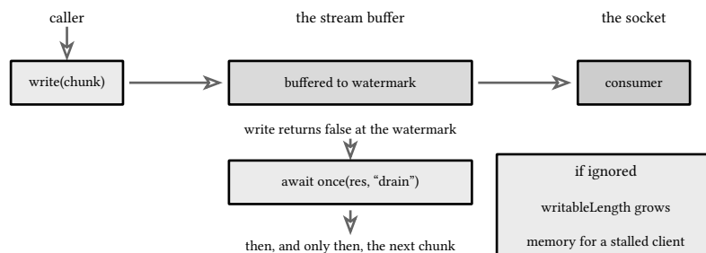
figure 201: the write path: offer, buffer, drain, offer again
