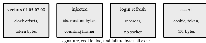
figure 156: an auth golden test: fixed inputs in, frozen bytes out
