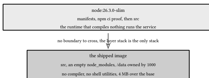
figure 203: one stage, nothing to cross: the runtime is the toolchain is the app
