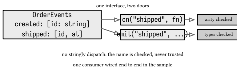
figure 111: the emitter, one interface behind both doors
