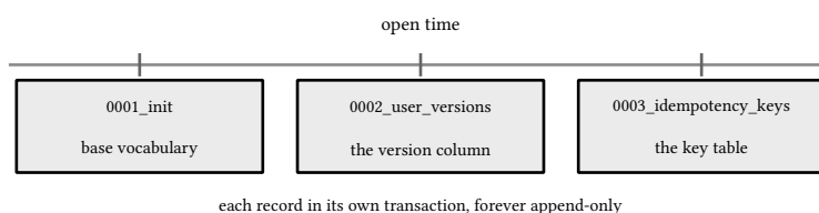
figure 165: the version list only grows right
