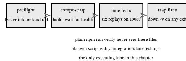
figure 205: the gate: one lane, one trap, no skips
