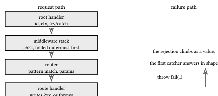
figure 129: the request climbs down the stack, a failure climbs back as a rejection
