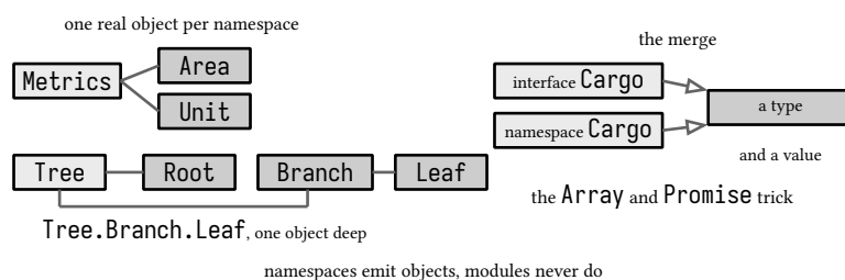
figure 101: namespaces as emitted objects, and the cargo merge
