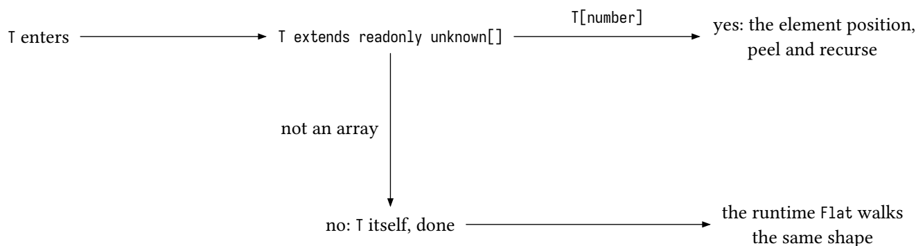
figure 91: the conditional type as routing, arrays peeled until they are not
