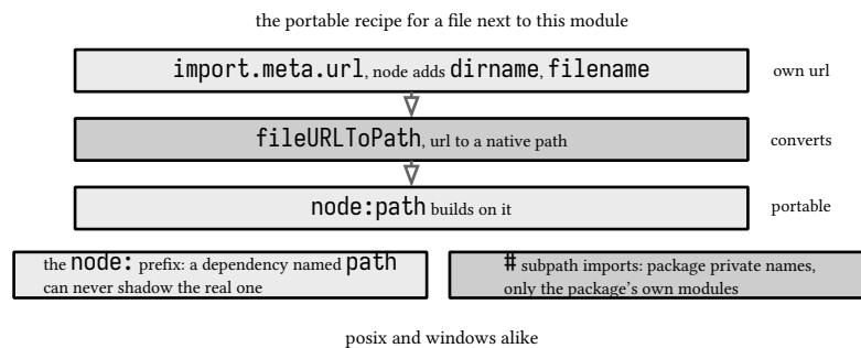
figure 38: the module's own address, made native
