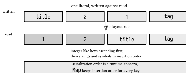
figure 16: the written order against the read order, one rule between them
