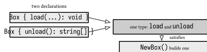
figure 83: declaration merging, two boxes into one type
