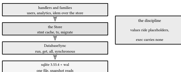
figure 164: the stack the store sits on
