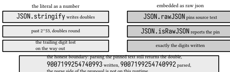
listing 62: raw digits surviving stringify, and the double that comes back from parse (source: javascript/samples/src/ch08-edition.mjs , lines 63-78)
