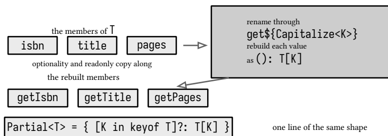
figure 90: the mapped type pipeline, rebuild and rename every member
