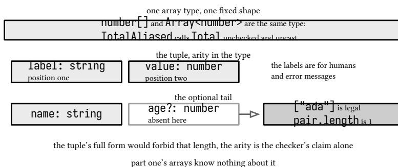
figure 68: arrays in two spellings, the tuple's fixed shape
