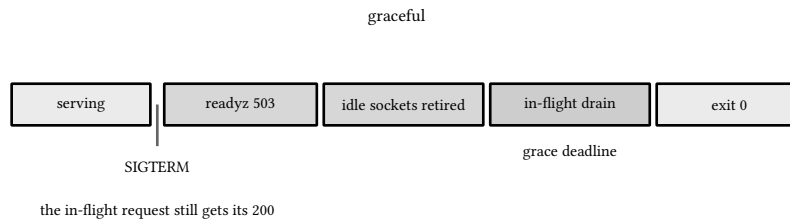
figure 197: SIGTERM to drain to exit, against the hard kill
