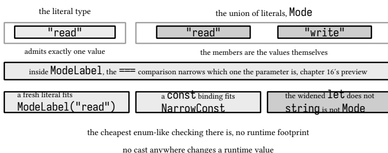
figure 67: literal and union literal types, the members are the values themselves
