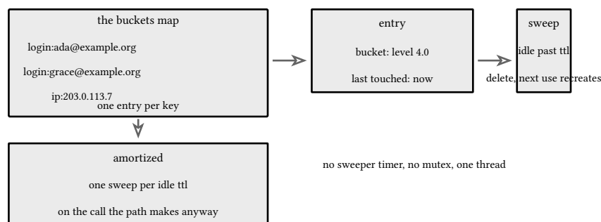
figure 186: key to bucket map, first use creates, idle age retires
