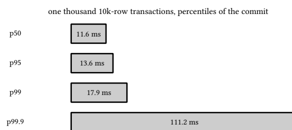
figure 58: the commit tail of the ten million row insert
