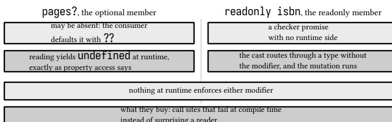
figure 80: the two modifiers, no runtime side on either
