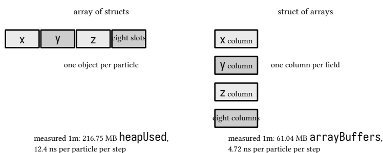
figure 51: the same state, two shapes of memory
