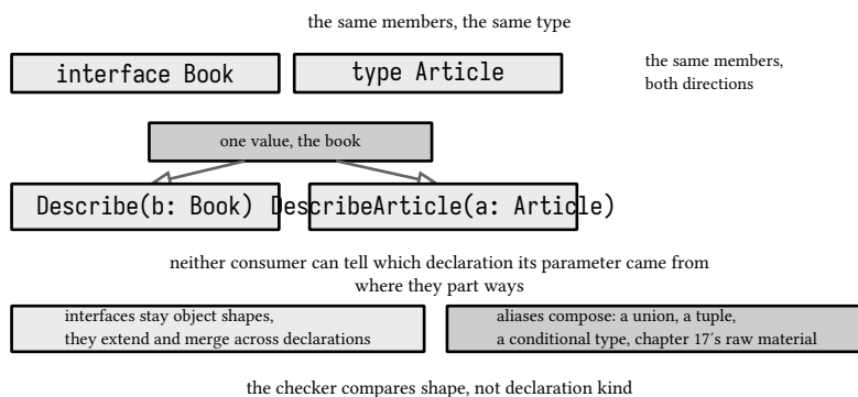
figure 79: interfaces against aliases, the same members as the same type
