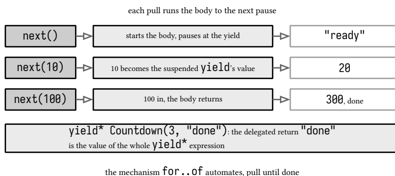
figure 23: the body paused and resumed, three pulls of one generator
