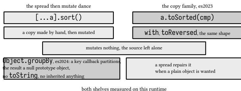
figure 41: the copy family, and the grouping it left to repair
