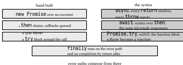
figure 31: the syntax against the hand built forms it replaces
