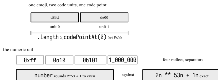
figure 6: one emoji in utf-16 memory, and the numeric rail beside it
