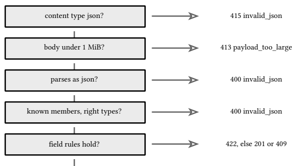
figure 143: the decode ladder: each rung rejects a class of bad input
