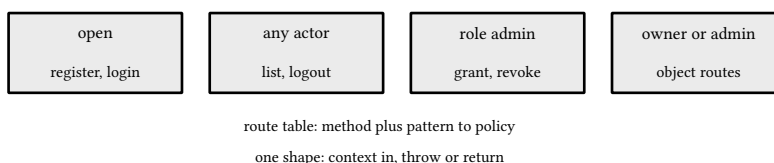
figure 159: four policies, one shape, the table maps routes onto them
