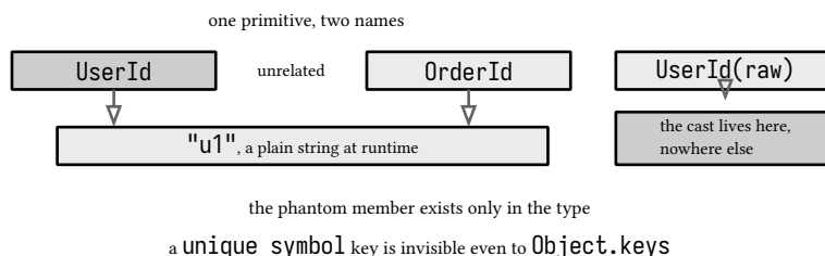
figure 106: the phantom member, two ids over one string
