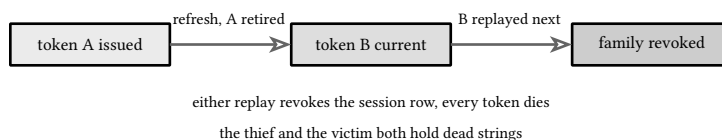
figure 155: the refresh family: rotation forks, reuse revokes everything
