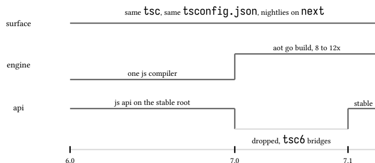
figure 61: the 7.0 port as a release timeline, three rails against the version axis
