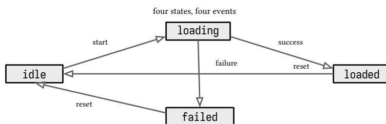
figure 110: the transition table as a machine, four states
