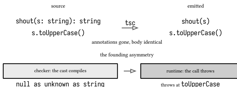
figure 60: the founding asymmetry, annotations erased at emit while the null cast reaches the runtime
