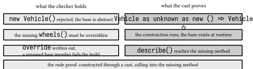
figure 95: abstract classes, a checker fact against the cast
