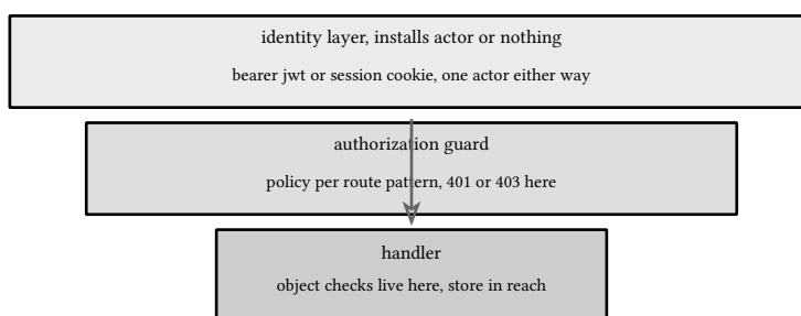
figure 157: two layers in wiring order: identity outside, guard inside, handler last
