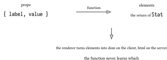
figure 115: props to elements, one direction
