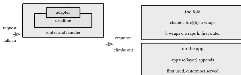
figure 136: the onion: first argument outermost, request in, response out
