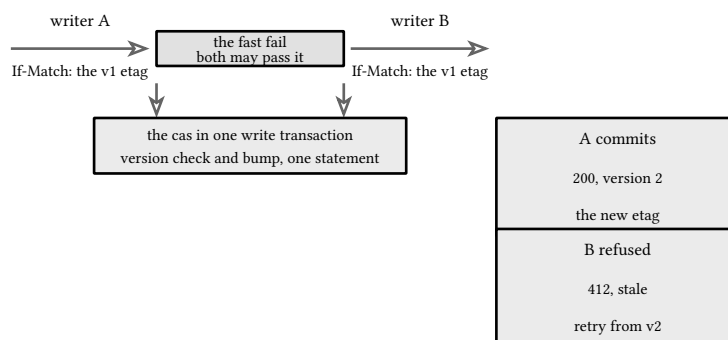
figure 174: two patchers, one fast fail, one cas, one winner
