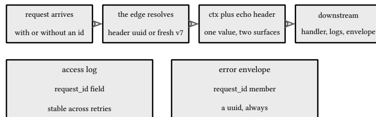
figure 133: one id, born at the edge, quoted by everything downstream
