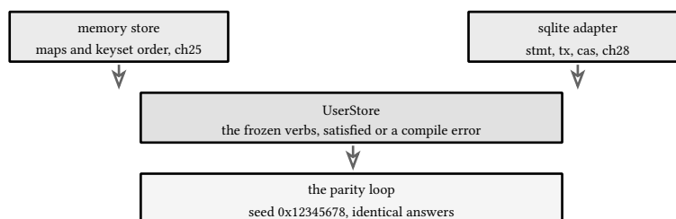
figure 218: two implementations, one interface, one property loop
