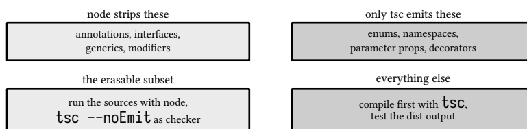
figure 104: the strip only subset, and the workflow split
