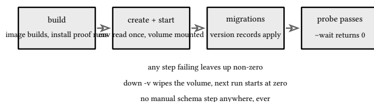
figure 204: what a green up proves, in order
