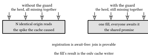
figure 181: the same expiry, with and without the guard
