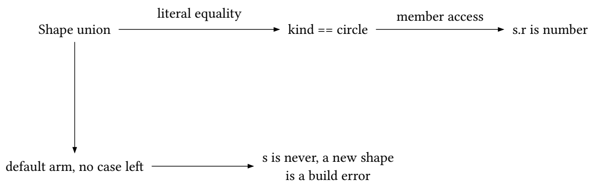
figure 88: a value narrowing as it flows through guards, the default arm to never
