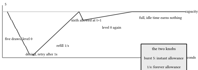
figure 185: bucket level over one draw timeline, the refill climbing between bursts
