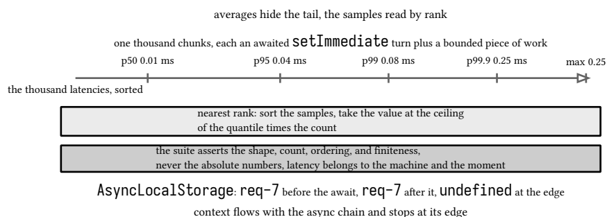
figure 57: the sorted thousand, read by rank
