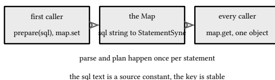
figure 166: same string in, same statement out
