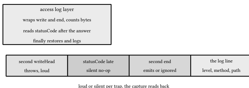
figure 137: status read after the answer, bytes counted at the writes, one line per request
