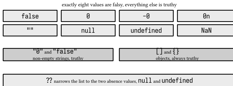
figure 8: the eight falsy values as a closed list, the surprises that stay truthy
