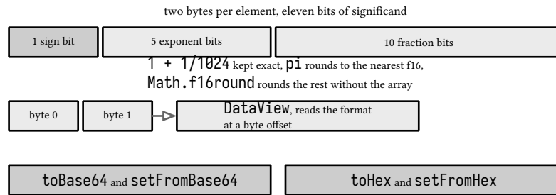
figure 28: f16 memory, the view over it, and the codec pairs
