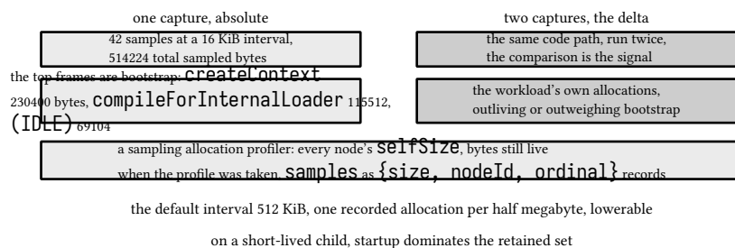
figure 54: one capture against two, the delta as the signal
