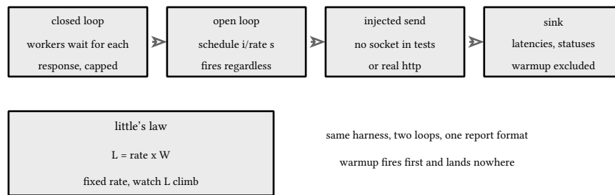
figure 199: workers, server, latency sink: one harness, two clocks
