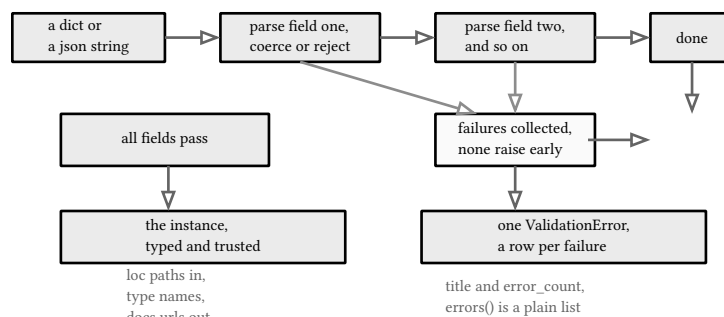
figure 108: validation as a state machine: parse each field, collect every failure, hand back one instance or one error with all rows
