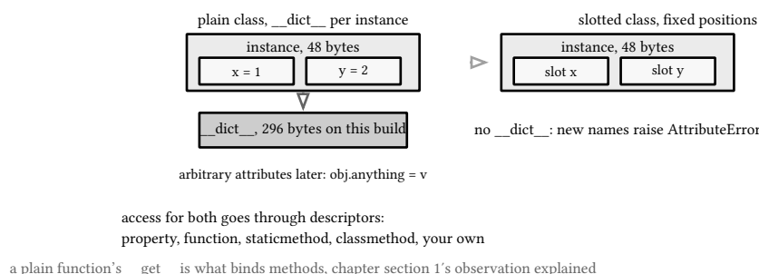
figure 28: where attributes live, with and without slots
