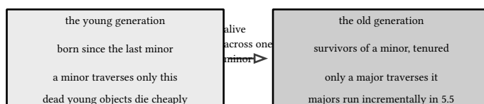
listing 65: tenured garbage is minor-proof, the major frees it (source: lua/samples/ch09_collector.lua, lines 120-139)
