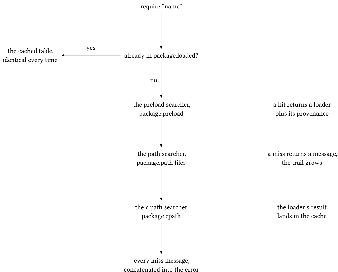
figure 62: the require pipeline, searchers in order, the cache in front
