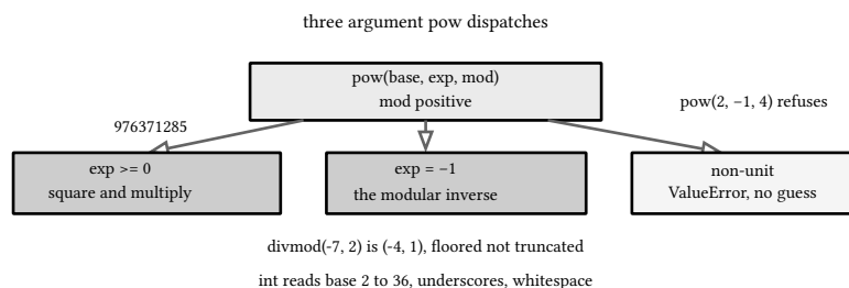
figure 60: one builtin, three exponents, and the floored pair
