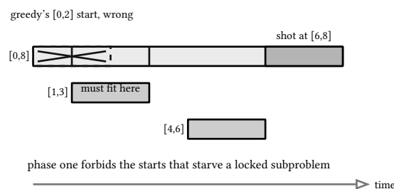
figure 90: three windows, the two short shots locked late, the [0,8] shot at [6,8] , the greedy's wrong [0,2] start crossed out
