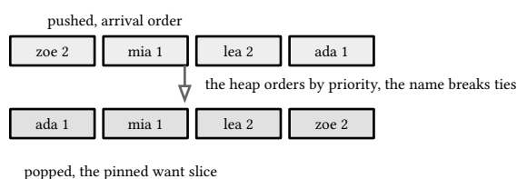
figure 32: four workers in arrival order, the drain order out, priority first and the name breaking ties
