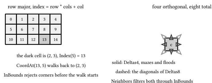
figure 37: row-major flattening and the two neighborhoods
