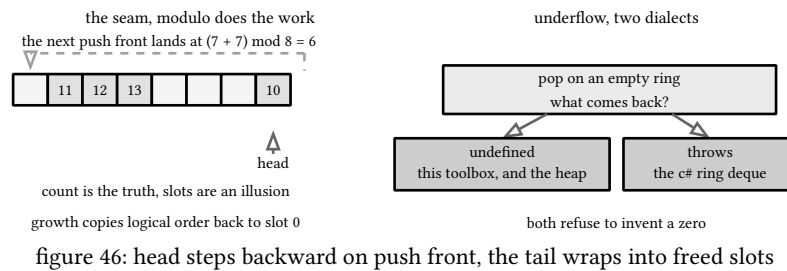
figure 46: head steps backward on push front, the tail wraps into freed slots
