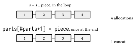
figure 74: two loops over four pieces: a dot in the loop body allocates four fresh strings, the parts table pays one concat
