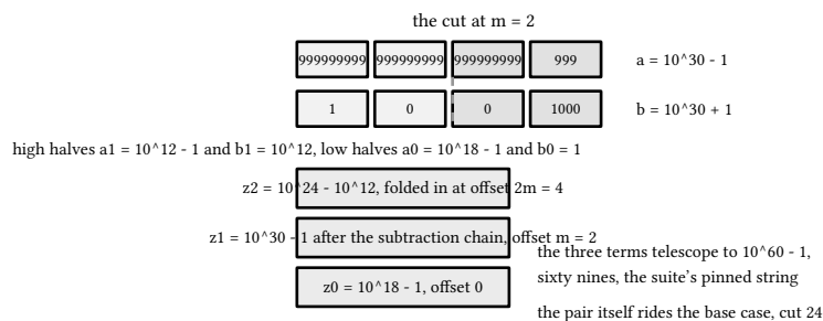
figure 183: one level on the carry stressor, both operands cut at m = 2 , three multiplies, the recombination telescoping to sixty nines The pinned sixty nines close the run, and the listings below build the split and the recombination in six languages.
