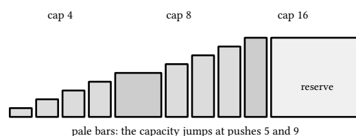
figure 15: size against capacity across the pinned pushes, the doubling staircase under every append
