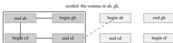
figure 99: the fixture's closure graph: the seeded end(ab) reaches three more vertices, and those four marks are exactly the printed commas
