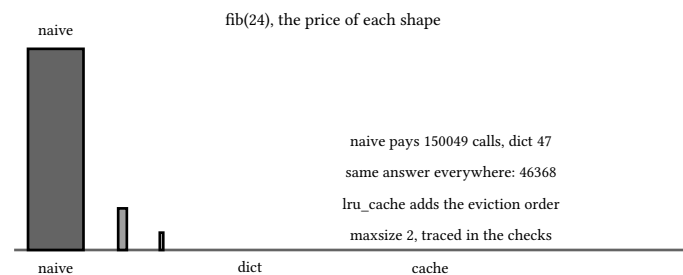
figure 56: one answer, three call counts
