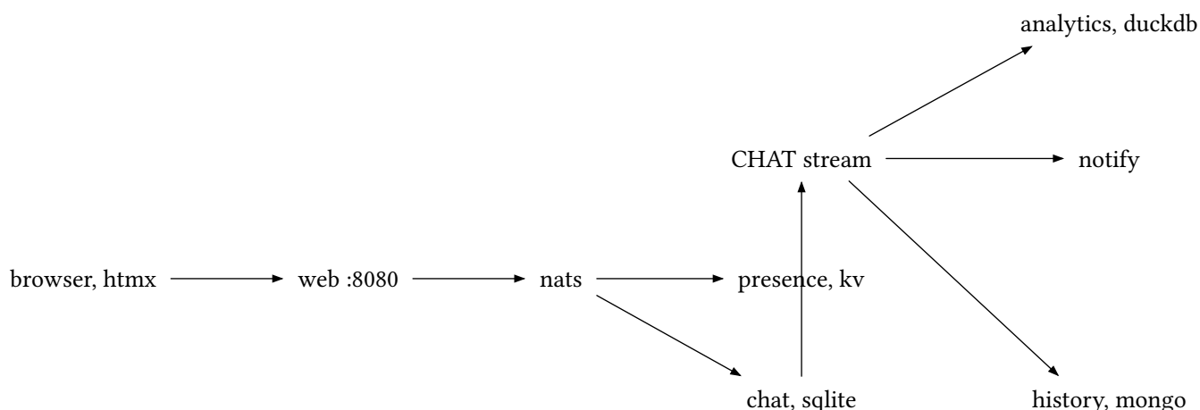
figure 57: the system, one message's path
