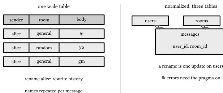
figure 15: the wide row against the normalized shape, and what a rename costs
