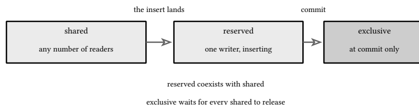
figure 18: the lock ladder a writer climbs, and what blocks at the top
