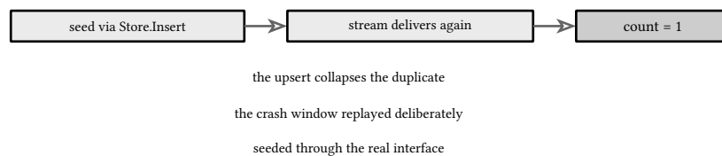
figure 52: seeding replays the crash window, through the real interface
