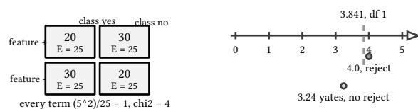
figure 32: the 2x2 table and the two verdicts against the df 1 threshold
