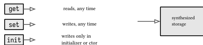
figure 24: a property, one storage behind three accessor gates
