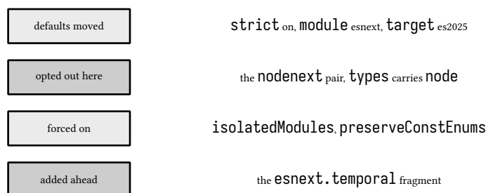
figure 63: tsconfig options by what 7.0 lets a project still turn
