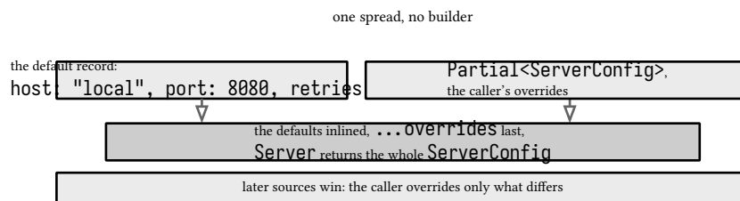
figure 112: defaults, Partial over one spread, no builder
