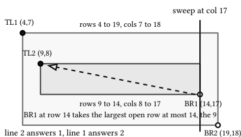
figure 97: the sample 1 rectangles nested, the sweep line on column 17 closing the inner block first
