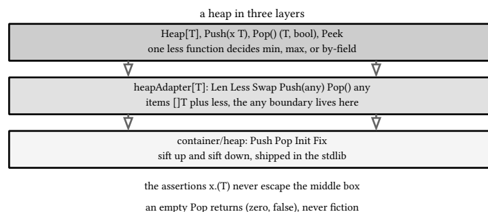
figure 26: three layers, the generic type on top, the any-typed adapter in the middle, the stdlib algorithm below
