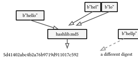
figure 63: the same five bytes by two shapes, one shot and streamed as hel then lo, one digest
