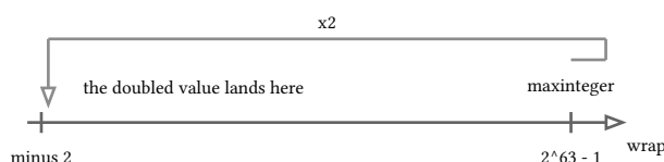
figure 77: the wrap, stated as a number line: maxinteger doubled runs off the end and reappears at minus two
