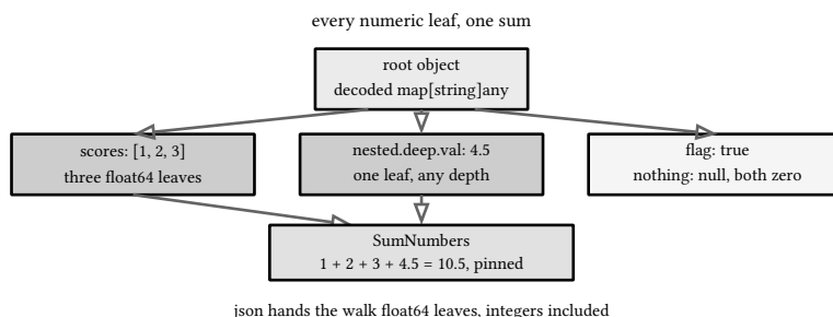
figure 35: the walk sums float64 leaves, the boolean and null are zeros
