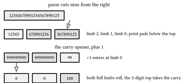
figure 183: the run as a sequence, the string cut from the right into three limbs then printed back top-bare, the carry opener rolling over beneath
