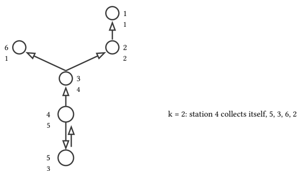
figure 128: sample 1's ring 4-5 with its hanging tree, every station labeled with its answer, station 4's five reachers marked
