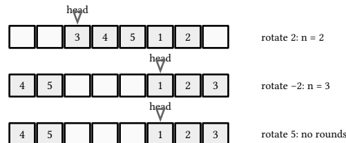
figure 70: the cap 8 slots across the three rotations, live entries and the head, the values wrapping the seam
