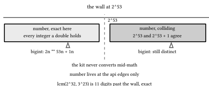
figure 50: the wall at 2^{53} , number collides, bigint keeps counting
