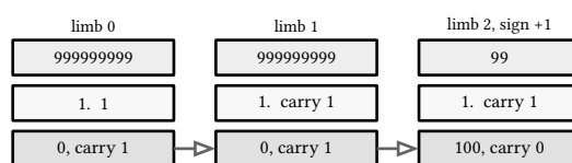
figure 7: the carry chain across all three limbs: each full base records a zero limb and passes one up, the top limb absorbs the last
