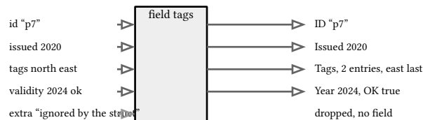
figure 34: the passport through the field tags: four keys map, the undeclared one drops
