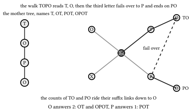
figure 127: the fixture's mother chain on the left, the query trie of reversed queries on the right, the name OPOT walking the heavy path TOPO whose suffix links feed the O and P queries
