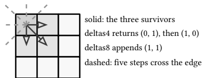
figure 29: the corner's eight offered steps: three survive, five cross the edge
