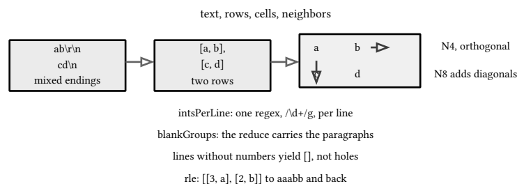
figure 52: text to rows to cells, the deltas ready for the walk
