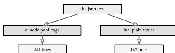
figure 81: the same grammar, two destinations: c parses into a tagged node pool, lua returns the tables the language already has
