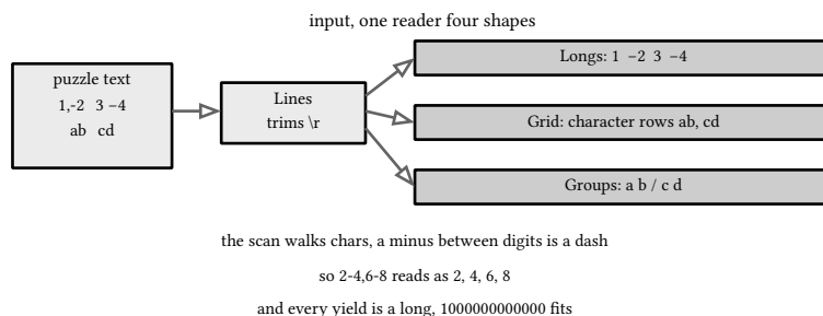
figure 39: one reader, four shapes, the scanner decides what a minus means
