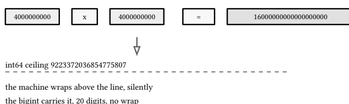
figure 67: why the toolbox needs a bigint: the 4e9 squared product sits past the int64 ceiling, and the machine says nothing
