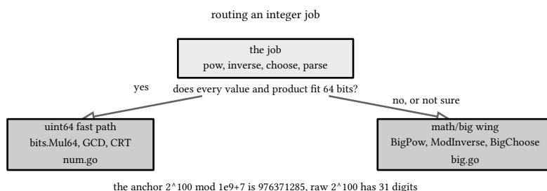
figure 31: routing an integer job, the 64-bit fast path against the unbounded wing
