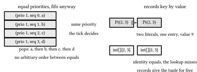
figure 37: equal priorities, the sequence decides: the bare heap leaves equal elements in arbitrary order, the stamped comparator restores arrival order
