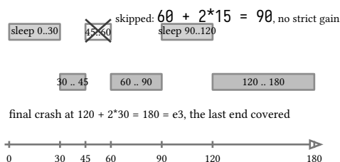
figure 158: sample 1's timeline: the two taken sleeps, the skipped middle gap crossed out, the crash bound landing exactly at 180
