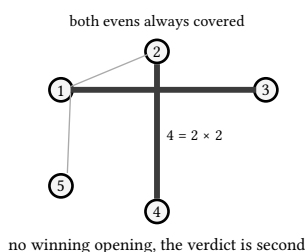
figure 166: the n = 5 prime-multiple graph, the size-2 matching bolded, both even numbers 2 and 4 covered by every maximum matching
