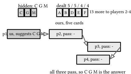
figure 84: 21 cards into 3 hidden plus hands of 5, 5, 4, 4, one suggestion passing three times then unseen evidence
