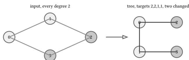
figure 115: the input 4-cycle beside the constructed tree, the two changed nodes shaded
