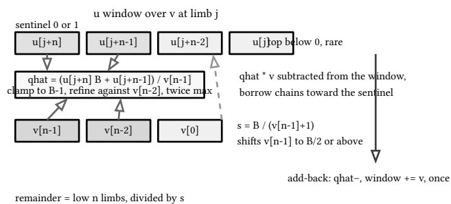
figure 190: one quotient digit: normalize, estimate two-over-one, refine, multiply-subtract down the window, add back on the rare negative top
