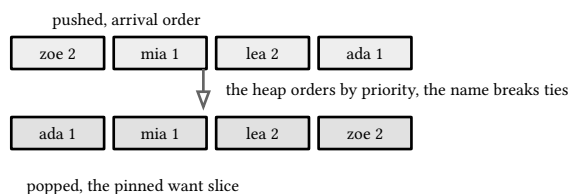
figure 25: four workers in arrival order, the drain order out, priority first and the name breaking ties
