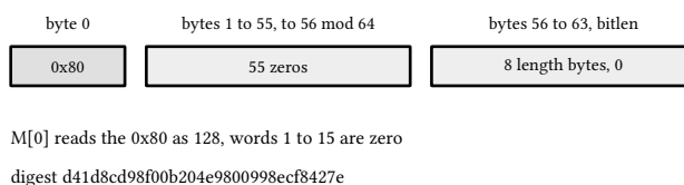
figure 78: the empty message's one chunk: one 0x80 byte, zeros to 56 mod 64 , eight zero length bytes
