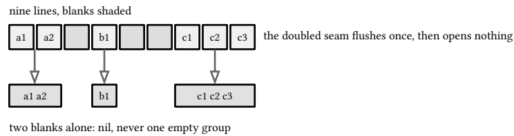
figure 27: nine lines, three seams, three groups: a blank that meets an empty pending group opens nothing
