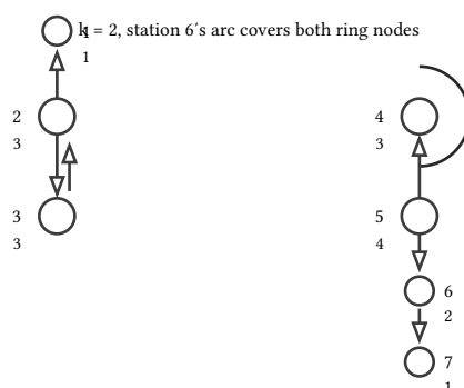
figure 129: the fixture's two rings with their hanging trees, every station labeled with its answer, station 6's +1 arc drawn as a heavy ring segment
