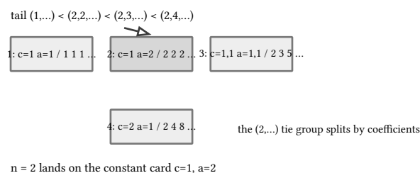
figure 154: cards ordered by generated tail, the tie at (2,...) split by coefficient lists, the pointer on card 2
