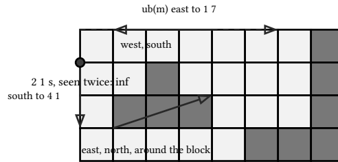
figure 130: sample 1's grid with the wall block shaded and program 2's wall-following lap: east to 1 7, around the block through 2 1, 4 2, 3 5 and 1 4, back to 2 1 south
