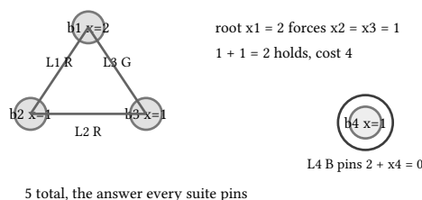
figure 134: the fixture: a button triangle with one consistent assignment, plus the single-button light that pins its own press
