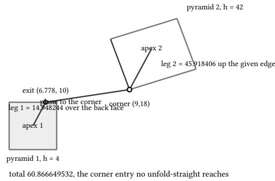
figure 139: sample 1's one-corner winner: down pyramid 1's back face, across to the corner (9,18), up pyramid 2's given-edge face
