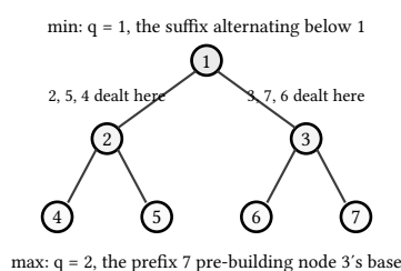
figure 164: the sample-1 tree, node 1 owning 2 and 3 over four leaves, with the min line's root-first split and the max line's one-element prefix annotated
