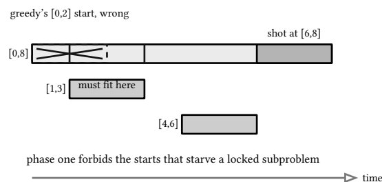
figure 92: three windows, the two short shots locked late, the [0,8] shot at [6,8] , the greedy's wrong [0,2] start crossed out
