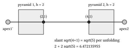
figure 153: the fixture: both squares, both apexes mirrored across the facing edges, the straight candidate threading both hinge midpoints
