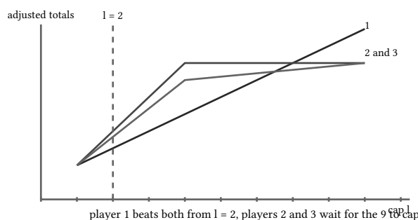
figure 132: the fixture's three adjusted-total lines over the cap axis, the cap 2 dashed vertical where player 1 first stands alone on top, the later crossover past player 1's 9
