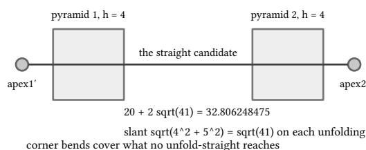
figure 140: the fixture: both squares, the unfolded apexes outside them, one straight candidate crossing both hinges
