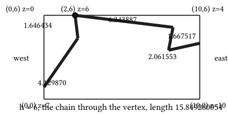
figure 173: terrain 3 in plan view, the corners and the north vertex labeled with elevations, and the level-6 west-east chain through the vertex (2,6) bolded
