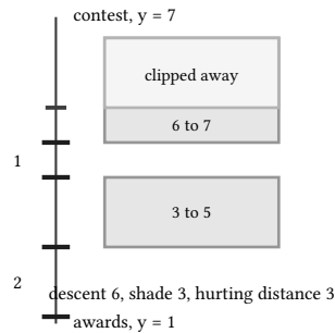
figure 181: the y-axis track, contest at 7 and awards at 1, the band 6 to 9 clipped at the contest's level, the band 3 to 5 whole, and the two unshaded gaps summing to 3
