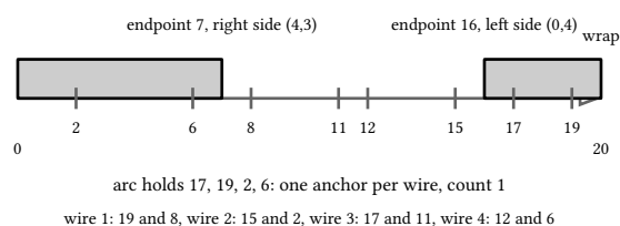
figure 110: sample 1's anchors unrolled on the perimeter ring: the winning arc from midpoint 16 wraps past corner 0 to midpoint 7 and holds exactly one anchor of each wire
