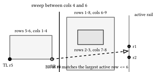
figure 98: the column sweep line between cols 4 and 6, the active top-left set as a row-ordered rail, one match arrow
