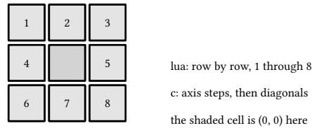
figure 74: the lua 8-neighbor order around a center cell, walked row by row, against the c axis-first order
