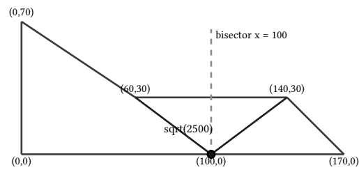
figure 108: sample 1's pentagon: the plateau bisector x = 100 crosses the bottom edge at (100,0) , exactly 50 from both plateau vertices, both triple points on the bisector falling outside
