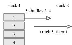
figure 135: one placement of the fixture: all four containers on stack 1, seven moves counted, expectation 6.000
