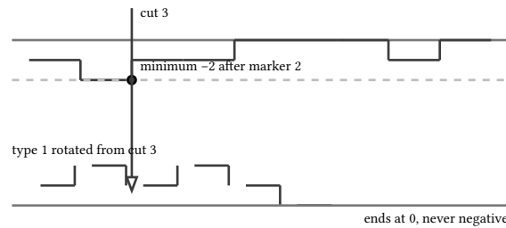
figure 120: type 1's prefix balance over the nine markers dipping to its minimum -2 after marker 2, and the rotated balance from cut 3 staying at or above zero
