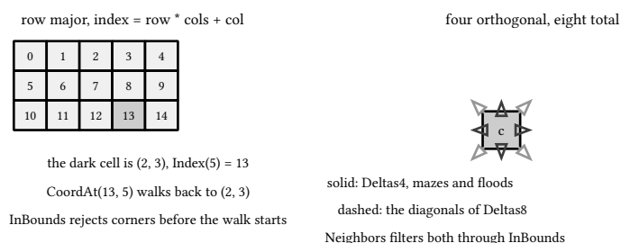
figure 30: row-major flattening and the two neighborhoods
