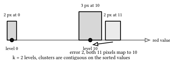
figure 89: the intensity line, three pixel masses, allowed values at 0 and 10, the error bar from 11
