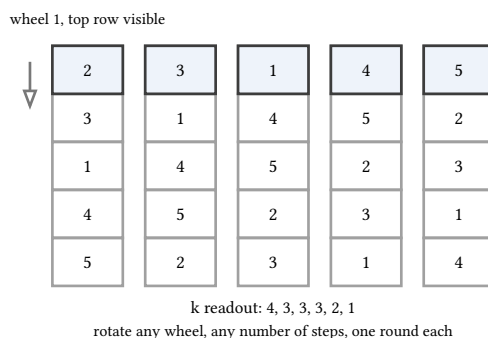
figure 176: five wheels as symbol columns with the visible row highlighted, one rotation arrow, and a distinct-count readout that shrinks toward 1 as rounds pass
