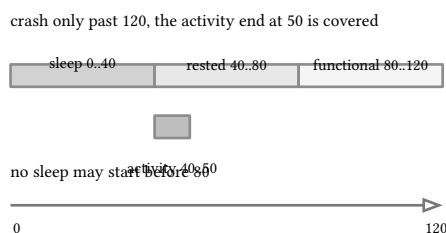
figure 159: the fixture: one full-gap sleep, its rested and functional stretches, the activity inside the window
