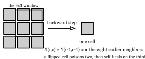
figure 91: the 3x3 block with the xor stencil centered on (1,1) collapsing to one cell, the arrow pointing backwards
