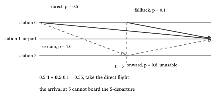
figure 99: the fixture on one clock: the certain bus reaches station 2 exactly at its onward departure, so the direct flight with the 0.1 fallback is the strategy that survives
