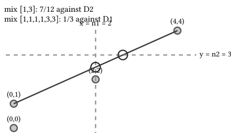
figure 151: the fixture's doubled points, the hull edge from (0,1) to (4,4), the two query lines and their winning points
