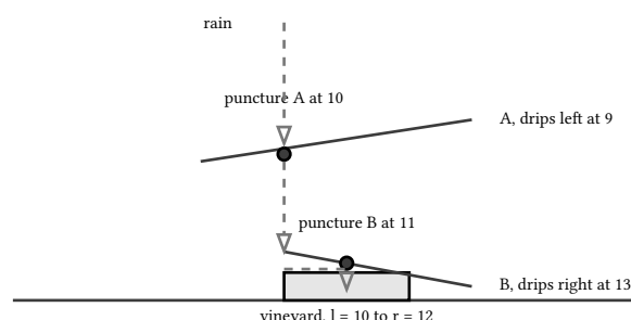
figure 125: the fixture's two tarps over the vineyard, the two punctures as dots, and the dashed drop path from above the field through both into the vineyard
