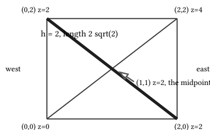
figure 174: the two triangles in plan view, elevations at the corners, and the level-2 polyline through (2,0) , (1,1) , (0,2) bolded
