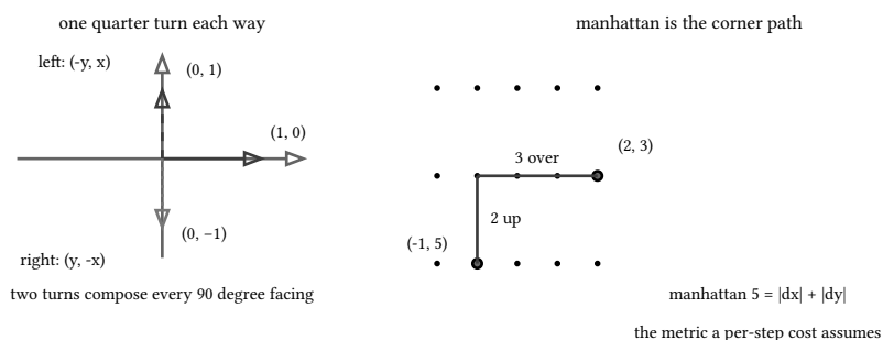
figure 41: quarter turns and the manhattan corner path
