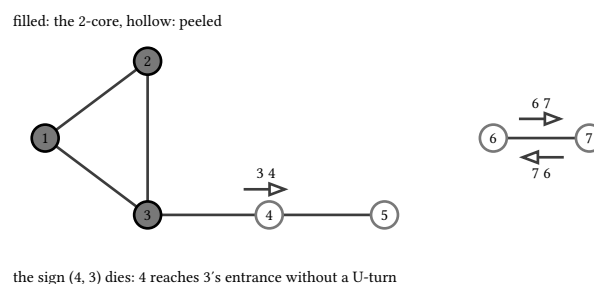
figure 123: the fixture graph: the triangle core keeps the sign at its boundary street, the two peeled vertices render hollow, and the isolated tree keeps both leaf signs
