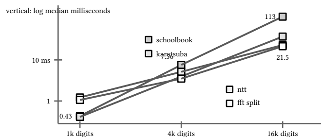
figure 191: lua medians, log milliseconds: karatsuba passes schoolbook between 1k and 4k digits, the transforms take over by 16k
