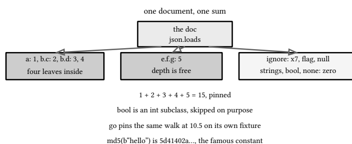
figure 64: the leaves sum to 15, the boolean is not a number
