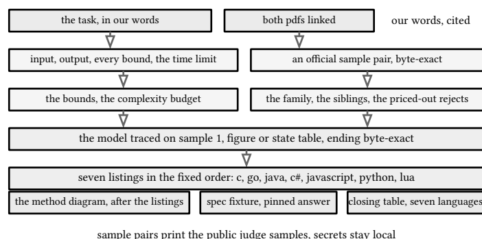
figure 4: the problem-chapter template: the task in our words, the contracts and bounds, an official sample pair, recognition, the worked run, seven listings in the fixed order, pinned answers, the closing table
