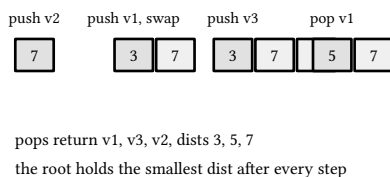
figure 45: the array under the dist comparator, one state per operation, the root always the smallest dist
