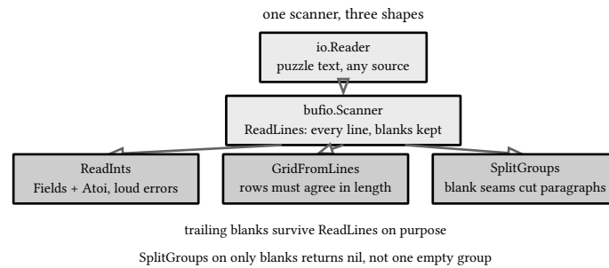
figure 28: one scanner, three downstream shapes
