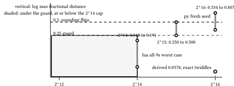
figure 189: measured fractional drift against the 0.25 guard and the 0.5 rounding cliff, the safe range shaded under the 2^{14} cap
