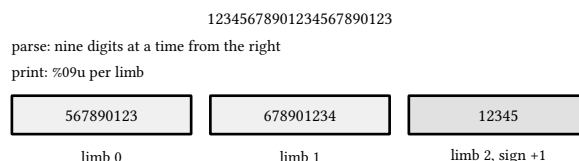
figure 8: the 23-digit fixture as three limbs, least significant first, and the nine-digit print width that reassembles it
