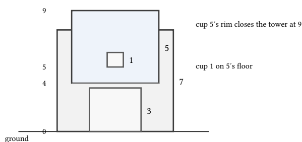
figure 177: cross-section of the sample tower, cup 7 on the ground, cup 3 on its floor, cup 5 on cup 3's rim, cup 1 hidden inside cup 5 on its floor, the spans labeled up to 9
