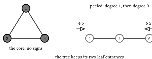
figure 122: sample 1: the triangle survives as the 2-core, the path 4-5-6 peels to a tree keeping only its two leaf signs
