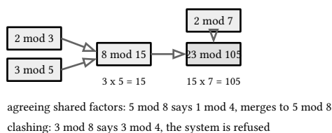
figure 32: the fold: two merges land the pinned class, and a shared-factor pair either collapses or is refused
