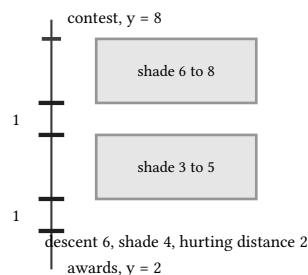
figure 182: the y -axis as a vertical track, contest and awards marked, the two shaded bands crossing it, and the unshaded gaps summing to 2
