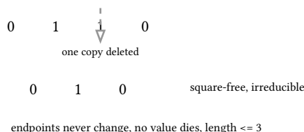
figure 146: the fixture: one of the doubled 1s removed, the irreducible result underneath
