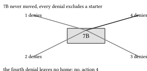
figure 145: four denials arranged around card 7B, the fourth closing the circle
