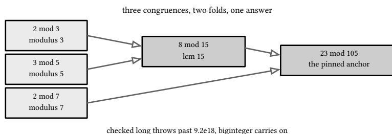
figure 44: the crt fold, pairwise combine grows the modulus toward the lcm
