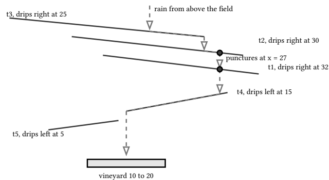
figure 124: sample 1's five tarps and the two-puncture trajectory: onto tarp 3, drip at 25 onto tarp 2, puncture onto tarp 1, puncture onto tarp 4, drip left at 15 into the field
