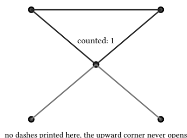
figure 112: sample 1's lattice: the one downward triangle the sweep counts, the bottom row's missing dash run killing the upward orientation
