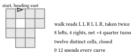
figure 142: the fixture's twelve-cell ring, start and heading marked
