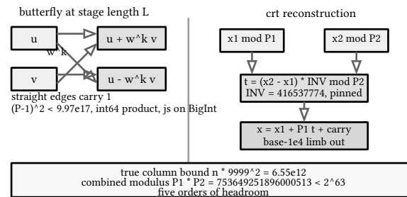
figure 187: one butterfly over w^k , then the CRT fold: two prime residues rebuilt into one column under the 2^{63} ceiling
