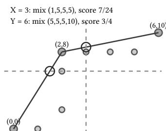
figure 150: sample 1's doubled score points, the three-vertex upper hull, the two query cuts and their winning mixes
