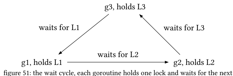
figure 51: the wait cycle, each goroutine holds one lock and waits for the next
