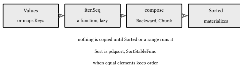
figure 65: iterators compose before anything materializes
