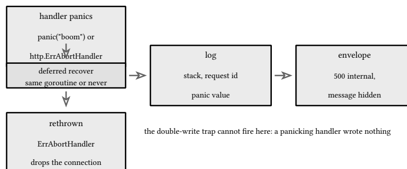
figure 109: panic unwind: one path to the log, one to the envelope, one rethrown
