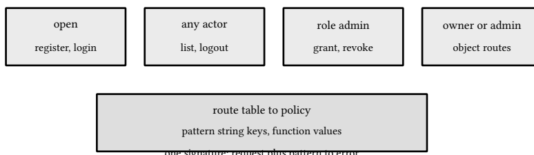
figure 132: four policies, one signature, the table maps routes onto them
