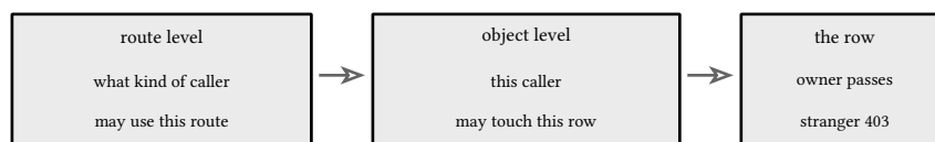
figure 158: route level versus object level, two doors on one request
