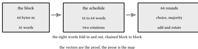
figure 145: one block through the digest: expand, mix, fold back into the eight words
