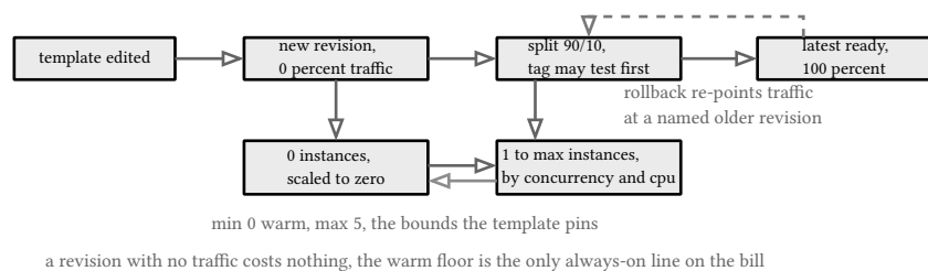
figure 118: the revision lifecycle as a state machine, with the scaling axis under every serving state
