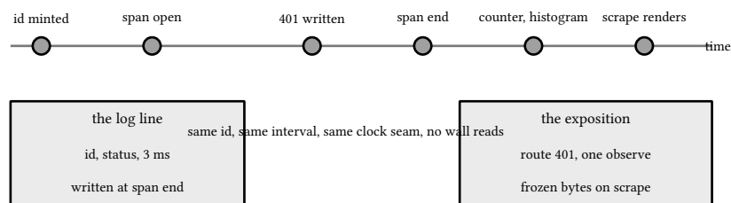
figure 198: one request through every signal, one id quoted everywhere
