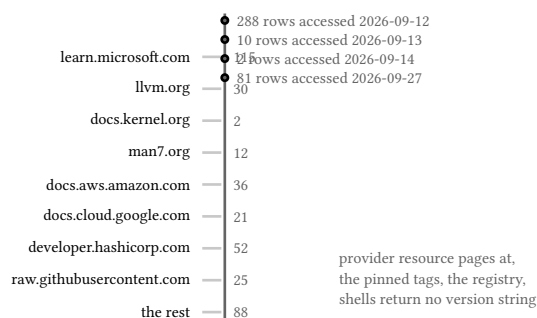
figure 222: the pin set on its access timeline: one circle per verification pass, one row per host family, the count beside each label computed from the array
