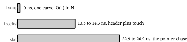
listing 234: the same million particles allocated behind bump, slab, and the chapter 14 freelist (source: c-os-cloud/samples/src/Ch21/kernel.c, lines 96-125)
