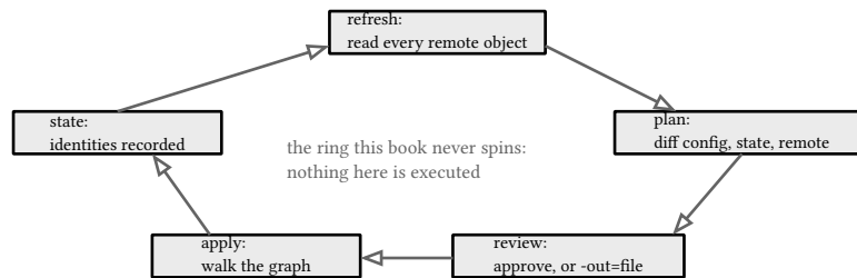
figure 103: the core loop as a ring: refresh reads, plan diffs, review gates, apply walks, state records
