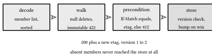
figure 141: a patch walks the members, then the precondition, then the store
