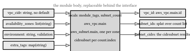
figure 105: the module as a data structure: variables enter left, outputs leave right, locals never leave
