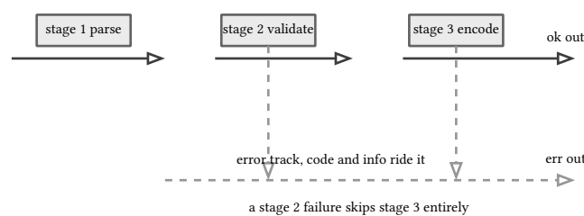
figure 164: the two track railway: stages on top, the dashed error track short circuiting stage 3
