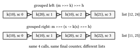
figure 173: evaluation order made visible: the same 4 calls in a different order give 12,24 against 11,25
