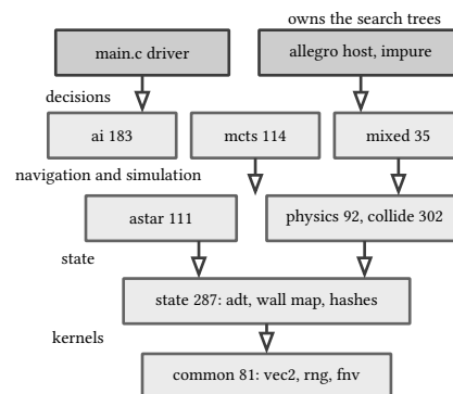
figure 181: the module map: the impure shells on top, decisions, navigation, simulation, and the state layer below, one direction of calls
