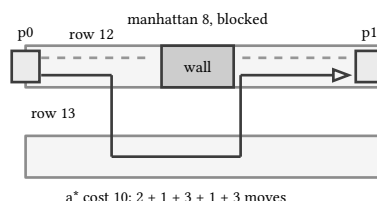
figure 189: spawn to spawn on rows 12 and 13: the straight manhattan line blocked by the center block, the 10-step detour below it
