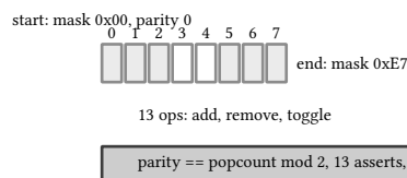
figure 79: before and after 13 mutations, the parity band asserted at each step
