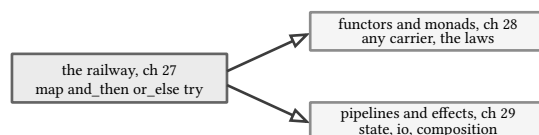
figure 167: the combinator core and the two chapters that generalize it
