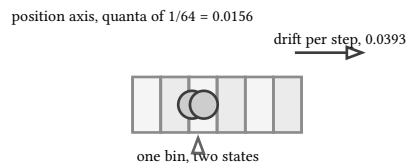
figure 194: quantization on a number line: two states inside one 1/64 bin collide, the per-step drift spans two and a half bins
