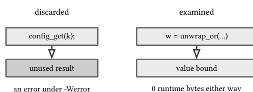
figure 165: two call sites, one diagnostic apart
