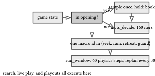
figure 184: the decision pipeline: one macro id per window, from the sampled opening book or the 160-iteration search, into the single execution path
