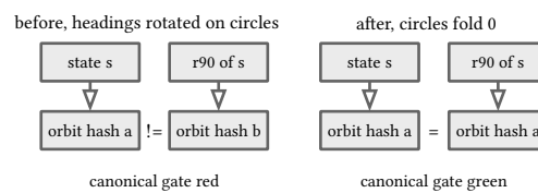
figure 190: the circle-heading bug: rotating a state's meaningless heading bits broke orbit equality, the fix folds them constant
