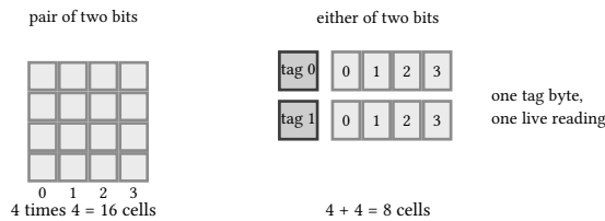
figure 156: inhabitants: a 4 by 4 pair grid against a 4 plus 4 tagged row, two bit cells
