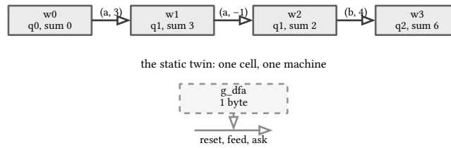
figure 176: the world threading above, the one byte static twin below
