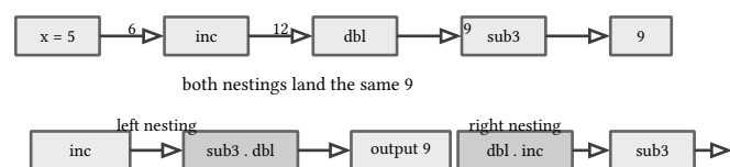
figure 174: the composed chain on top, the two associativity nestings below, same output
