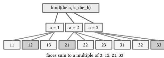
figure 171: the list monad as a tree: two dice enumerate 9 ordered pairs, the 3 darkened leaves survive the sum filter
