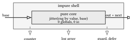
figure 178: the core takes and returns values only, the shell ring carries every effect
