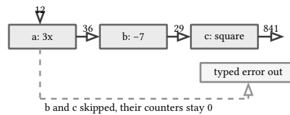
figure 170: the result railway: an error at any stage drops to the dashed rail and later stages never run
