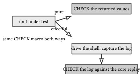
figure 179: the test route for a pure unit and for an effectful one
