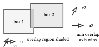
figure 187: the sat between two boxes: each candidate axis with the projected radii and the gap, the minimum overlap becoming the contact normal
