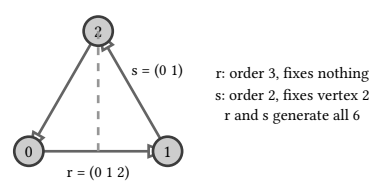
figure 99: the labeled triangle: the rotation r cycles all three vertex labels, the reflection s fixes vertex 2 and swaps 0 with 1, together generating all six symmetries
