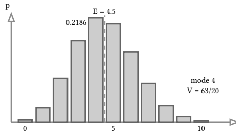
figure 111: binomial pmf bars for N = 15 , \mu = 0.3 , mean line at 4.5
