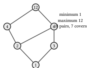
figure 91: hasse diagram of the divisors of 12, upward means divides, 7 covers carry 18 pairs
