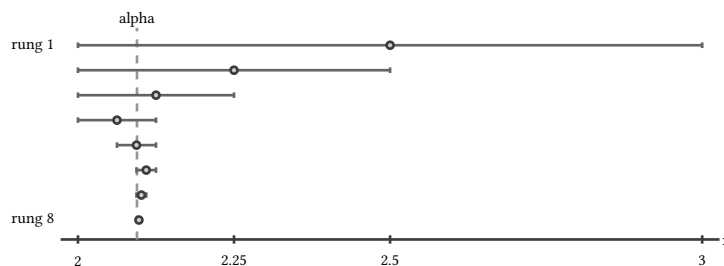
figure 120: nested brackets funnel onto alpha, each rung halves the interval that still certifies a root
