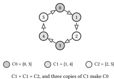
figure 101: z_6 as a ring of 6 residues: opposite pairs form the three cosets of \{0,3\} , shaded dark, medium, light, and they add like z_3
