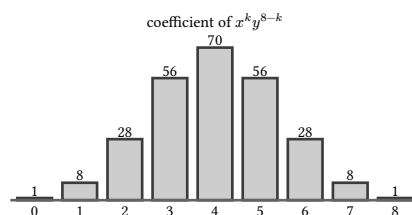
figure 83: coefficients of (x + y)^8 , the binomial row as a symmetric bar profile
