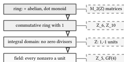
figure 103: the containment ladder from ring to field: z6 dies at zero divisors, z survives them but keeps only 1 and -1 invertible, z5 and gf(4) arrive at the field rung
