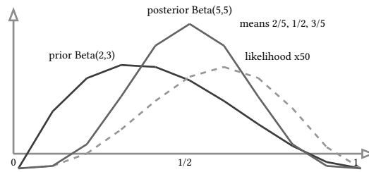
figure 113: prior, likelihood, and posterior on the coin weight
