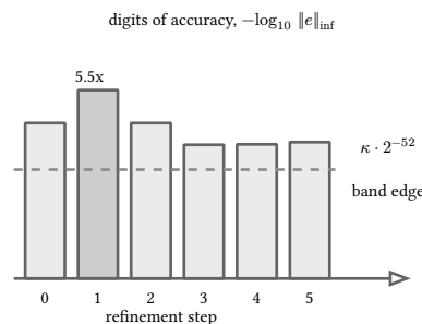
figure 143: the refinement ladder in digits of accuracy, one gain then wandering above the band edge
