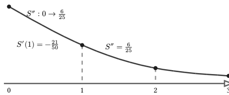
figure 130: the 4-knot fixture, one smooth curve from three cubics, second derivative continuous across the interior knots
