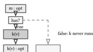
figure 169: bind over option: the tag decides, k runs only under some
