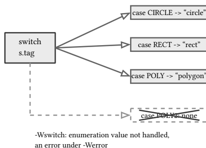
figure 158: exhaustive dispatch: three cases return, a fourth tag with no case stops the build
