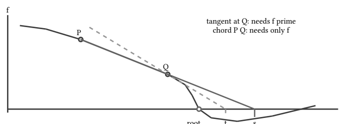
figure 123: the two local models on one curve: the tangent uses a point and its derivative, the chord uses two points, both aim at the next iterate
