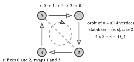
figure 105: the square under its own symmetry: r cycles the vertices, s holds 0 and 2 fixed across the diagonal
