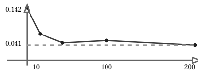
figure 149: average regret of the pinned run, decaying from 0.142 at round 10 to 0.041 at round 200
