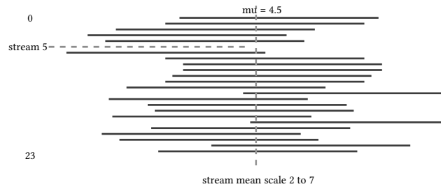
figure 118: the first 24 intervals against the true mean 4.5, stream 5 misses
