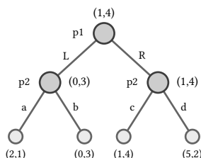
figure 150: fixture A in extensive form, rollback values beside each node
