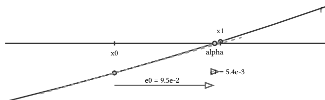
figure 122: tangent steps down the curve: each tangent crosses the axis at the next iterate, the error spans shrink quadratically
