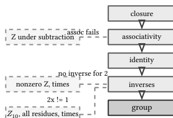
figure 94: the axiom gates: four checks in sequence, three near-miss structures dropping out where they fail
