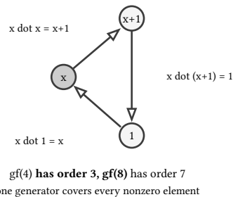
figure 104: the multiplicative group of gf(4) is a 3-cycle: multiplying by x walks x, x+1, 1 and closes
