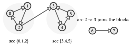
figure 89: D1: two 3-cycles, a bridge arc, and a tail, 4 strong components under 2 weak ones
