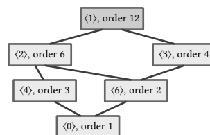
figure 96: the subgroup lattice of z_{12} , one subgroup per divisor of 12, edges are containment
