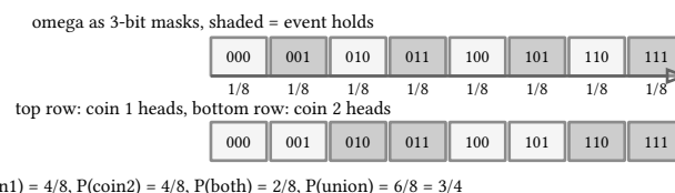
figure 108: bitmask events on the 8-outcome coin space, weight 1/8 each
