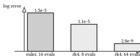
figure 135: integration error against evaluation budget on the logistic fixture, log scale heights
