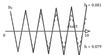
figure 134: ten euler steps on the decay fixture, h = 0.081 grows to 1.28 while h = 0.079 decays toward the exact solution, flat zero on this scale
