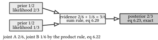
figure 87: bayes on the two-urn table, joints by the product rule, evidence by the sum rule
