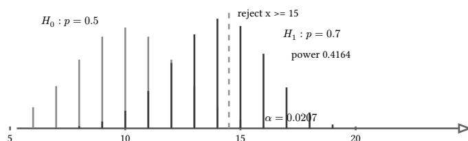
figure 117: the two binomials behind the test, rejection region x \geq 15 shaded darker
