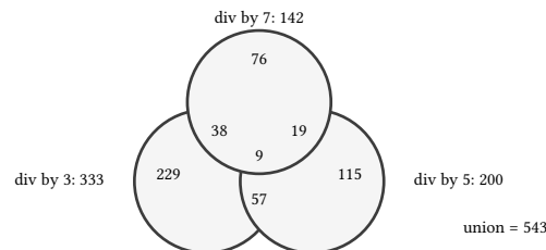
figure 84: the three-set venn for 1..1000 divisible by 3, 5, 7, region counts netting to 543
