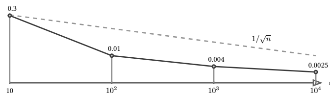
figure 114: the llm ladder on one fixed stream, deviation against n, with the 1/sqrt(n) guide
