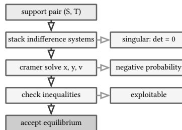
figure 148: support enumeration as a decision flow, each pair solved then filtered by singular, negative, and exploitability gates
