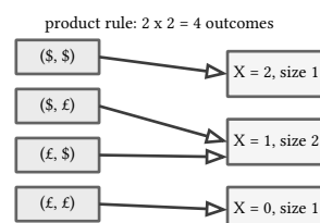
figure 81: the example 6.1 mapping, 4 outcomes of the product space collapsing onto 3 states with pre-image sizes 1, 2, 1
