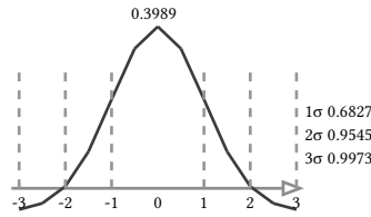
figure 112: standard gaussian with the 1, 2, and 3 sigma bands
