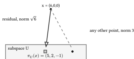
figure 41: the projection is the foot of the perpendicular, everything else on U is farther
