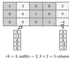
figure 36: pivot columns shaded, free columns light, each free column generates one null space witness
