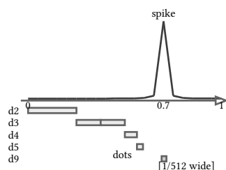
figure 133: the spike fixture true to scale with its leaf intervals stacked by depth below, the census clustering under 0.7, the depth 9 bar enlarged to stay visible
