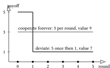
figure 154: stage payoffs by round at delta 2/3, flat 3 for cooperation against 5 then 1 for deviation
