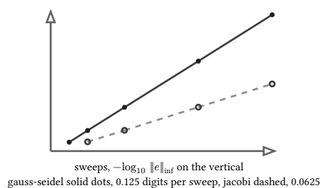
figure 139: digits of accuracy gained per sweep, gauss-seidel climbing at twice jacobi's slope
