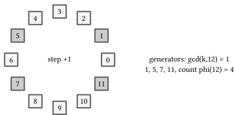
figure 97: the z12 residue wheel, the four coprime residues shaded as the generators, count \text{phi}(12) = 4
