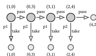
figure 151: the centipede, take drops out and pass chains right, rollback value above each node
