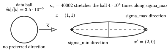
figure 142: the input ball mapped through the matrix to a kappa-stretched ellipse, the flip as one endpoint
