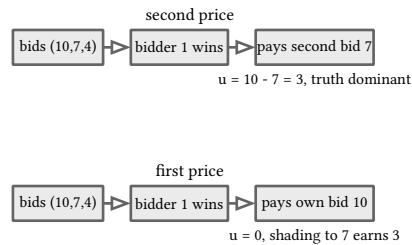
figure 155: the same bids under two payment rules, truth pays 3 at second price and 0 at first price
