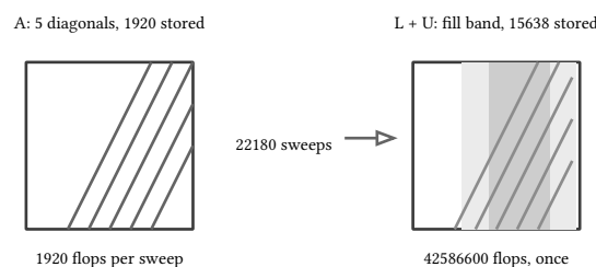
figure 138: the sparsity of the stencil against the fill band of its LU factors
