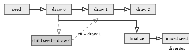
figure 177: the parent stream, the naive handoff rejoining it, the finalized branch diverging
