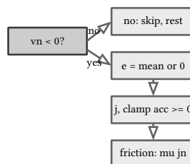
figure 188: one contact in one solver pass: the three gates in order, approach speed, restitution threshold, friction bound
