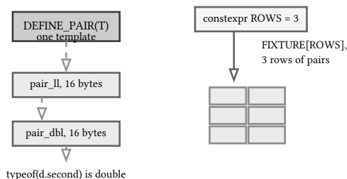
figure 159: one macro stamps every pair type, constexpr sizes the fixture, typeof picks the field type
