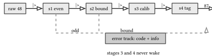
figure 175: the happy track with the macro sugar, the dashed error track bypassing the later stages
