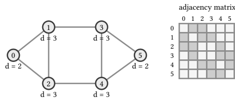
figure 88: G1 with its degrees and adjacency matrix, 36 cells holding 8 edges
