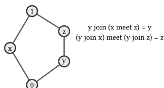
figure 92: the pentagon N_5 : every pair joins and meets, distributivity fails on the witness triple
