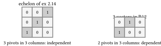
figure 28: pivot patterns, every column carrying a pivot against one column left over
