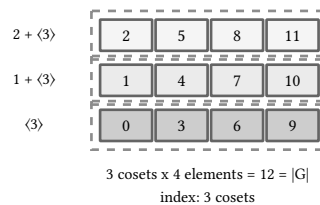
figure 98: the coset tiling of z12 by \langle 3 \rangle : three disjoint translates of size 4 covering all 12 residues
