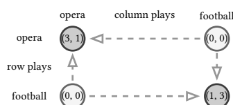
figure 145: battle of the sexes deviation arrows, both miscoordinate profiles have a profitable unilateral move and drain into the two shaded equilibria
