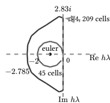
figure 136: the absolute stability regions on the h\lambda plane at equal scale, euler a disk of radius 1 inside the rk4 region reaching past minus 2.78
