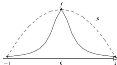
figure 126: the runge bump on three nodes and its exact parabola, agreeing at the nodes and nowhere else
