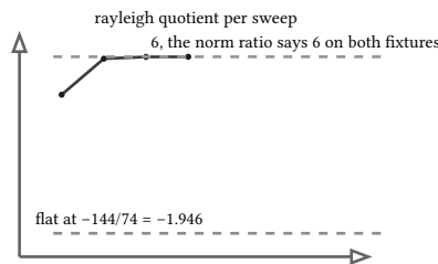
figure 141: the rayleigh quotient per sweep, one ladder climbing to 6, the equal-magnitude fixture flat at -1.946
