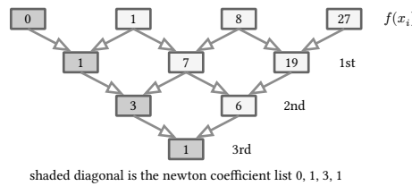
figure 127: the divided-difference triangle, its diagonal marked as the newton coefficient list
