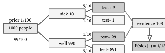
figure 109: bayes tree for the screening table, counts out of 1000
