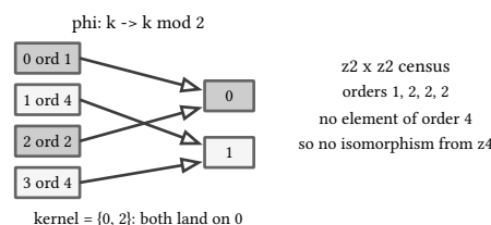
figure 100: the parity map collapses z_4 onto z_2 with kernel \{0, 2\} , while the order census separates z_4 from z_2 \times z_2 with no map at all
