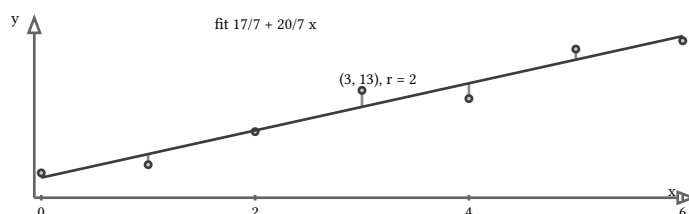
figure 119: the fit y = 17/7 + 20/7 x through seven integer points with residuals
