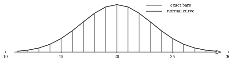
figure 115: binomial(40, 1/2) as exact bars with the normal curve through the bar tops
