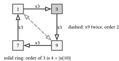
figure 95: the power cycles of u(10) : multiplying by 3 walks a 4-cycle, the sub-ladder of 9 collapses to a 2-cycle
