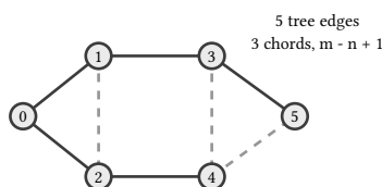
figure 90: G1 with the pinned spanning tree solid and its 3 chords dashed
