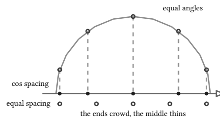
figure 129: chebyshev nodes as equal angles projected onto the axis, against equally spaced dots
