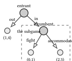
figure 152: entry deterrence, the dashed box is the incumbent subgame where the threat fails
