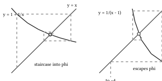
figure 121: two cobwebs for one equation: the convergent staircase into phi on the left, the repelling orbit that escapes on the right
