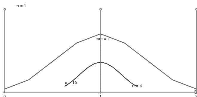
figure 116: the exact distribution of the sample mean sharpening with n , uniform \{0,1,2\} population
