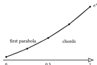
figure 132: the e^x fixture with 4 trapezoid chords and the first simpson parabola over [0, 0.5]
