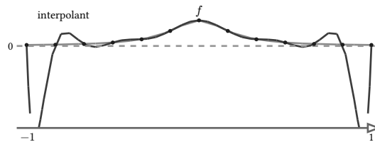
figure 128: degree 12 interpolation of the runge bump on 13 equally spaced nodes, plunging out of frame near both ends
