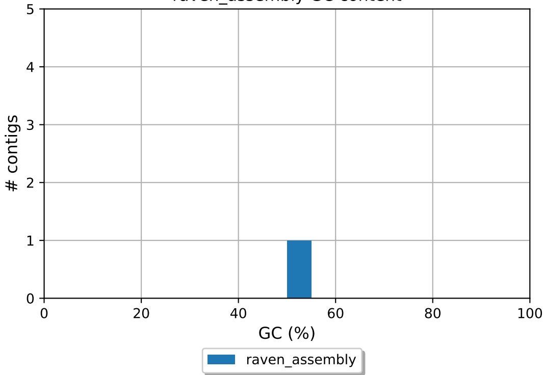
raven_assembly GC content
