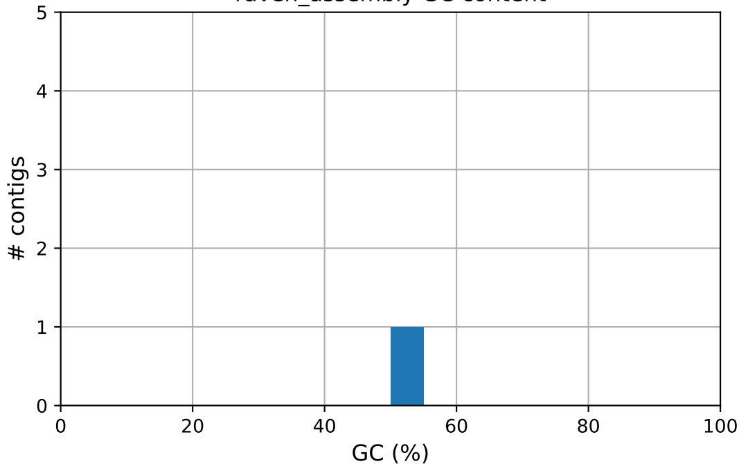
raven_assembly GC content
