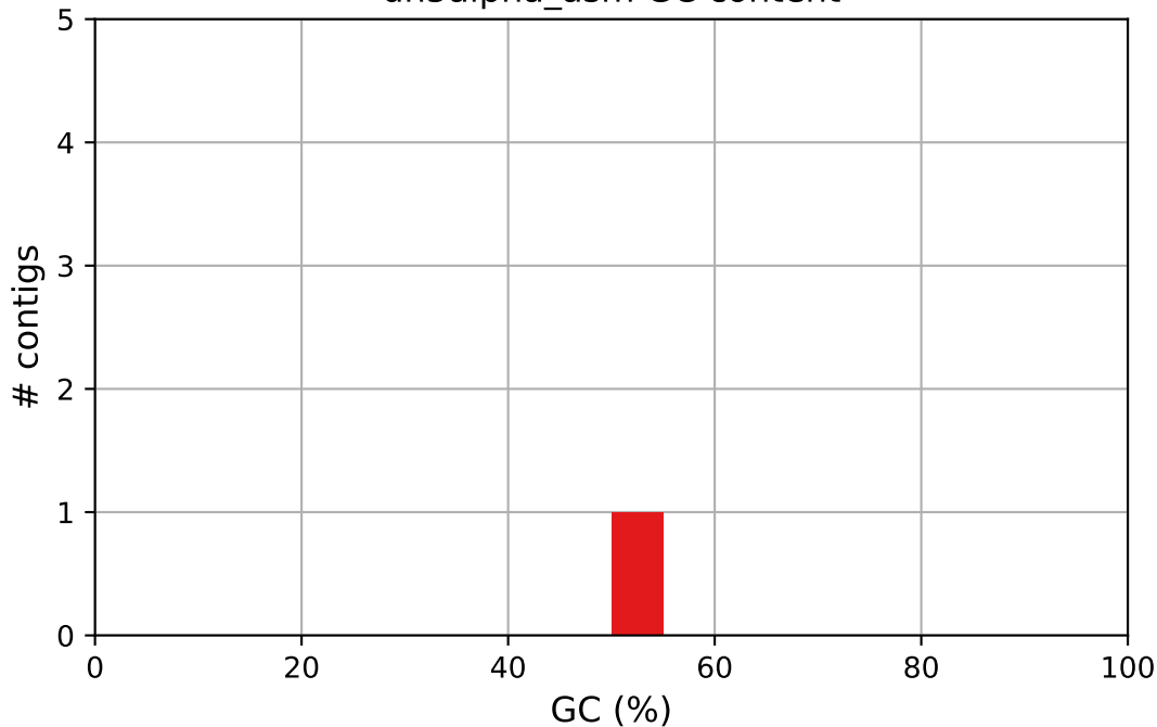
dh5alpha_asm GC content
