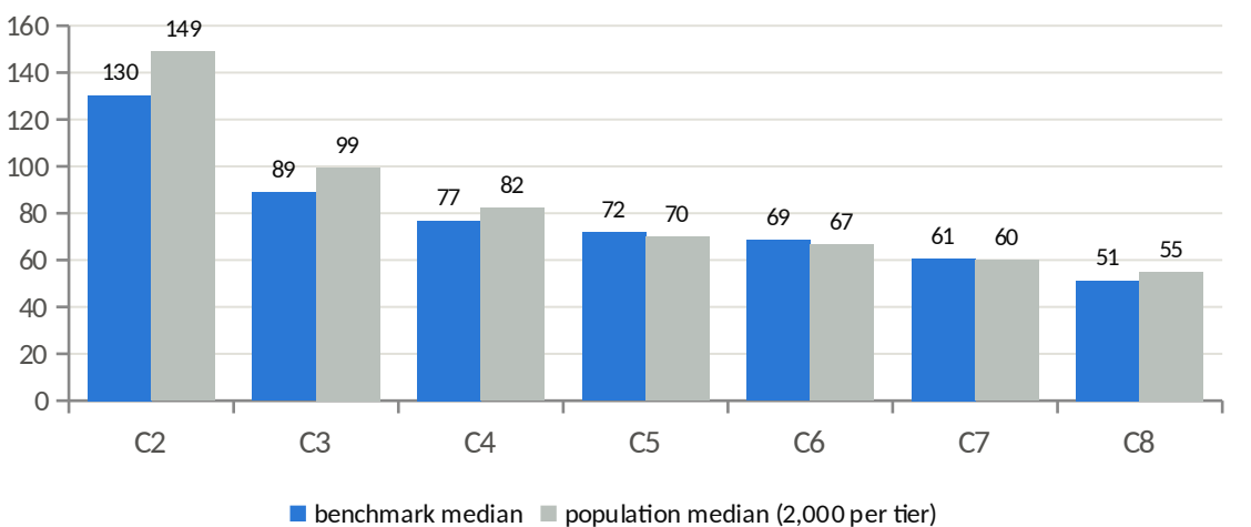
Tighter with the tier: median closest clear gap (mm)
