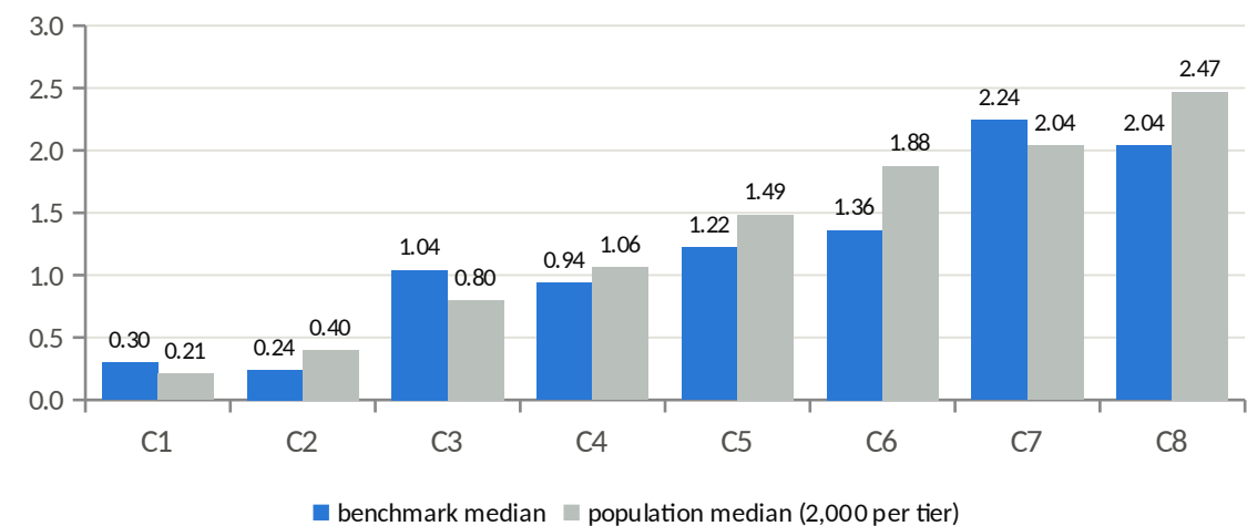
Heavier with the tier: median load at the support (kN)
