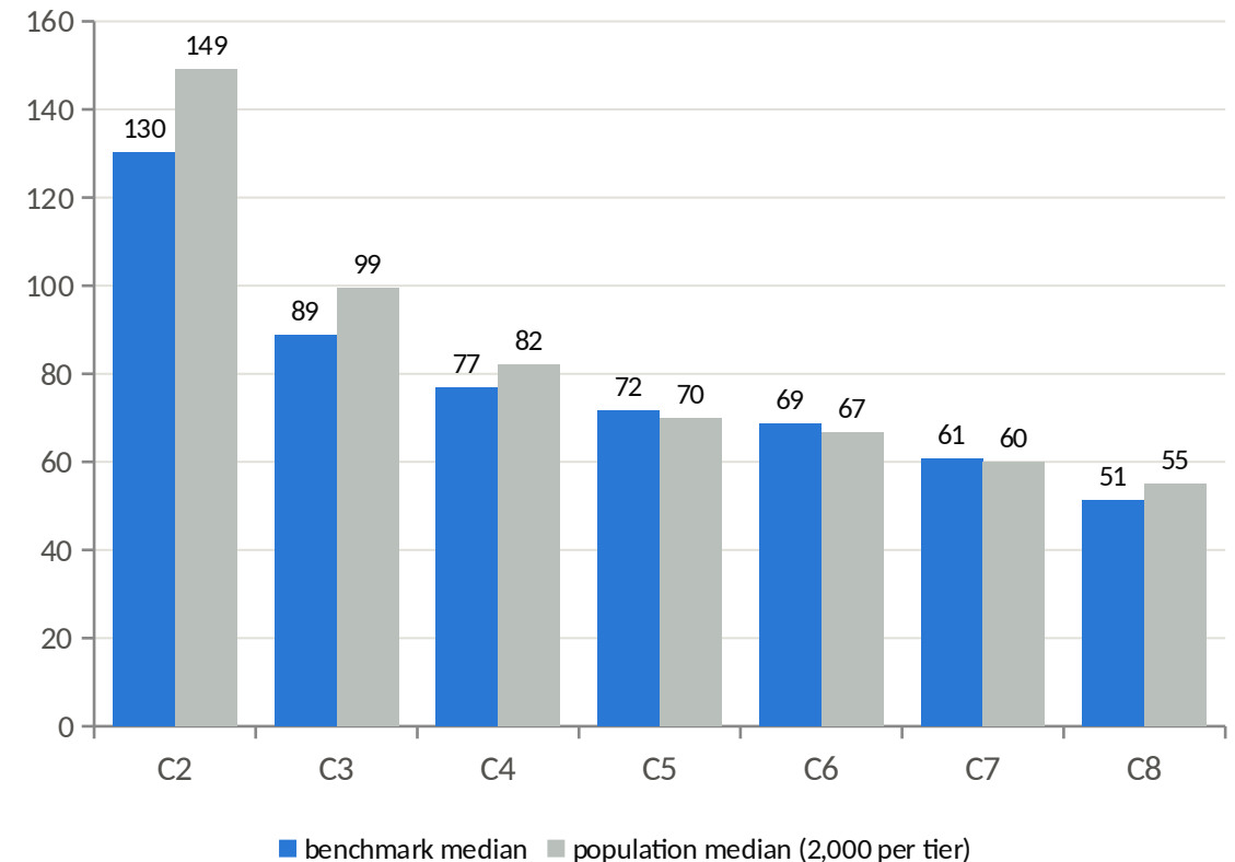
Tighter with the tier: median closest clear gap (mm)
