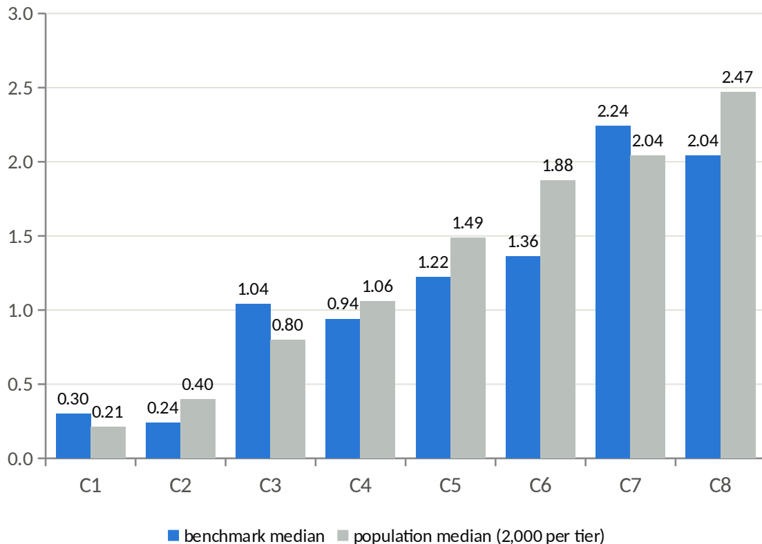
Heavier with the tier: median load at the support (kN)
