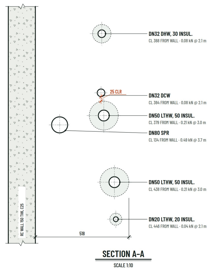
Tier C6, seed 0, section 5: six pipes fixed to a wall; offsets from the wall face, the closest clear gap 25 mm.
