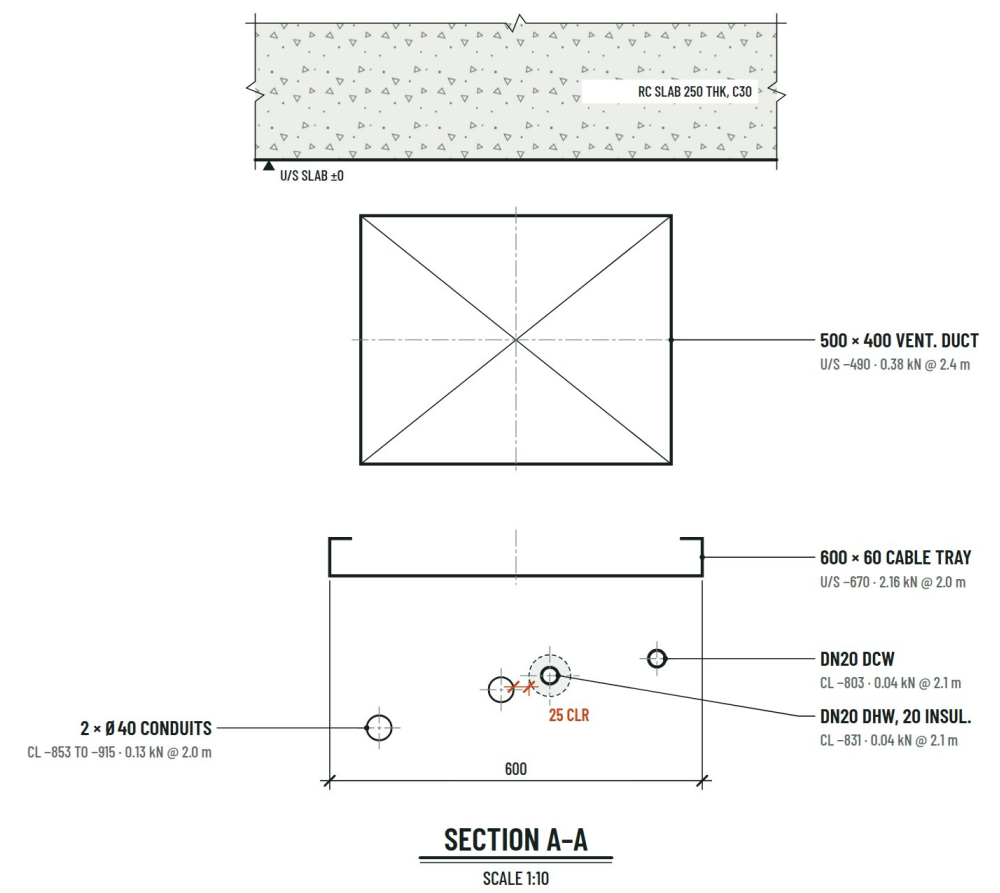
Exact mix: 2 pipes, 1 tray, 1 duct, 2 conduits on a slab; levels below the soffit and the load at the support.
