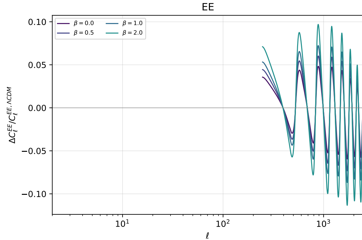
Forward-model \beta sweep at c_D = 8.0 , c_{s,X}^2 = 0.5 (Phase 3 pre-flight §5.1)
