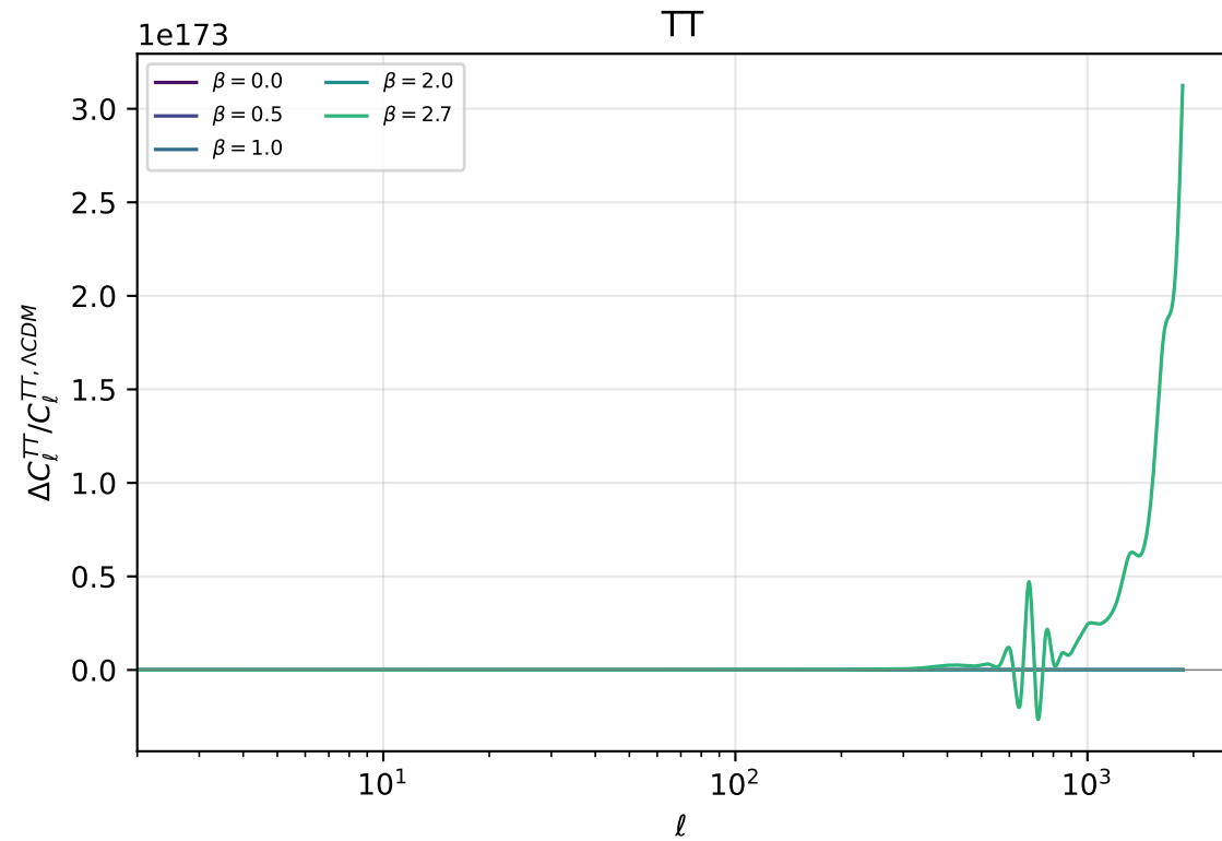
Forward-model \beta sweep at c_D = 8.0 , c_{s,X}^2 = 0.5 (Phase 3 pre-flight §5.1)
