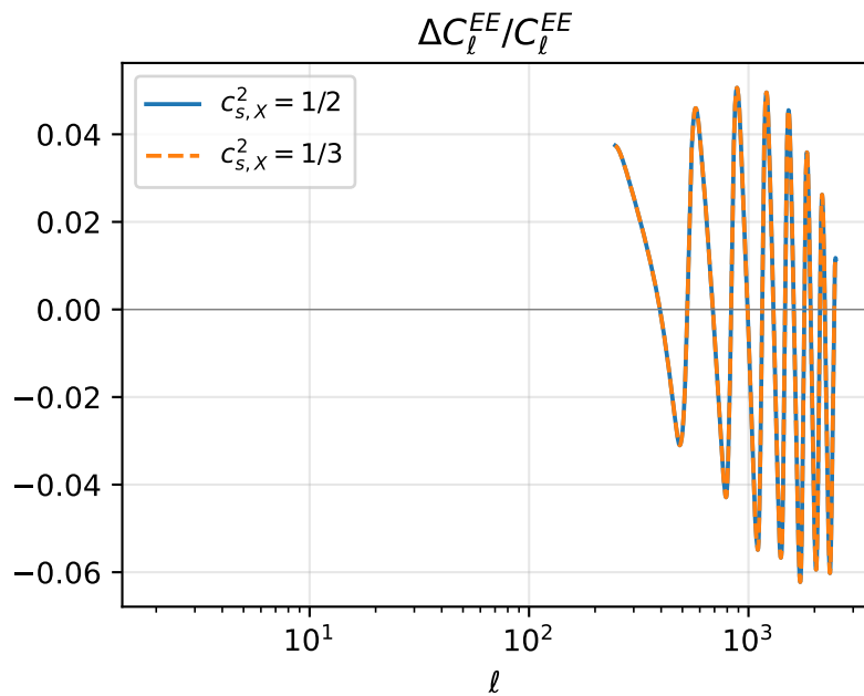
c_{s,x}^2 sensitivity at \beta = 0.1 , c_D = 8.0 (Phase 3 decision 2 probe)
