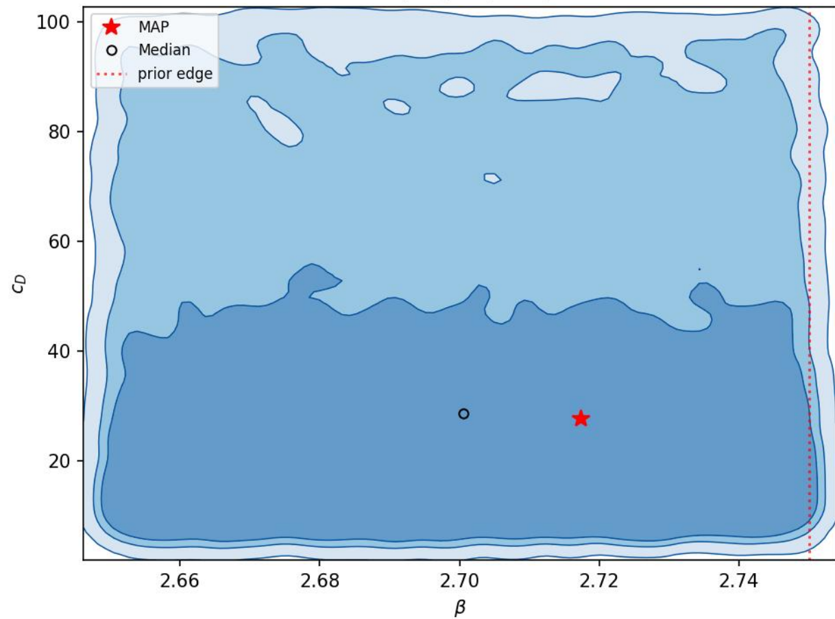
3c: \beta \in [2.65, 2.75]
