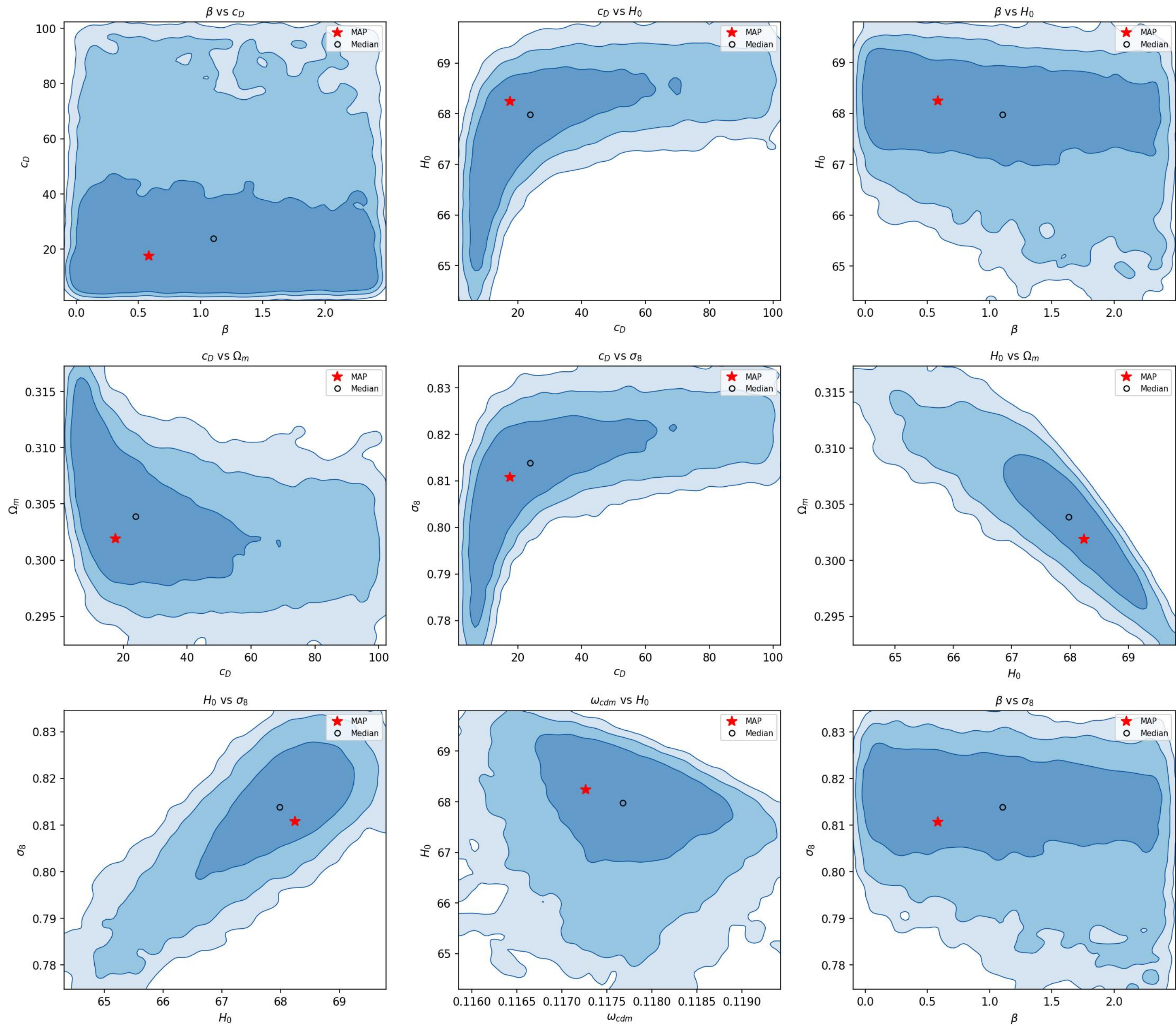
3b ( \beta \in [0, 2.4] , non-crossing) — 2D marginals
