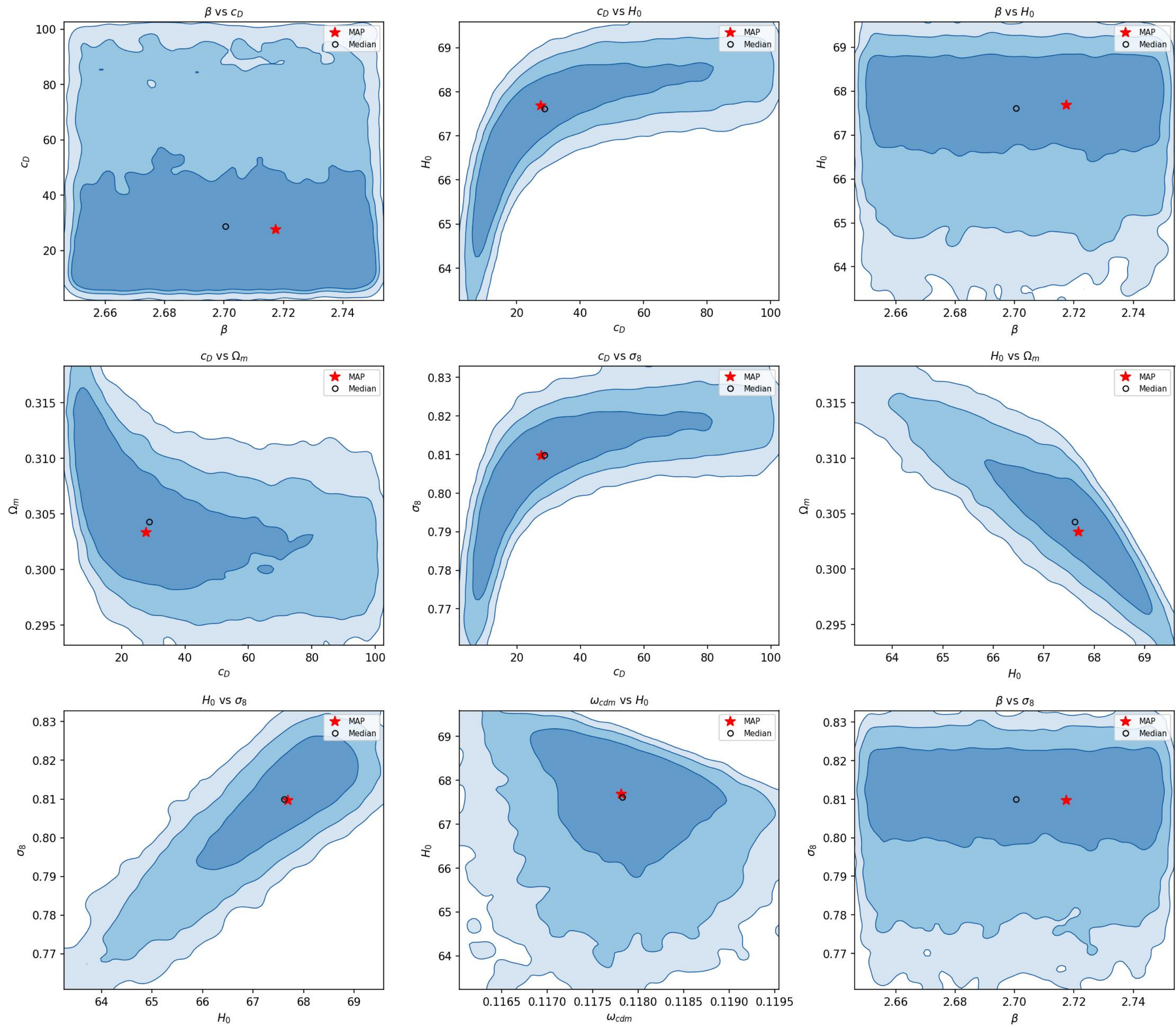
3c ( \beta \in [2.65, 2.75] , B1-narrow) — 2D marginals
