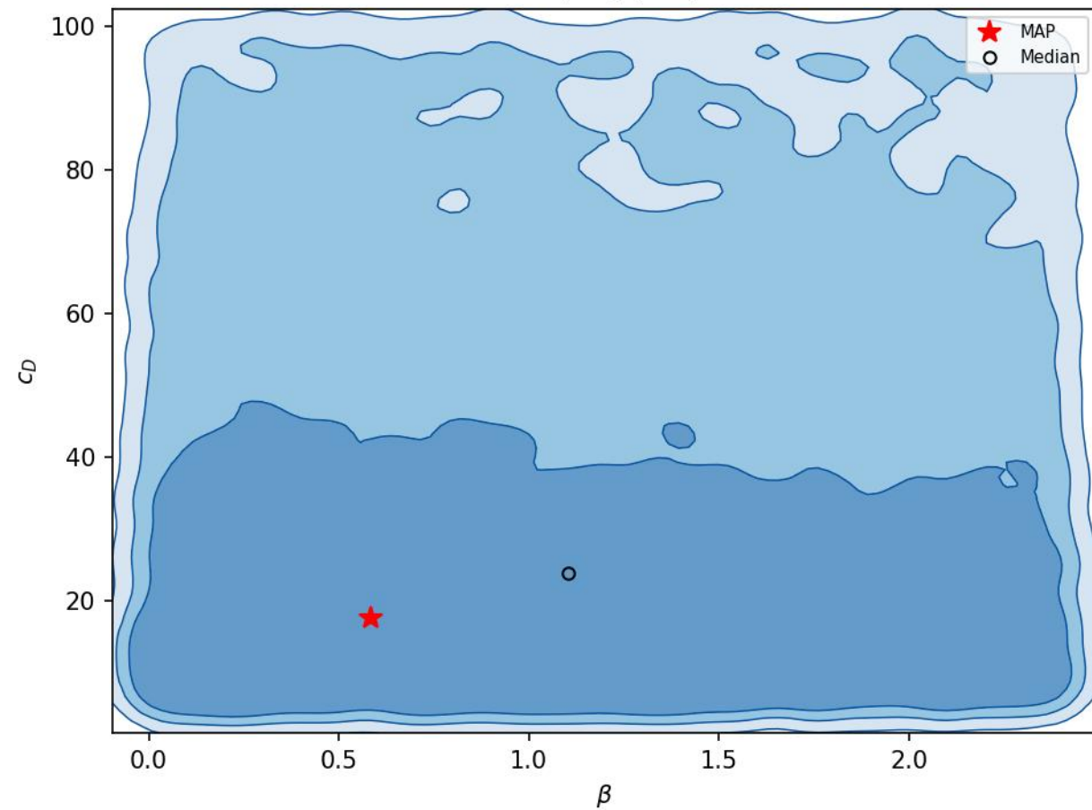
3b: \beta \in [0, 2.4]
