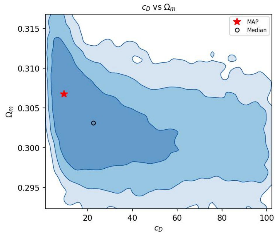
3a ( \beta = 0 , baseline) — 2D marginals
