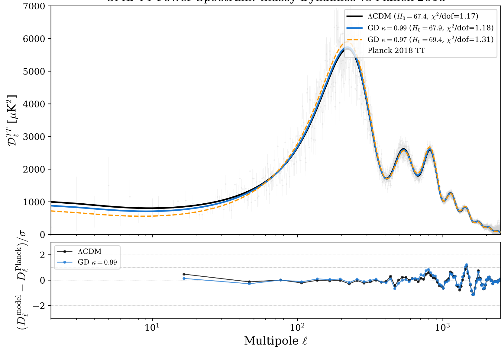
CMB TT Power Spectrum: Glassy Dynamics vs Planck 2018
