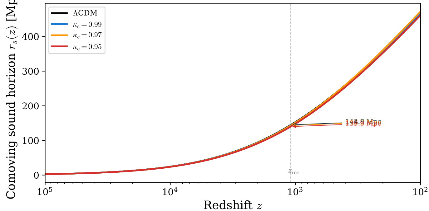
(a) Sound horizon accumulation
