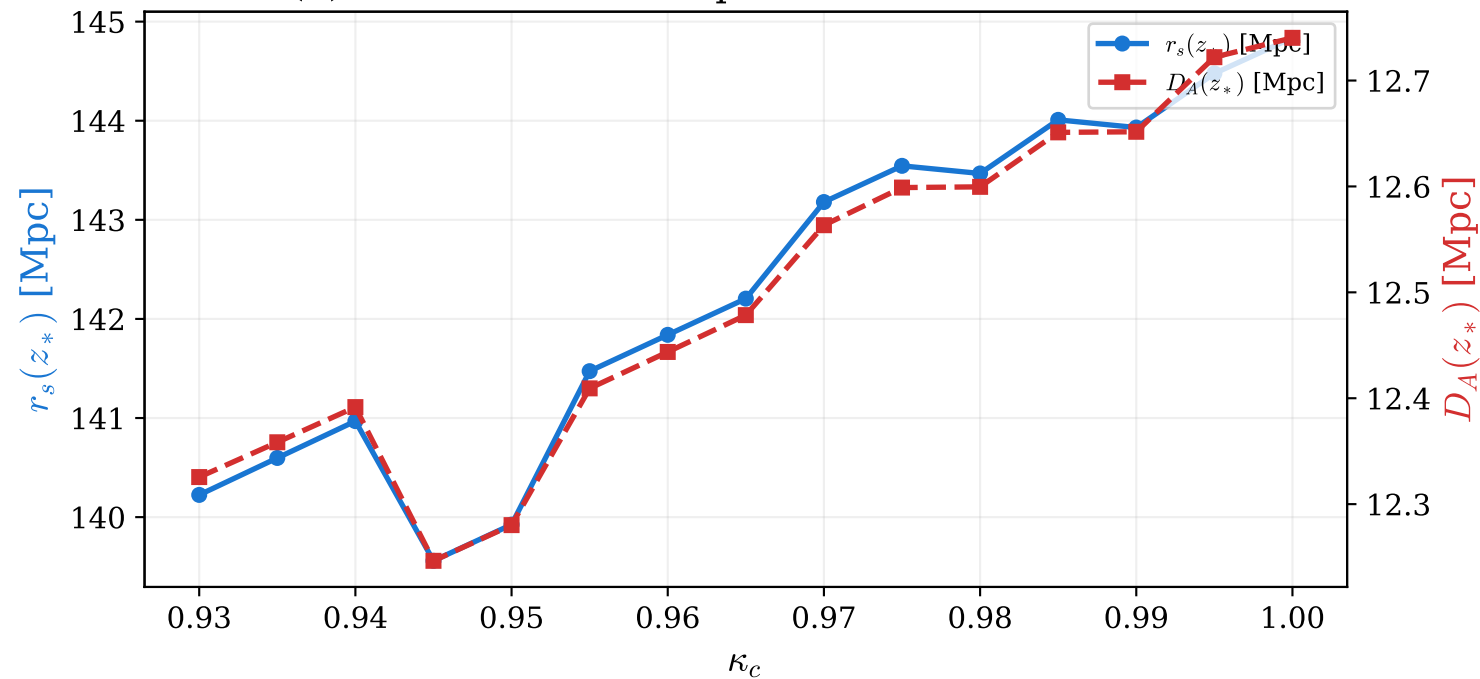
(b) Acoustic scale components at recombination
