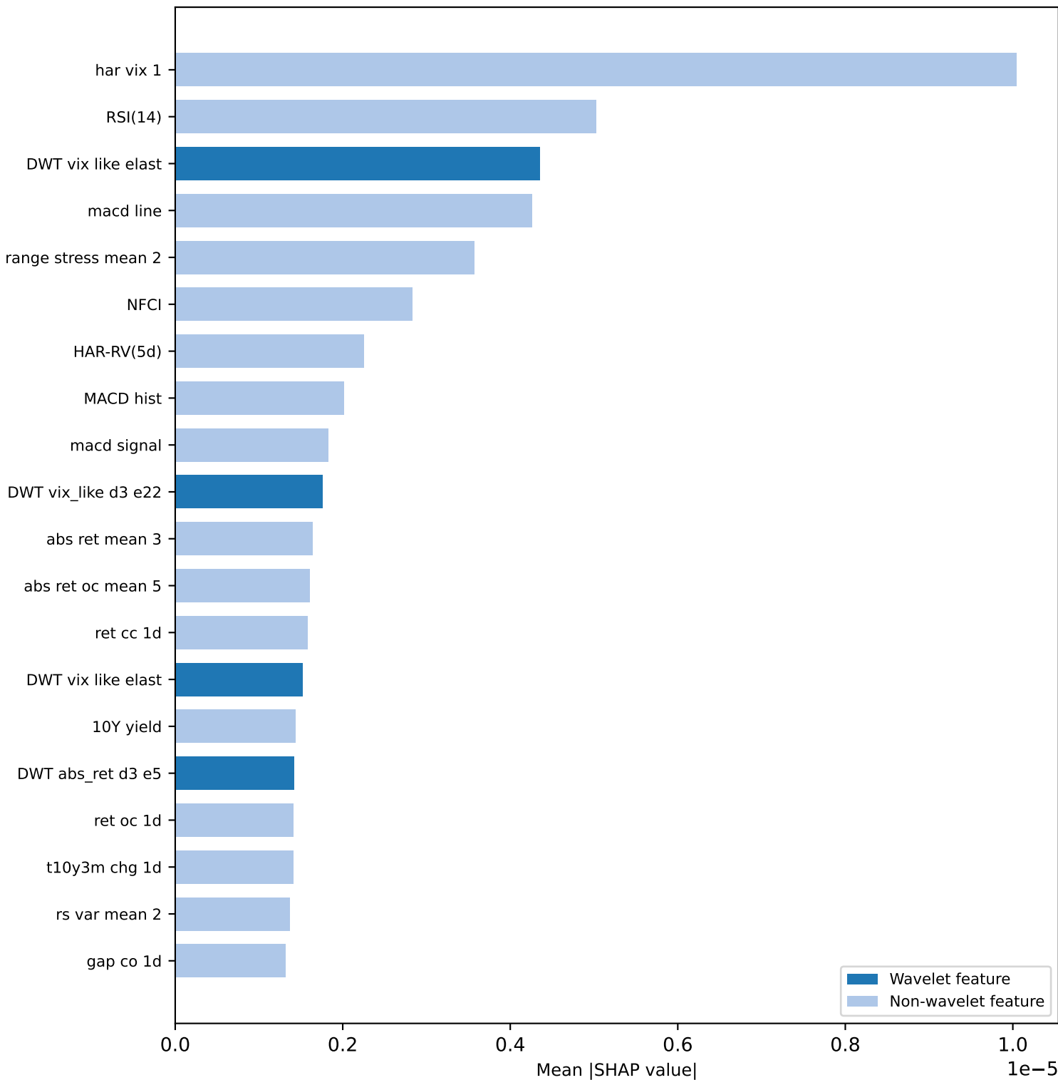
SHAP feature importance — wavelet\lightgbm SPX · h=1d · top-20
