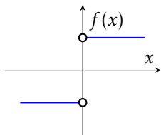
Figure 2.4: The derivative of the absolute value function.
